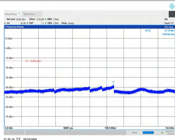
Band5_10MHz_QPSK_20600_1RB#0_3000~10000_3000~1000
