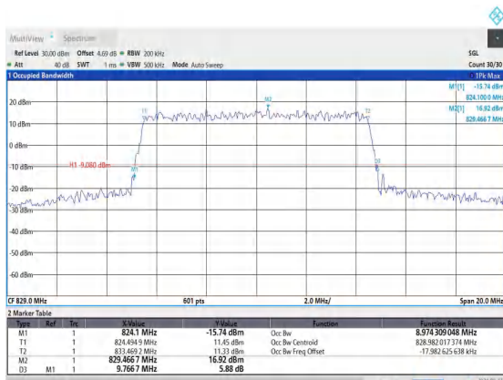
Band5-10MHz-QPSK-20450-50RB#0-PASS
