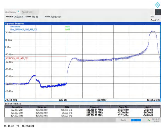
Band5_3MHz_QPSK_20415_1RB#14
