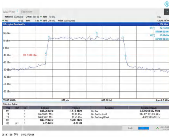
Band5-3MHz-QPSK-20635-15RB#0-PASS
