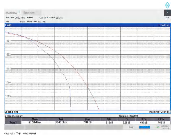
Band5-1.4MHz-16QAM-20525-6RB#0-PASS
