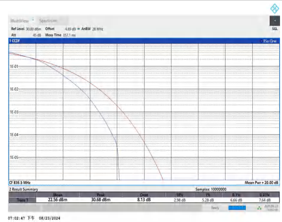
Band5-10MHz-16QAM-20525-50RB#0-PASS
