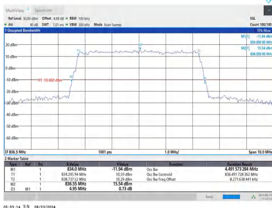
Band5-5MHz-16QAM-20525-25RB#0-PASS
