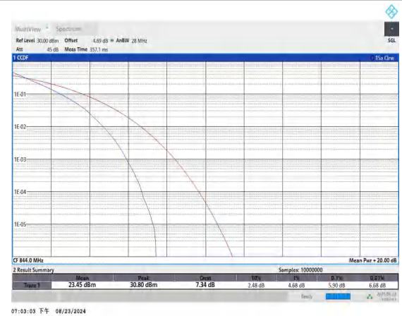
Band5-10MHz-QPSK-20600-50RB#0-PASS
