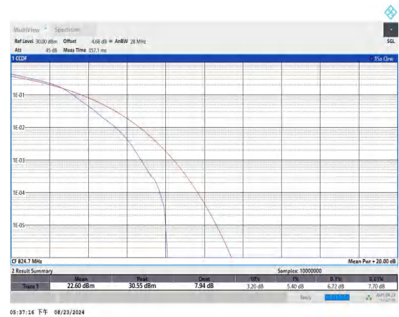
Band5-1.4MHz-16QAM-20407-6RB#0-PASS
