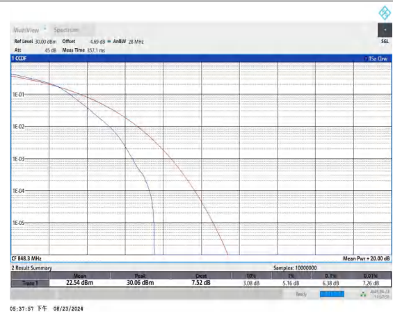
Band5-1.4MHz-16QAM-20643-6RB#0-PASS
