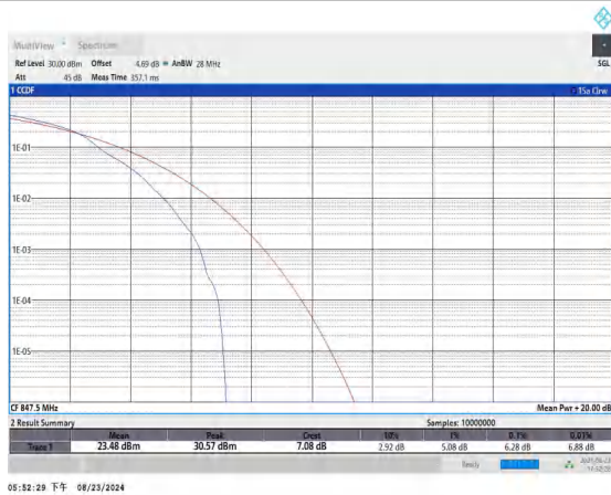
Band5-3MHz-16QAM-20635-1RB#0-PASS
