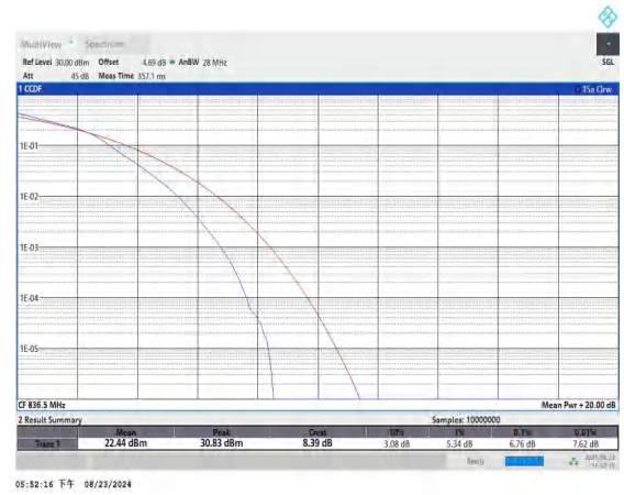
Band5-3MHz-16QAM-20525-15RB#0-PASS
