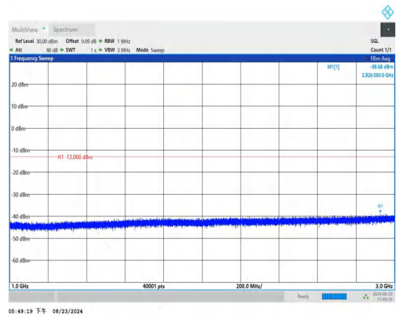
Band5_3MHz_QPSK_20525_1RB#0_1000~3000_1000~3000
