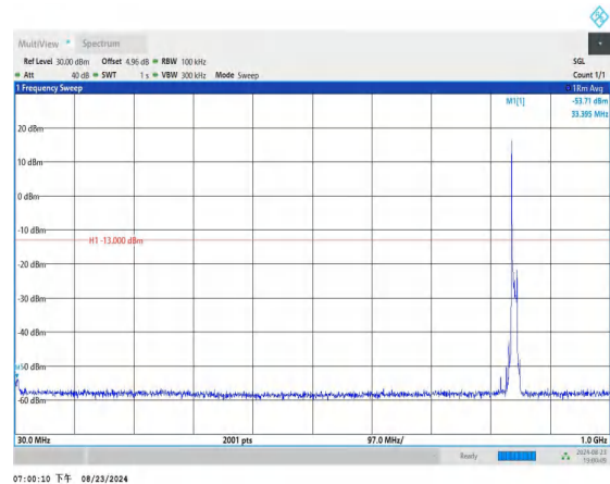
Band5_10MHz_QPSK_20600_1RB#0_30~1000_30~1000
