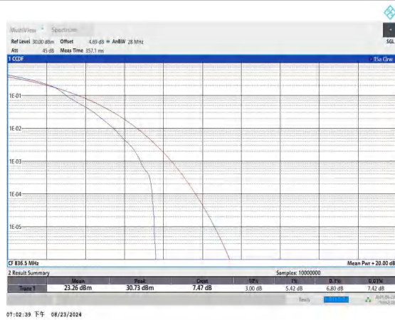
Band5-10MHz-16QAM-20525-1RB#0-PASS
