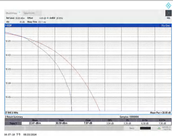
Band5-5MHz-16QAM-20625-25RB#0-PASS
