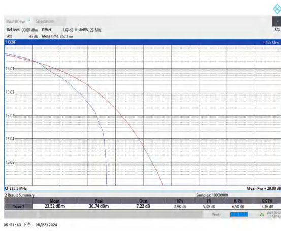
Band5-3MHz-16QAM-20415-1RB#0-PASS
