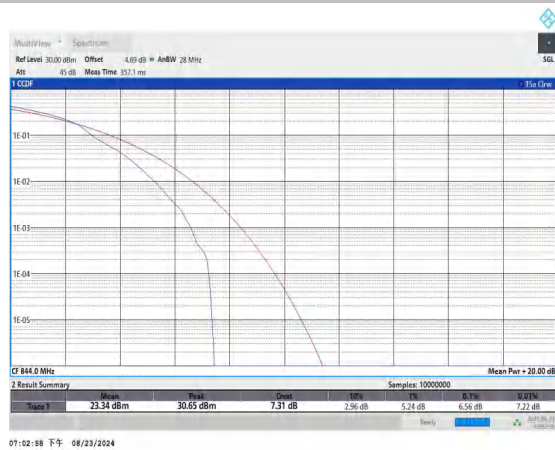
Band5-10MHz-16QAM-20600-1RB#0-PASS
