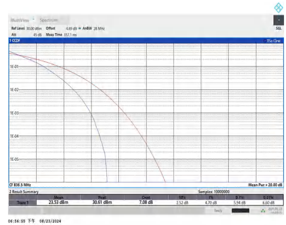
Band5-5MHz-QPSK-20525-25RB#0-PASS
