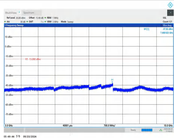
Band5_3MHz_QPSK_20635_1RB#0_3000~10000_3000~10000
