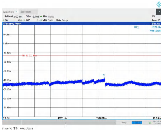
Band5_10MHz_QPSK_20525_1RB#0_3000~10000_3000~1000
