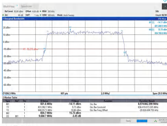
Band5-10MHz-16QAM-20525-50RB#0-PASS
