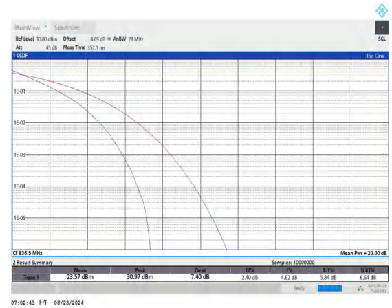
Band5-10MHz-QPSK-20525-50RB#0-PASS
