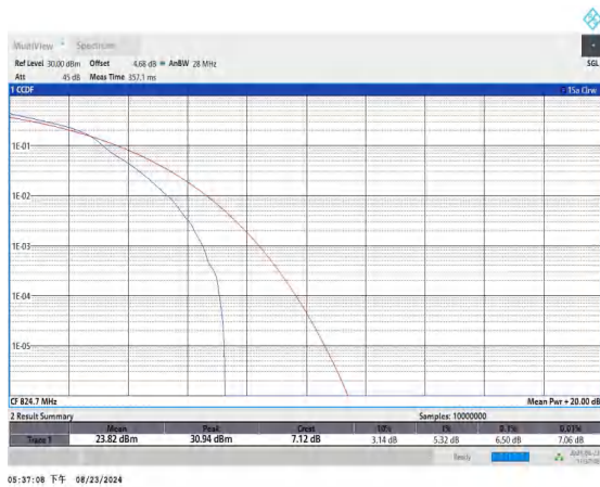
Band5-1.4MHz-16QAM-20407-1RB#0-PASS
