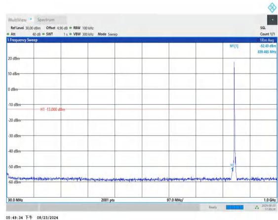
Band5_3MHz_QPSK_20635_1RB#0_30~1000_30~1000
