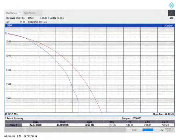
Band5-3MHz-16QAM-20415-15RB#0-PASS
