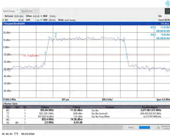
Band5-3MHz-16QAM-20525-15RB#0-PASS
