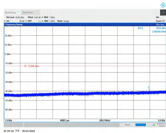
Band5_10MHz_QPSK_20525_1RB#0_1000~3000_1000~3000
