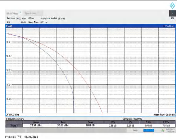
Band5-10MHz-16QAM-20600-50RB#0-PASS
