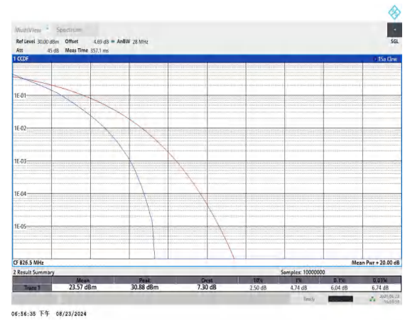
Band5-5MHz-QPSK-20425-25RB#0-PASS
