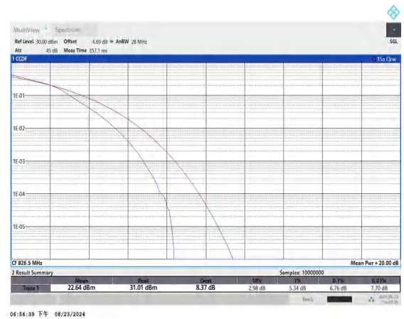
Band5-5MHz-16QAM-20425-25RB#0-PASS
