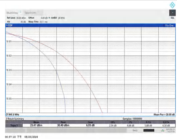
Band5-5MHz-QPSK-20625-25RB#0-PASS
