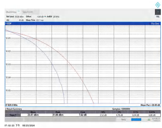
Band5-10MHz-QPSK-20450-50RB#0-PASS
