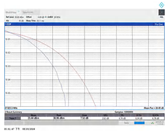
Band5-3MHz-QPSK-20415-15RB#0-PASS
