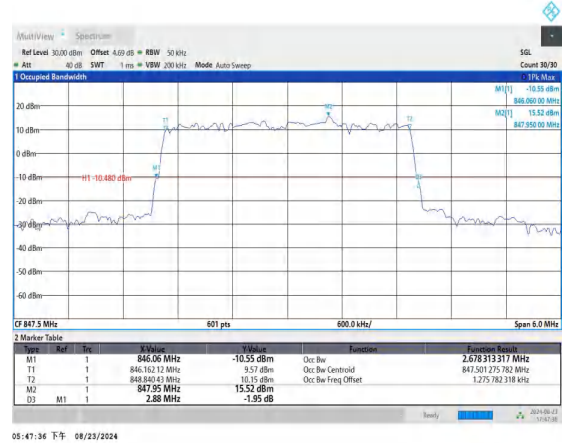
Band5-3MHz-16QAM-20635-15RB#0-PASS
