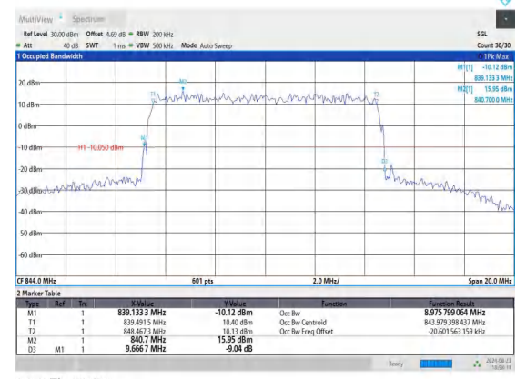
Band5-10MHz-16QAM-20600-50RB#0-PASS
