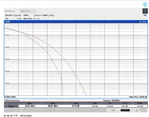
Band5-5MHz-16QAM-20525-25RB#0-PASS
