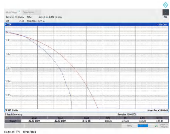
Band5-3MHz-16QAM-20635-15RB#0-PASS
