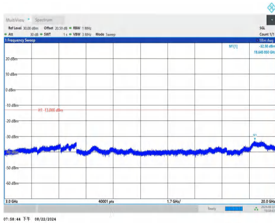
Band2_1.4MHz_QPSK_19193_1RB#0_3000~20000_3000~20000
