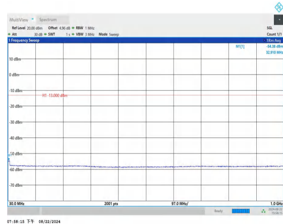
Band2_1.4MHz_QPSK_18900_1RB#0_30~1000_30~1000
