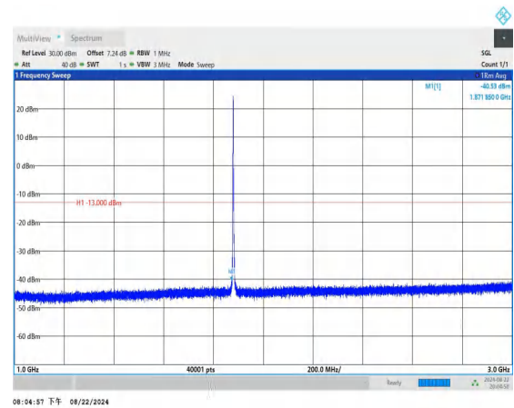
Band2_3MHz_QPSK_18900_1RB#0_1000~3000_1000~3000
