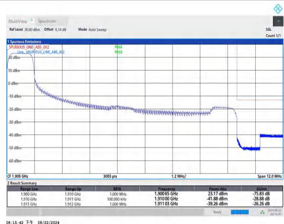
Band2_10MHz_QPSK_19150_1RB#0
