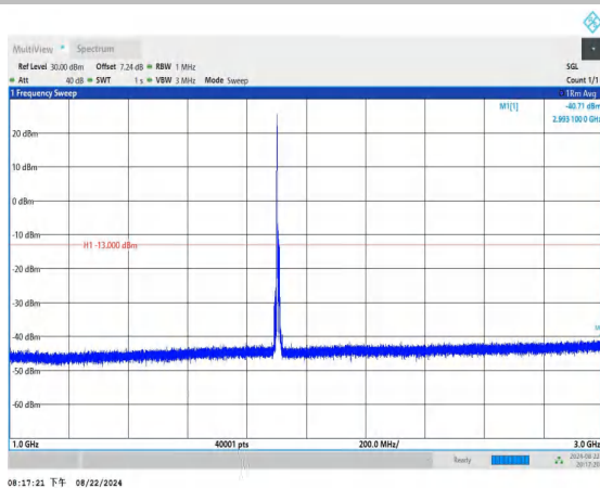
Band2_10MHz_QPSK_19150_1RB#0_1000~3000_1000~3000
