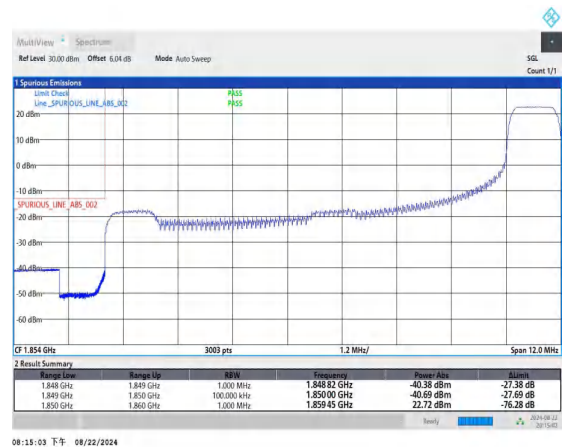
Band2_10MHz_QPSK_18650_1RB#49
