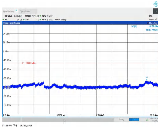
Band2_1.4MHz_QPSK_18607_1RB#0_3000~20000_3000~20000
