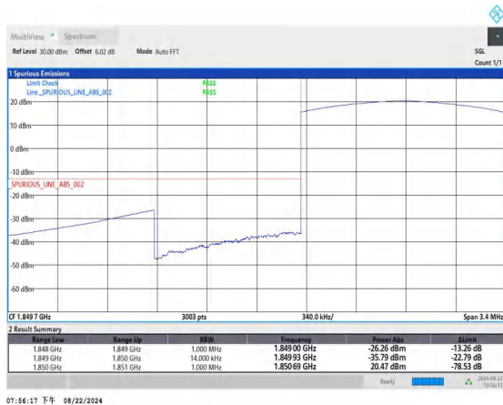
Band2_1.4MHz_16QAM_18607_6RB#0
