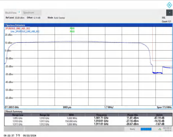
Band2_15MHz_QPSK_19125_75RB#0
