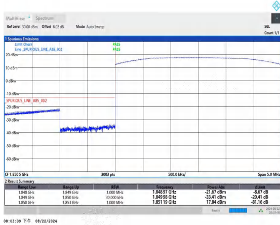
Band2_3MHz_QPSK_18615_15RB#0
