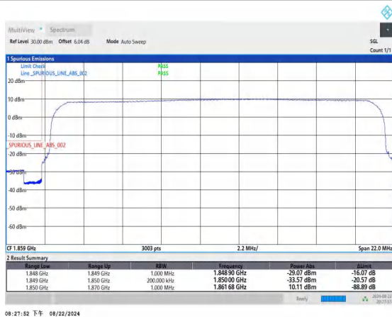
Band2_20MHz_QPSK_18700_100RB#0
