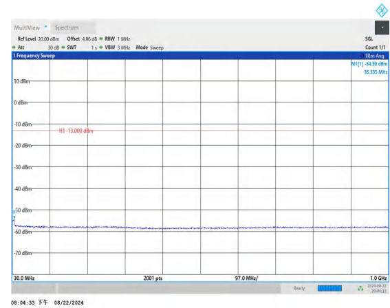
Band2_3MHz_QPSK_18615_1RB#0_30~1000_30~1000
