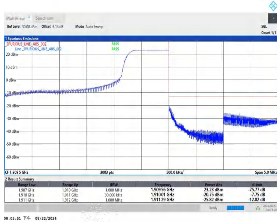
Band2_3MHz_QPSK_19185_1RB#14
