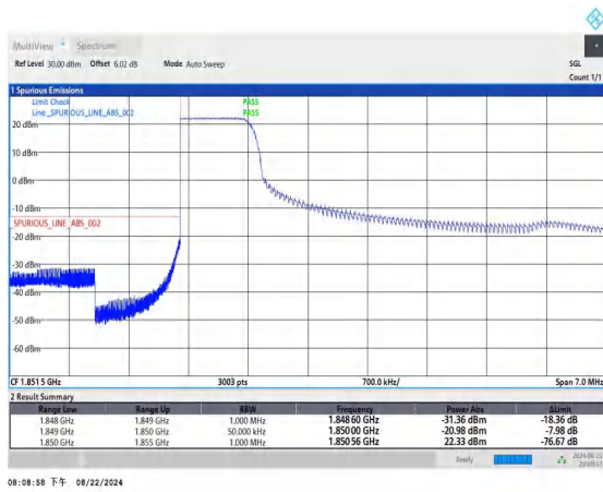
Band2_5MHz_16QAM_18625_1RB#0
