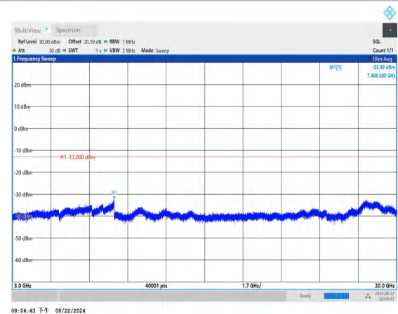
Band2_3MHz_QPSK_18615_1RB#0_3000~20000_3000~20000
