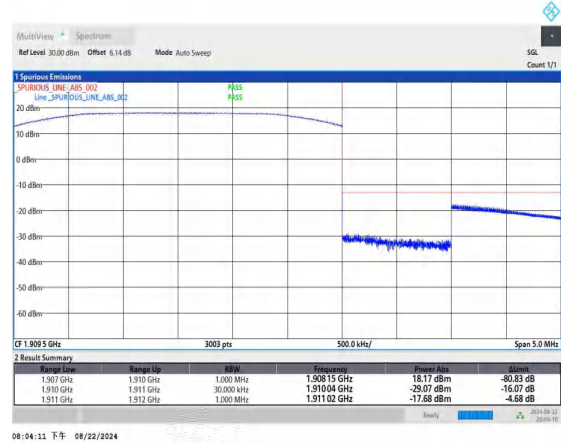
Band2_3MHz_QPSK_19185_15RB#0
