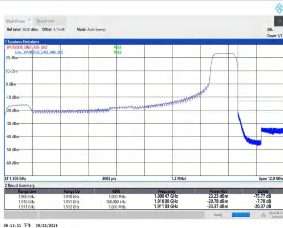
Band2_10MHz_QPSK_19150_1RB#49
