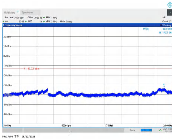
Band2_10MHz_QPSK_18900_1RB#0_3000~20000_3000~2000
