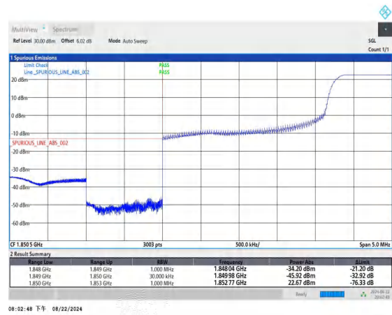
Band2_3MHz_QPSK_18615_1RB#14
