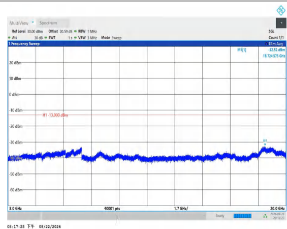
Band2_10MHz_QPSK_19150_1RB#0_3000~20000_3000~2000
