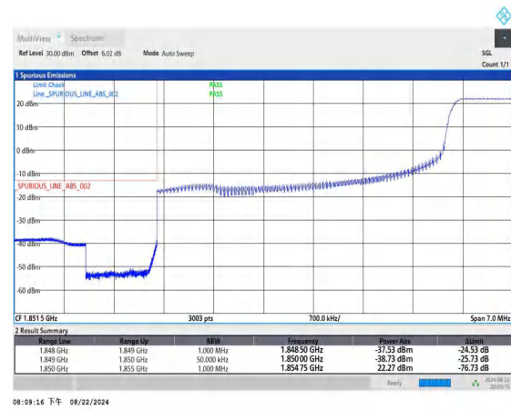
Band2_5MHz_16QAM_18625_1RB#24
