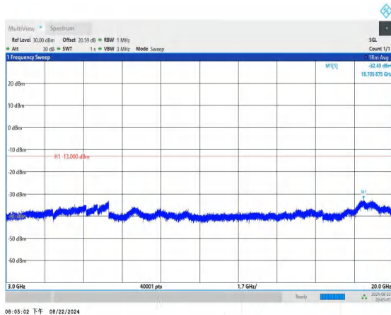
Band2_3MHz_QPSK_18900_1RB#0_3000~20000_3000~20000
