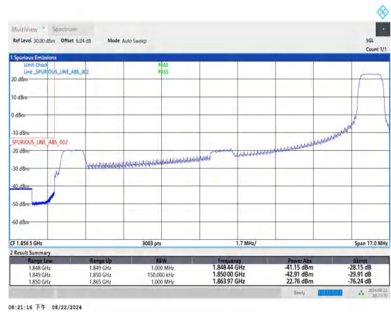
Band2_15MHz_QPSK_18675_1RB#74
