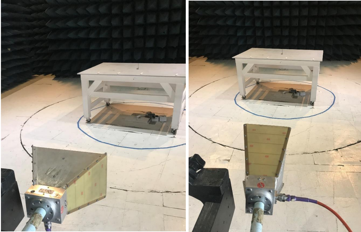
RE Test Setup – Horn Antenna (1 GHz to 13 GHz) Vertical and Horizontal Polarization
