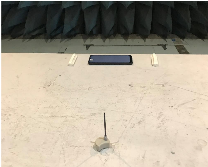
EUT RE Test Setup
