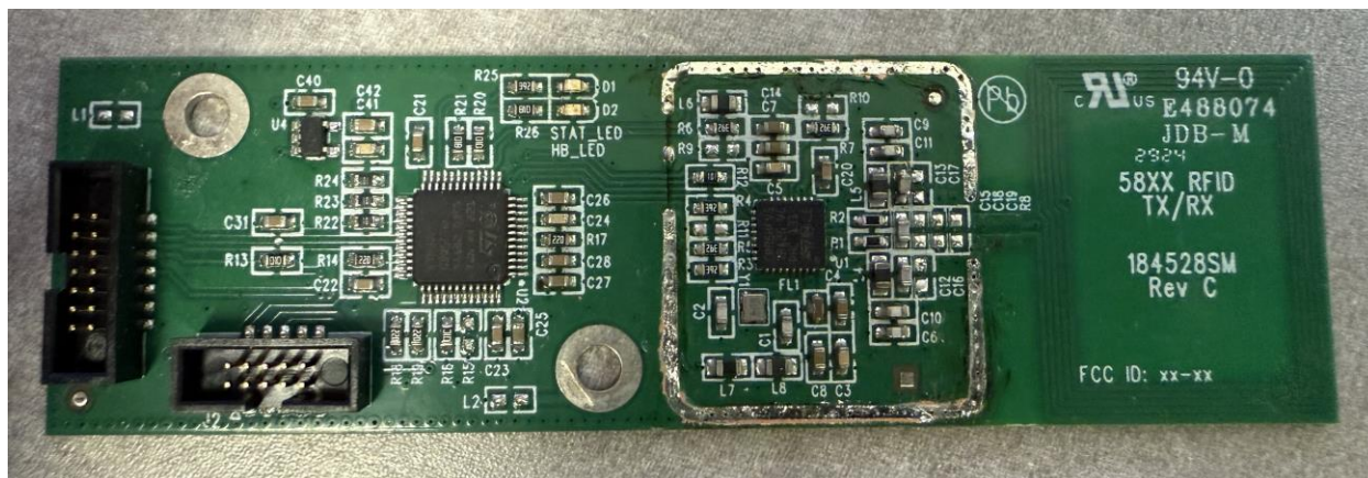
Figure 1: Top View
