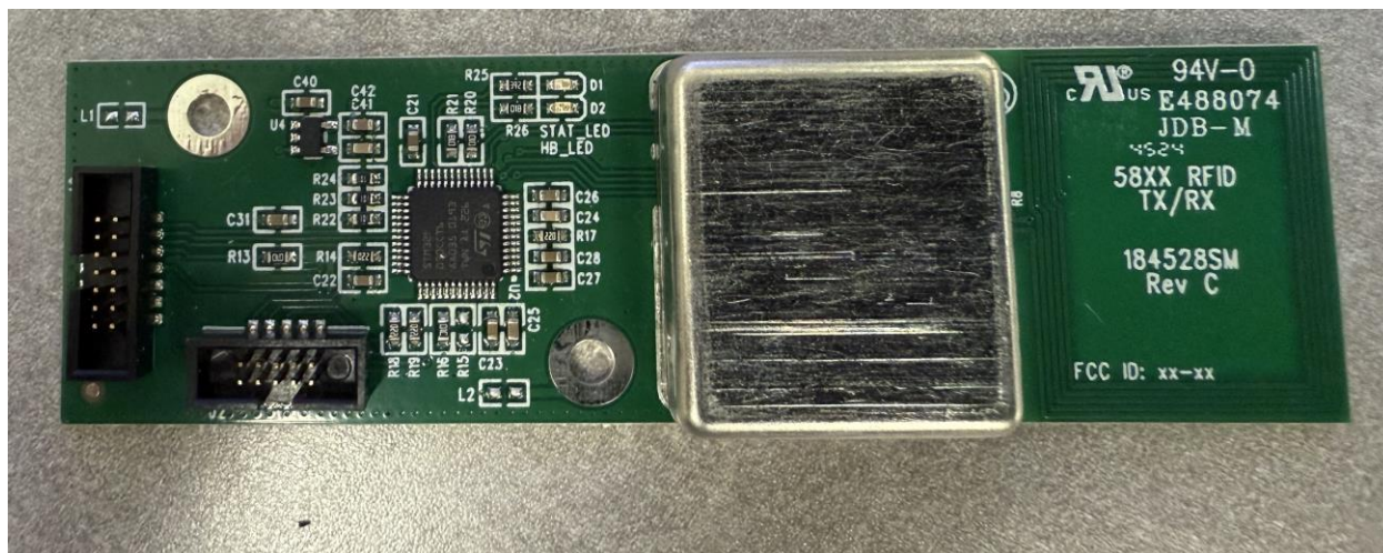
Figure 1: Top View
