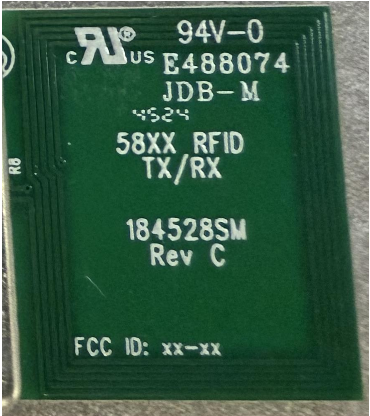
Permanently attached integrated PCB loop; 5 loops; outside dimension of outer loop 27mm x 21.6mm
