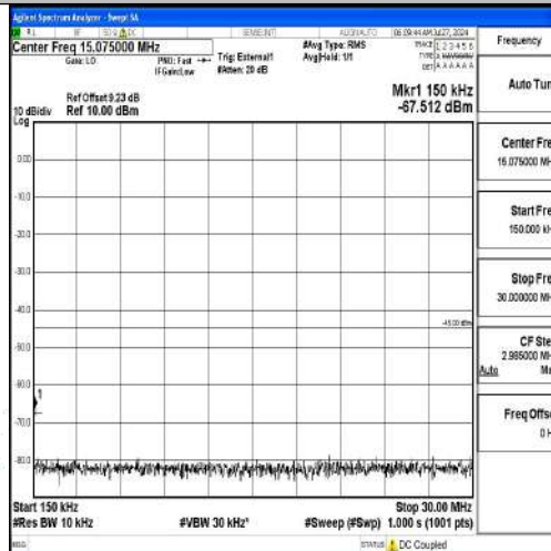
Band41-5MHz-16QAM-39675-1RB#0-0.15~30-PASS
