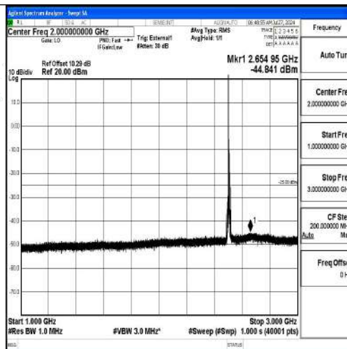
Band41-10MHz-16QAM-39700-1RB#0-1000~3000-PASS
