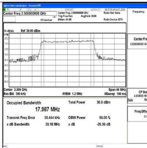
Band41-20MHz-QPSK-39750-100RB#0-PASS
