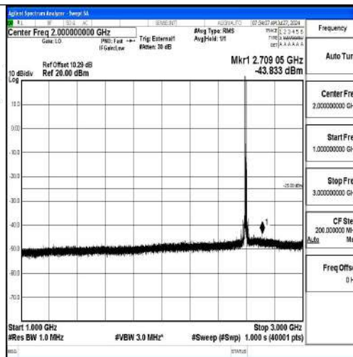
Band41-15MHz-16QAM-40620-1RB#0-1000~3000-PASS
