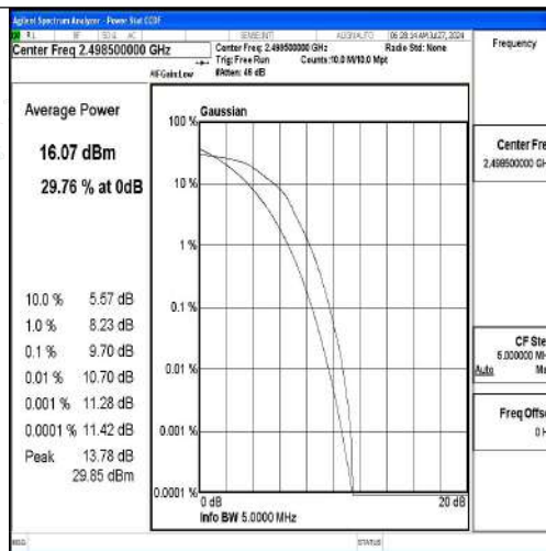
Band41-5MHz-16QAM-39675-25RB#0-PASS
