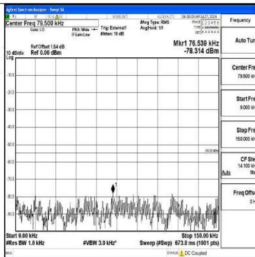
Band41-10MHz-QPSK-40620-1RB#0-0.009~0.15-PASS
