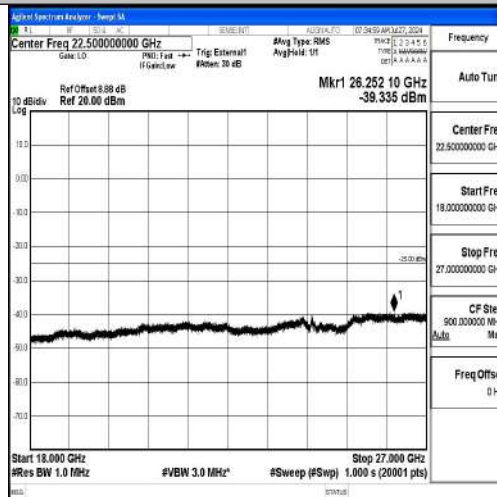
Band41-15MHz-16QAM-40620-1RB#0-18000~27000-PASS
