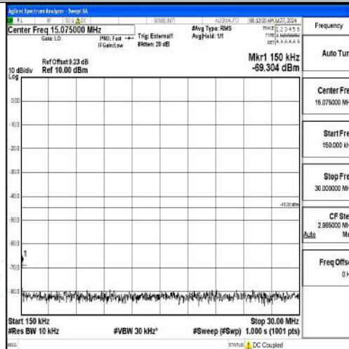
Band41-20MHz-QPSK-39750-1RB#0-0.15~30-PASS
