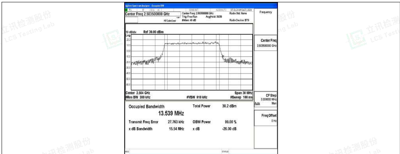
Band41-15MHz-QPSK-39725-75RB#0-PASS
