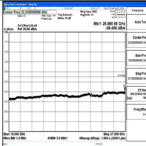
Band41-10MHz-QPSK-39700-1RB#0-18000~27000-PASS
