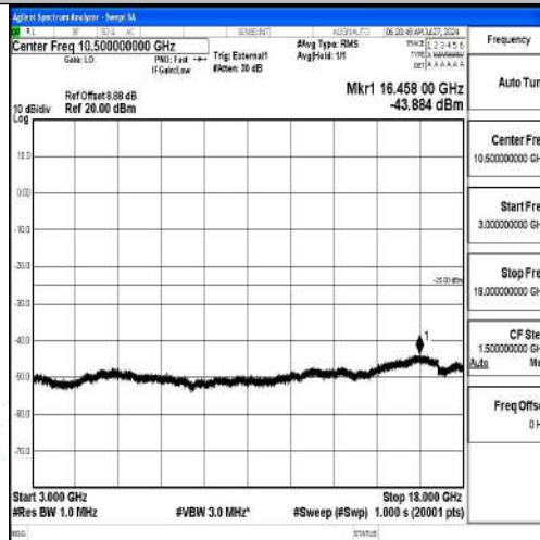
Band41-5MHz-16QAM-41565-1RB#0-3000~18000-PASS
