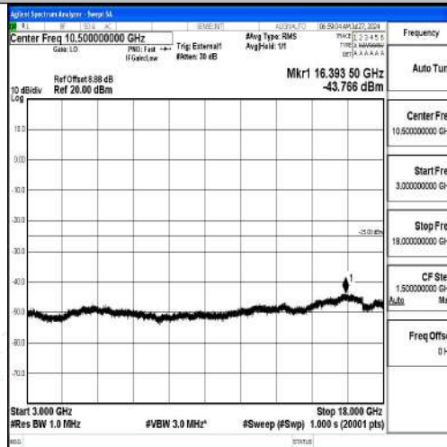
Band41-10MHz-16QAM-41540-1RB#0-3000~18000-PASS
