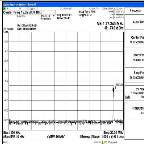
Band41-10MHz-QPSK-40620-1RB#0-0.15~30-PASS
