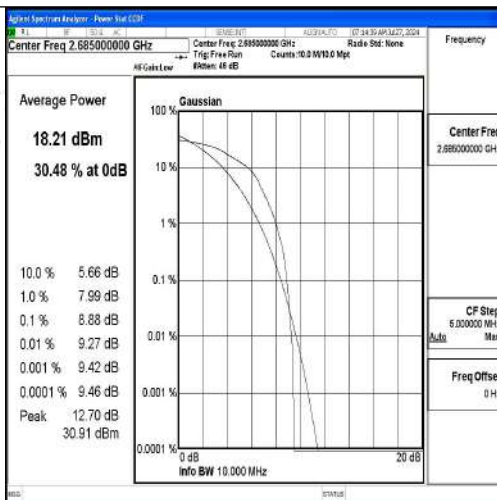
Band41-10MHz-16QAM-41540-1RB#0-PASS
