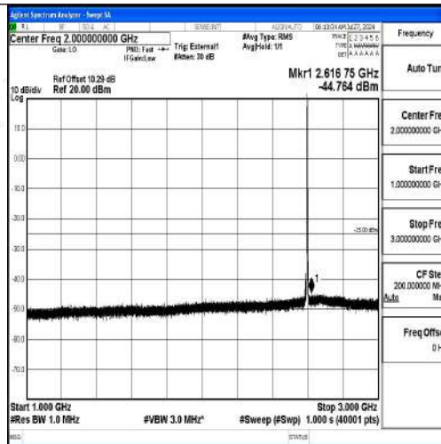
Band41-5MHz-QPSK-40620-1RB#0-1000~3000-PASS
