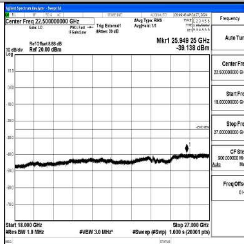
Band41-10MHz-16QAM-39700-1RB#0-18000~27000-PASS
