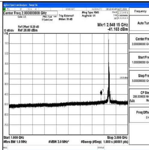
Band41-20MHz-QPSK-41490-1RB#0-1000~3000-PASS
