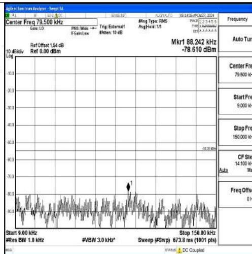
Band41-20MHz-16QAM-39750-1RB#0-0.009~0.15-PASS
