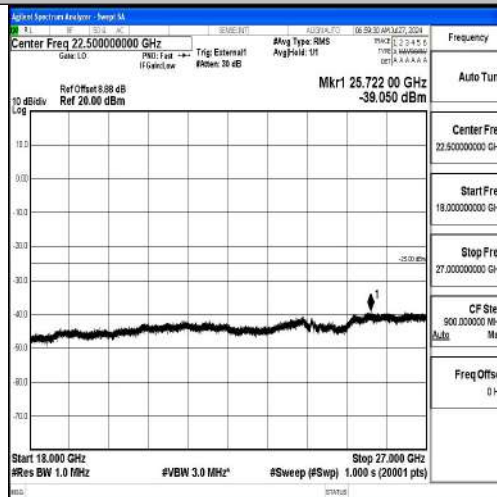
Band41-10MHz-16QAM-41540-1RB#0-18000~27000-PASS
