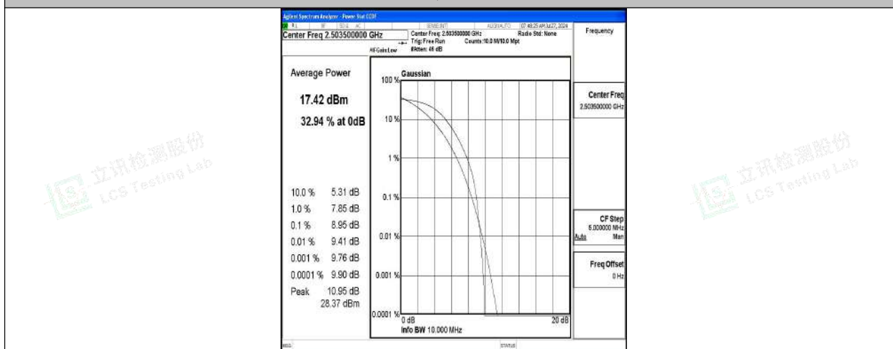
Band41-15MHz-QPSK-39725-75RB#0-PASS
