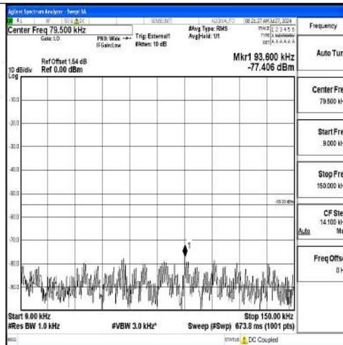
Band41-20MHz-QPSK-41490-1RB#0-0.009~0.15-PASS
