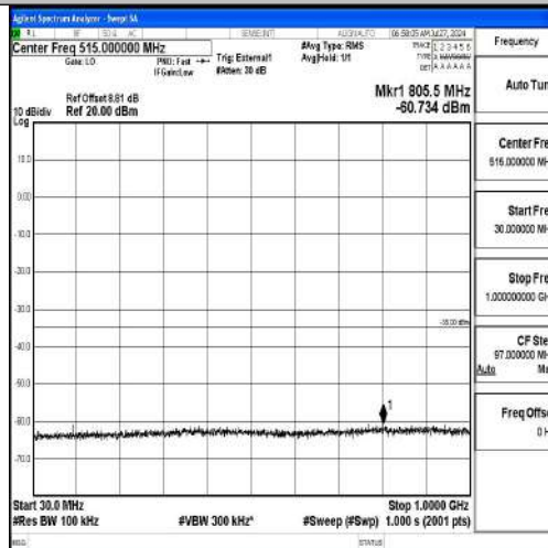
Band41-10MHz-16QAM-41540-1RB#0-30~1000-PASS
