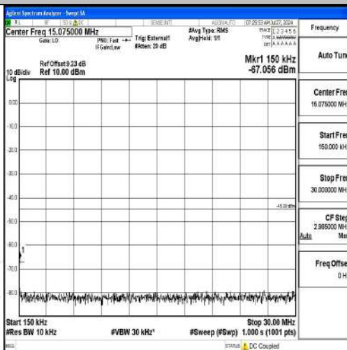
Band41-15MHz-QPSK-39725-1RB#0-0.15~30-PASS
