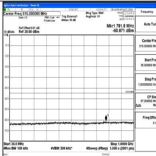
Band41-5MHz-16QAM-40620-1RB#0-30~1000-PASS
