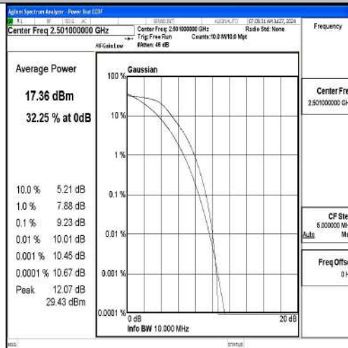
Band41-10MHz-QPSK-39700-50RB#0-PASS
