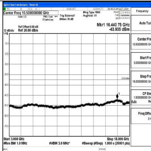
Band41-10MHz-16QAM-39700-1RB#0-3000~18000-PASS
