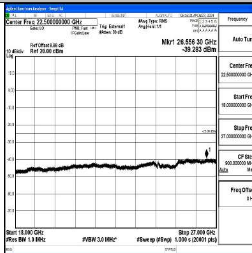
Band41-5MHz-16QAM-40620-1RB#0-18000~27000-PASS
