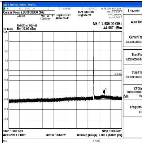
Band41-5MHz-QPSK-39675-1RB#0-1000~3000-PASS
