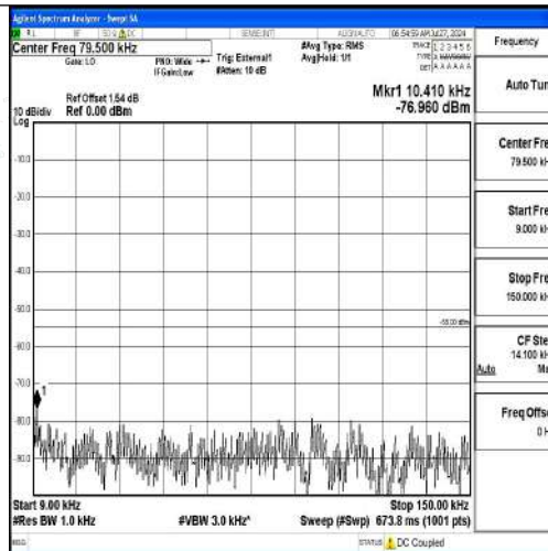
Band41-10MHz-QPSK-41540-1RB#0-0.009~0.15-PASS
