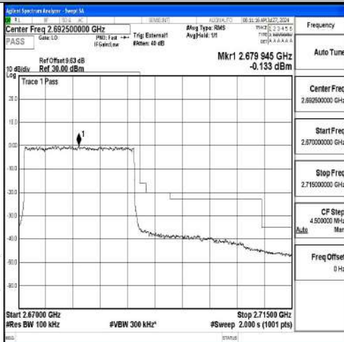
Band41-20MHz-16QAM-41490-100RB#0-PASS
