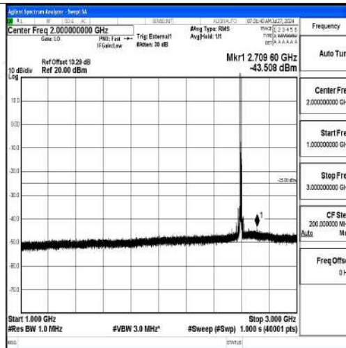
Band41-15MHz-QPSK-40620-1RB#0-1000~3000-PASS
