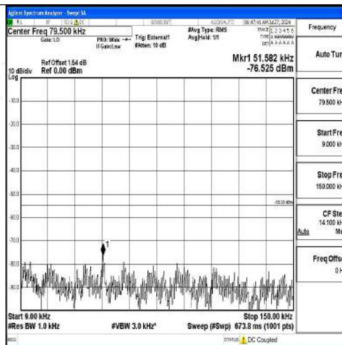
Band41-10MHz-16QAM-39700-1RB#0-0.009~0.15-PASS
