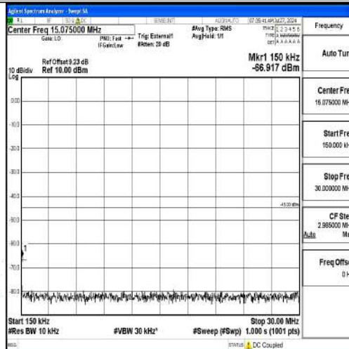
Band41-15MHz-QPSK-41515-1RB#0-0.15~30-PASS
