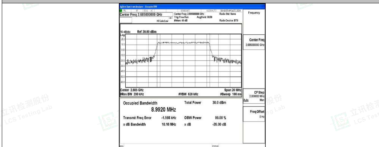
Band41-10MHz-QPSK-41540-50RB#0-PASS
