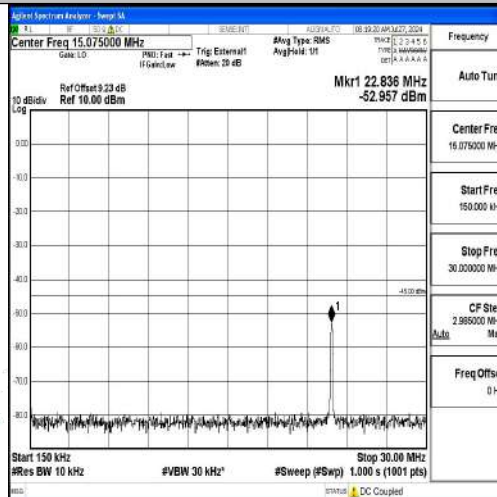
Band41-20MHz-16QAM-40620-1RB#0-0.15~30-PASS
