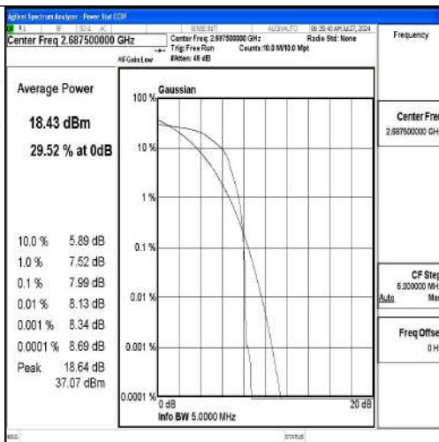
Band41-5MHz-16QAM-41565-1RB#0-PASS
