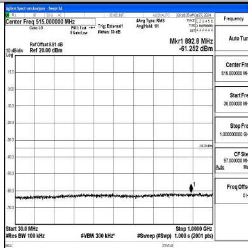
Band41-5MHz-16QAM-39675-1RB#0-30~1000-PASS
