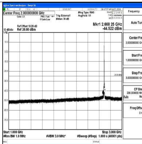
Band41-5MHz-QPSK-41565-1RB#0-1000~3000-PASS
