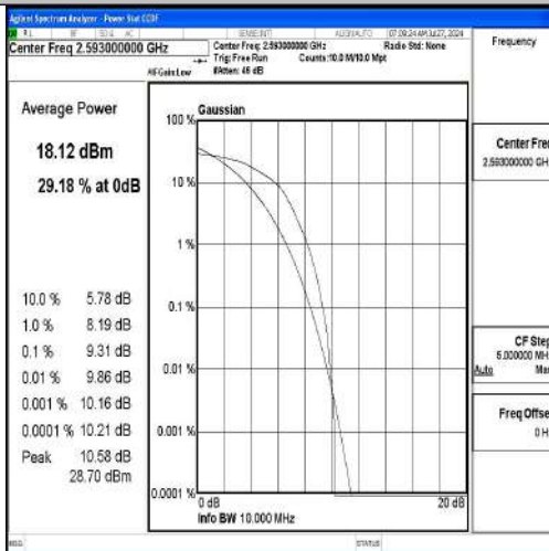
Band41-10MHz-16QAM-40620-1RB#0-PASS
