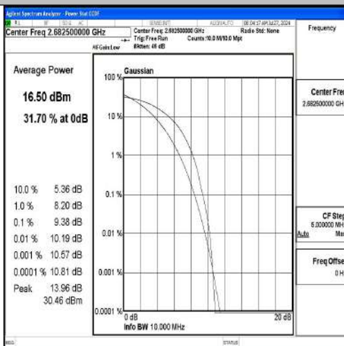
Band41-15MHz-16QAM-41515-75RB#0-PASS
