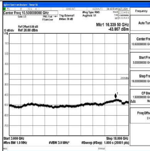
Band41-5MHz-16QAM-40620-1RB#0-3000~18000-PASS
