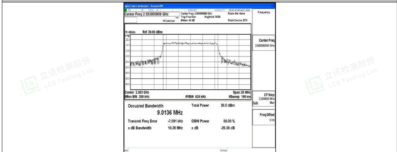
Band41-10MHz-QPSK-40620-50RB#0-PASS
