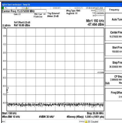
Band41-15MHz-16QAM-39725-1RB#0-0.15~30-PASS
