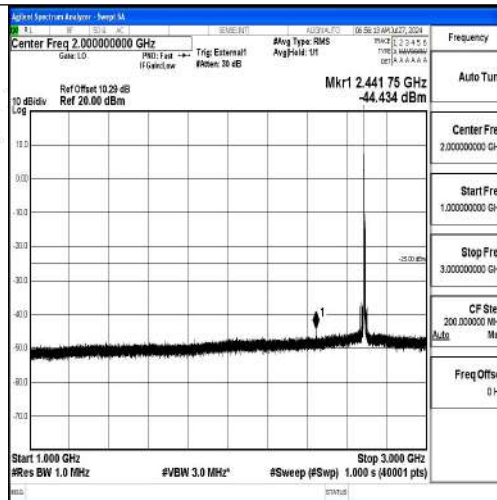
Band41-10MHz-QPSK-41540-1RB#0-1000~3000-PASS
