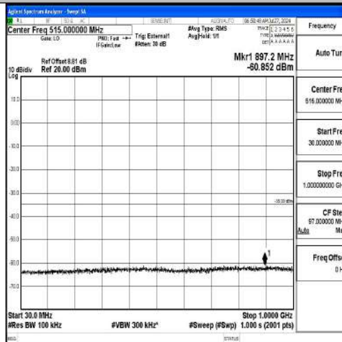
Band41-10MHz-QPSK-40620-1RB#0-30~1000-PASS
