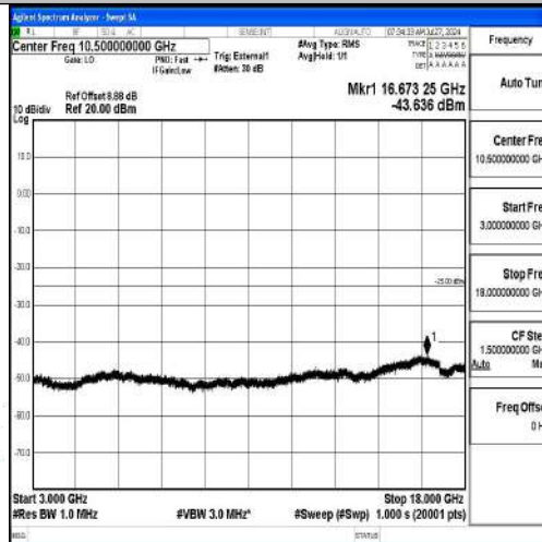
Band41-15MHz-16QAM-40620-1RB#0-3000~18000-PASS
