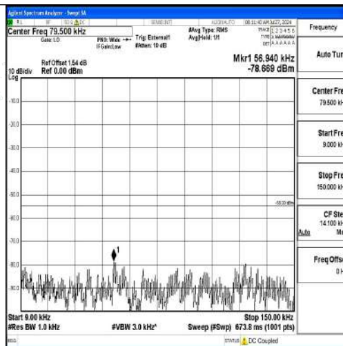
Band41-20MHz-QPSK-39750-1RB#0-0.009~0.15-PASS
