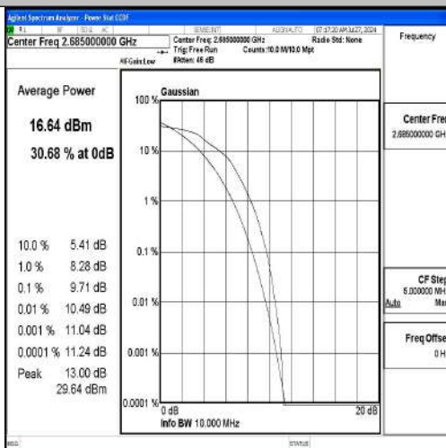
Band41-10MHz-16QAM-41540-50RB#0-PASS
