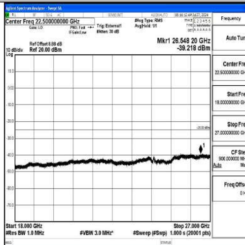
Band41-20MHz-16QAM-39750-1RB#0-18000~27000-PASS
