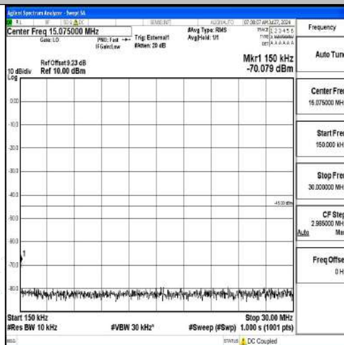
Band41-15MHz-16QAM-41515-1RB#0-0.15~30-PASS
