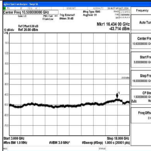
Band41-10MHz-QPSK-39700-1RB#0-3000~18000-PASS
