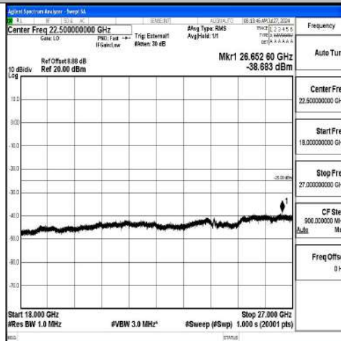
Band41-20MHz-QPSK-39750-1RB#0-18000~27000-PASS
