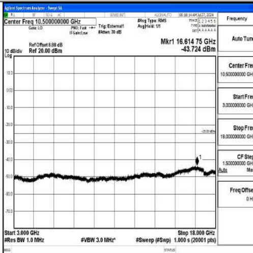
Band41-20MHz-QPSK-40620-1RB#0-3000~18000-PASS
