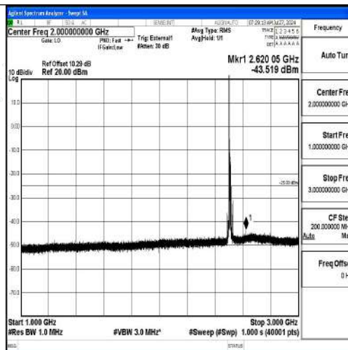
Band41-15MHz-16QAM-39725-1RB#0-1000~3000-PASS
