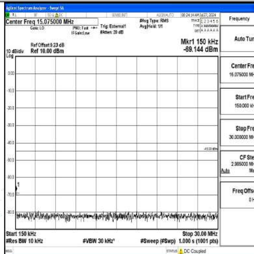
Band41-20MHz-16QAM-41490-1RB#0-0.15~30-PASS
