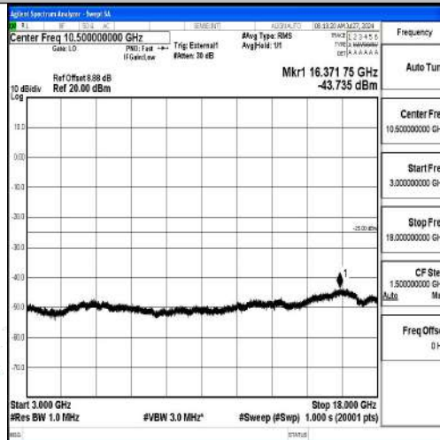
Band41-20MHz-QPSK-39750-1RB#0-3000~18000-PASS
