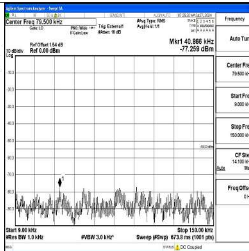
Band41-15MHz-QPSK-41515-1RB#0-0.009~0.15-PASS
