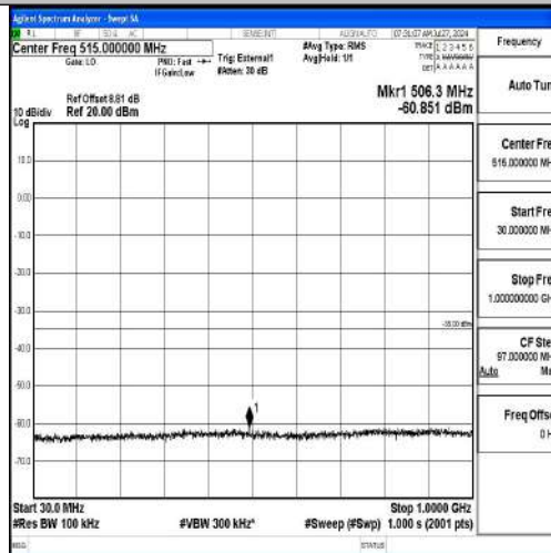
Band41-15MHz-QPSK-40620-1RB#0-30~1000-PASS
