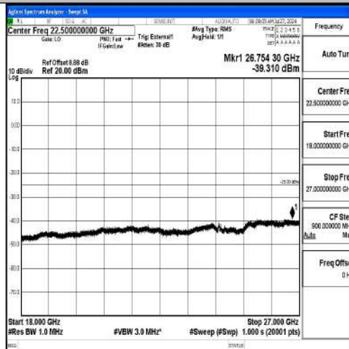
Band41-5MHz-QPSK-39675-1RB#0-18000~27000-PASS
