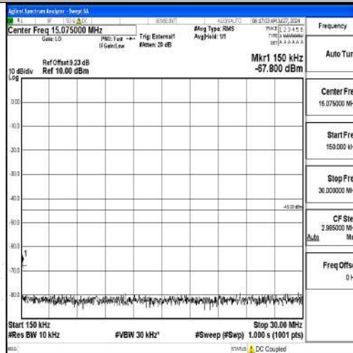
Band41-5MHz-QPSK-41565-1RB#0-0.15~30-PASS
