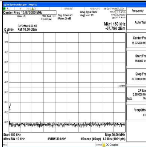
Band41-20MHz-QPSK-41490-1RB#0-0.15~30-PASS
