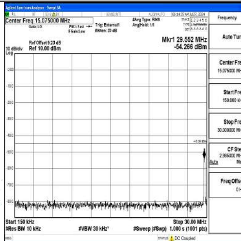
Band41-5MHz-16QAM-40620-1RB#0-0.15~30-PASS
