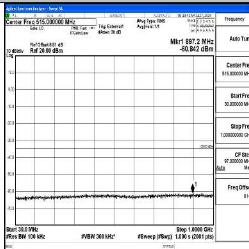
Band41-20MHz-16QAM-40620-1RB#0-30~1000-PASS
