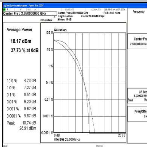
Band41-20MHz-QPSK-41490-100RB#0-PASS
