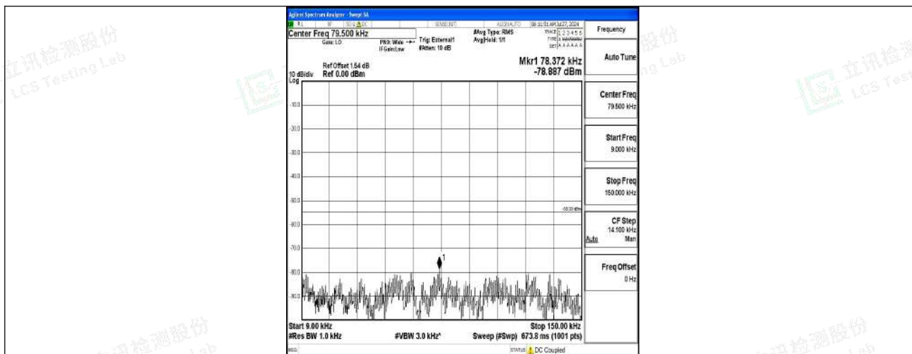
Band41-5MHz-QPSK-40620-1RB#0-0.009~0.15-PASS
