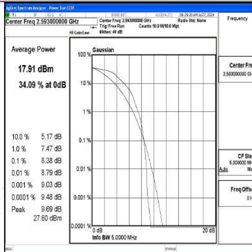
Band41-5MHz-QPSK-40620-1RB#0-PASS
