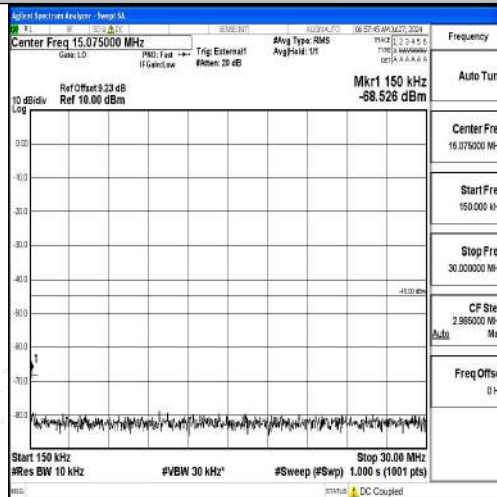
Band41-10MHz-16QAM-41540-1RB#0-0.15~30-PASS
