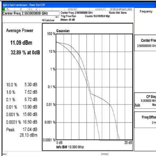
Band41-15MHz-QPSK-40620-1RB#0-PASS
