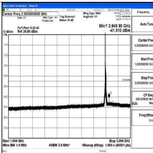
Band41-20MHz-QPSK-40620-1RB#0-1000~3000-PASS
