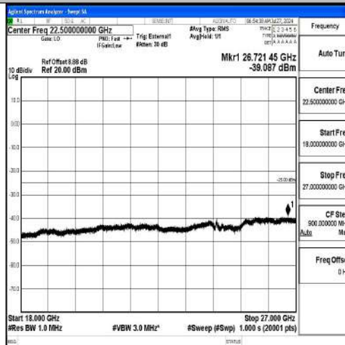
Band41-10MHz-16QAM-40620-1RB#0-18000~27000-PASS
