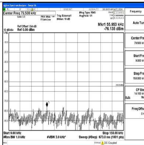
Band41-20MHz-16QAM-40620-1RB#0-0.009~0.15-PASS
