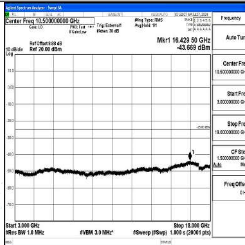
Band41-15MHz-QPSK-40620-1RB#0-3000~18000-PASS
