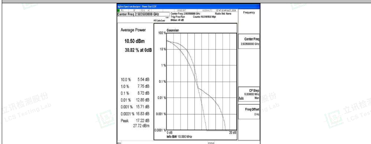
Band41-15MHz-16QAM-39725-1RB#0-PASS
