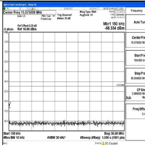
Band41-10MHz-QPSK-41540-1RB#0-0.15~30-PASS
