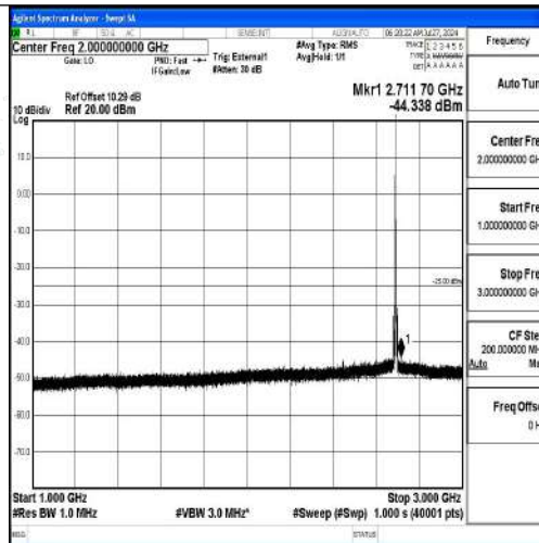
Band41-5MHz-16QAM-41565-1RB#0-1000~3000-PASS
