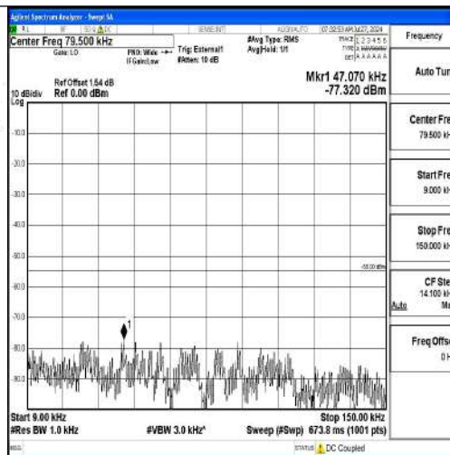
Band41-15MHz-16QAM-40620-1RB#0-0.009~0.15-PASS
