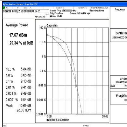
Band41-5MHz-16QAM-40620-1RB#0-PASS
