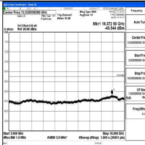
Band41-15MHz-QPSK-39725-1RB#0-3000~18000-PASS
