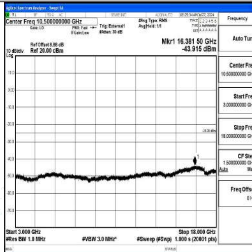
Band41-20MHz-16QAM-41490-1RB#0-3000~18000-PASS
