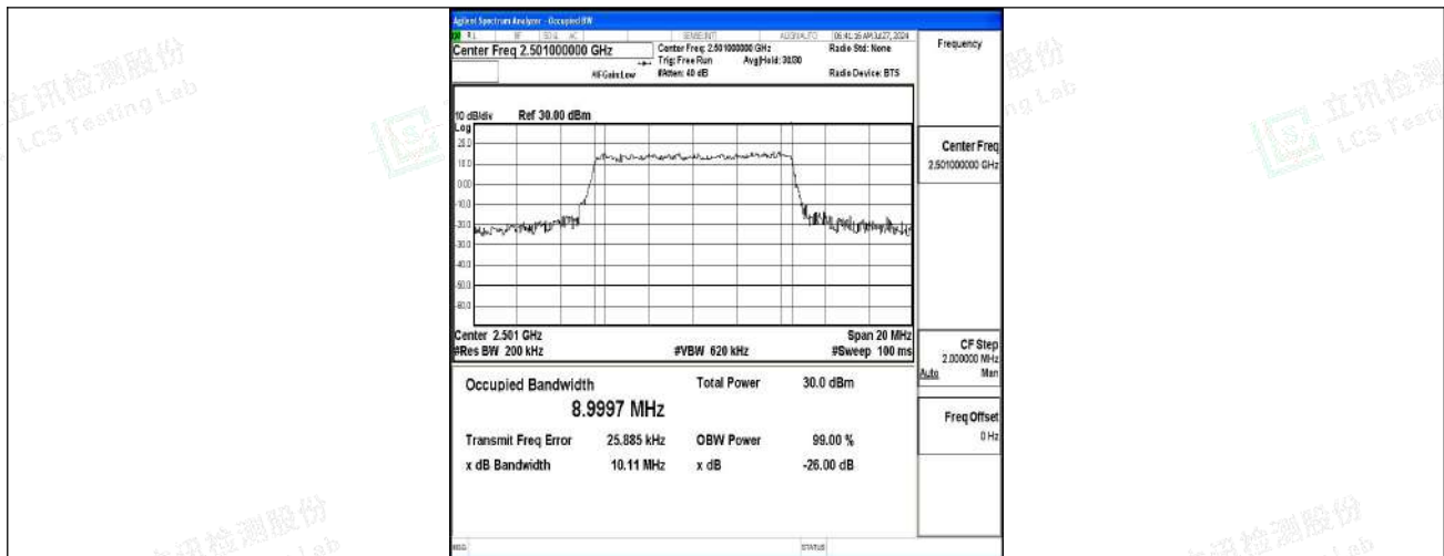
Band41-10MHz-QPSK-39700-50RB#0-PASS
