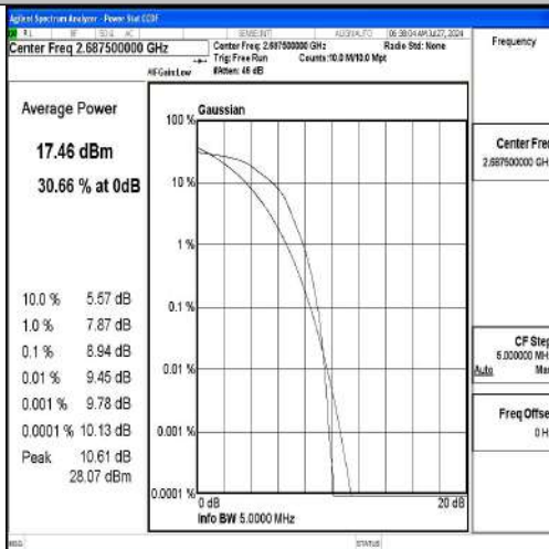
Band41-5MHz-16QAM-41565-25RB#0-PASS
