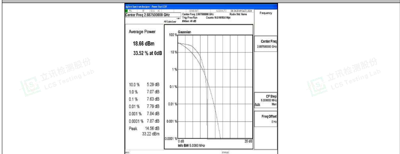
Band41-5MHz-QPSK-41565-1RB#0-PASS
