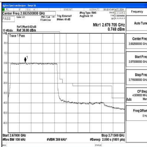
Band41-20MHz-QPSK-41490-100RB#0-PASS
