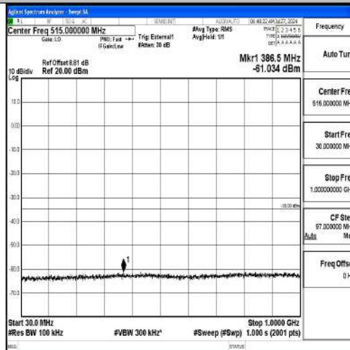
Band41-10MHz-16QAM-39700-1RB#0-30~1000-PASS
