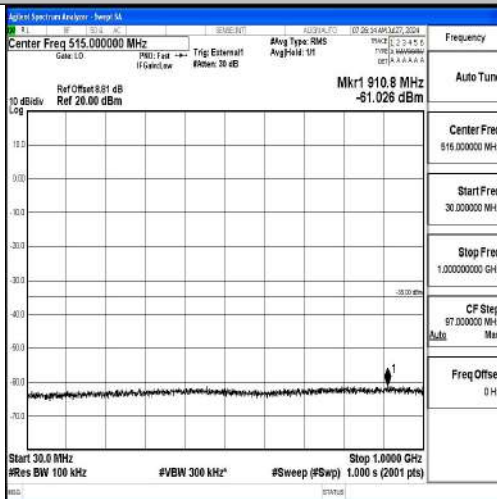
Band41-15MHz-QPSK-39725-1RB#0-30~1000-PASS
