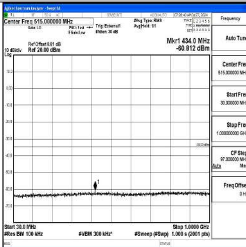
Band41-15MHz-16QAM-39725-1RB#0-30~1000-PASS
