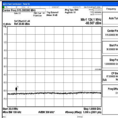
Band41-5MHz-QPSK-41565-1RB#0-30~1000-PASS
