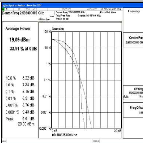
Band41-20MHz-QPSK-40620-1RB#0-PASS
