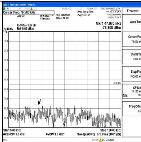
Band41-10MHz-16QAM-40620-1RB#0-0.009~0.15-PASS
