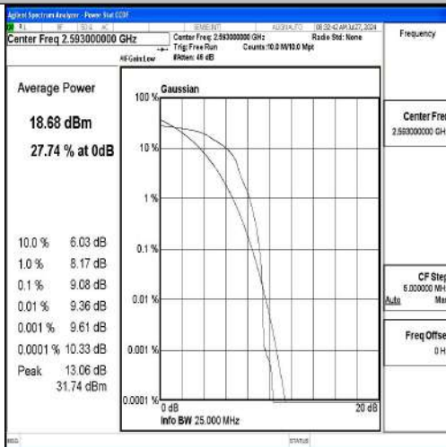
Band41-20MHz-16QAM-40620-1RB#0-PASS
