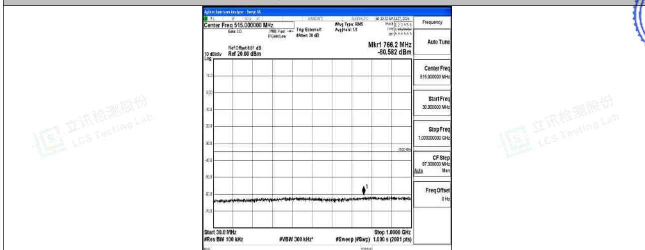
Band41-5MHz-QPSK-40620-1RB#0-30~1000-PASS
