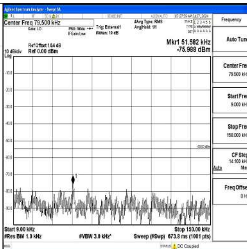
Band41-15MHz-16QAM-39725-1RB#0-0.009~0.15-PASS
