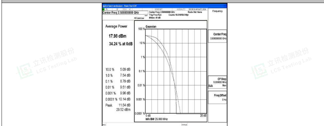
Band41-20MHz-QPSK-39750-100RB#0-PASS
