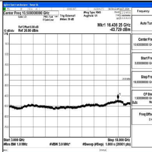
Band41-10MHz-16QAM-40620-1RB#0-3000~18000-PASS
