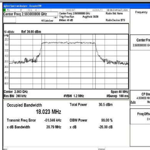
Band41-20MHz-QPSK-40620-100RB#0-PASS
