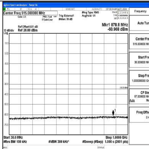
Band41-15MHz-16QAM-40620-1RB#0-30~1000-PASS
