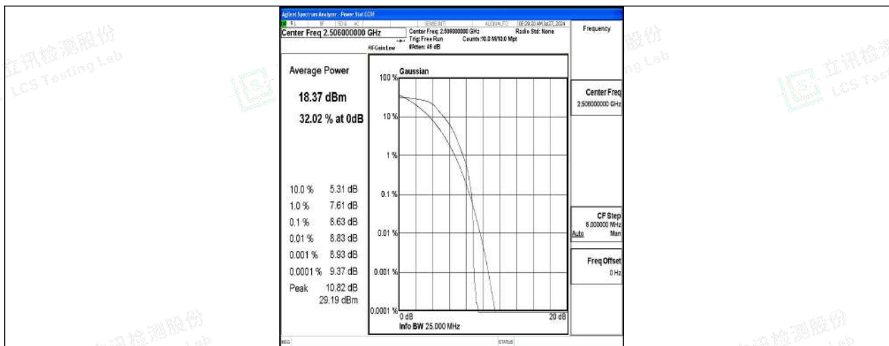
Band41-20MHz-QPSK-39750-1RB#0-PASS
