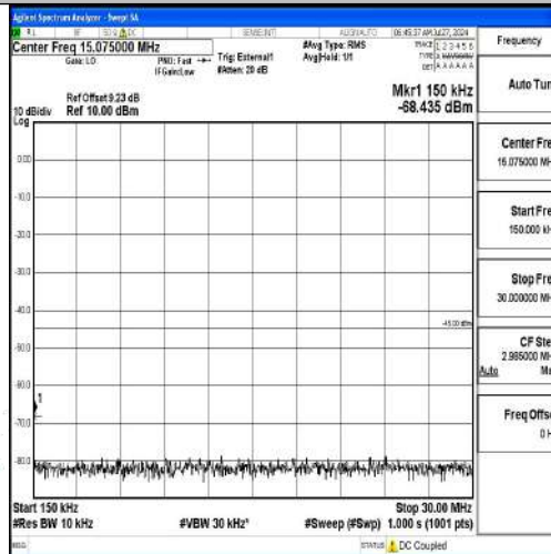
Band41-10MHz-QPSK-39700-1RB#0-0.15~30-PASS
