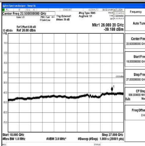
Band41-10MHz-QPSK-40620-1RB#0-18000~27000-PASS
