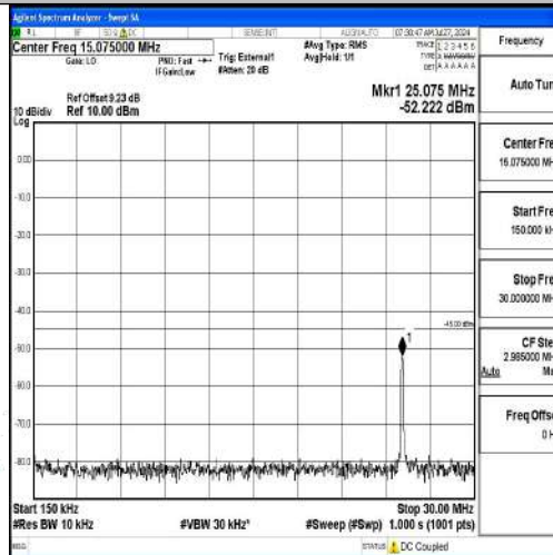
Band41-15MHz-QPSK-40620-1RB#0-0.15~30-PASS
