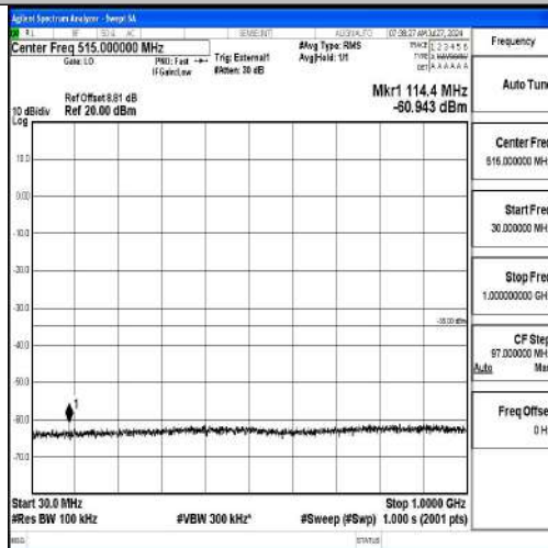
Band41-15MHz-16QAM-41515-1RB#0-30~1000-PASS
