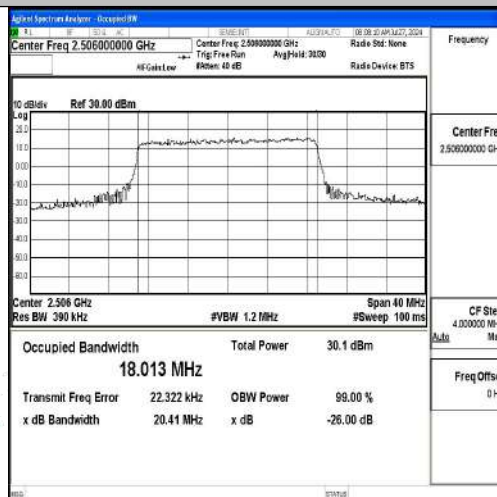
Band41-20MHz-16QAM-39750-100RB#0-PASS
