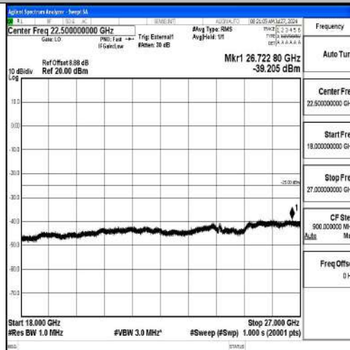
Band41-20MHz-16QAM-40620-1RB#0-18000~27000-PASS
