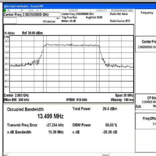
Band41-15MHz-16QAM-41515-75RB#0-PASS
