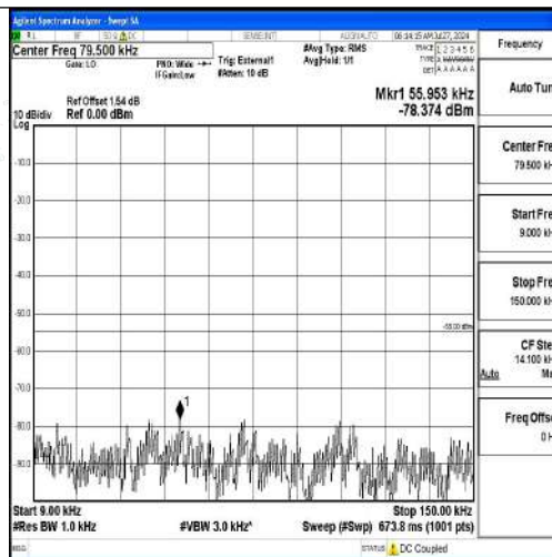
Band41-5MHz-16QAM-40620-1RB#0-0.009~0.15-PASS
