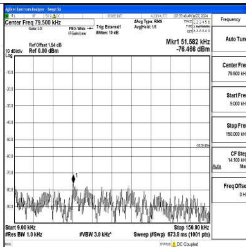
Band41-15MHz-16QAM-41515-1RB#0-0.009~0.15-PASS
