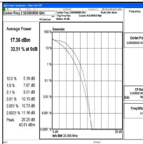
Band41-20MHz-QPSK-40620-100RB#0-PASS
