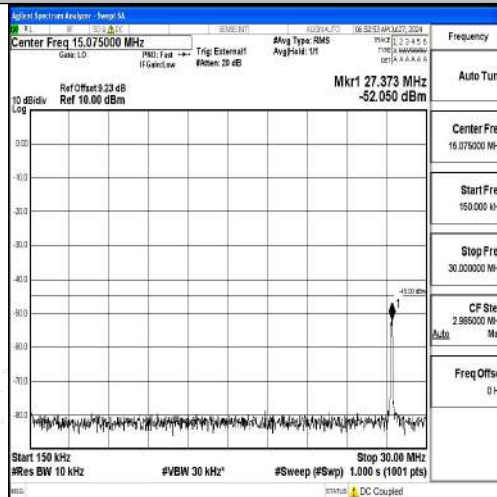
Band41-10MHz-16QAM-40620-1RB#0-0.15~30-PASS
