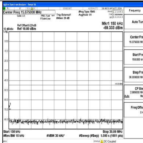
Band41-10MHz-16QAM-39700-1RB#0-0.15~30-PASS
