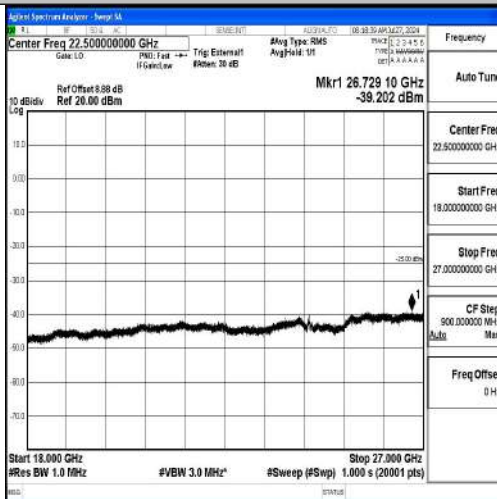
Band41-20MHz-QPSK-40620-1RB#0-18000~27000-PASS
