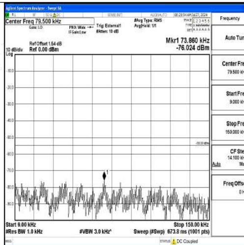
Band41-20MHz-16QAM-41490-1RB#0-0.009~0.15-PASS
