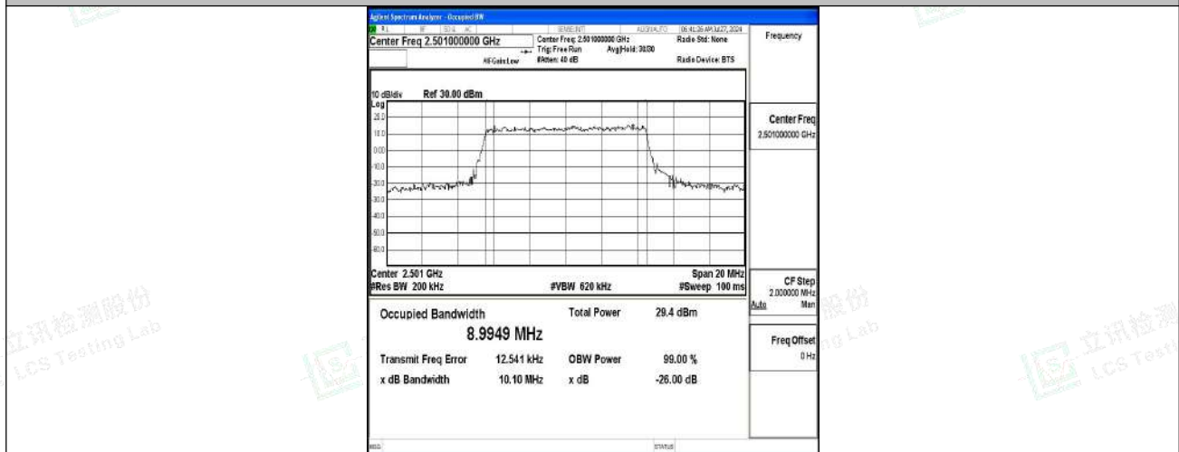
Band41-10MHz-16QAM-39700-50RB#0-PASS
