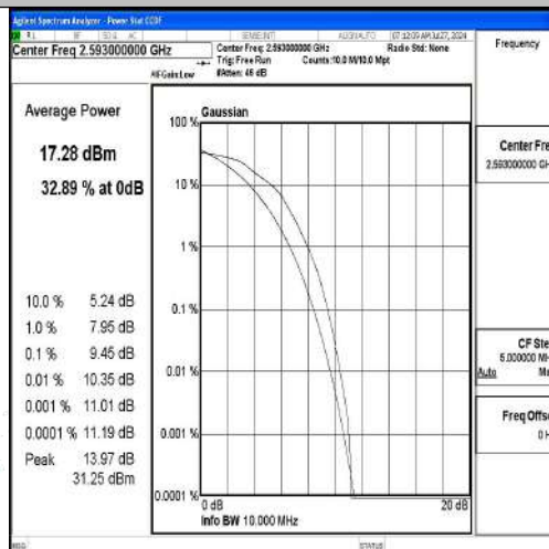
Band41-10MHz-16QAM-40620-50RB#0-PASS
