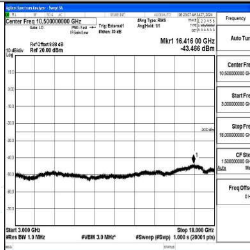
Band41-20MHz-QPSK-41490-1RB#0-3000~18000-PASS
