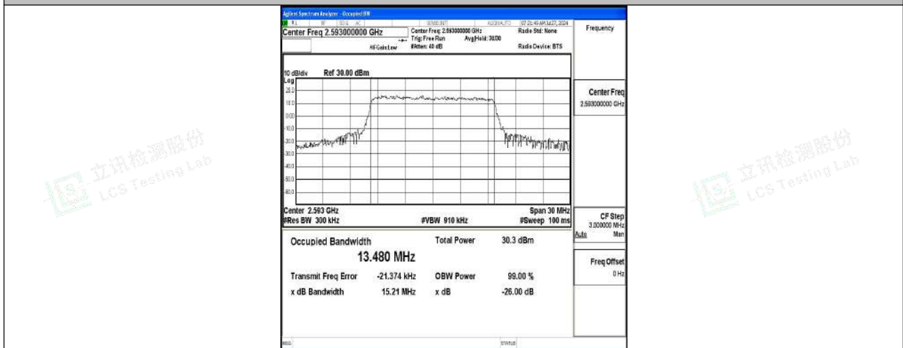
Band41-15MHz-QPSK-40620-75RB#0-PASS
