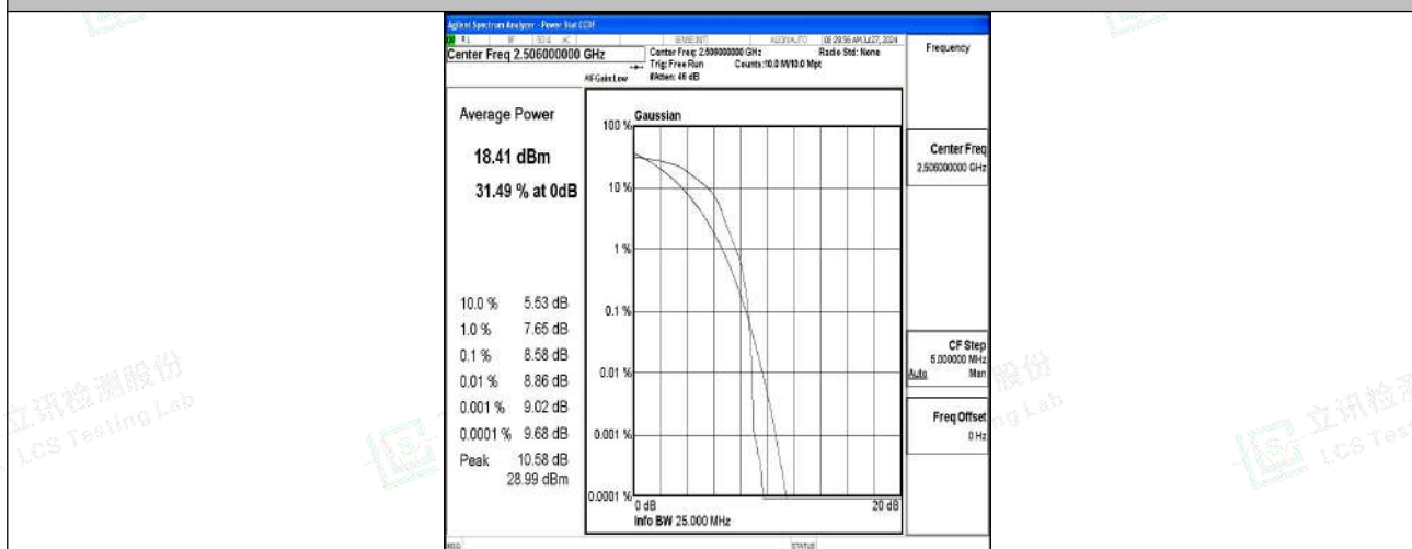
Band41-20MHz-16QAM-39750-1RB#0-PASS
