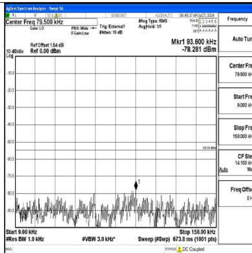
Band41-10MHz-QPSK-39700-1RB#0-0.009~0.15-PASS
