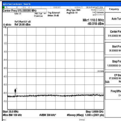
Band41-20MHz-16QAM-41490-1RB#0-30~1000-PASS
