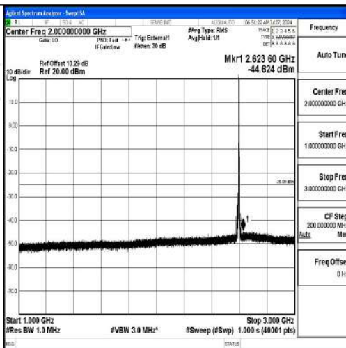
Band41-10MHz-QPSK-40620-1RB#0-1000~3000-PASS
