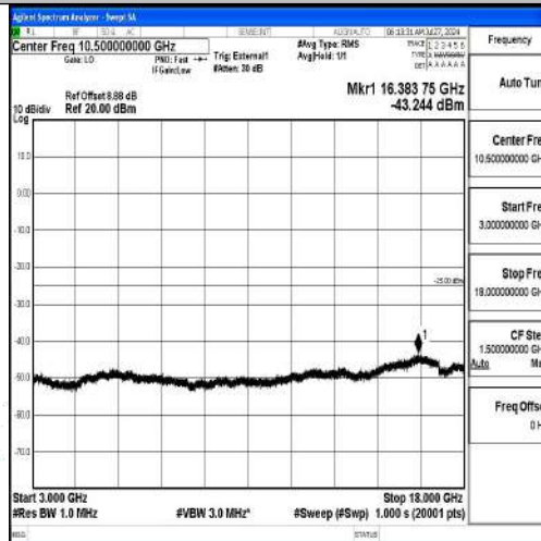
Band41-5MHz-QPSK-40620-1RB#0-3000~18000-PASS
