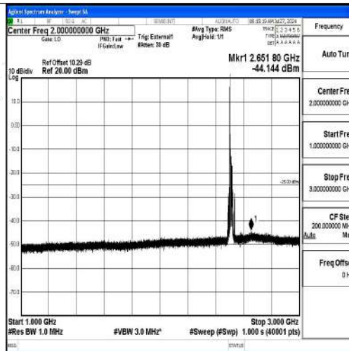
Band41-20MHz-16QAM-39750-1RB#0-1000~3000-PASS
