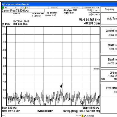
Band41-15MHz-QPSK-39725-1RB#0-0.009~0.15-PASS
