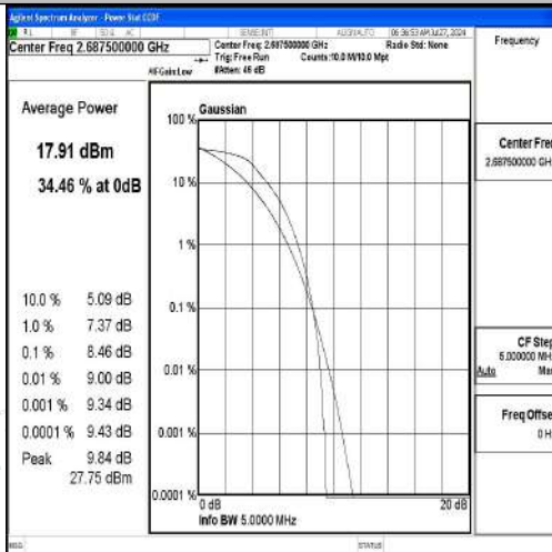
Band41-5MHz-QPSK-41565-25RB#0-PASS
