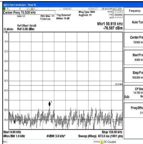
Band41-5MHz-QPSK-41565-1RB#0-0.009~0.15-PASS
