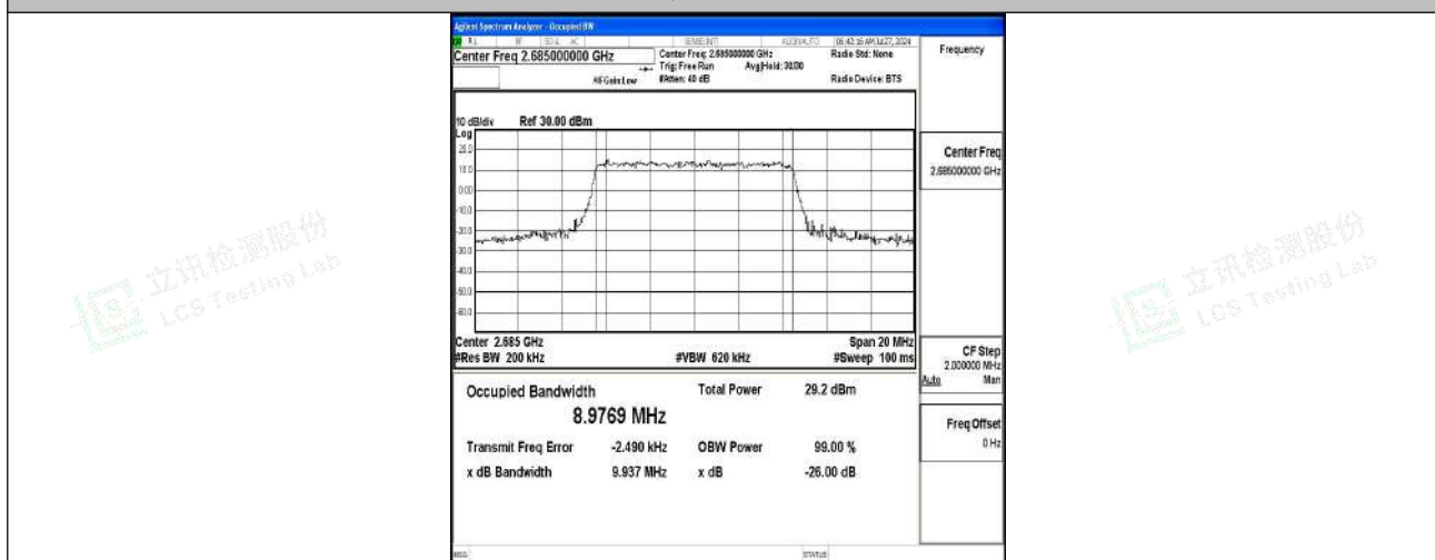
Band41-10MHz-16QAM-41540-50RB#0-PASS
