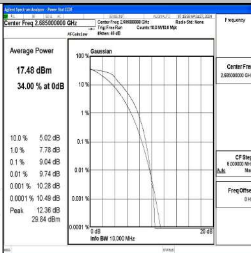
Band41-10MHz-QPSK-41540-50RB#0-PASS
