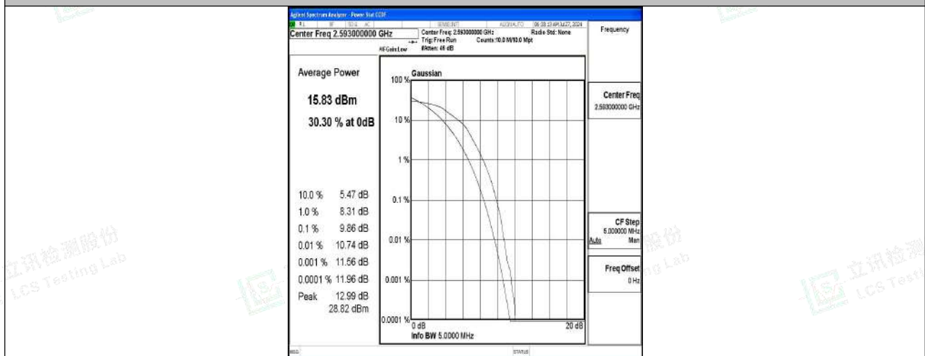
Band41-5MHz-16QAM-40620-25RB#0-PASS
