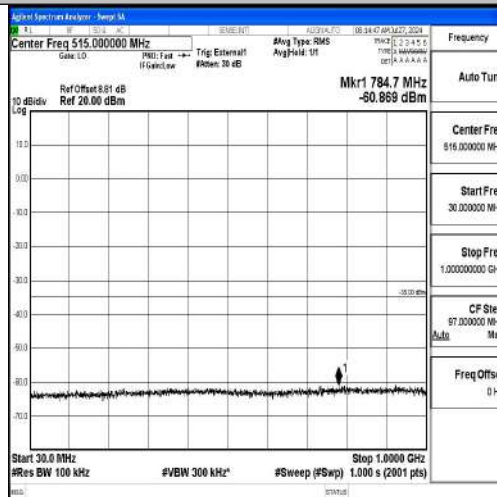
Band41-20MHz-16QAM-39750-1RB#0-30~1000-PASS
