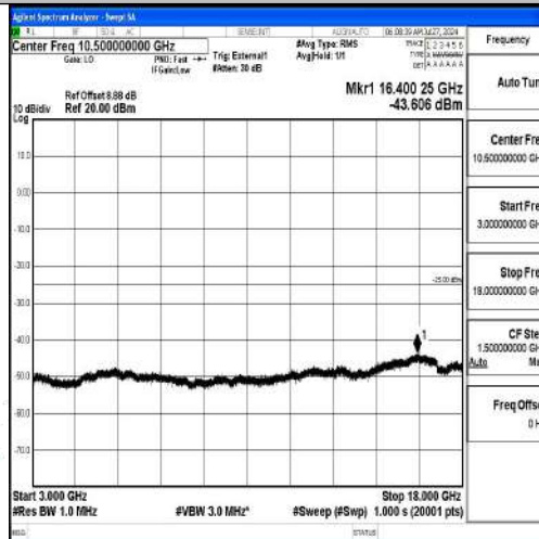
Band41-5MHz-QPSK-39675-1RB#0-3000~18000-PASS
