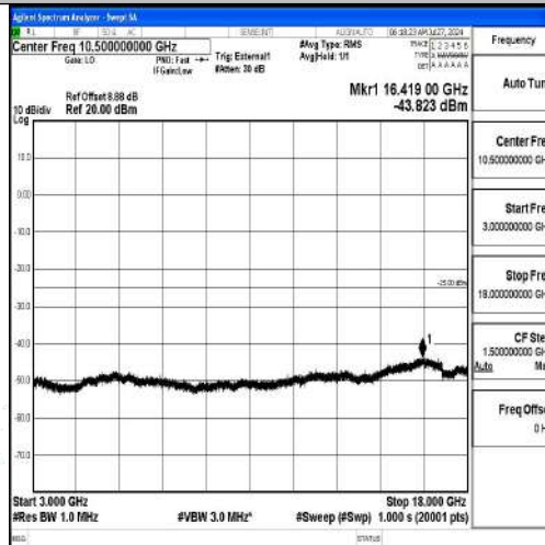
Band41-5MHz-QPSK-41565-1RB#0-3000~18000-PASS
