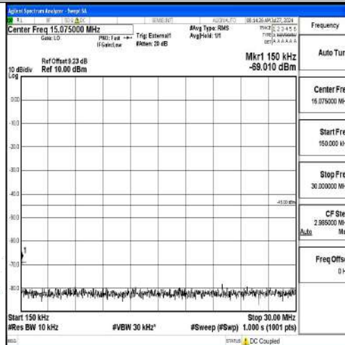
Band41-20MHz-16QAM-39750-1RB#0-0.15~30-PASS
