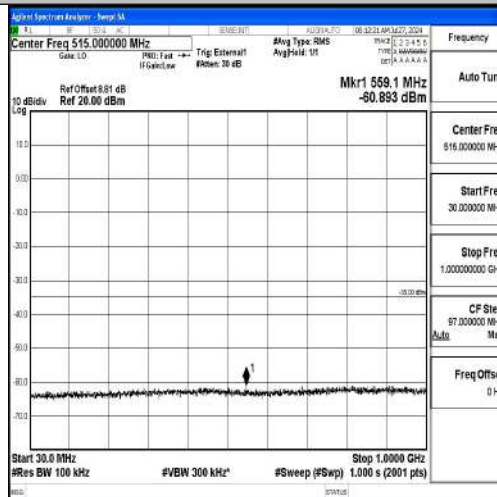
Band41-20MHz-QPSK-39750-1RB#0-30~1000-PASS
