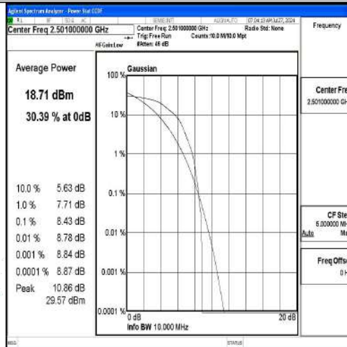
Band41-10MHz-16QAM-39700-1RB#0-PASS
