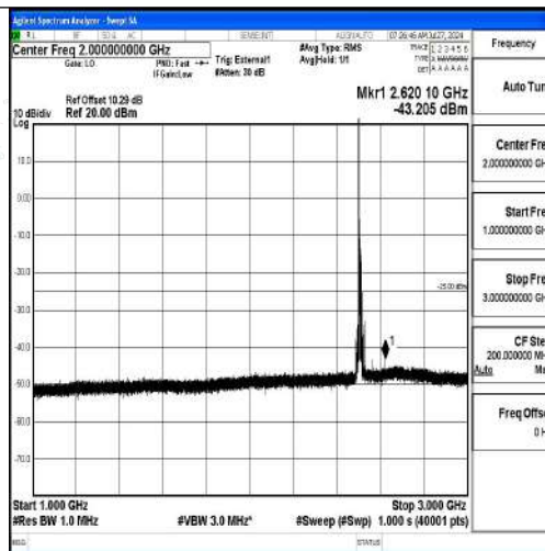
Band41-15MHz-QPSK-39725-1RB#0-1000~3000-PASS
