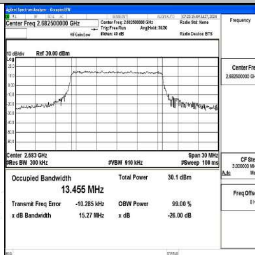
Band41-15MHz-QPSK-41515-75RB#0-PASS
