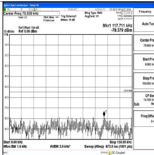
Band41-15MHz-QPSK-40620-1RB#0-0.009~0.15-PASS
