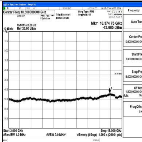
Band41-20MHz-16QAM-39750-1RB#0-3000~18000-PASS
