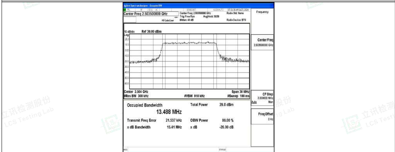
Band41-15MHz-16QAM-39725-75RB#0-PASS
