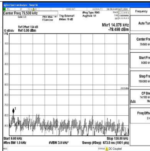
Band41-5MHz-16QAM-39675-1RB#0-0.009~0.15-PASS
