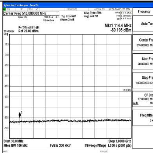
Band41-15MHz-QPSK-41515-1RB#0-30~1000-PASS
