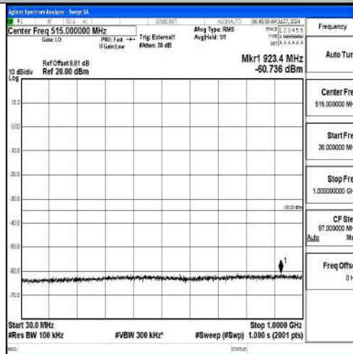
Band41-10MHz-QPSK-39700-1RB#0-30~1000-PASS
