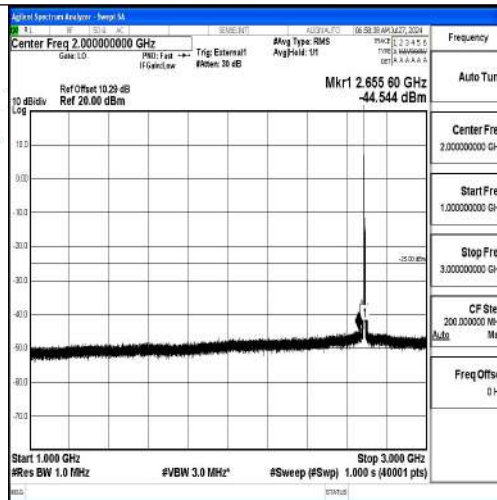
Band41-10MHz-16QAM-41540-1RB#0-1000~3000-PASS
