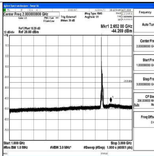
Band41-20MHz-QPSK-39750-1RB#0-1000~3000-PASS
