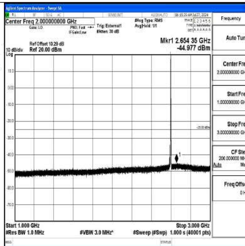
Band41-5MHz-16QAM-40620-1RB#0-1000~3000-PASS
