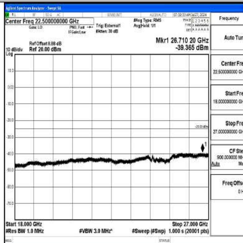
Band41-15MHz-QPSK-40620-1RB#0-18000~27000-PASS
