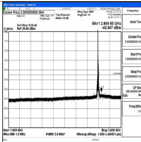
Band41-20MHz-16QAM-40620-1RB#0-1000~3000-PASS
