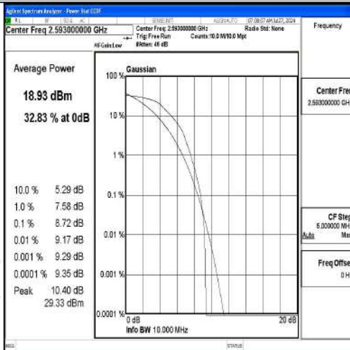
Band41-10MHz-QPSK-40620-1RB#0-PASS
