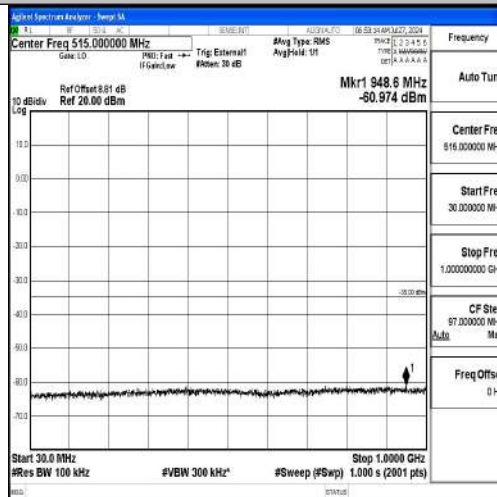
Band41-10MHz-16QAM-40620-1RB#0-30~1000-PASS
