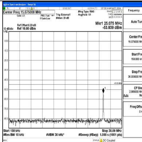
Band41-15MHz-16QAM-40620-1RB#0-0.15~30-PASS
