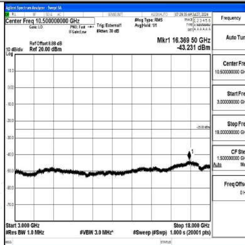
Band41-15MHz-16QAM-39725-1RB#0-3000~18000-PASS
