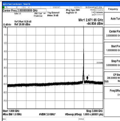
Band41-10MHz-16QAM-40620-1RB#0-1000~3000-PASS
