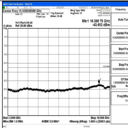
Band41-20MHz-16QAM-40620-1RB#0-3000~18000-PASS
