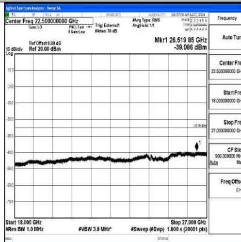
Band41-10MHz-QPSK-41540-1RB#0-18000~27000-PASS
