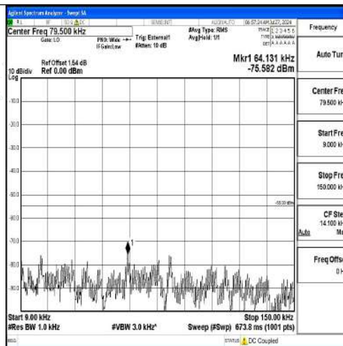
Band41-10MHz-16QAM-41540-1RB#0-0.009~0.15-PASS
