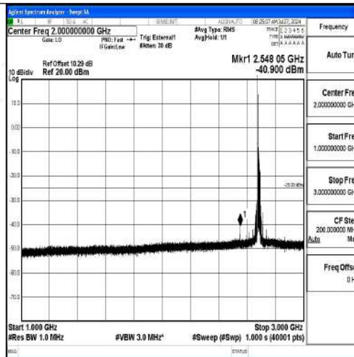
Band41-20MHz-16QAM-41490-1RB#0-1000~3000-PASS
