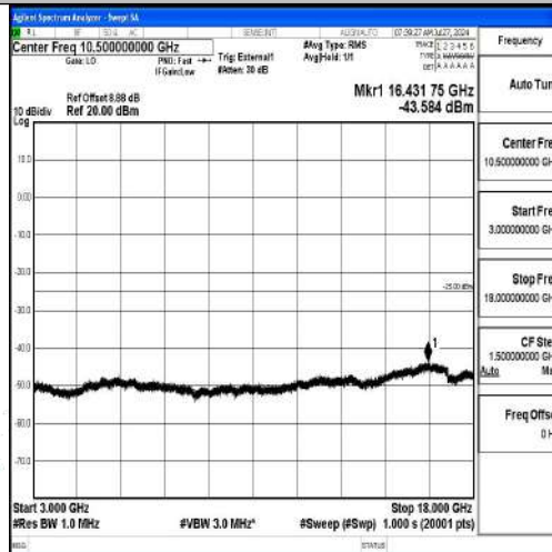
Band41-15MHz-16QAM-41515-1RB#0-3000~18000-PASS
