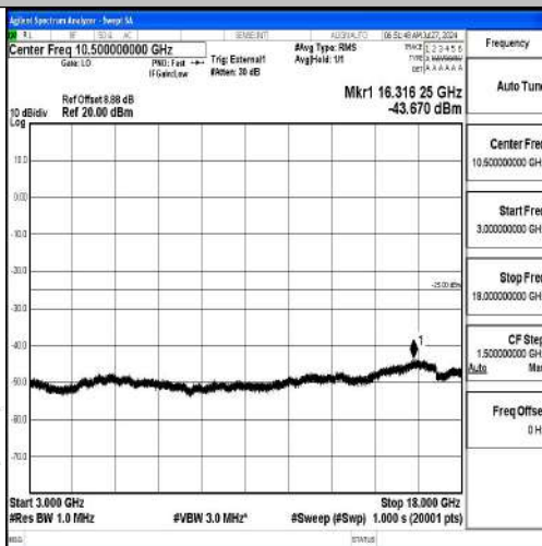
Band41-10MHz-QPSK-40620-1RB#0-3000~18000-PASS
