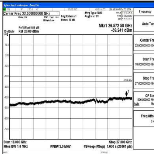
Band41-5MHz-QPSK-40620-1RB#0-18000~27000-PASS
