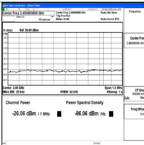
Band41-10MHz-QPSK-39700-50RB#0-PASS_Final1
