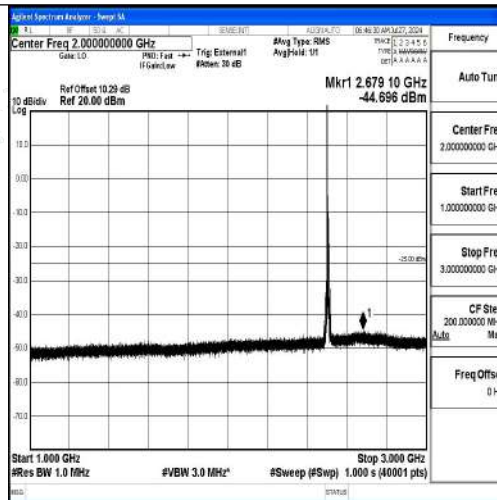
Band41-10MHz-QPSK-39700-1RB#0-1000~3000-PASS
