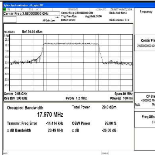
Band41-20MHz-16QAM-41490-100RB#0-PASS
