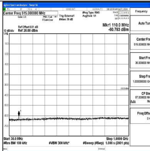
Band41-20MHz-QPSK-41490-1RB#0-30~1000-PASS
