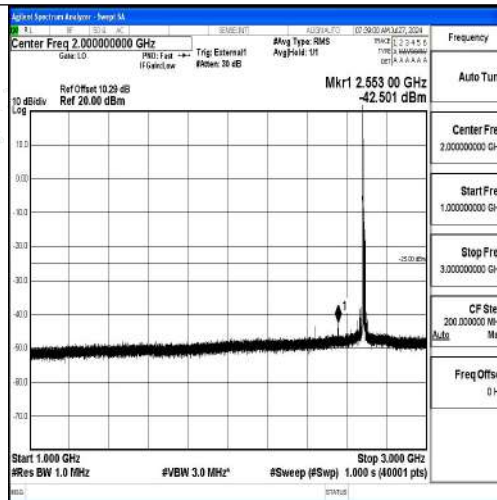
Band41-15MHz-16QAM-41515-1RB#0-1000~3000-PASS
