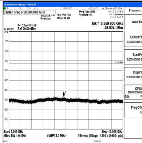
Band12-5MHz-16QAM-23035-1RB#0-3000~10000-PASS
