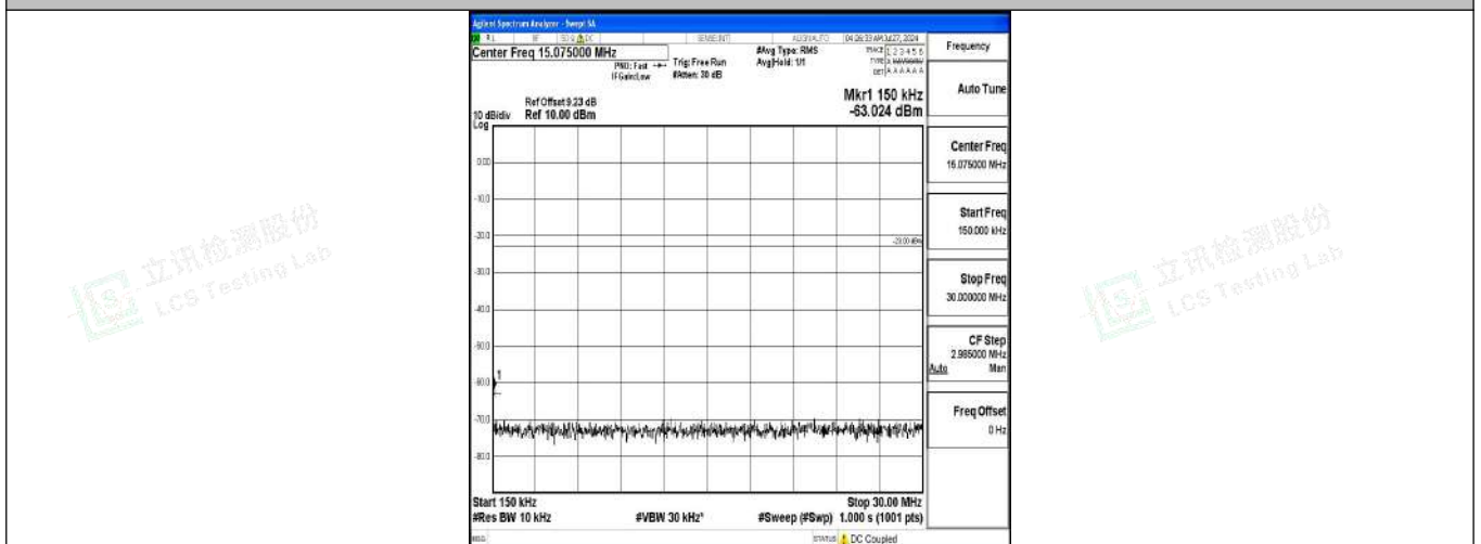
Band12-5MHz-16QAM-23095-1RB#0-0.15~30-PASS
