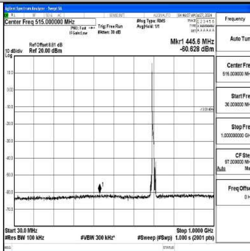
Band12-10MHz-16QAM-23060-1RB#0-30~1000-PASS
