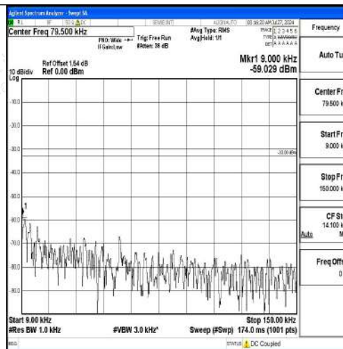
Band12-1.4MHz-QPSK-23173-1RB#0-0.009~0.15-PASS
