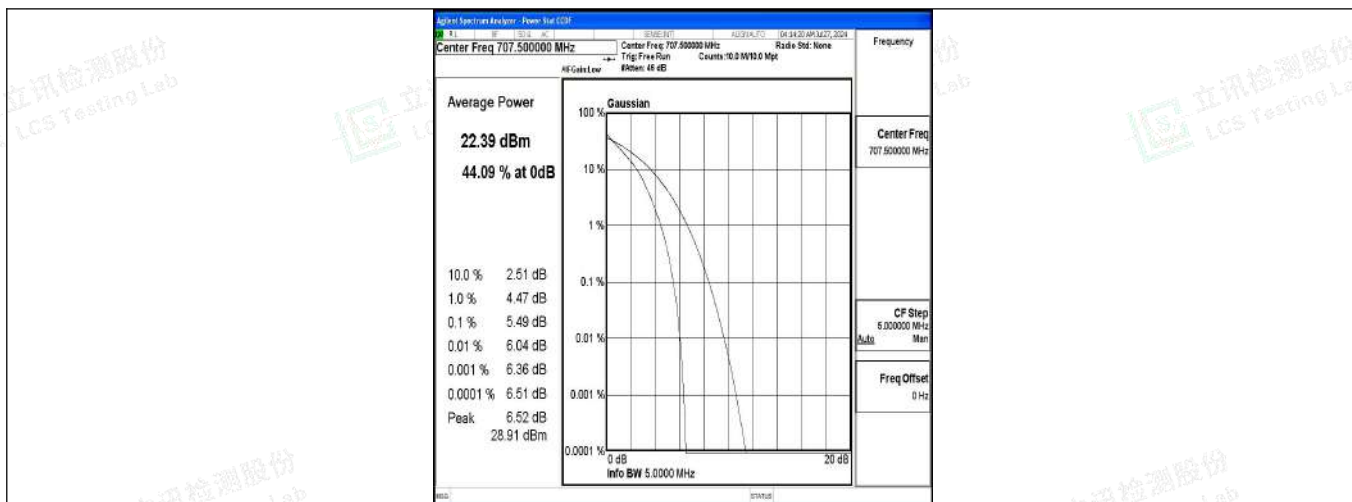
Band12-3MHz-QPSK-23095-15RB#0-PASS
