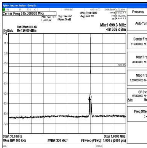
Band12-3MHz-16QAM-23095-1RB#0-30~1000-PASS
