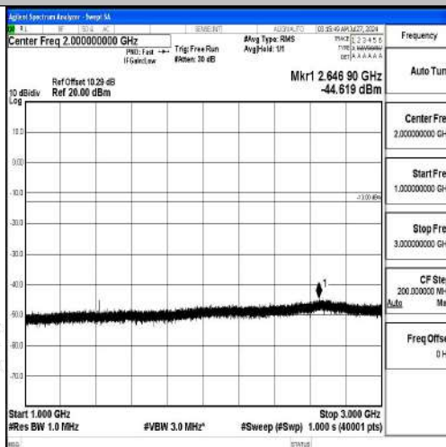
Band12-1.4MHz-16QAM-23095-1RB#0-1000~3000-PASS
