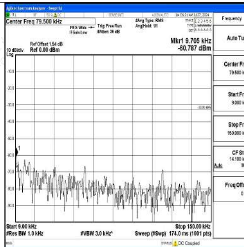
Band12-3MHz-QPSK-23165-1RB#0-0.009~0.15-PASS
