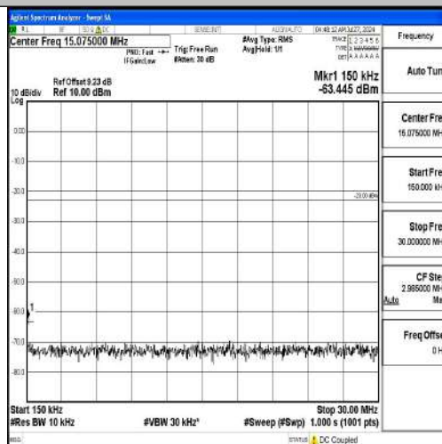
Band12-10MHz-16QAM-23095-1RB#0-0.15~30-PASS
