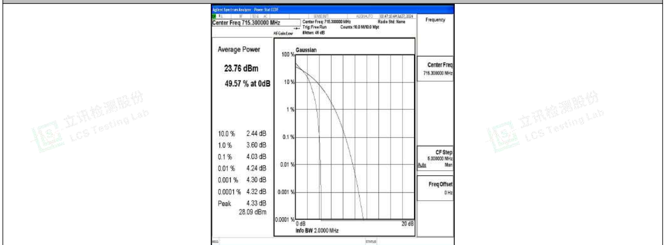
Band12-1.4MHz-QPSK-23173-1RB#0-PASS
