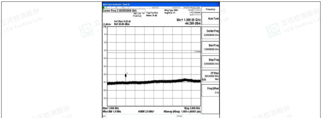
Band12-3MHz-16QAM-23025-1RB#0-1000~3000-PASS
