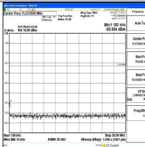
Band12-3MHz-16QAM-23025-1RB#0-0.15~30-PASS
