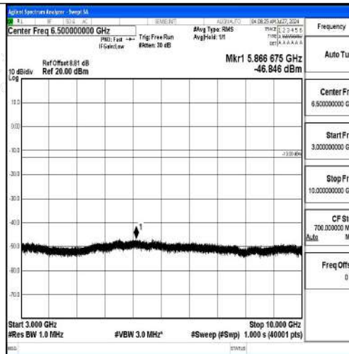
Band12-3MHz-16QAM-23165-1RB#0-3000~10000-PASS
