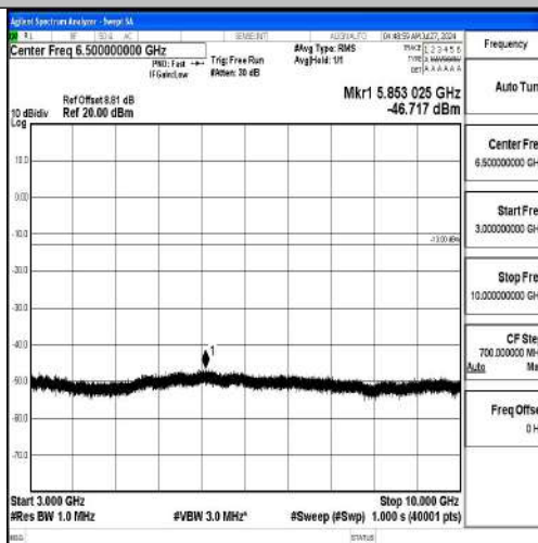
Band12-10MHz-16QAM-23095-1RB#0-3000~10000-PASS
