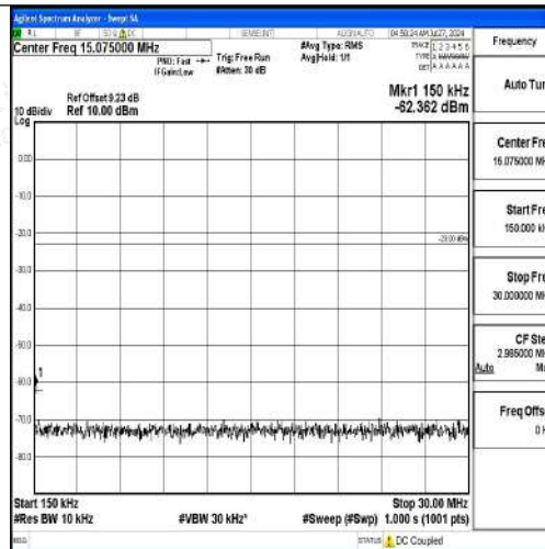
Band12-10MHz-16QAM-23130-1RB#0-0.15~30-PASS
