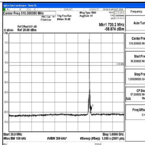
Band12-5MHz-16QAM-23095-1RB#0-30~1000-PASS
