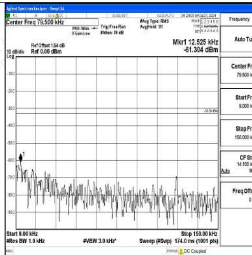
Band12-5MHz-16QAM-23035-1RB#0-0.009~0.15-PASS
