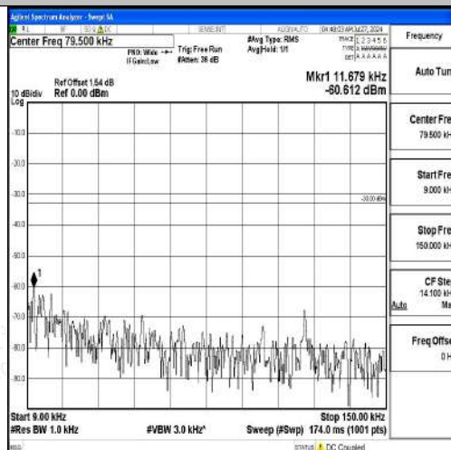
Band12-10MHz-16QAM-23095-1RB#0-0.009~0.15-PASS
