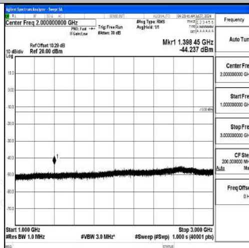
Band12-5MHz-QPSK-23035-1RB#0-1000~3000-PASS
