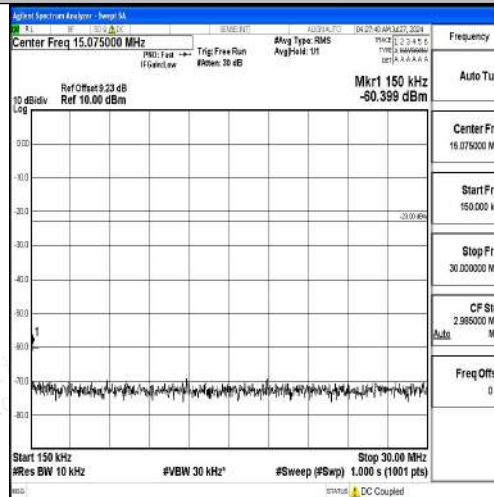
Band12-5MHz-QPSK-23155-1RB#0-0.15~30-PASS
