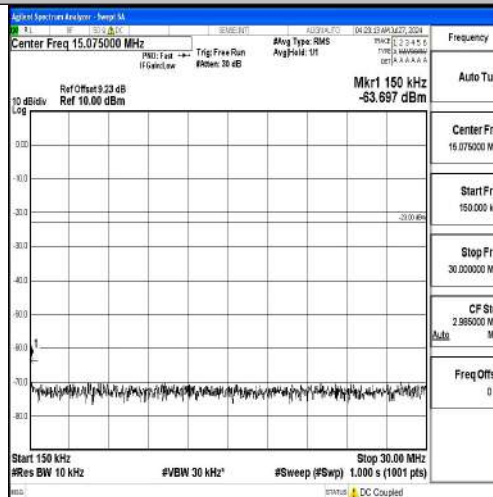
Band12-5MHz-QPSK-23035-1RB#0-0.15~30-PASS
