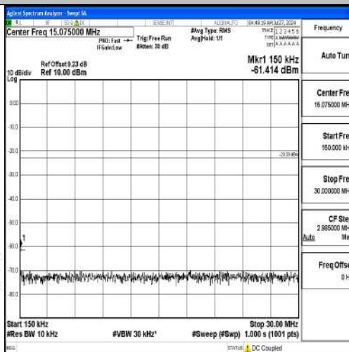
Band12-10MHz-QPSK-23130-1RB#0-0.15~30-PASS
