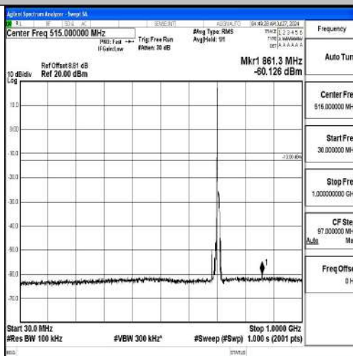
Band12-10MHz-QPSK-23130-1RB#0-30~1000-PASS
