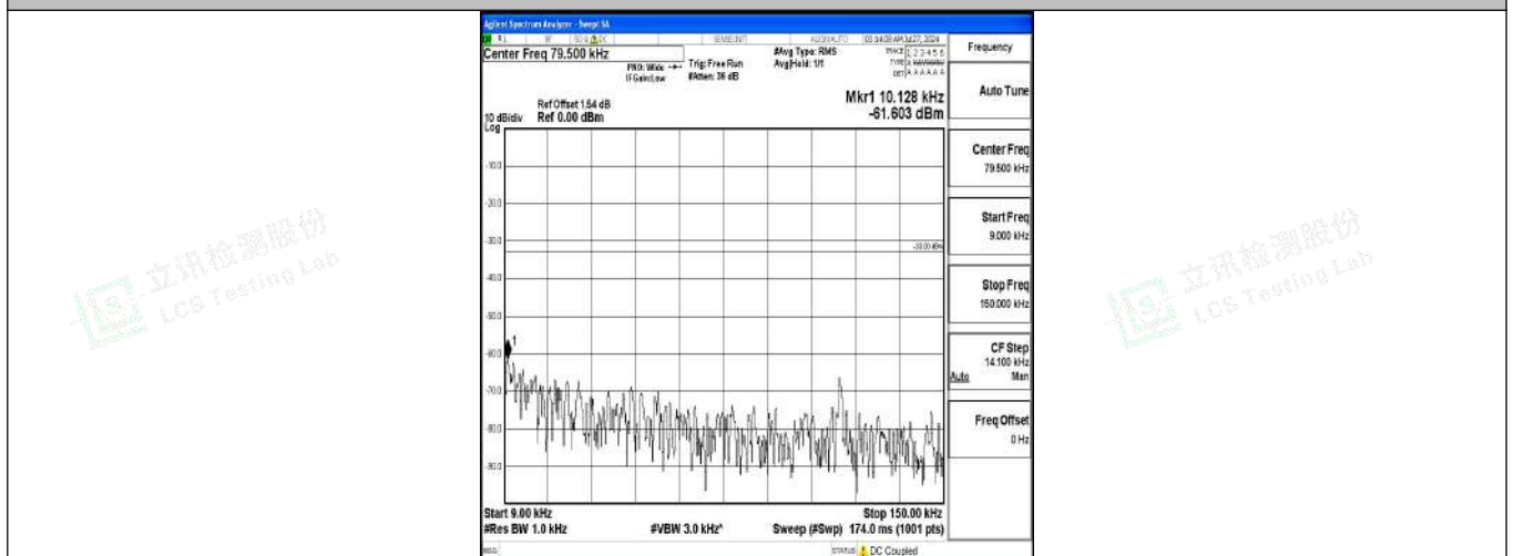
Band12-1.4MHz-QPSK-23095-1RB#0-0.009~0.15-PASS
