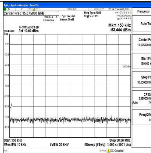
Band12-1.4MHz-QPSK-23095-1RB#0-0.15~30-PASS
