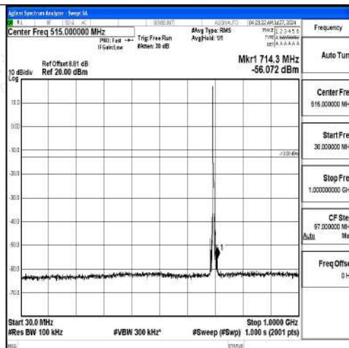
Band12-5MHz-QPSK-23035-1RB#0-30~1000-PASS
