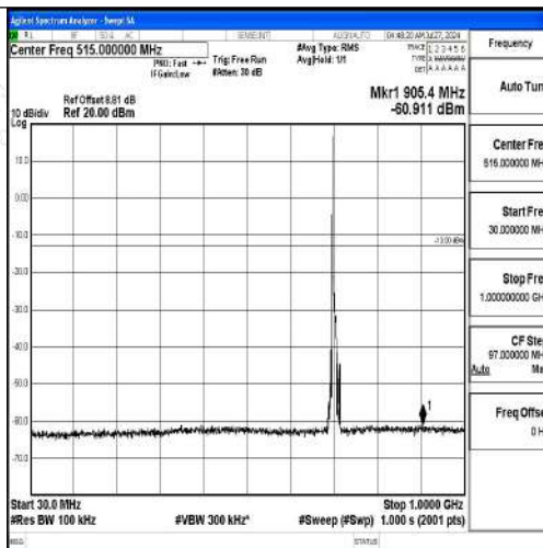
Band12-10MHz-16QAM-23095-1RB#0-30~1000-PASS
