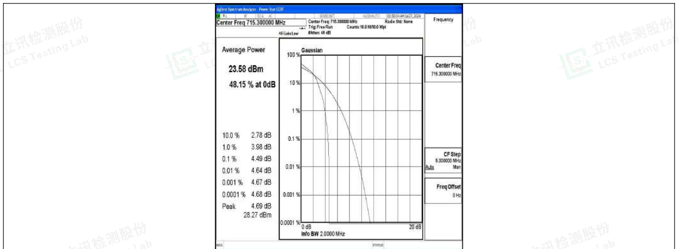
Band12-1.4MHz-16QAM-23173-1RB#0-PASS
