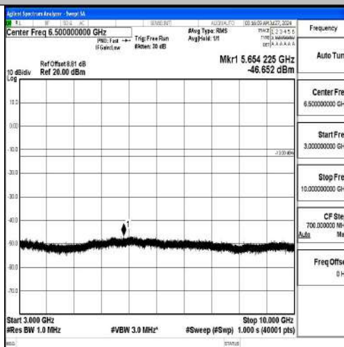
Band12-1.4MHz-16QAM-23095-1RB#0-3000~10000-PASS
