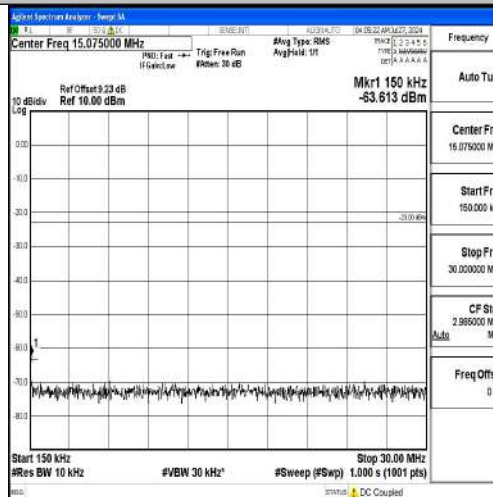
Band12-3MHz-16QAM-23095-1RB#0-0.15~30-PASS
