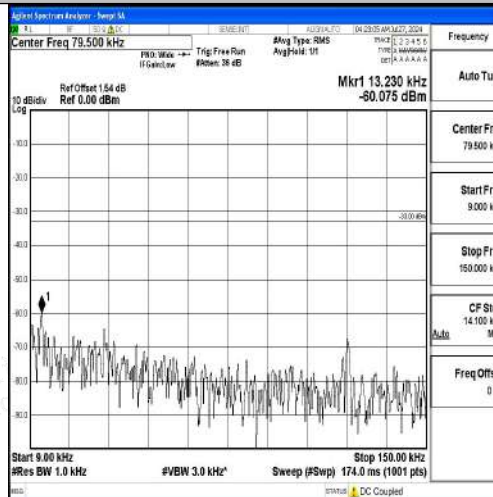
Band12-5MHz-QPSK-23035-1RB#0-0.009~0.15-PASS
