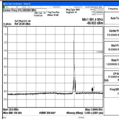
Band12-10MHz-QPSK-23095-1RB#0-30~1000-PASS
