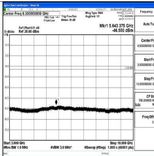
Band12-3MHz-QPSK-23095-1RB#0-3000~10000-PASS
