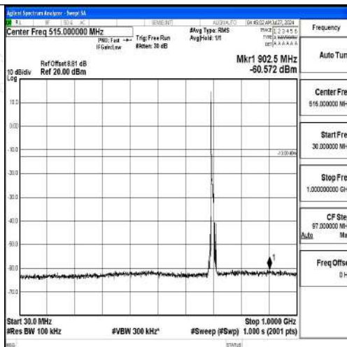
Band12-10MHz-QPSK-23060-1RB#0-30~1000-PASS
