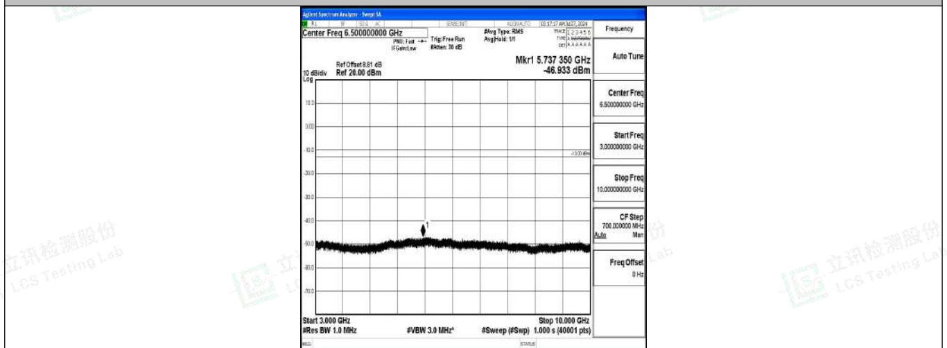
Band12-1.4MHz-QPSK-23173-1RB#0-3000~10000-PASS
