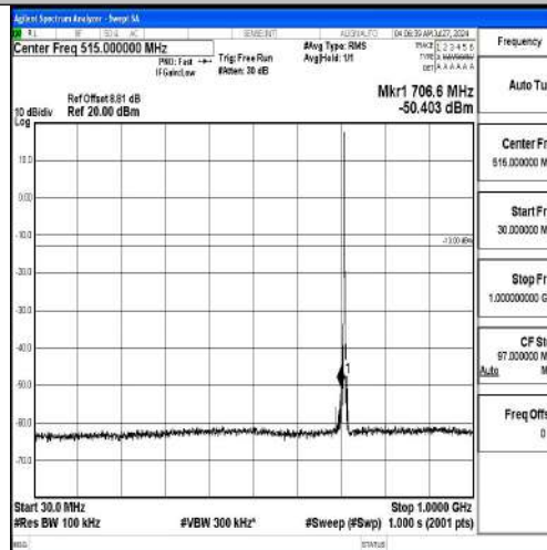
Band12-3MHz-QPSK-23165-1RB#0-30~1000-PASS
