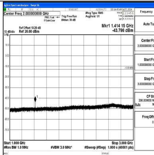
Band12-1.4MHz-QPSK-23095-1RB#0-1000~3000-PASS
