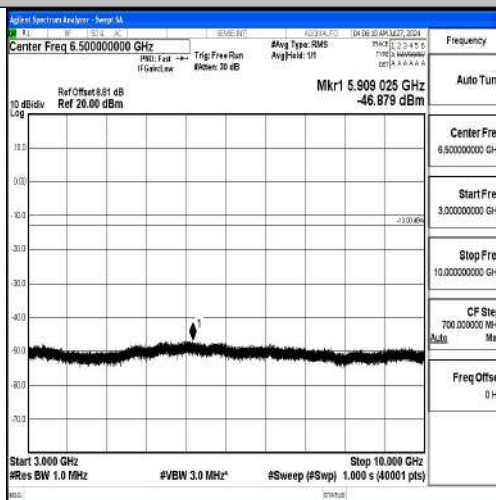
Band12-3MHz-16QAM-23095-1RB#0-3000~10000-PASS
