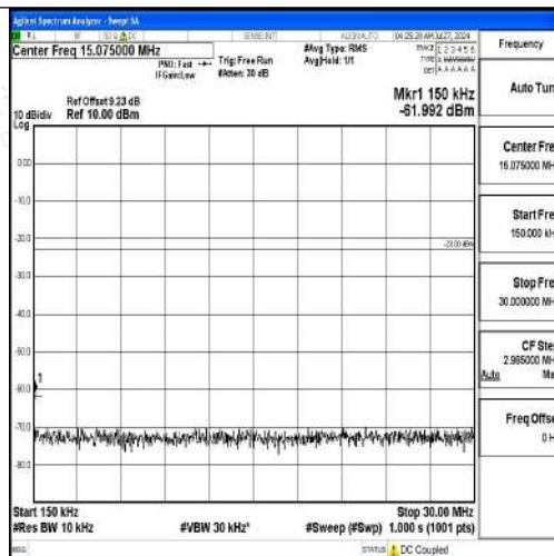
Band12-5MHz-QPSK-23095-1RB#0-0.15~30-PASS
