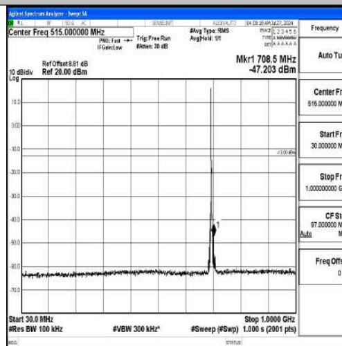
Band12-3MHz-16QAM-23025-1RB#0-30~1000-PASS
