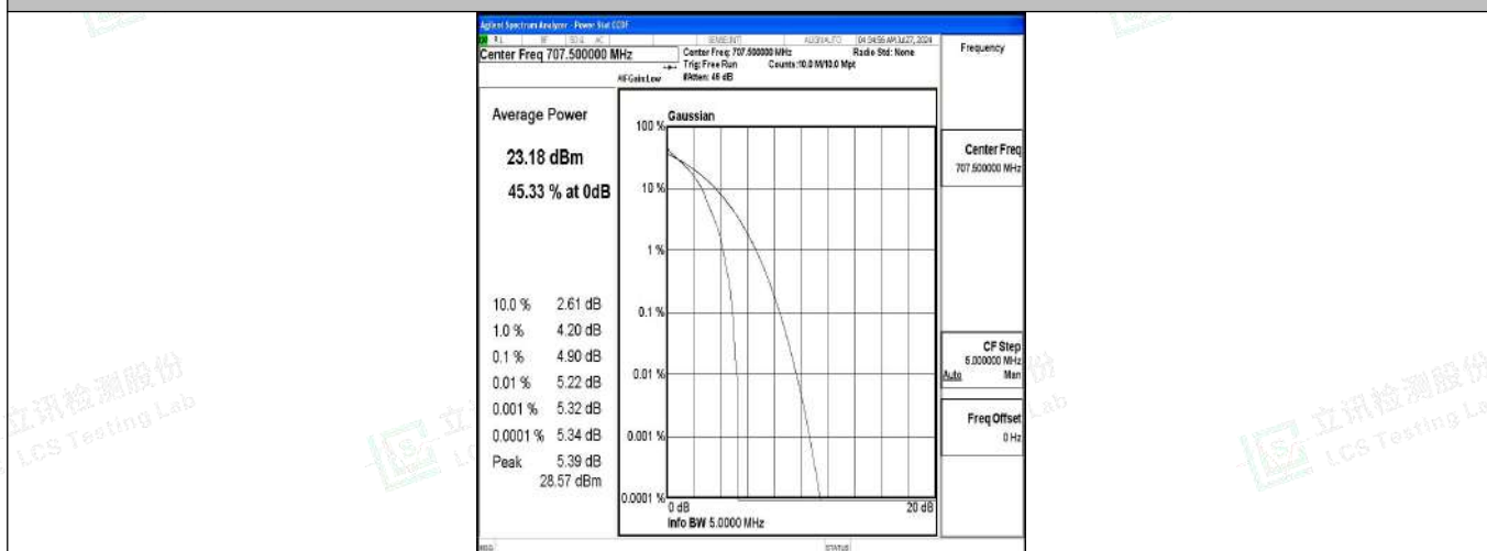
Band12-5MHz-QPSK-23095-1RB#0-PASS
