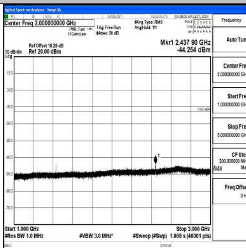
Band12-3MHz-16QAM-23165-1RB#0-1000~3000-PASS
