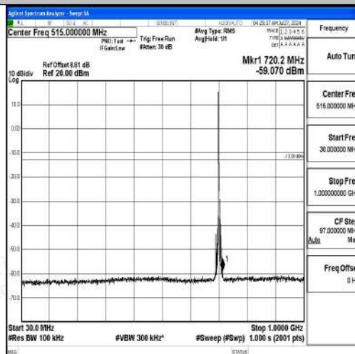
Band12-5MHz-QPSK-23095-1RB#0-30~1000-PASS
