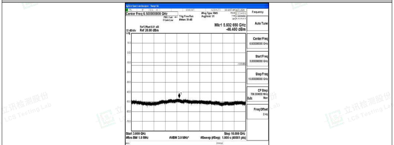
Band12-1.4MHz-16QAM-23017-1RB#0-3000~10000-PASS
