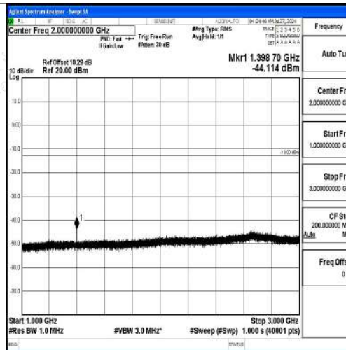
Band12-5MHz-16QAM-23035-1RB#0-1000~3000-PASS
