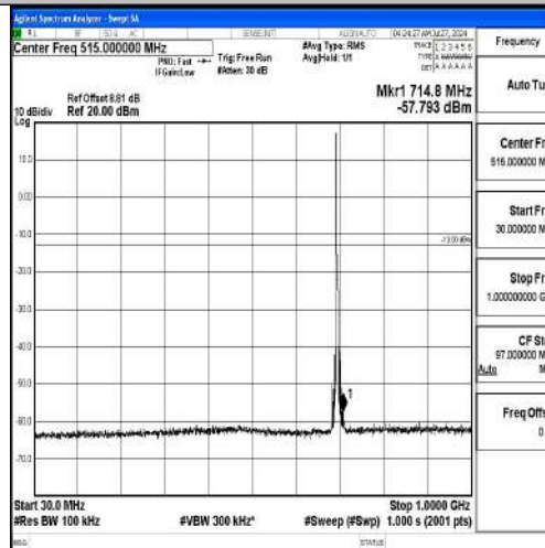
Band12-5MHz-16QAM-23035-1RB#0-30~1000-PASS
