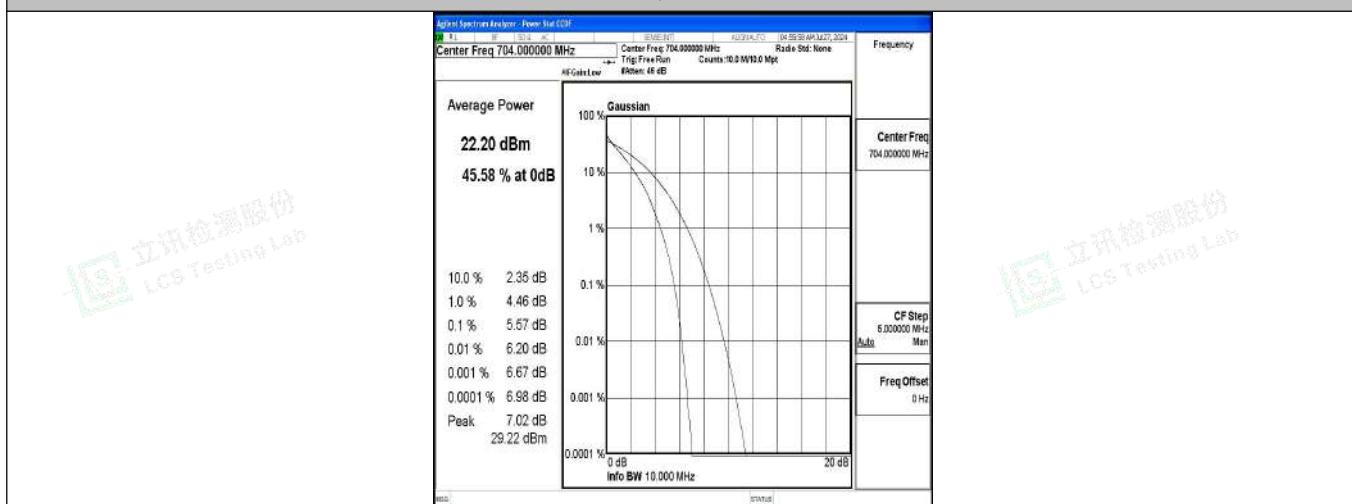
Band12-10MHz-QPSK-23060-50RB#0-PASS
