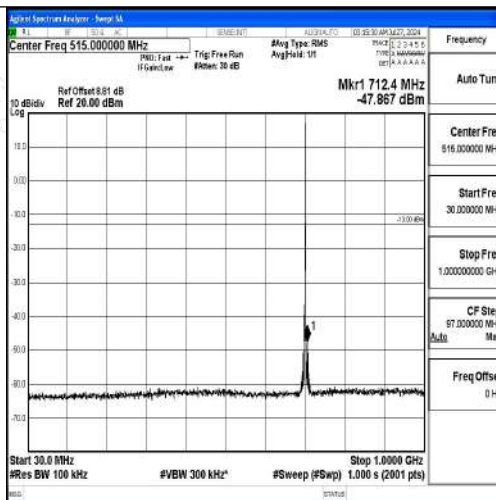
Band12-1.4MHz-16QAM-23095-1RB#0-30~1000-PASS
