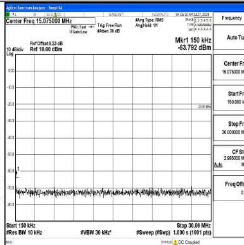
Band12-3MHz-QPSK-23165-1RB#0-0.15~30-PASS
