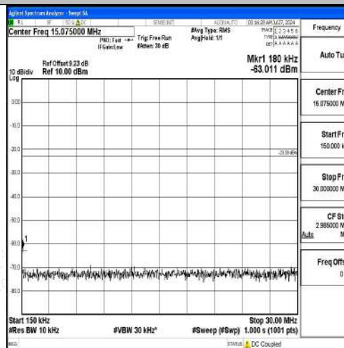
Band12-1.4MHz-QPSK-23173-1RB#0-0.15~30-PASS
