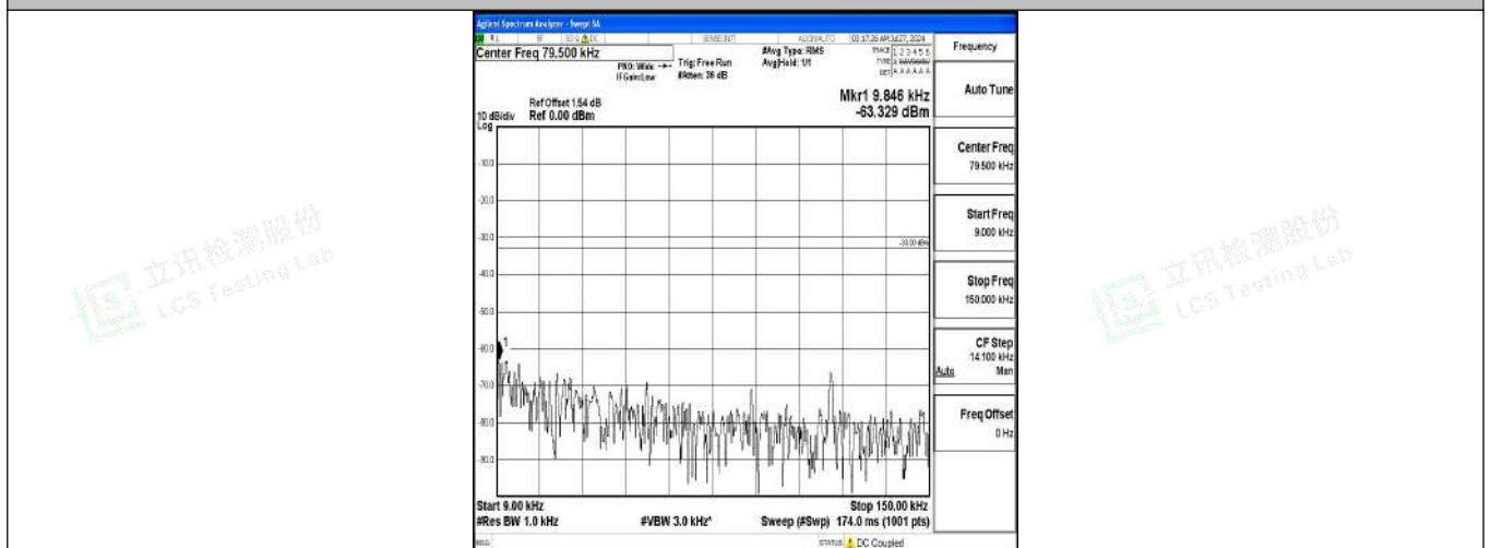
Band12-1.4MHz-16QAM-23173-1RB#0-0.009~0.15-PASS
