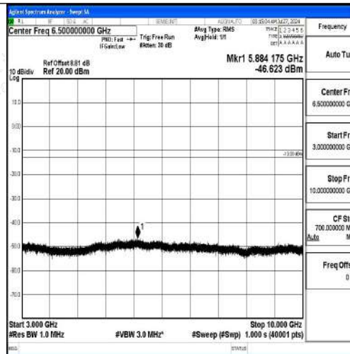
Band12-1.4MHz-QPSK-23095-1RB#0-3000~10000-PASS
