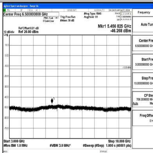
Band12-5MHz-QPSK-23035-1RB#0-3000~10000-PASS
