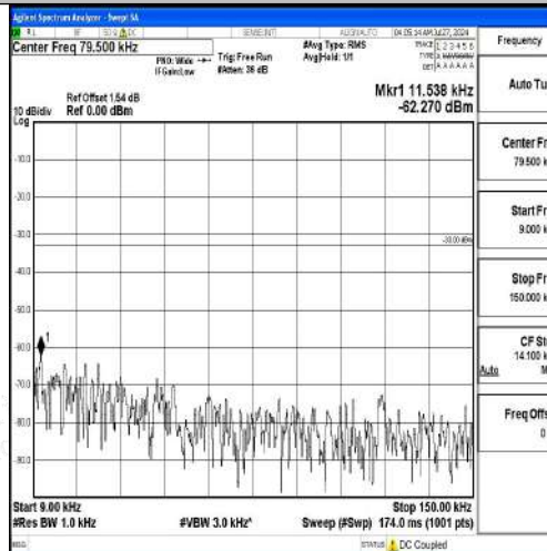
Band12-3MHz-16QAM-23095-1RB#0-0.009~0.15-PASS
