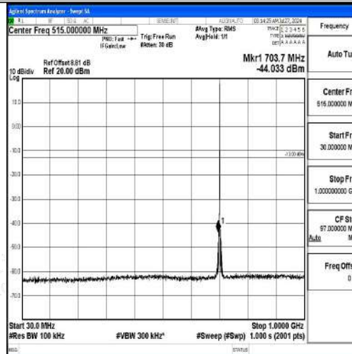
Band12-1.4MHz-QPSK-23095-1RB#0-30~1000-PASS
