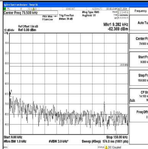
Band12-1.4MHz-16QAM-23095-1RB#0-0.009~0.15-PASS
