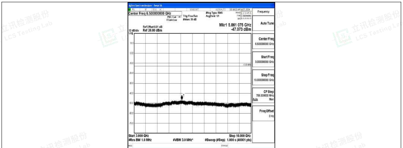
Band12-1.4MHz-16QAM-23173-1RB#0-3000~10000-PASS
