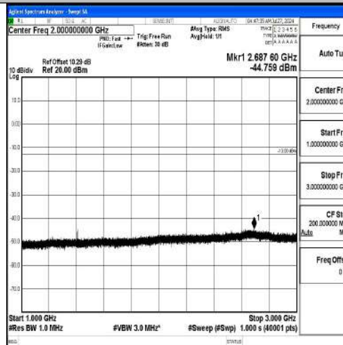
Band12-10MHz-QPSK-23095-1RB#0-1000~3000-PASS
