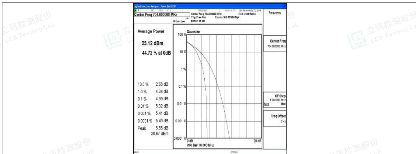
Band12-10MHz-QPSK-23060-1RB#0-PASS
