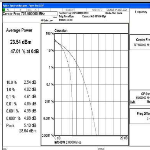
Band12-1.4MHz-QPSK-23095-1RB#0-PASS
