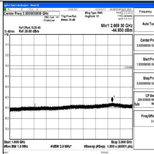
Band12-10MHz-16QAM-23130-1RB#0-1000~3000-PASS
