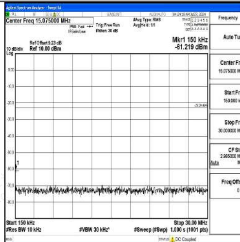
Band12-5MHz-16QAM-23035-1RB#0-0.15~30-PASS
