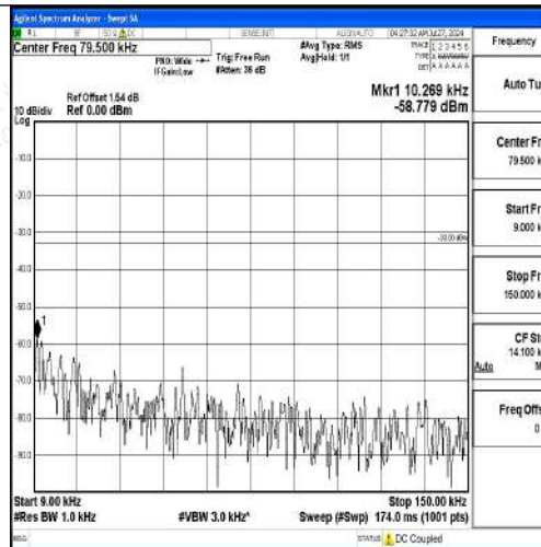
Band12-5MHz-QPSK-23155-1RB#0-0.009~0.15-PASS
