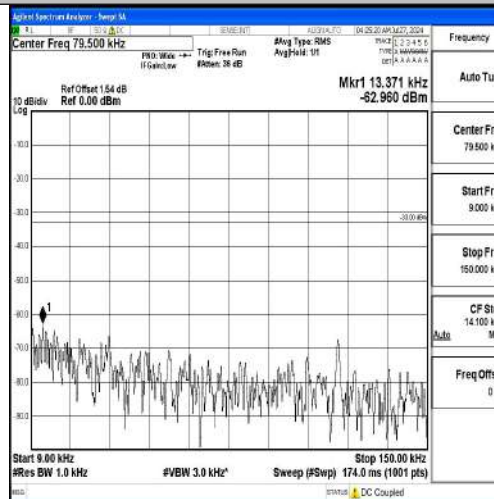
Band12-5MHz-QPSK-23095-1RB#0-0.009~0.15-PASS
