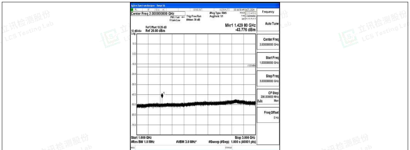
Band12-1.4MHz-QPSK-23173-1RB#0-1000~3000-PASS
