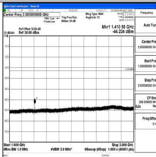
Band12-5MHz-QPSK-23095-1RB#0-1000~3000-PASS
