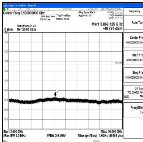
Band12-10MHz-QPSK-23095-1RB#0-3000~10000-PASS
