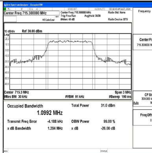
Band12-1.4MHz-QPSK-23173-6RB#0-PASS
