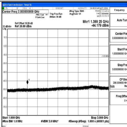
Band12-10MHz-QPSK-23060-1RB#0-1000~3000-PASS
