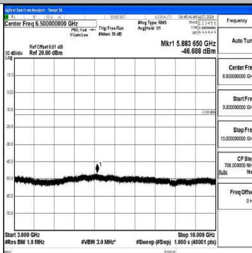
Band12-10MHz-QPSK-23060-1RB#0-3000~10000-PASS
