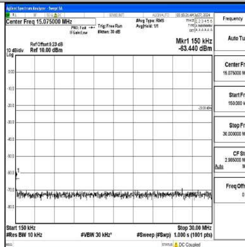
Band12-1.4MHz-16QAM-23095-1RB#0-0.15~30-PASS
