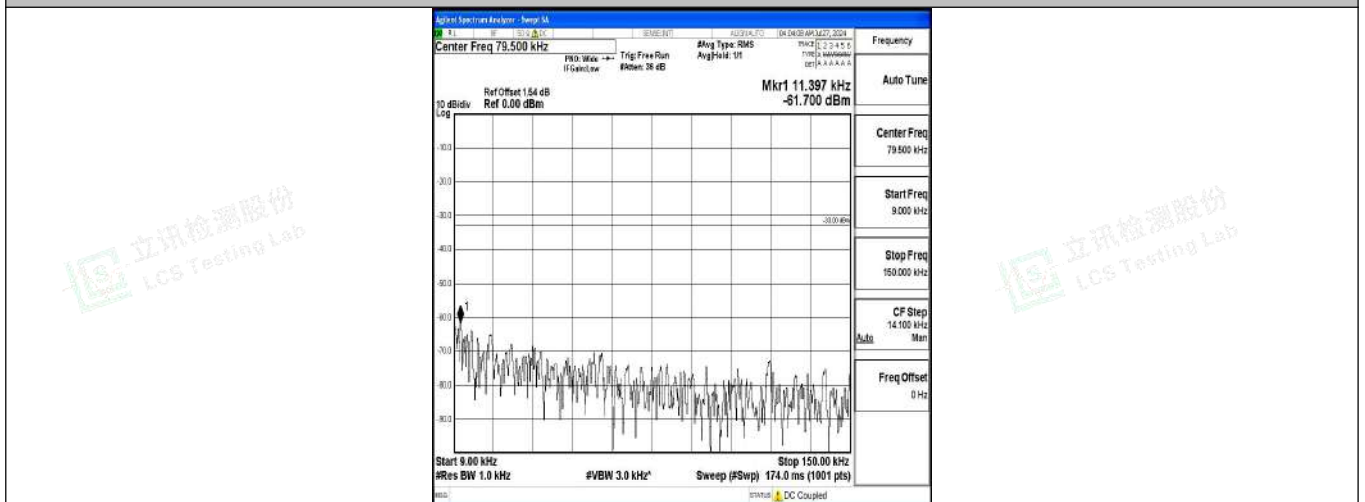
Band12-3MHz-QPSK-23095-1RB#0-0.009~0.15-PASS
