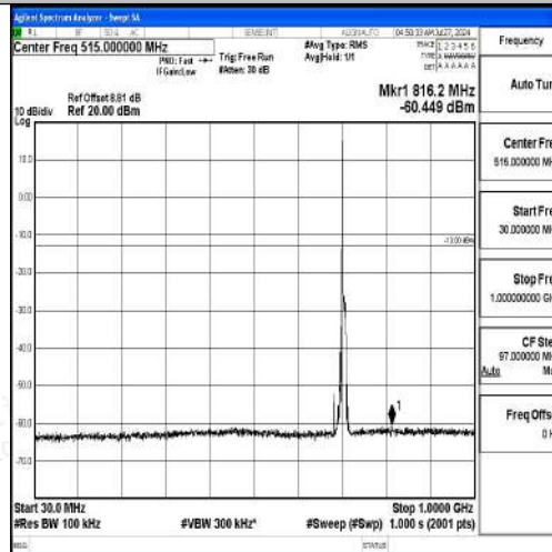
Band12-10MHz-16QAM-23130-1RB#0-30~1000-PASS
