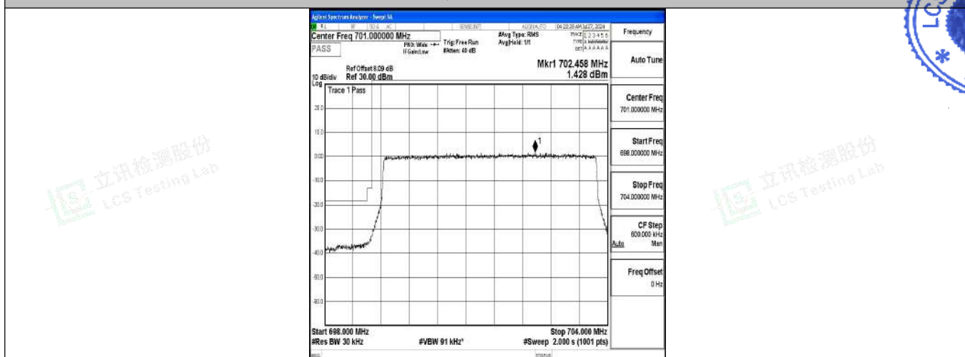
Band12-5MHz-16QAM-23035-25RB#0-PASS
