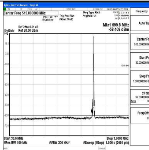
Band12-5MHz-QPSK-23155-1RB#0-30~1000-PASS
