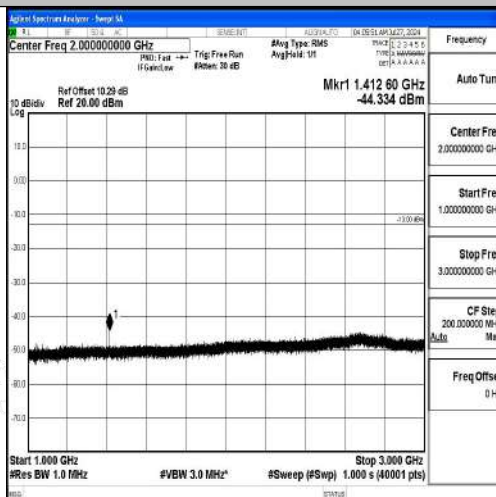
Band12-3MHz-16QAM-23095-1RB#0-1000~3000-PASS
