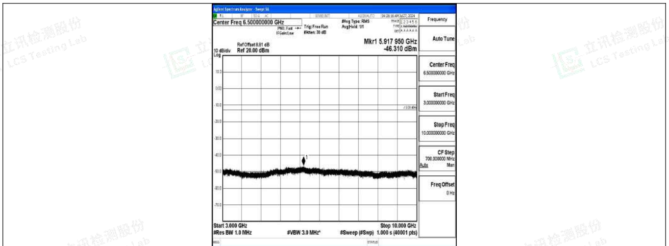
Band12-5MHz-QPSK-23095-1RB#0-3000~10000-PASS
