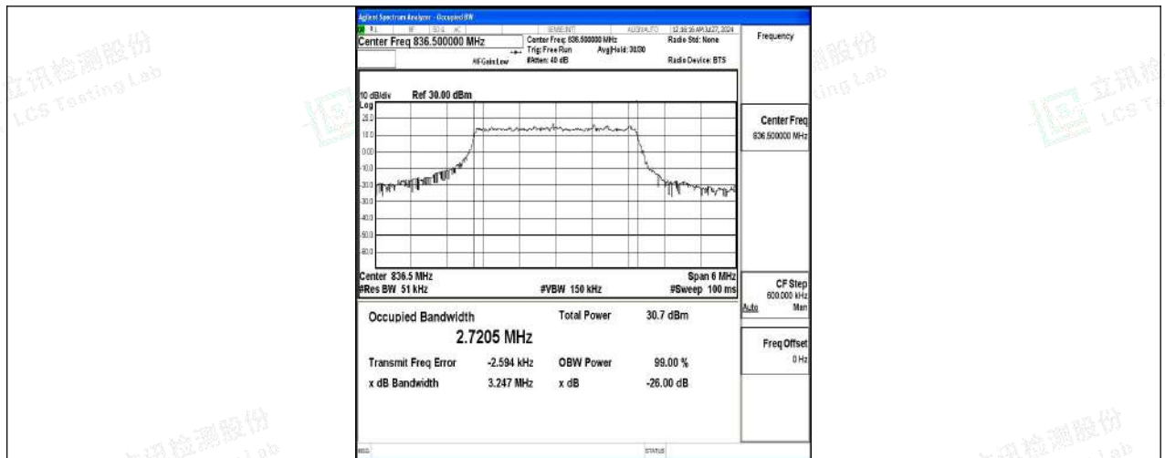
Band5-3MHz-16QAM-20525-15RB#0-PASS
