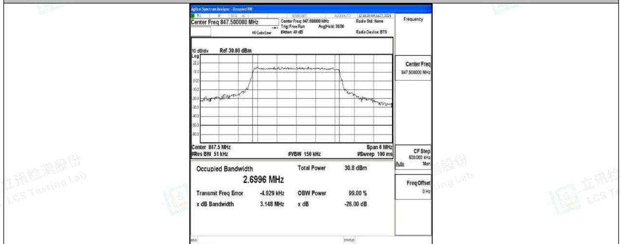
Band5-3MHz-QPSK-20635-15RB#0-PASS
