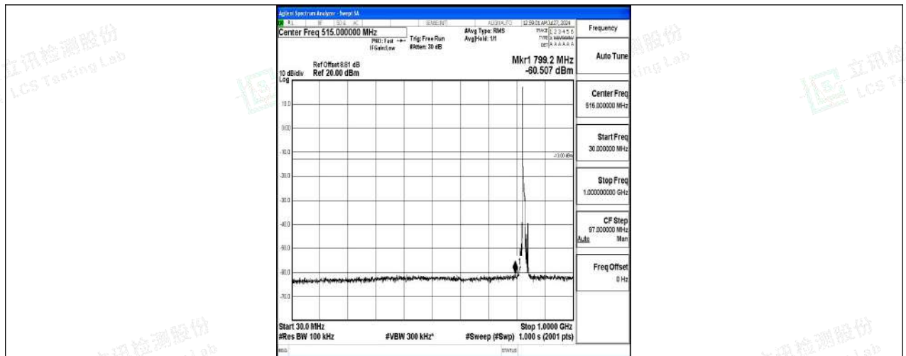
Band5-10MHz-QPSK-20450-1RB#0-30~1000-PASS
