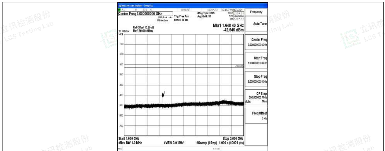
Band5-3MHz-16QAM-20415-1RB#0-1000~3000-PASS
