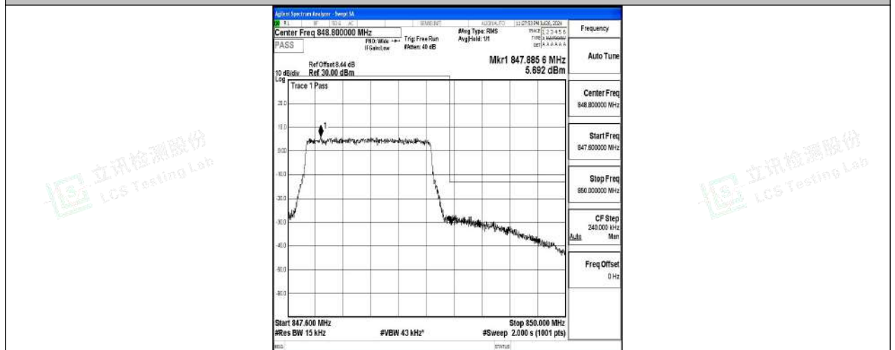
Band5-1.4MHz-16QAM-20643-6RB#0-PASS
