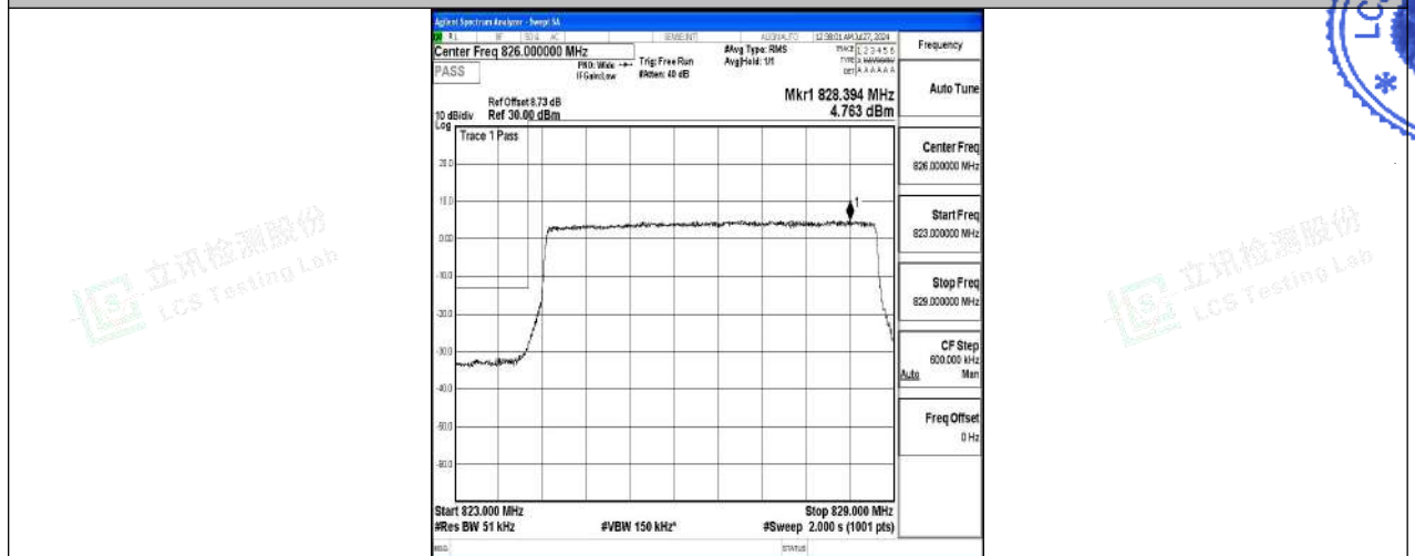
Band5-5MHz-16QAM-20425-25RB#0-PASS
