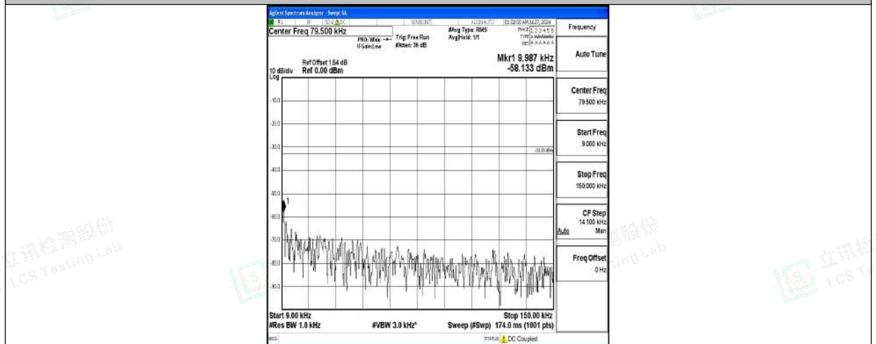
Band5-10MHz-16QAM-20525-1RB#0-0.009~0.15-PASS
