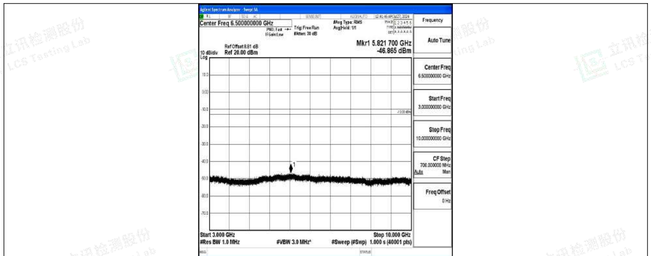
Band5-5MHz-QPSK-20525-1RB#0-3000~10000-PASS
