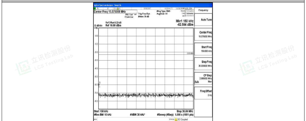
Band5-1.4MHz-16QAM-20525-1RB#0-0.15~30-PASS
