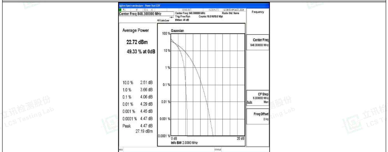
Band5-1.4MHz-QPSK-20643-6RB#0-PASS
