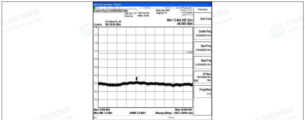
Band5-1.4MHz-QPSK-20525-1RB#0-3000~10000-PASS
