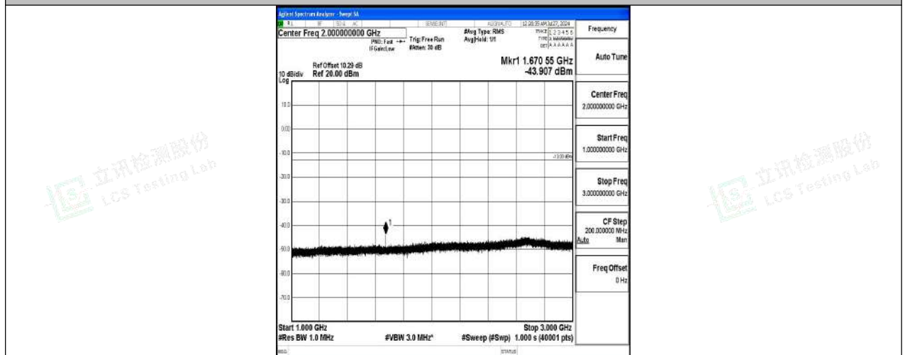
Band5-3MHz-QPSK-20525-1RB#0-1000~3000-PASS
