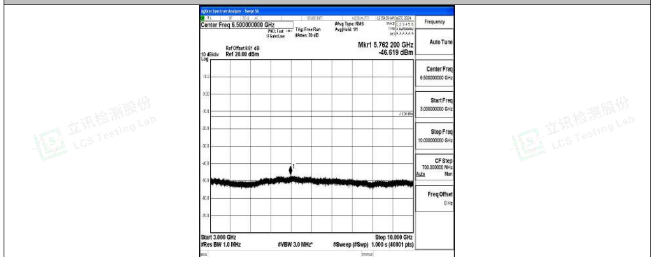
Band5-10MHz-QPSK-20450-1RB#0-3000~10000-PASS
