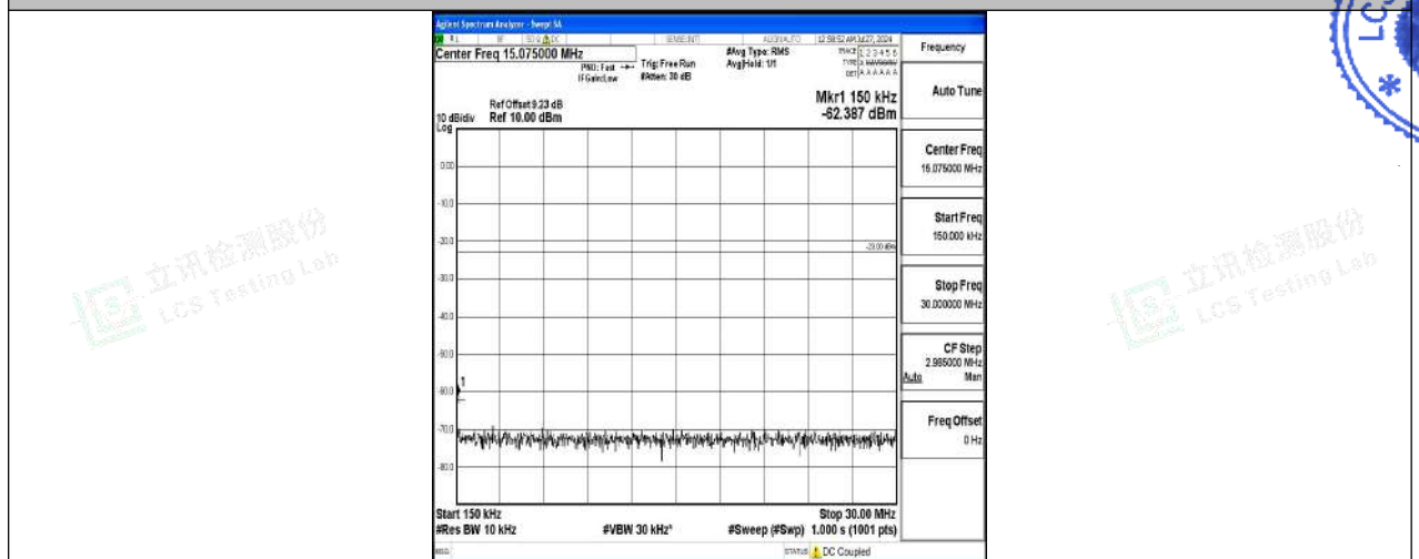
Band5-10MHz-QPSK-20450-1RB#0-0.15~30-PASS
