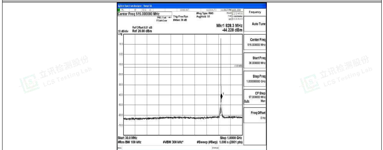
Band5-1.4MHz-16QAM-20407-1RB#0-30~1000-PASS
