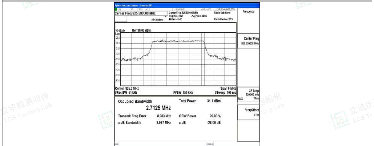
Band5-3MHz-16QAM-20415-15RB#0-PASS
