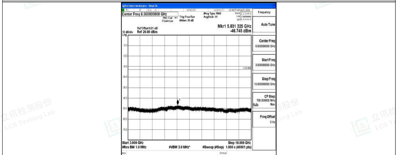
Band5-5MHz-QPSK-20625-1RB#0-3000~10000-PASS
