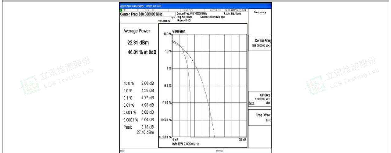
Band5-1.4MHz-16QAM-20643-6RB#0-PASS
