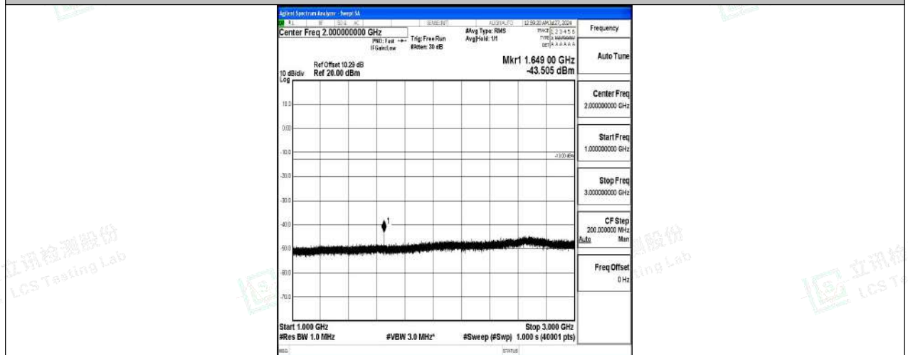
Band5-10MHz-QPSK-20450-1RB#0-1000~3000-PASS
