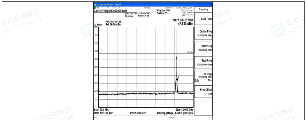
Band5-3MHz-QPSK-20415-1RB#0-30~1000-PASS
