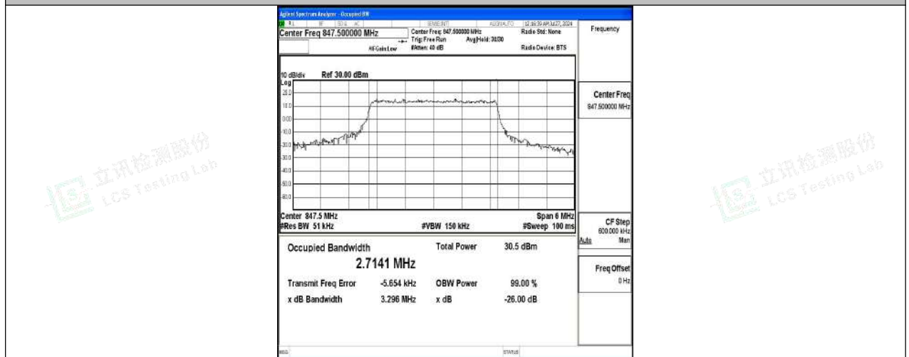
Band5-3MHz-16QAM-20635-15RB#0-PASS
