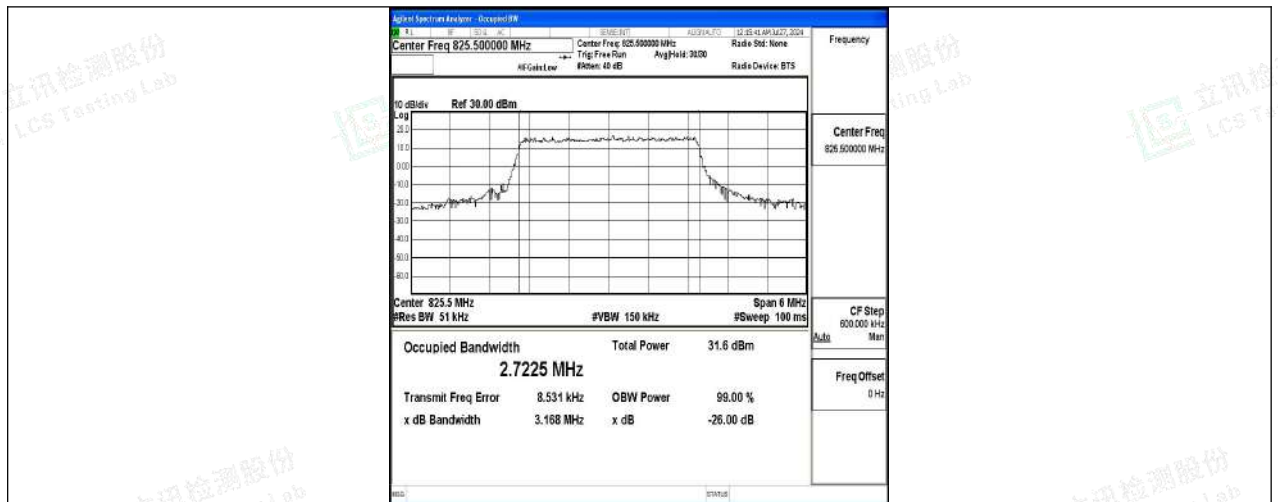
Band5-3MHz-QPSK-20415-15RB#0-PASS
