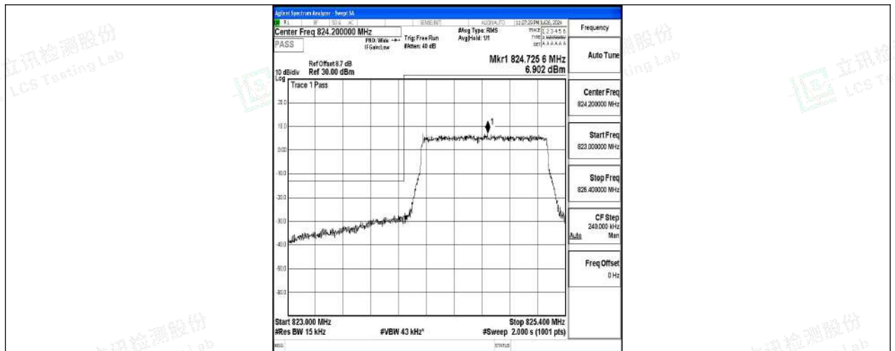
Band5-1.4MHz-16QAM-20407-6RB#0-PASS
