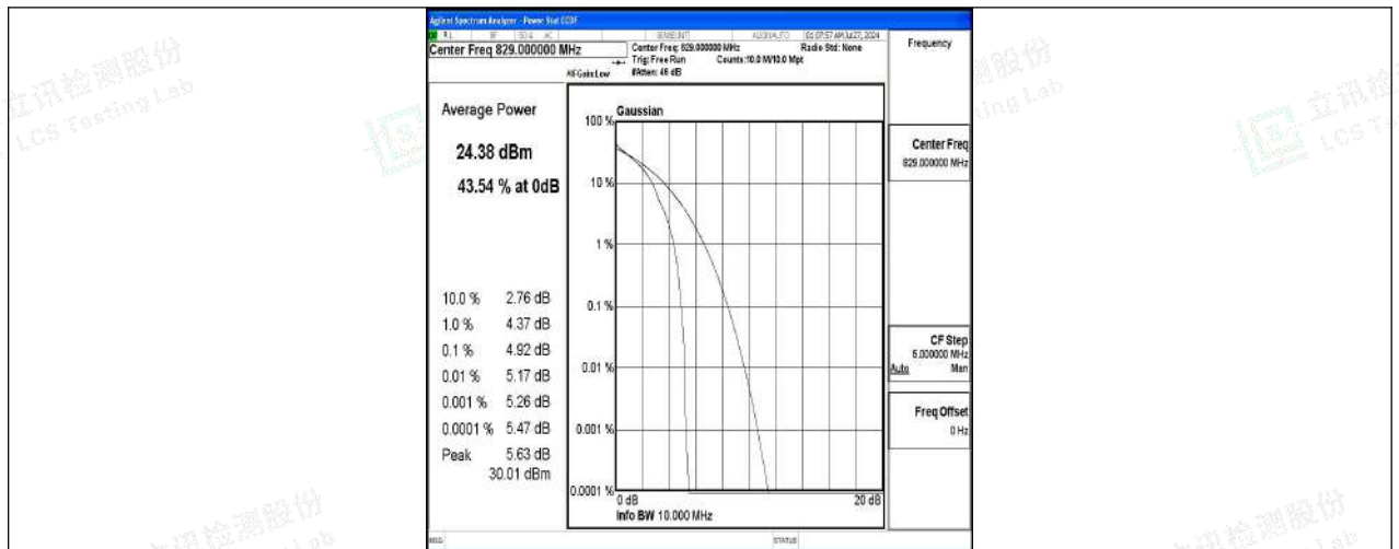
Band5-10MHz-QPSK-20450-1RB#0-PASS
