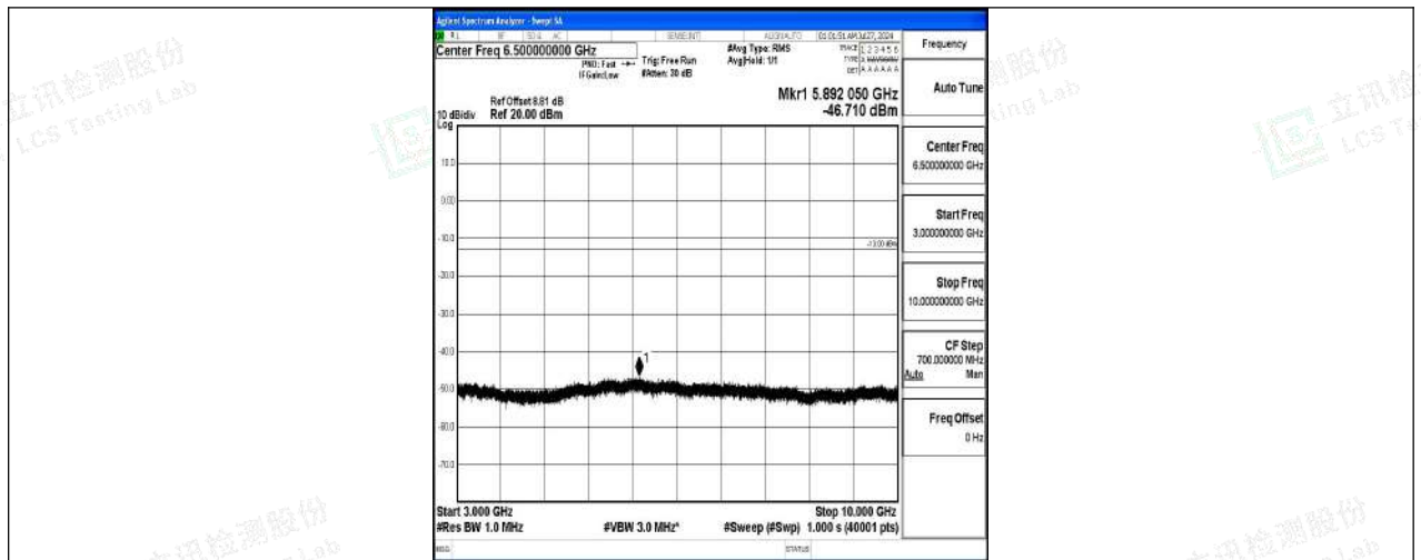
Band5-10MHz-QPSK-20525-1RB#0-3000~10000-PASS
