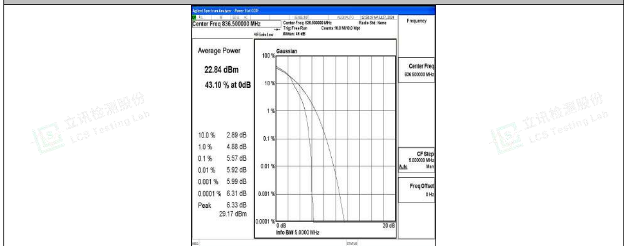
Band5-5MHz-16QAM-20525-1RB#0-PASS
