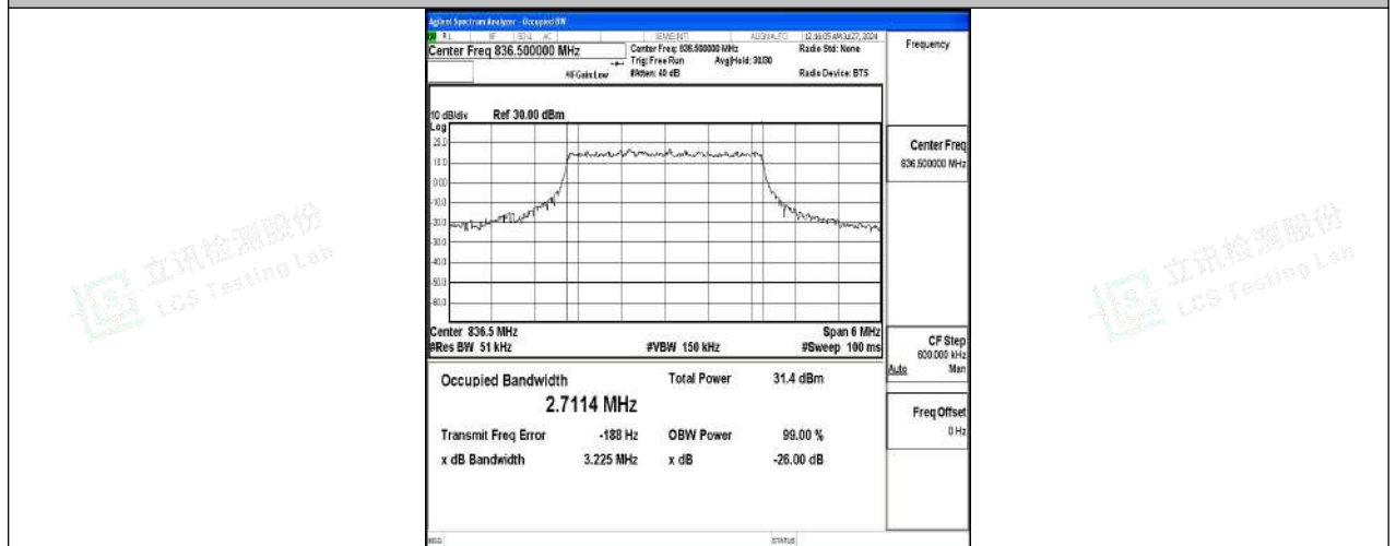
Band5-3MHz-QPSK-20525-15RB#0-PASS
