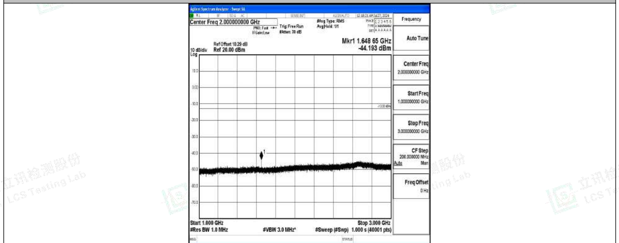
Band5-3MHz-QPSK-20415-1RB#0-1000~3000-PASS
