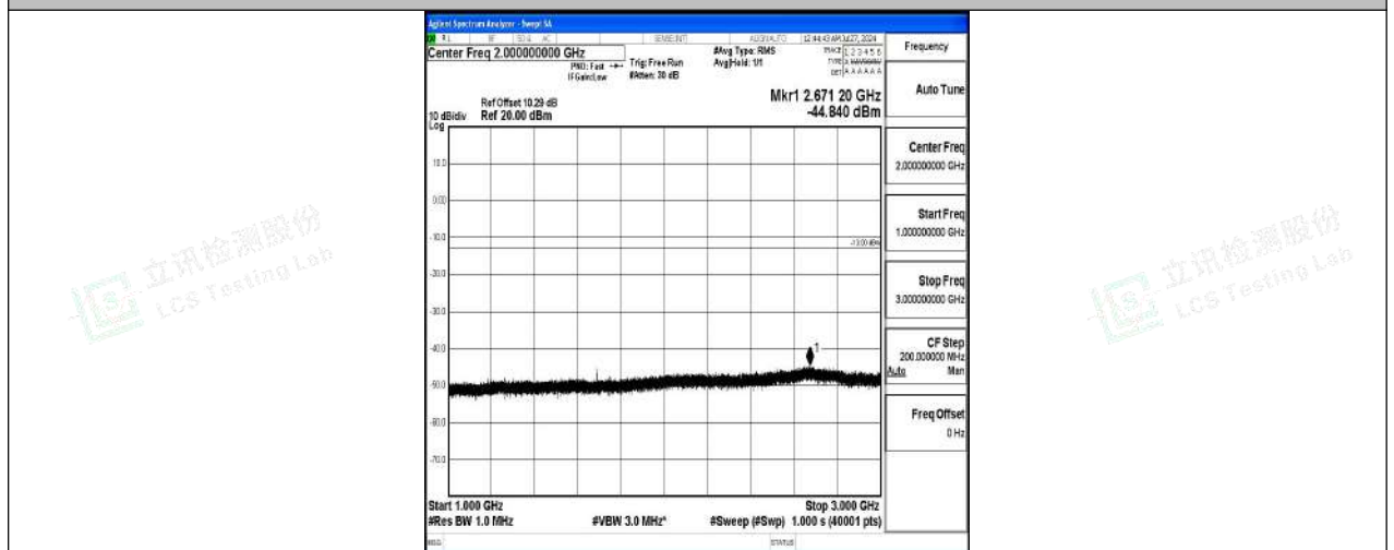
Band5-5MHz-16QAM-20625-1RB#0-1000~3000-PASS
