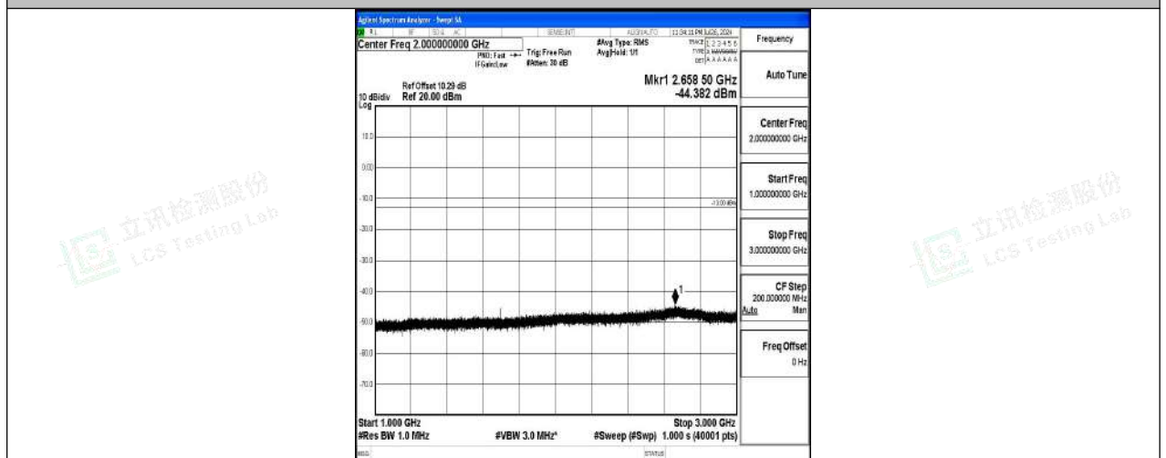
Band5-1.4MHz-16QAM-20643-1RB#0-1000~3000-PASS
