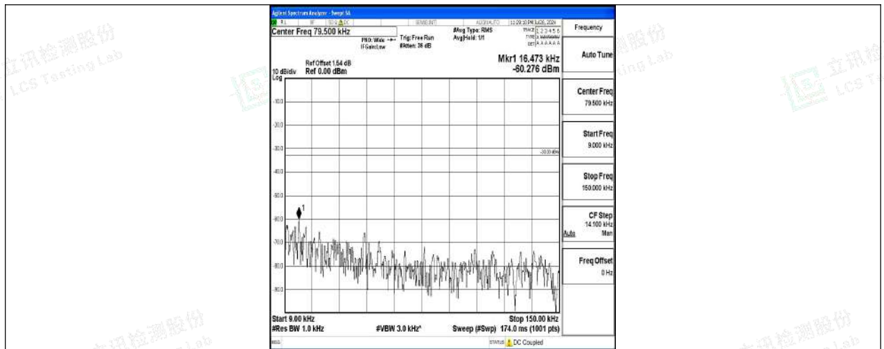
Band5-1.4MHz-16QAM-20407-1RB#0-0.009~0.15-PASS
