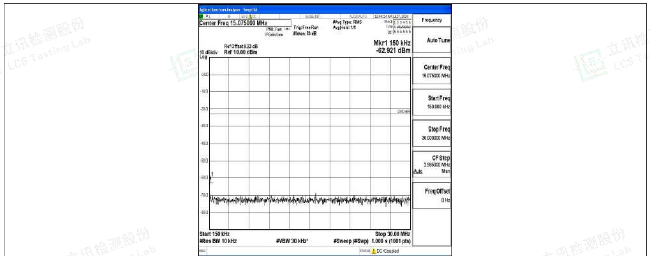
Band5-5MHz-16QAM-20625-1RB#0-0.15~30-PASS
