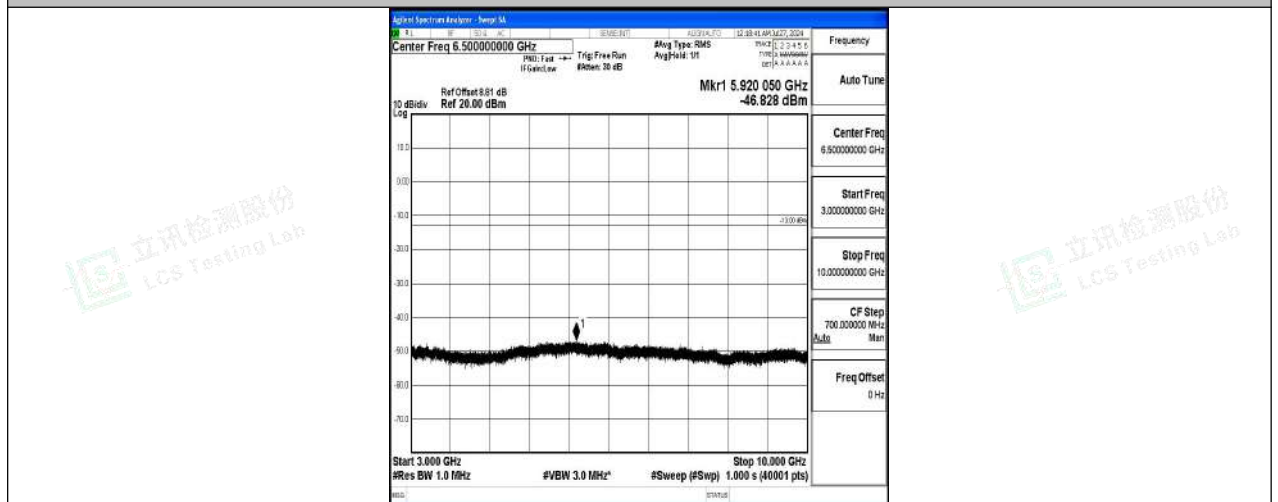
Band5-3MHz-QPSK-20415-1RB#0-3000~10000-PASS
