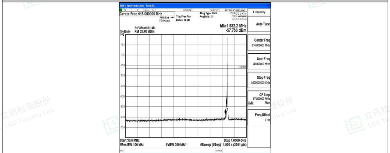
Band5-5MHz-16QAM-20625-1RB#0-30~1000-PASS
