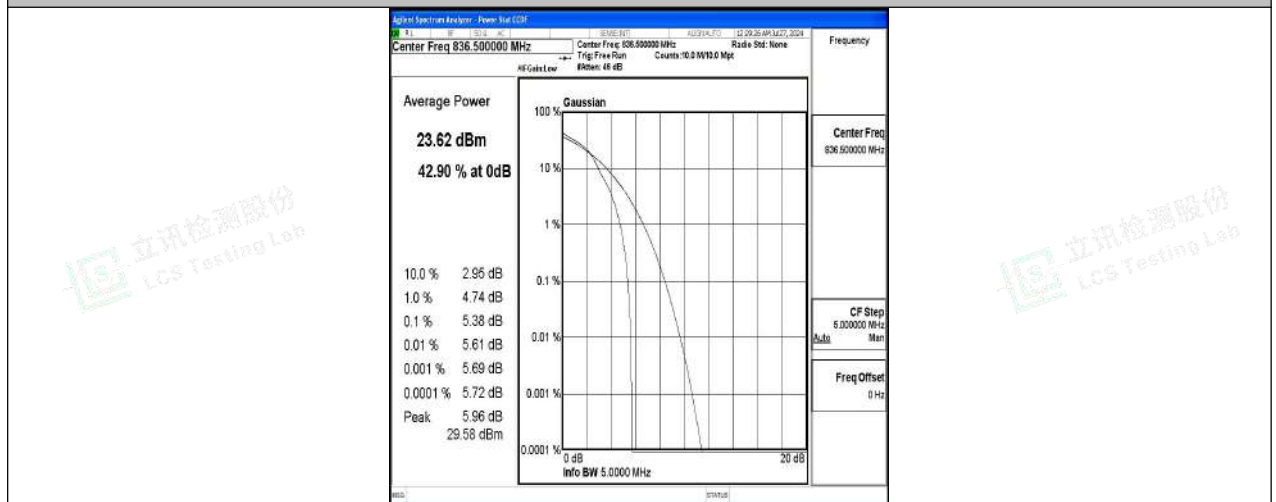
Band5-3MHz-16QAM-20525-1RB#0-PASS
