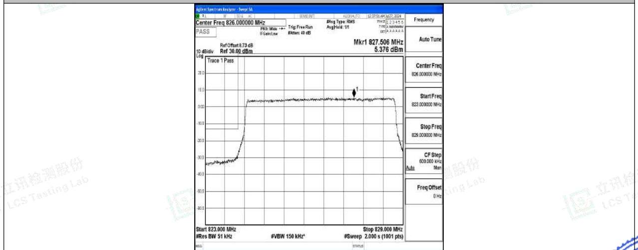
Band5-5MHz-QPSK-20425-25RB#0-PASS
