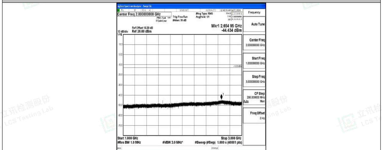
Band5-5MHz-16QAM-20525-1RB#0-1000~3000-PASS
