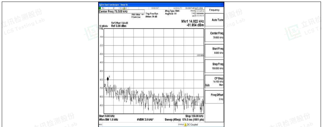
Band5-10MHz-QPSK-20600-1RB#0-0.009~0.15-PASS
