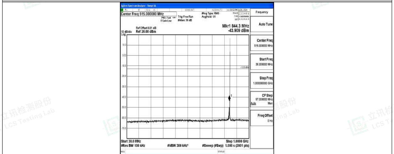
Band5-1.4MHz-16QAM-20643-1RB#0-30~1000-PASS
