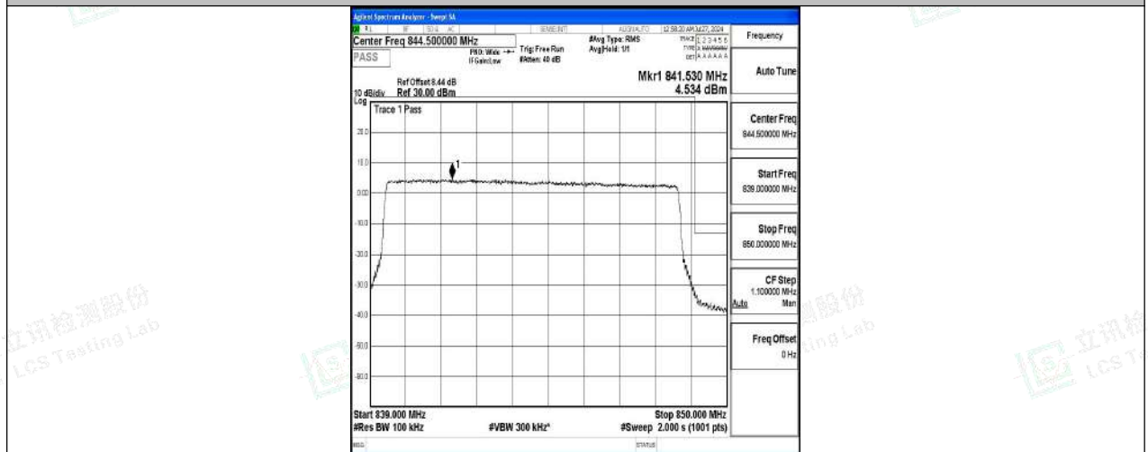
Band5-10MHz-QPSK-20600-50RB#0-PASS
