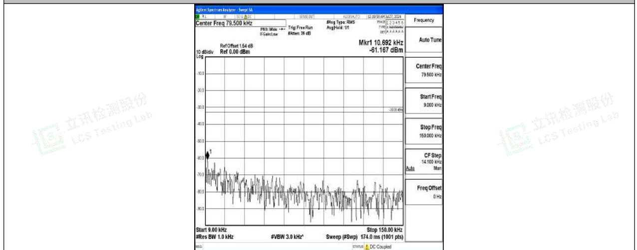
Band5-3MHz-QPSK-20525-1RB#0-0.009~0.15-PASS
