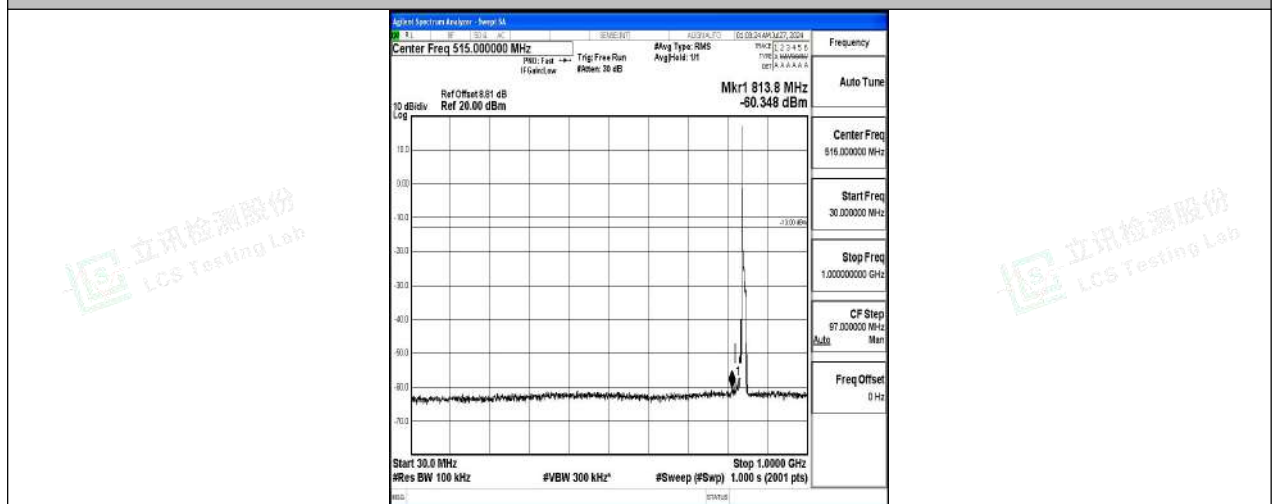
Band5-10MHz-QPSK-20600-1RB#0-30~1000-PASS
