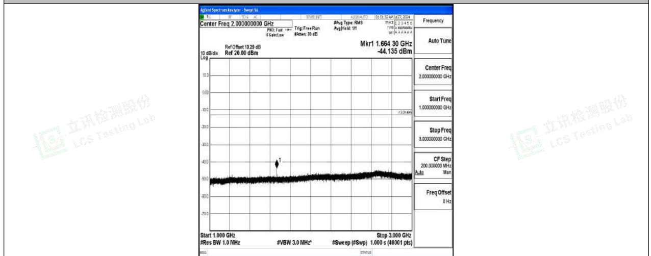
Band5-10MHz-QPSK-20525-1RB#0-1000~3000-PASS
