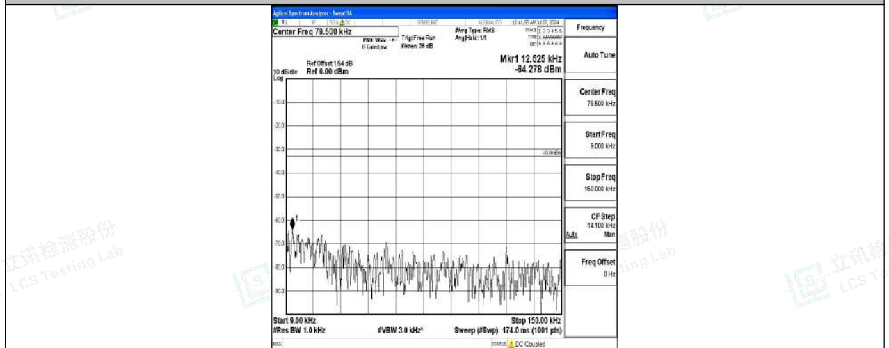
Band5-5MHz-16QAM-20525-1RB#0-0.009~0.15-PASS
