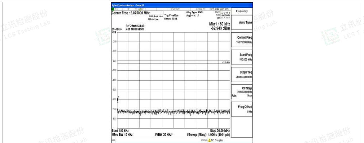
Band5-1.4MHz-16QAM-20643-1RB#0-0.15~30-PASS
