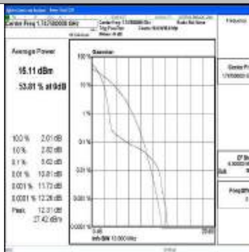
Band4-15MHz-QPSK-20325-1RB#0-PASS
