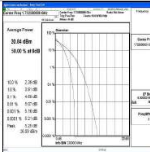
Band4-1.4MHz-QPSK-20175-1RB#0-PASS
