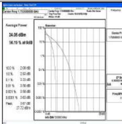
Band4-3MHz-QPSK-20385-1RB#0-PASS
