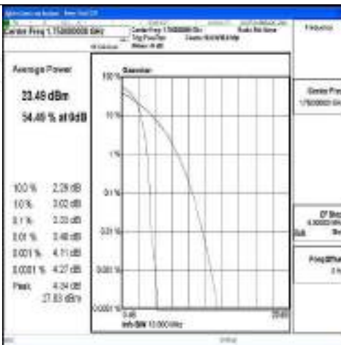
Band4-10MHz-16QAM-20350-1RB#0-PASS
