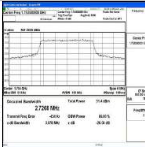
Band4-3MHz-QPSK-20385-15RB#0-PASS
