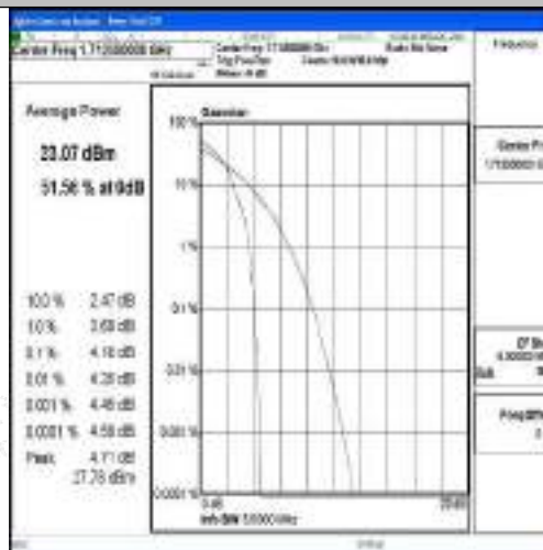
Band4-5MHz-16QAM-19975-1RB#0-PASS
