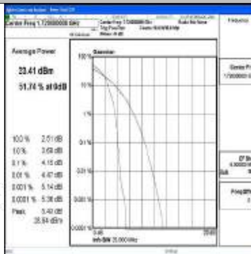
Band4-20MHz-16QAM-20050-1RB#0-PASS
