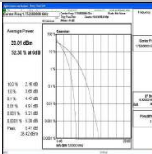
Band4-5MHz-QPSK-20375-25RB#0-PASS
