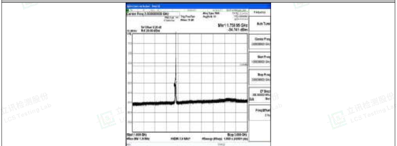
Band4-5MHz-16QAM-20375-1RB#0-1000~3000-PASS
