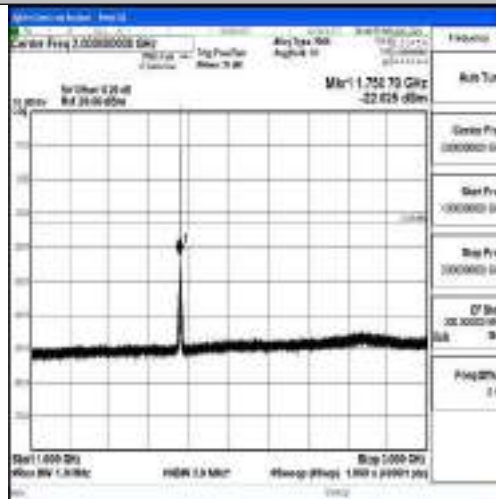
Band4-1.4MHz-QPSK-20393-1RB#0-1000~3000-PASS
