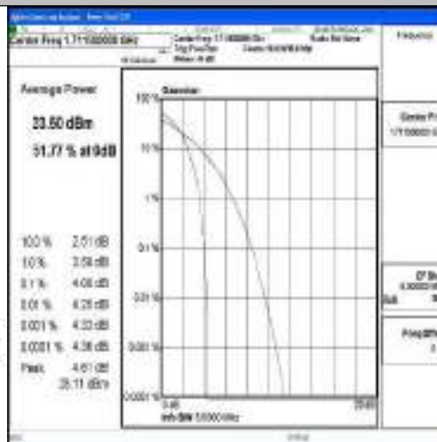
Band4-3MHz-16QAM-19965-1RB#0-PASS
