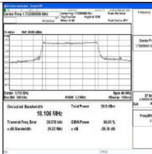
Band4-20MHz-16QAM-20175-100RB#0-PASS
