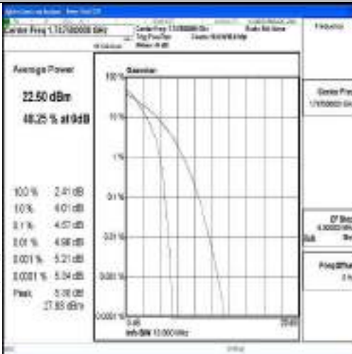
Band4-15MHz-QPSK-20325-75RB#0-PASS
