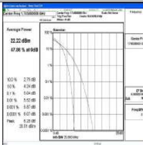
Band4-20MHz-16QAM-20300-100RB#0-PASS
