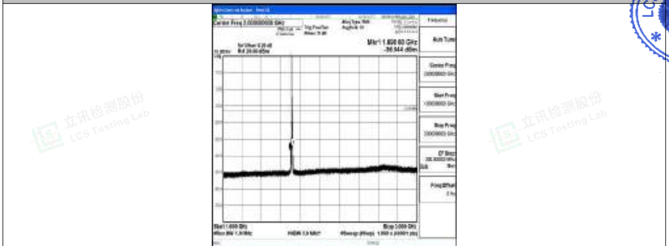
Band4-5MHz-16QAM-19975-1RB#0-1000~3000-PASS
