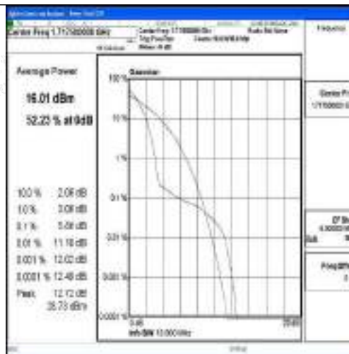
Band4-15MHz-QPSK-20025-1RB#0-PASS
