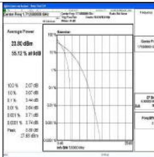
Band4-5MHz-QPSK-19975-1RB#0-PASS
