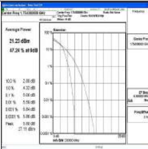
Band4-1.4MHz-16QAM-20393-6RB#0-PASS
