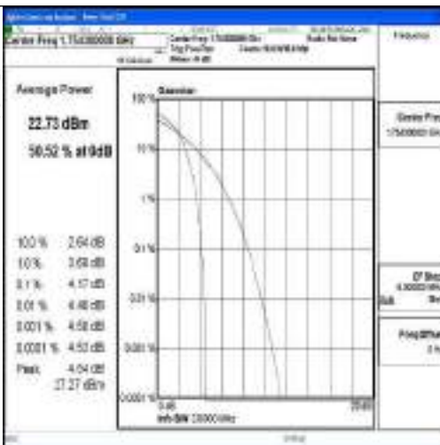
Band4-1.4MHz-16QAM-20393-1RB#0-PASS
