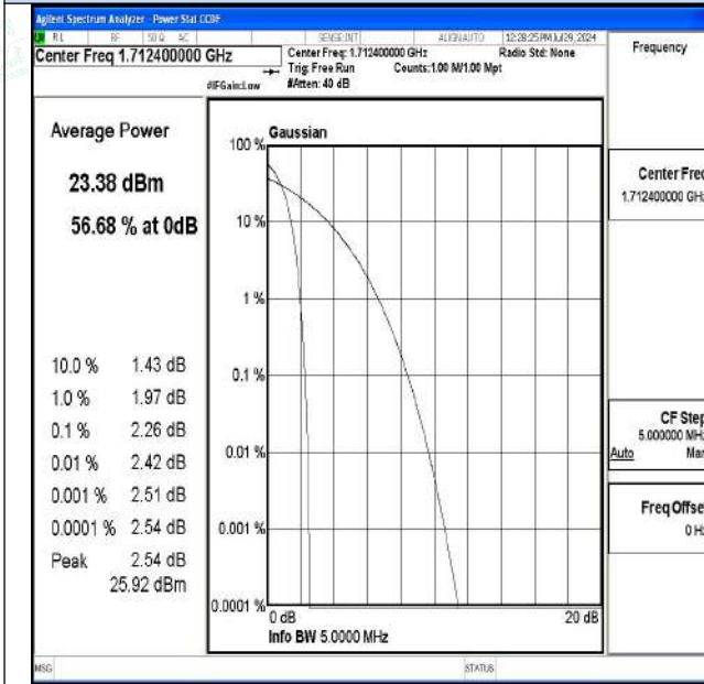
Channel 1312 / 1712.4 MHz
