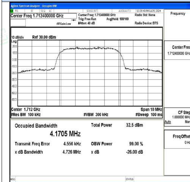
Channel 1312 / 1712.4 MHz
