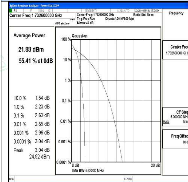
Channel 1413 / 1732.6 MHz
