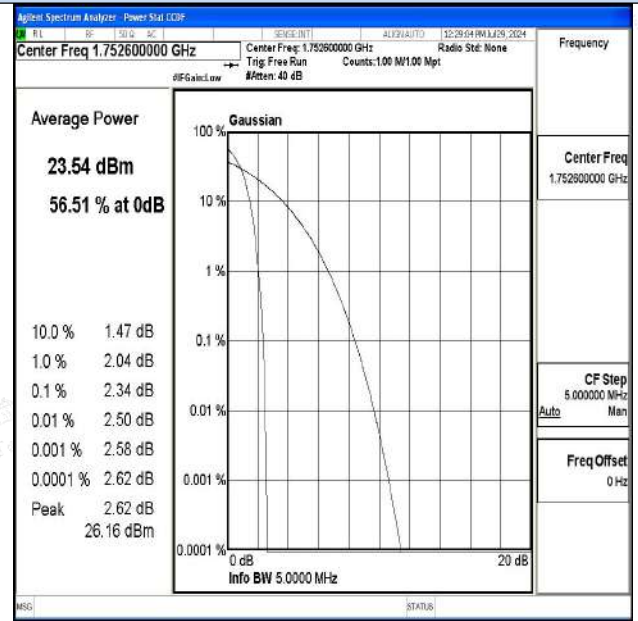
Channel 1513 / 1752.6 MHz
