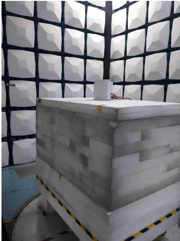
Radiated Emission 60-90GHz View
