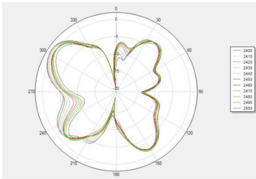
Phi 90 2D
