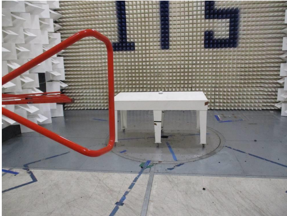
Figure 0-19 Radiated Emissions Test Setup Charging Mode Front 30 MHz-1 GHz
