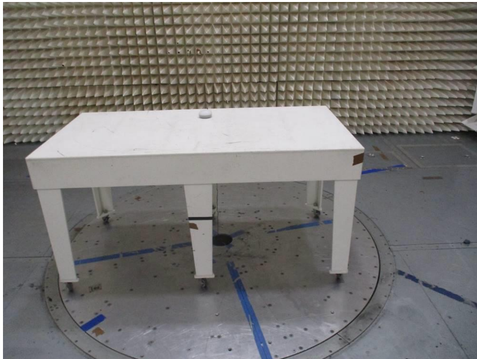
Figure 0-20 Radiated Emissions Test Setup Charging Mode 30 MHz-1 GHz
