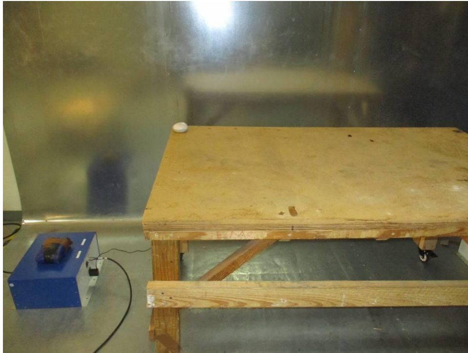
Figure 0-23 Conducted Emissions Test Setup Charging Mode
