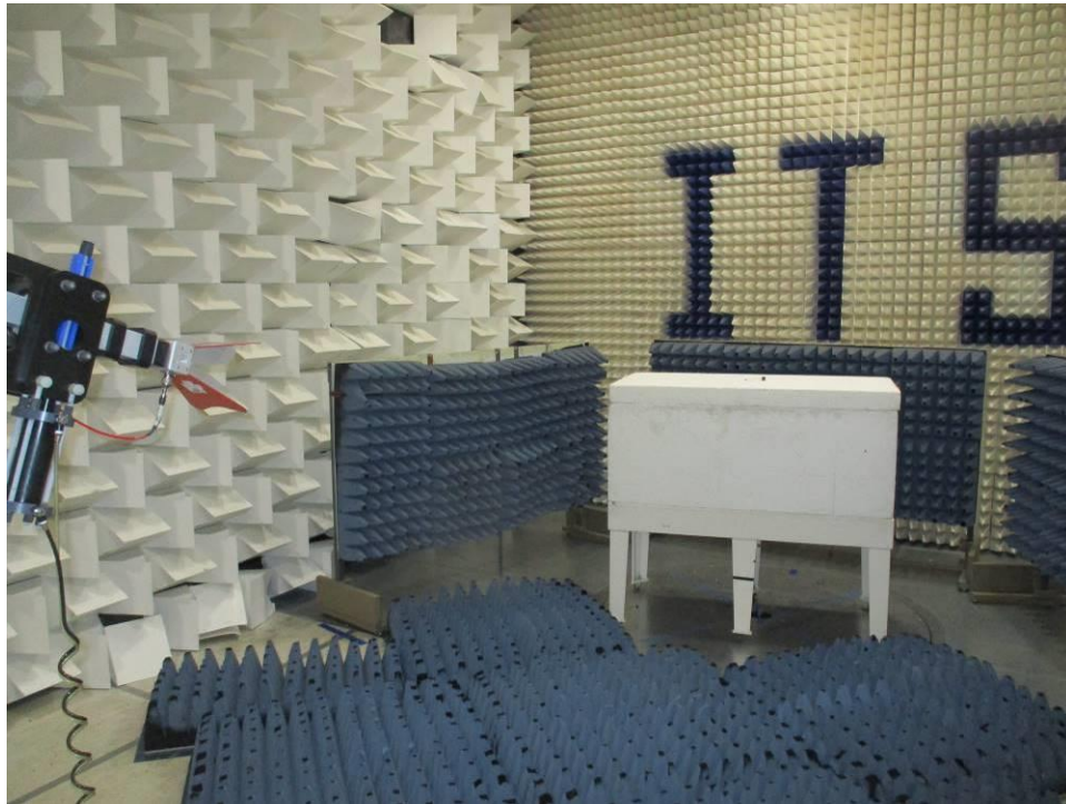
Figure 0-1 Band Edge Earpiece Battery Mode Test Setup
