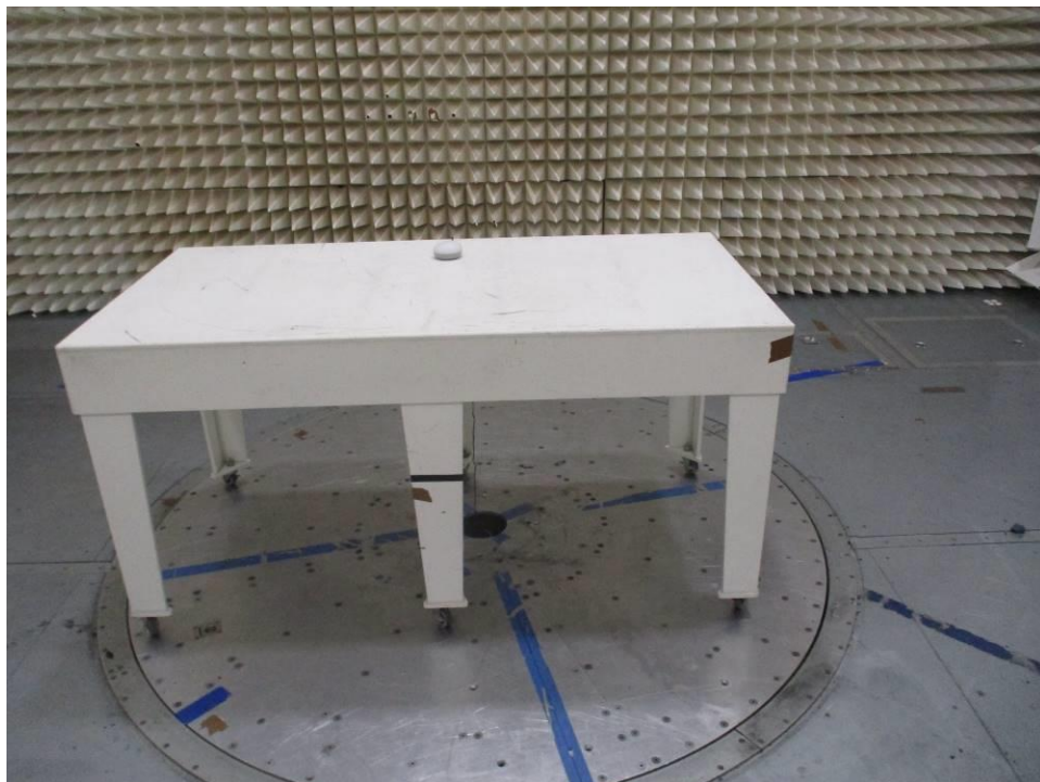
Figure 0-6 Radiated Spurious Emissions Test Setup Charging Mode 30 MHz-1 GHz
