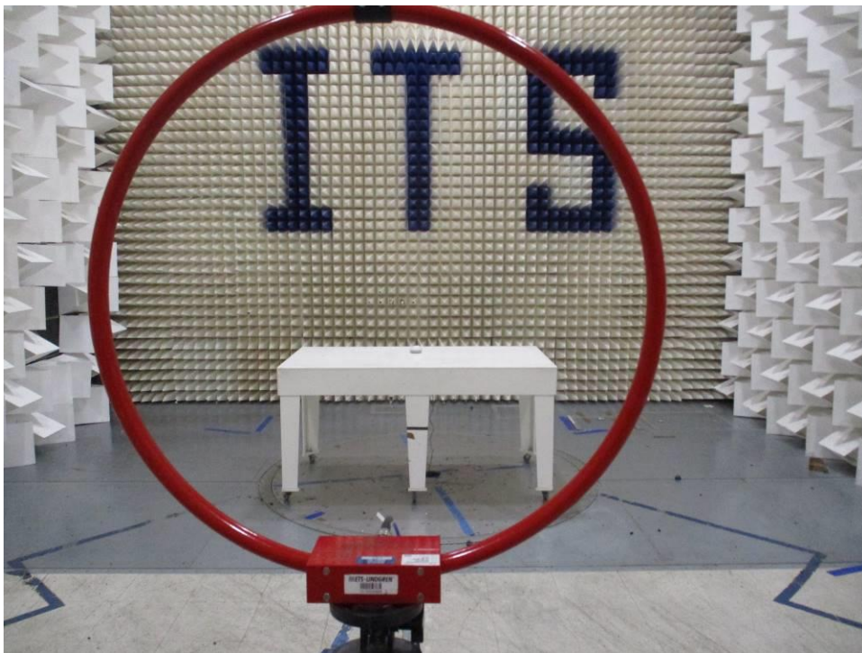
Figure 0-10 Radiated Spurious Emissions Test Setup Charging Mode 9 kHz – 30 MHz
