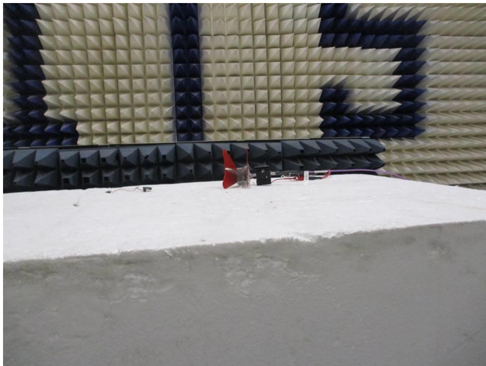
Figure 0-14 Radiated Spurious Emissions Test Setup Earpiece Battery Mode Above 18 GHz
