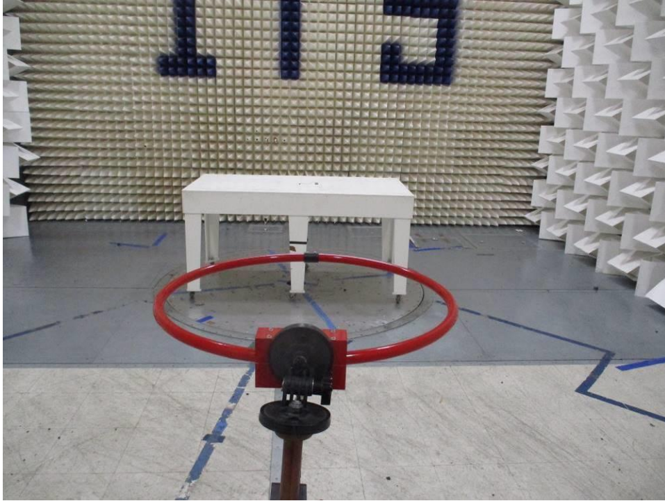
Figure 0-9 Radiated Spurious Emissions Test Setup Earpiece Battery Mode 9 kHz – 30 MHz Z Axis
