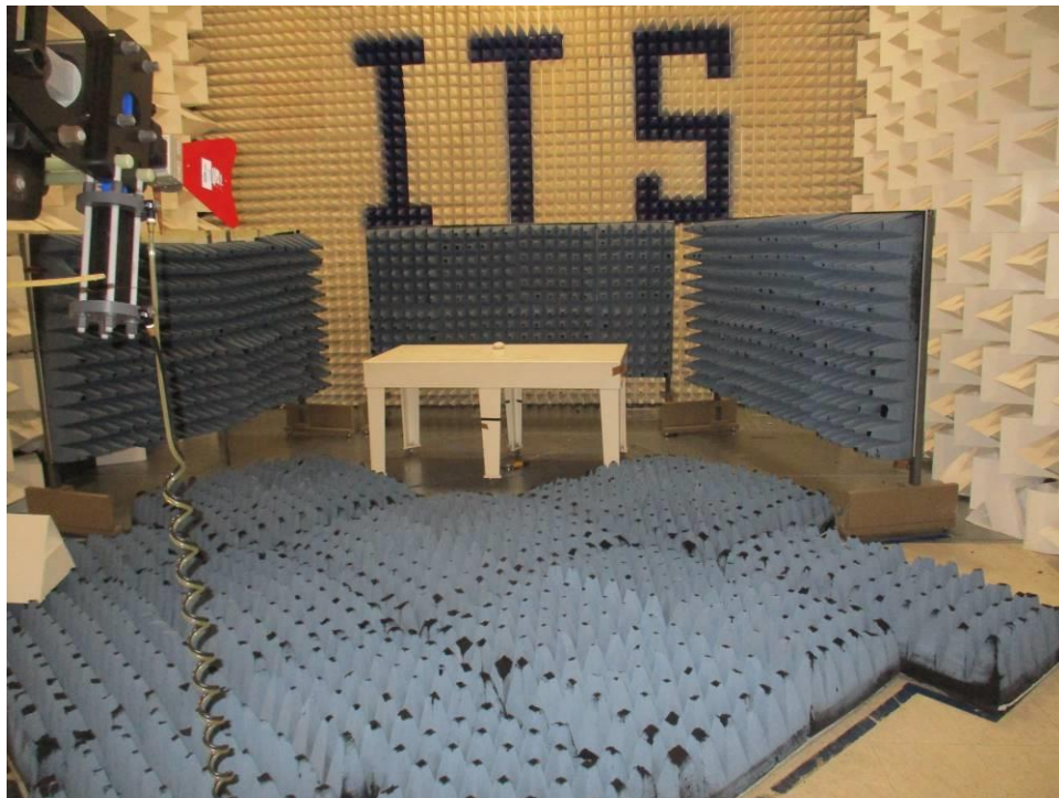
Figure 0-22 Radiated Emissions Test Setup Charging Mode 1 GHz- 18 GHz
