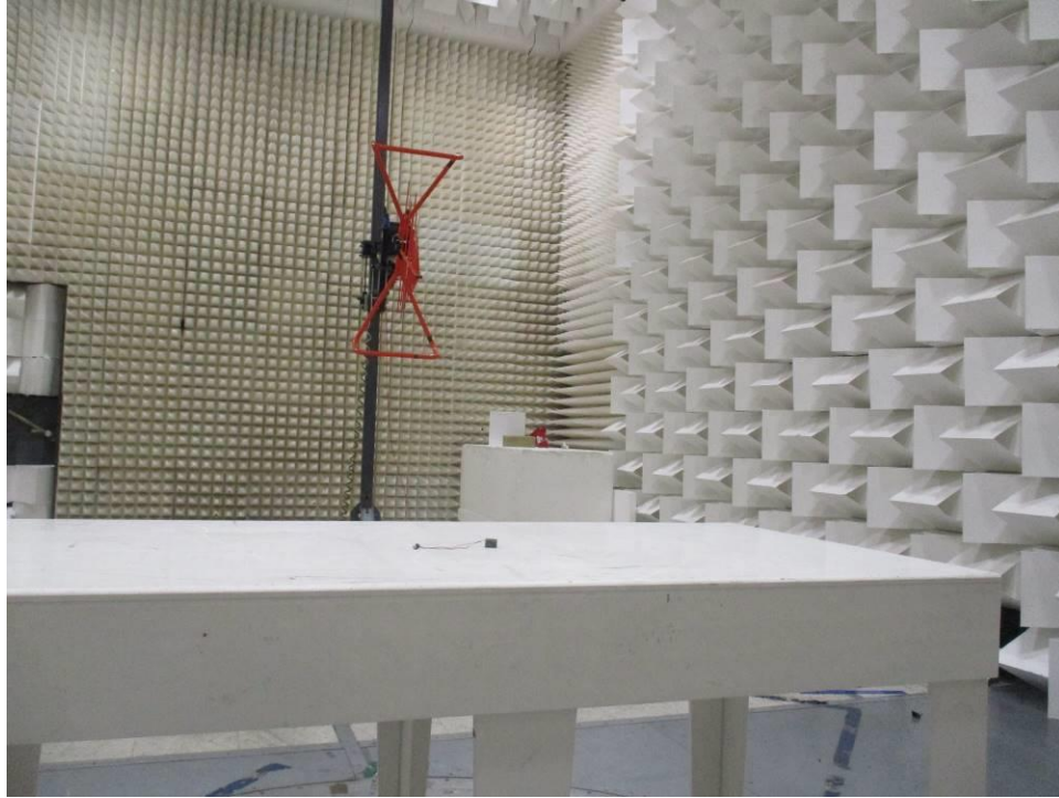
Figure 0-17 Radiated Emissions Test Setup Earpiece Battery Mode 30 MHz-1 GHz
