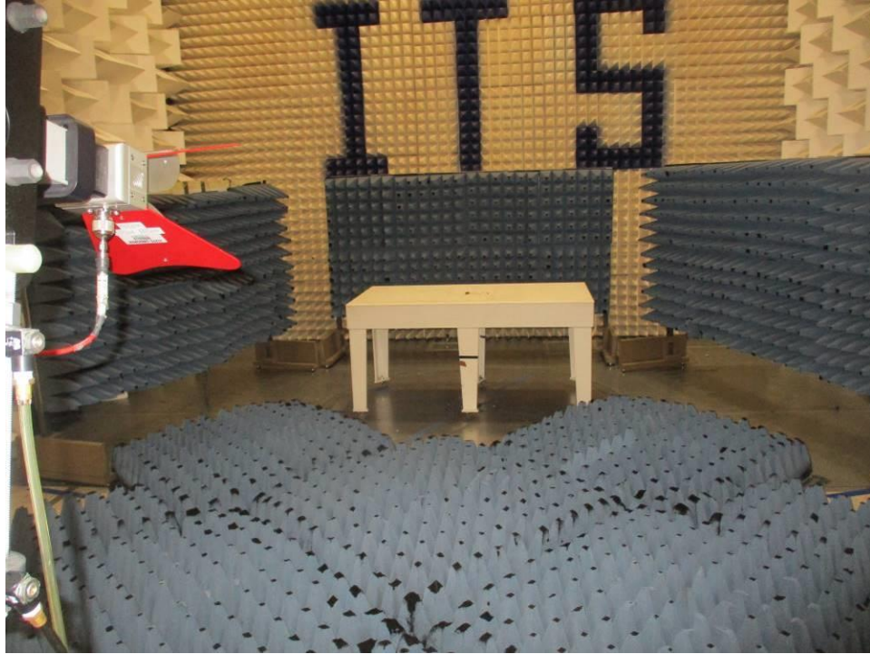
Figure 0-21 Radiated Emissions Test Setup Earpiece Battery Mode 1 GHz- 18 GHz
