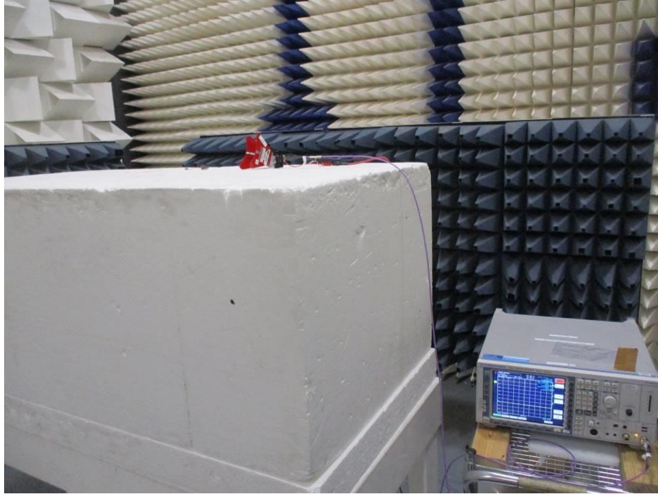
Figure 0Error! No text of specified style in document.-13 Radiated Spurious Emissions Test Setup Earpiece Battery Mode Above 18 GHz
