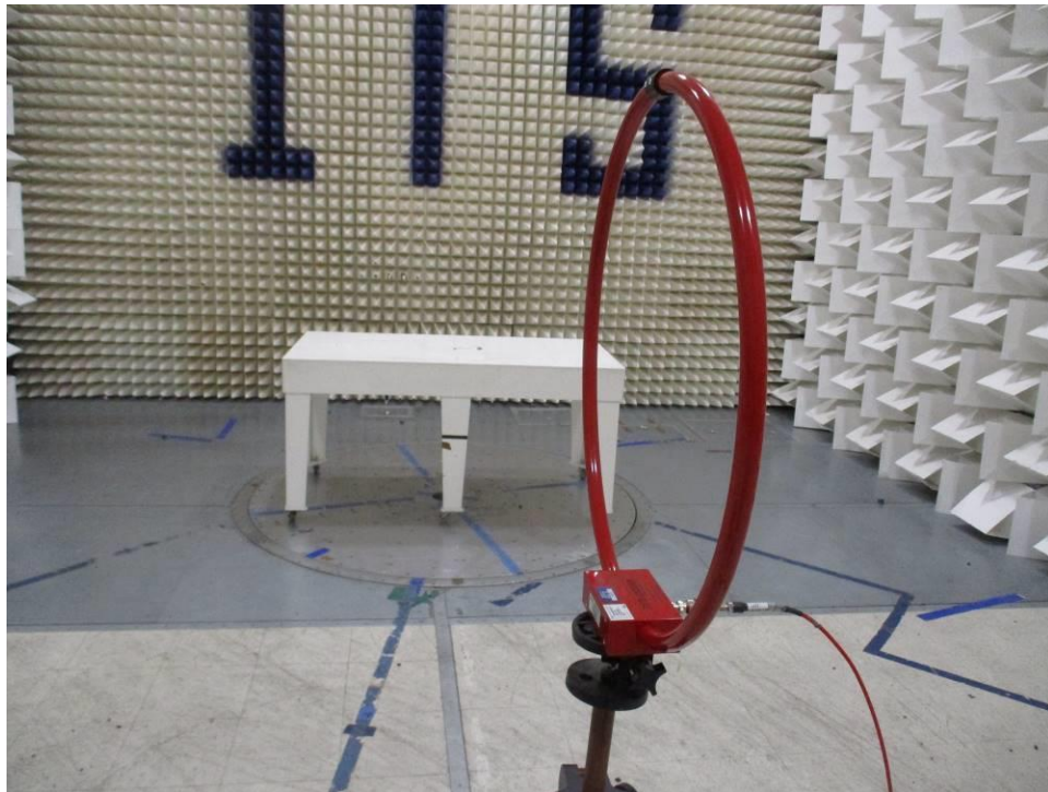
Figure 0-8 Radiated Spurious Emissions Test Setup Earpiece Battery Mode 9 kHz – 30 MHz Y Axis
