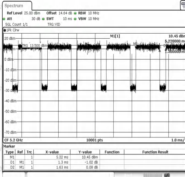
NTNV-11N20SISO-Ant1-5200
