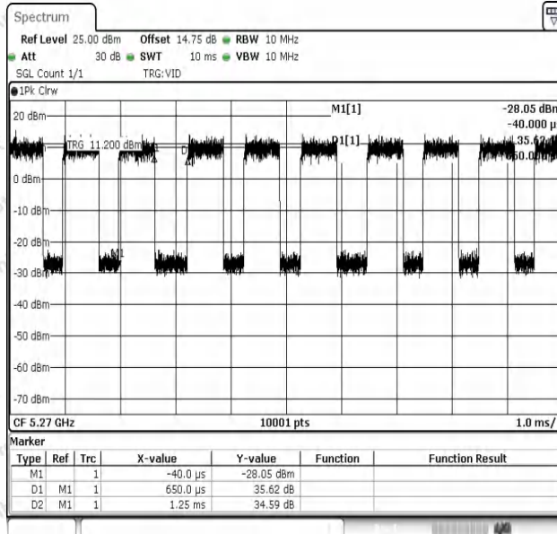
NTNV-11AC40SISO-Ant1-5270
