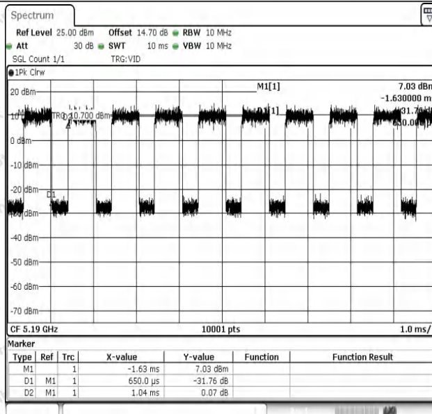
NTNV-11AC40SISO-Ant1-5190
