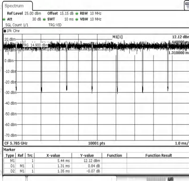
NTNV-11AC20SISO-Ant1-5785
