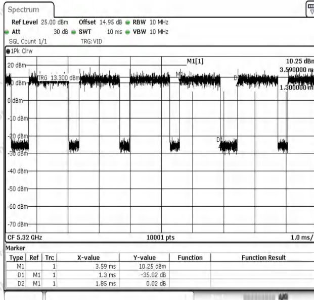
NTNV-11N20SISO-Ant1-5320
