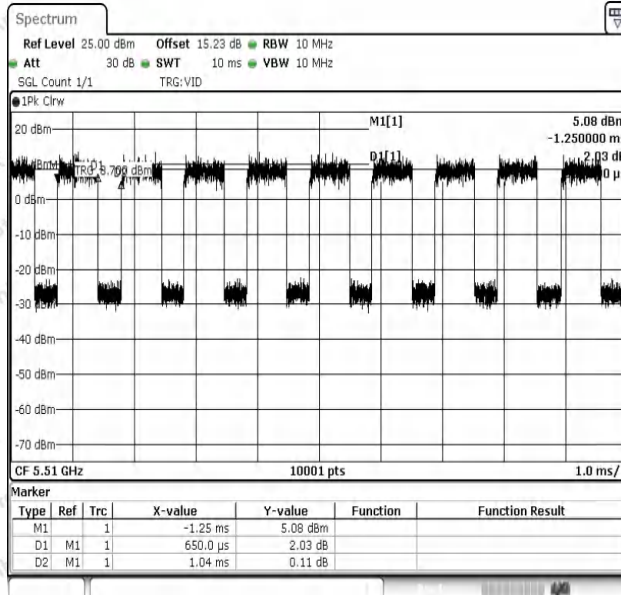
NTNV-11AC40SISO-Ant1-5510
