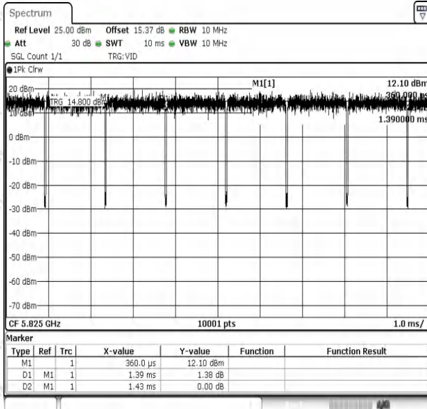
NTNV-11A-Ant1-5825
