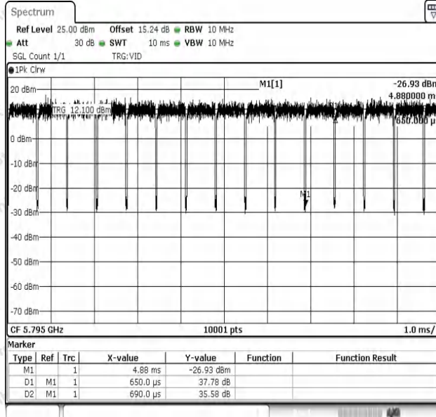
NTNV-11AC40SISO-Ant1-5795
