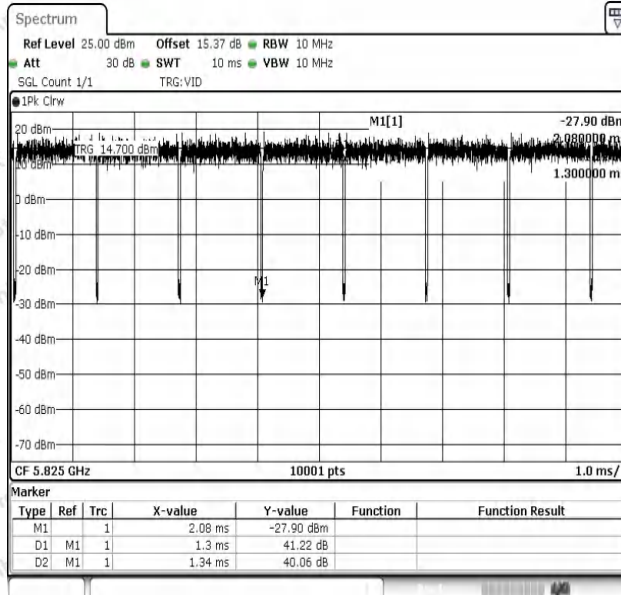
NTNV-11N20SISO-Ant1-5825
