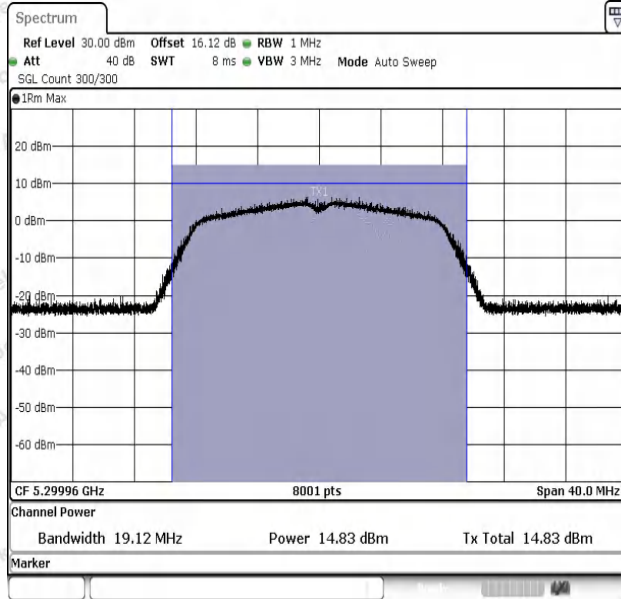
11A-Ant1-5300-PASS
