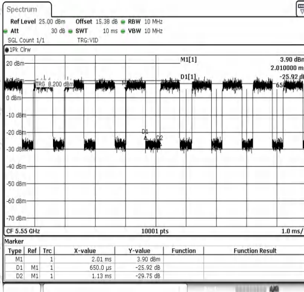
NTNV-11N40SISO-Ant1-5550
