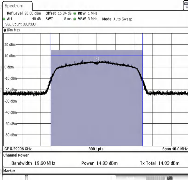
11AC20SISO-Ant1-5300-PASS
