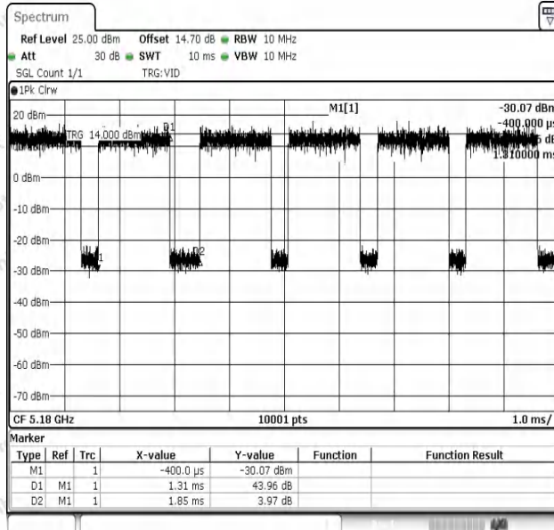
NTNV-11AC20SISO-Ant1-5180
