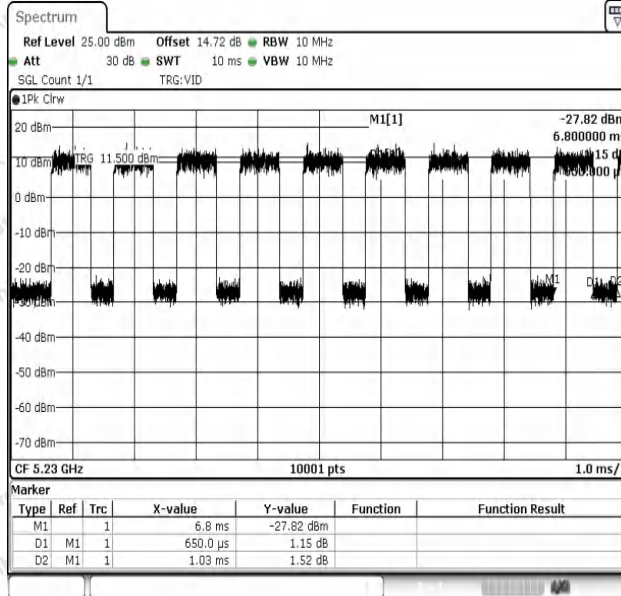
NTNV-11N40SISO-Ant1-5230
