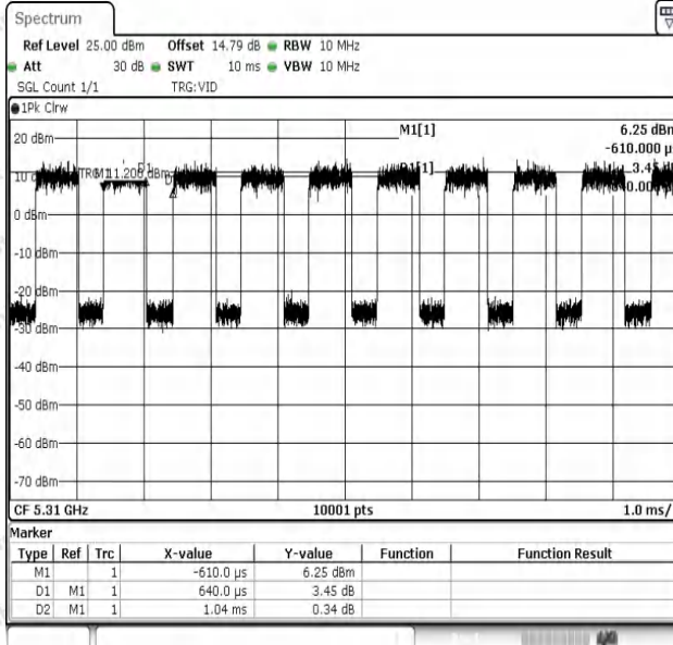
NTNV-11N40SISO-Ant1-5310
