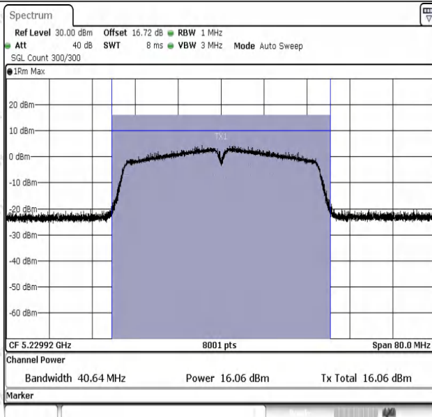
11N40SISO-Ant1-5230-PASS
