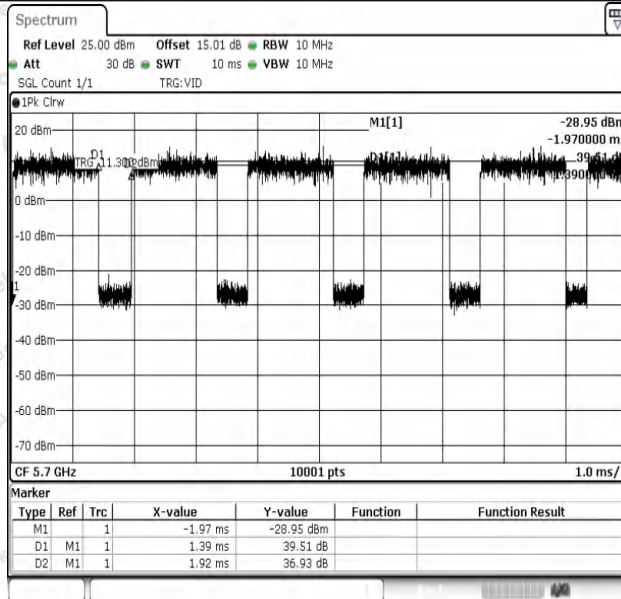
NTNV-11A-Ant1-5700
