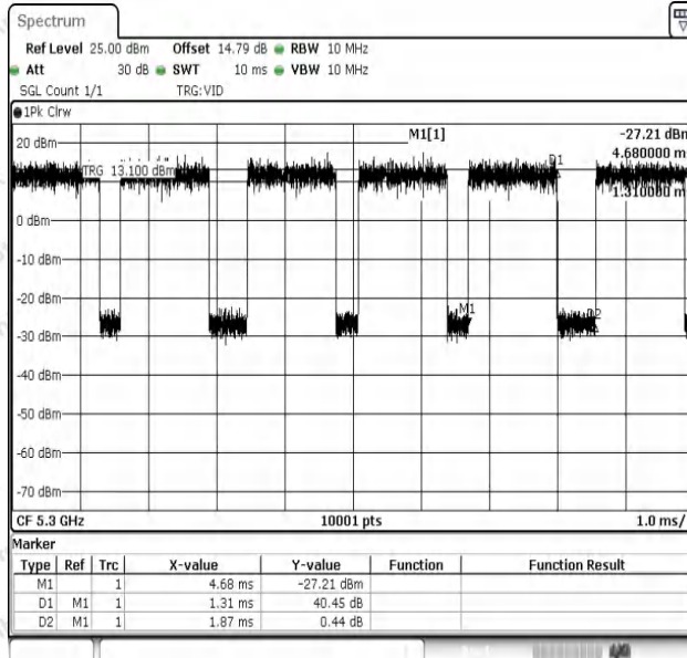
NTNV-11AC20SISO-Ant1-5300
