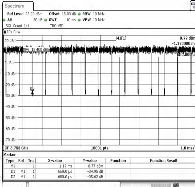
NTNV-11N40SISO-Ant1-5755
