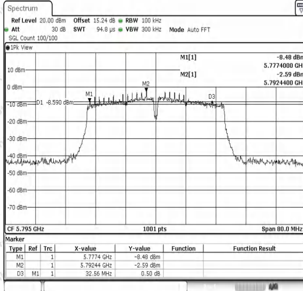
11N40SISO-Ant1-5795-PASS
