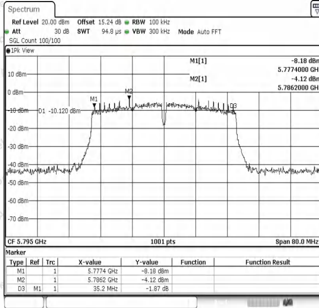
11AC40SISO-Ant1-5795-PASS
