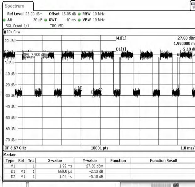
NTNV-11AC40SISO-Ant1-5670
