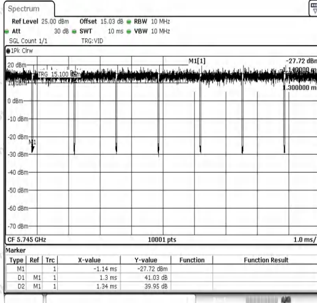
NTNV-11N20SISO-Ant1-5745
