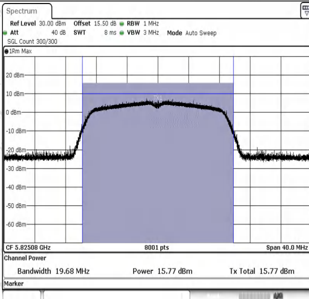
11N20SISO-Ant1-5825-PASS
