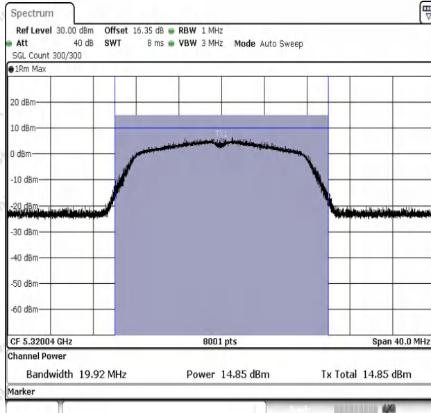
11A-Ant1-5320-PASS
