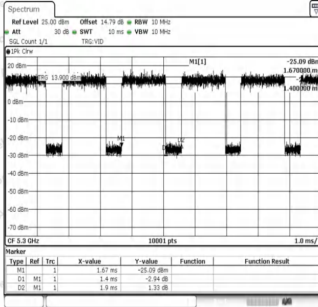
NTNV-11A-Ant1-5300
