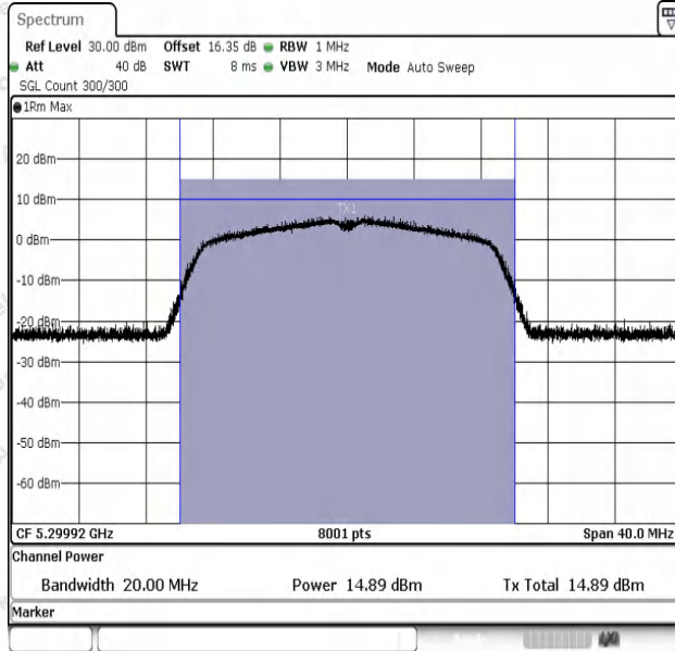
11N20SISO-Ant1-5300-PASS
