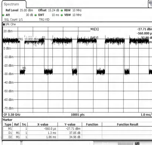
NTNV-11N20SISO-Ant1-5580
