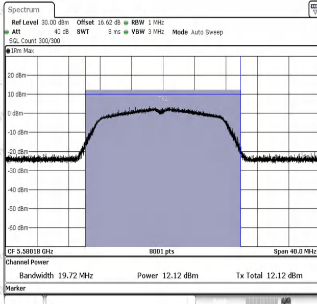
11A-Ant1-5580-PASS
