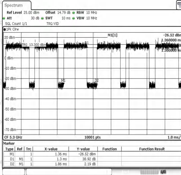
NTNV-11N20SISO-Ant1-5300
