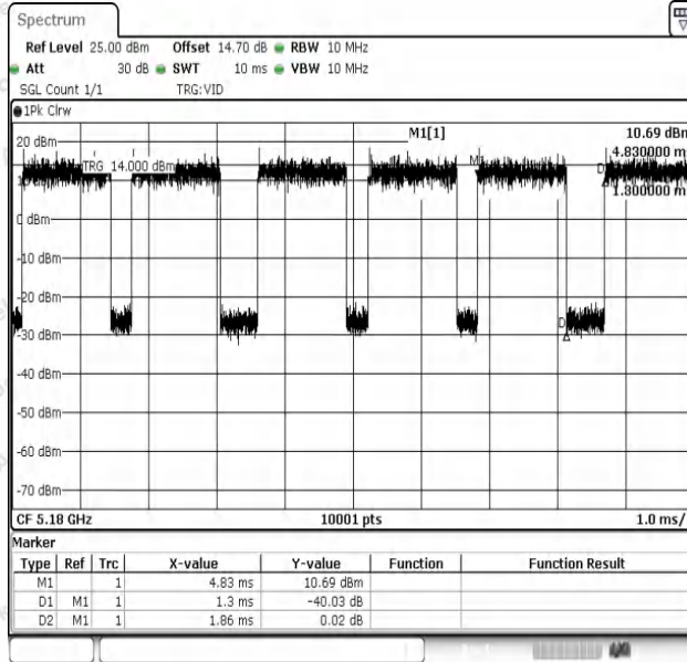
NTNV-11N20SISO-Ant1-5180
