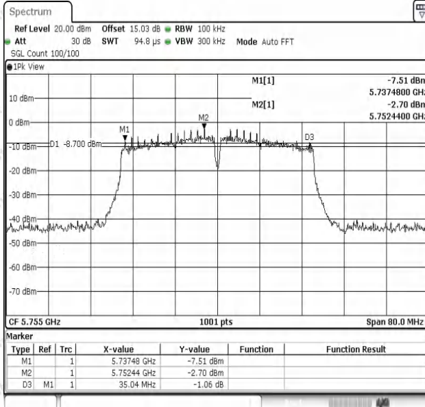
11AC40SISO-Ant1-5755-PASS
