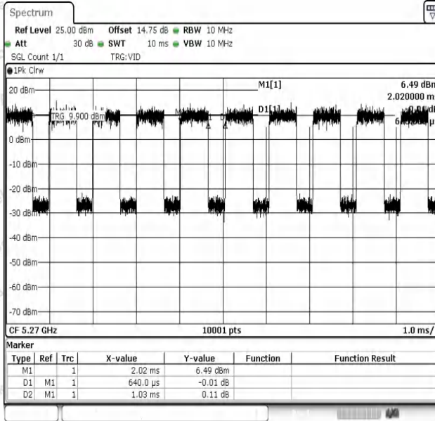
NTNV-11N40SISO-Ant1-5270
