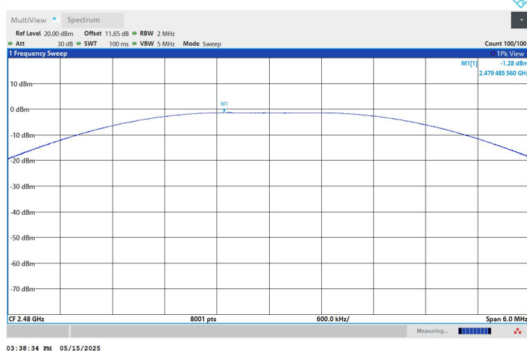
BLE_2M-Ant1-2480-PASS
