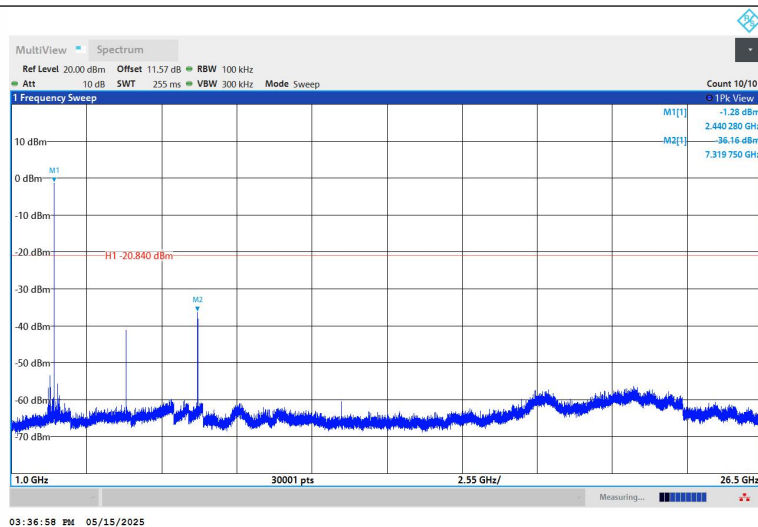
BLE_2M-Ant1-2440-1000~26500-PASS
