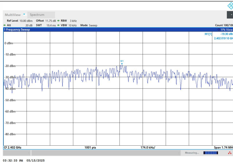
BLE_2M-Ant1-2402-PASS
