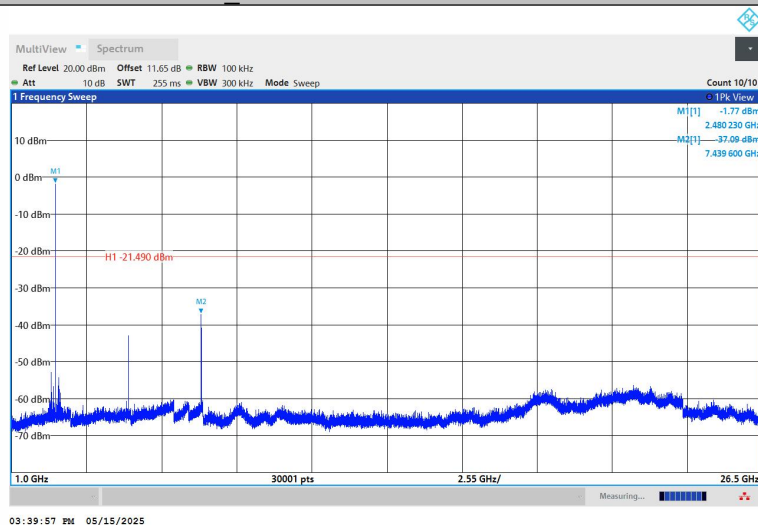
BLE_2M-Ant1-2480-1000~26500-PASS
