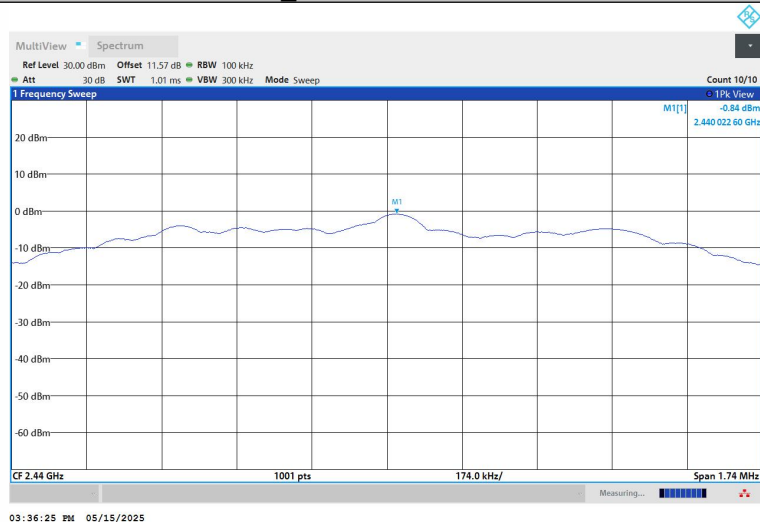
BLE_2M-Ant1-2440-PASS
