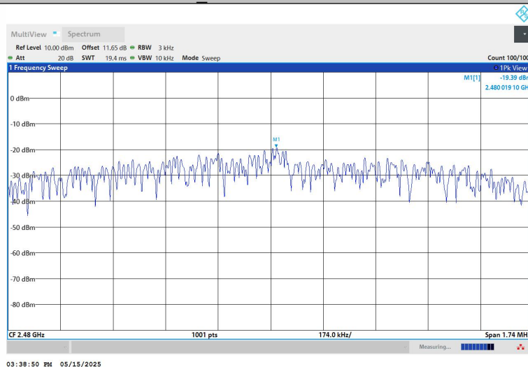
BLE_2M-Ant1-2480-PASS
