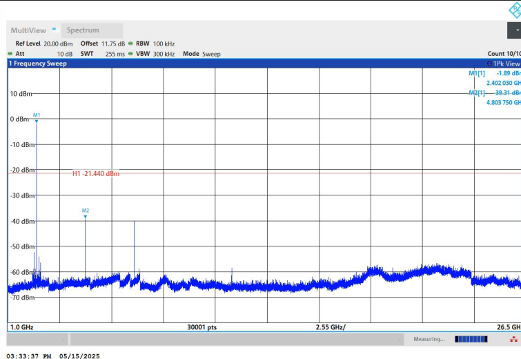
BLE_2M-Ant1-2402-1000~26500-PASS
