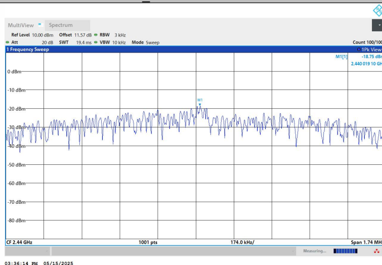
BLE_2M-Ant1-2440-PASS
