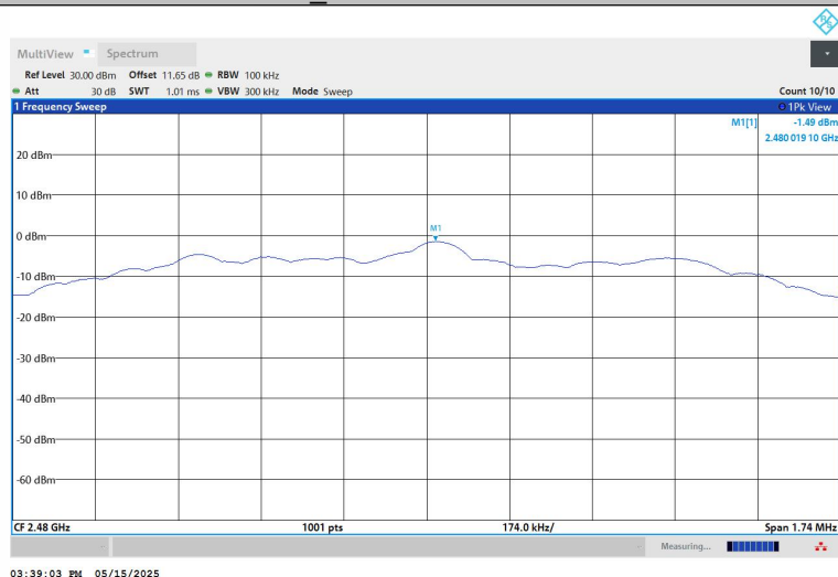
BLE_2M-Ant1-2480-PASS
