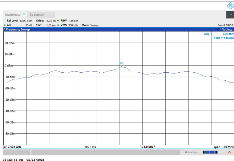
BLE_2M-Ant1-2402-PASS
