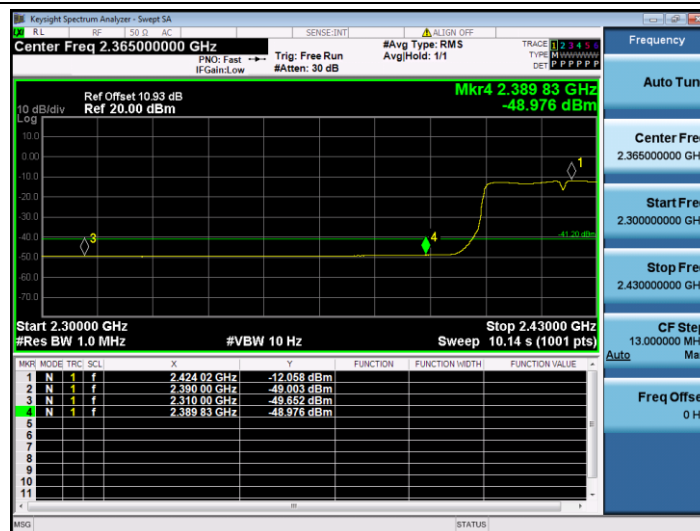
11N40SISO_Ant1_Low_2422_Peak
