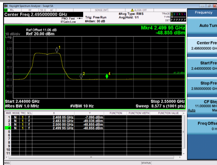
11G_Ant1_High_2462_Peak
