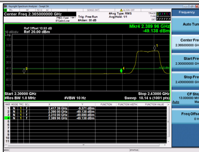
11N20SISO_Ant1_Low_2412_Peak
