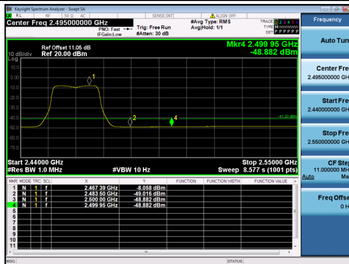
11N20SISO_Ant1_High_2462_Peak
