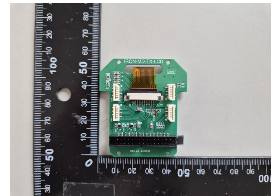
LCD_Rear
