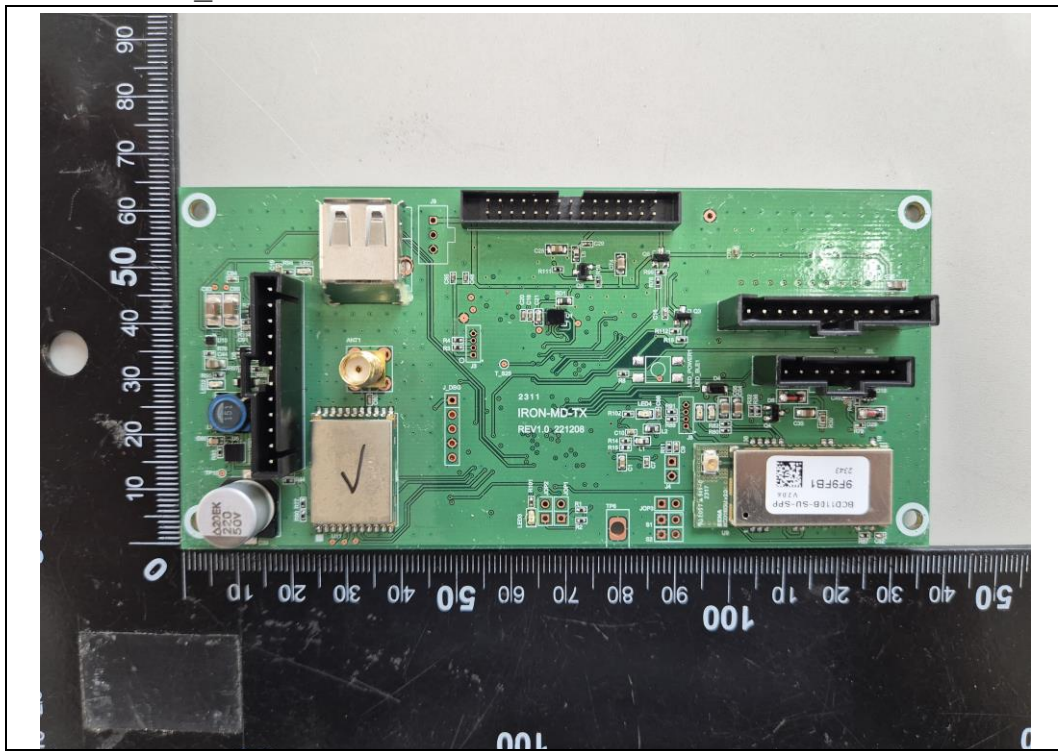
Main Board_Front
