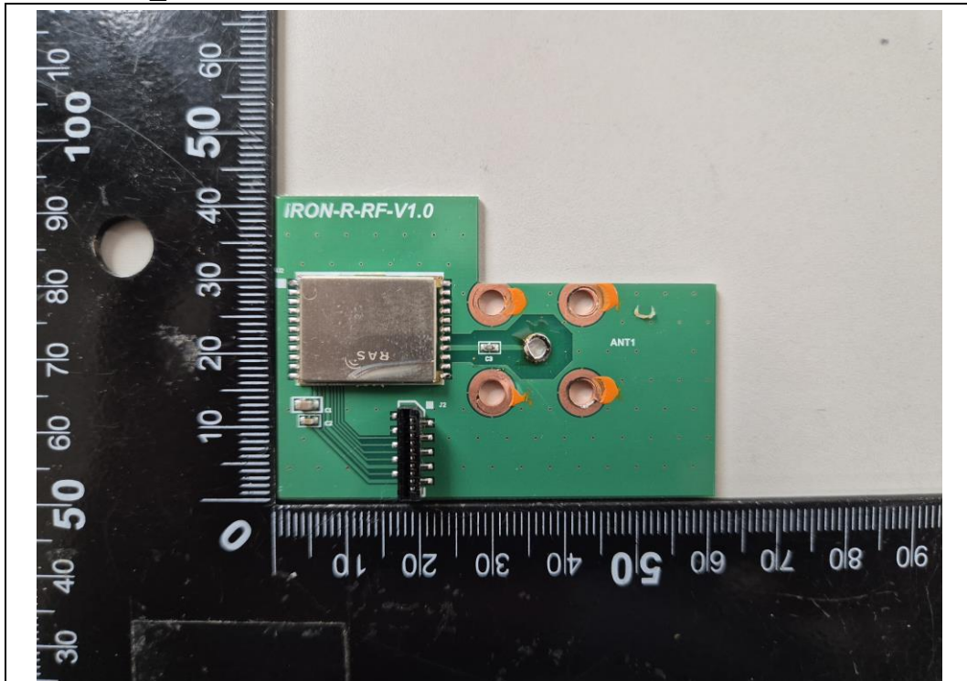
RF Board_Front
