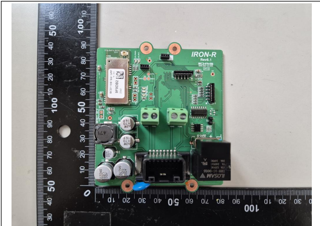
Main Board_Front
