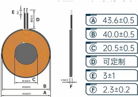
Antenna Top View [With Ruler]
