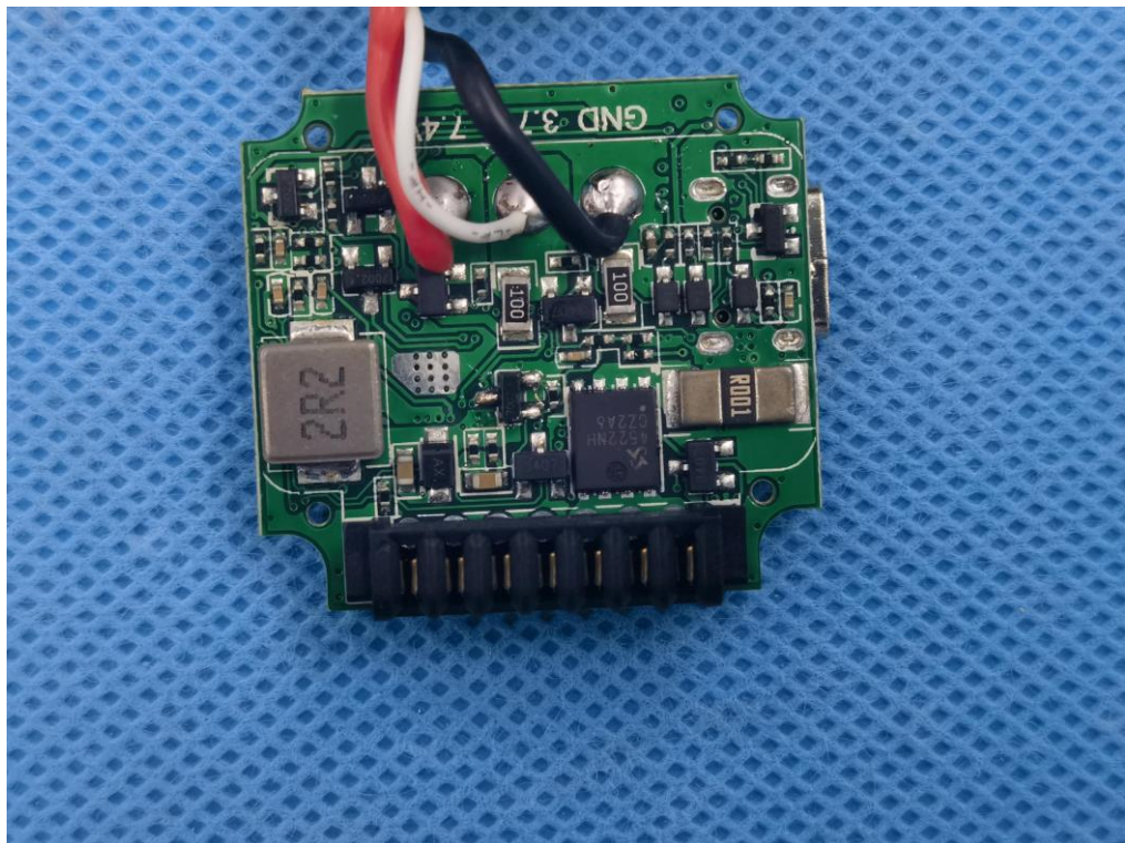
INTERNAL VIEW OF EUT (FIGURE 18)
