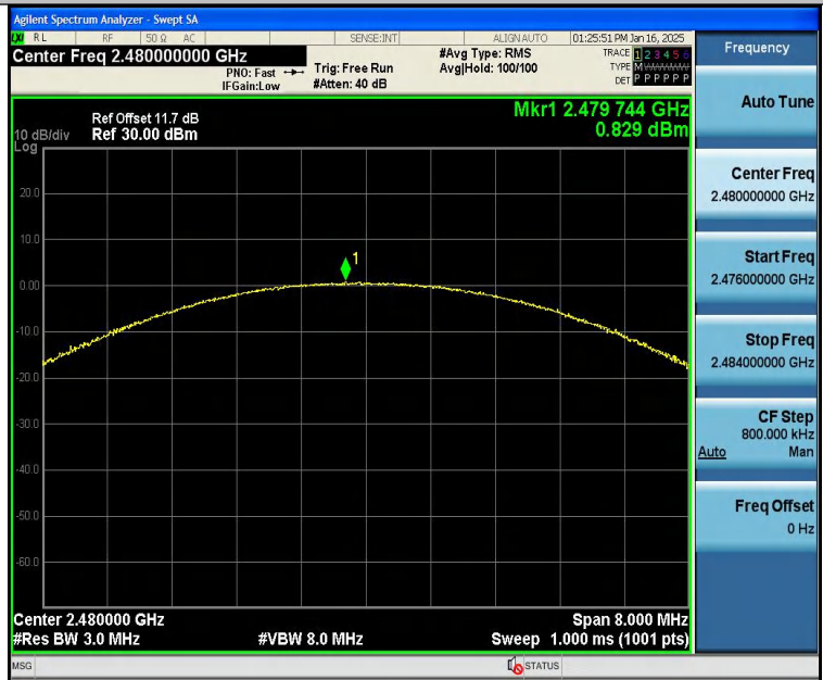
2DH5-Ant1-2480-PASS
