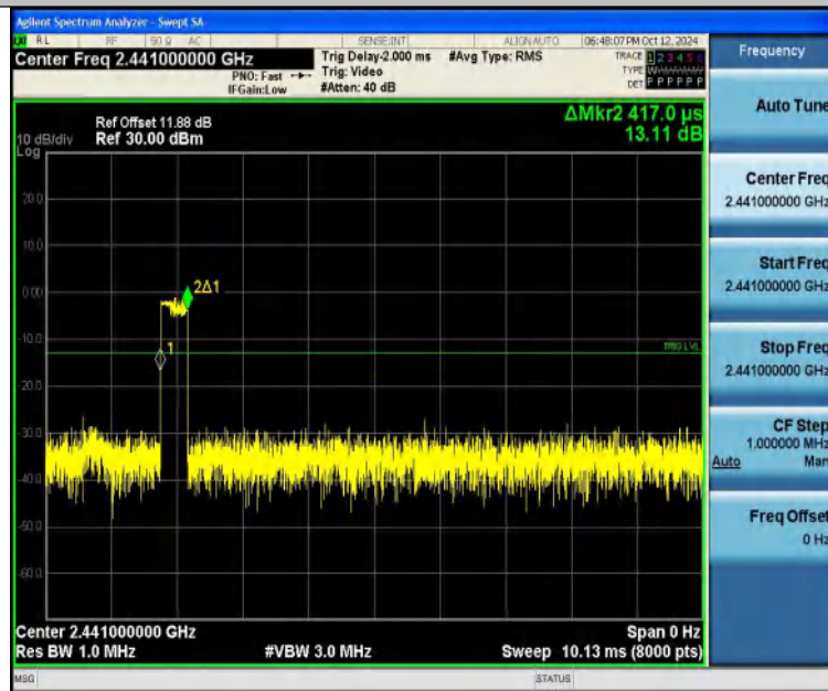
3DH1-Ant1-Hop-PASS
