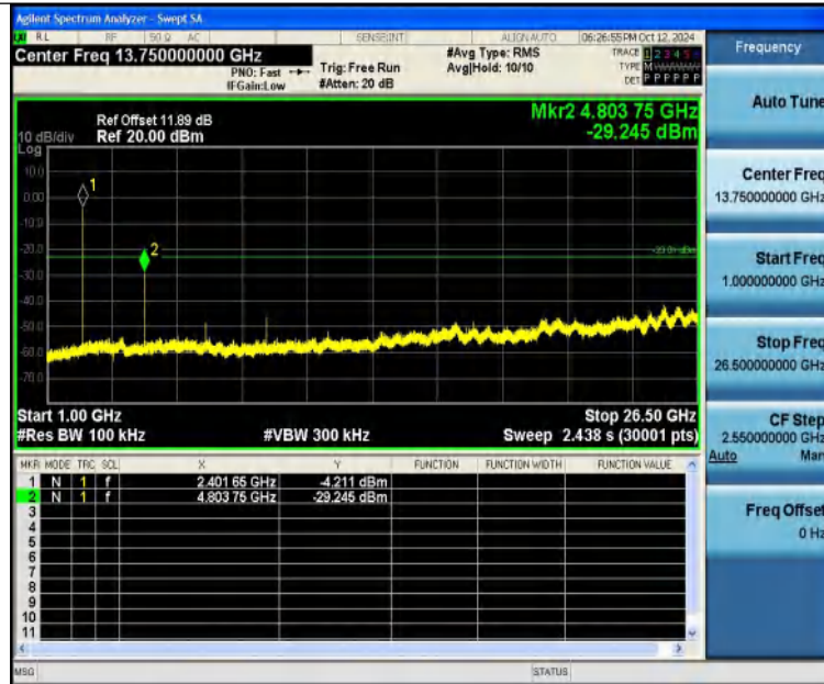
3DH5-Ant1-2402-1000~26500-PASS
