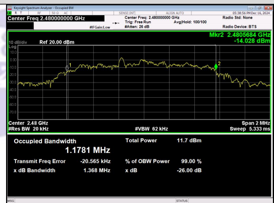
n/4DQPSK_2-DH1_Channel 78
