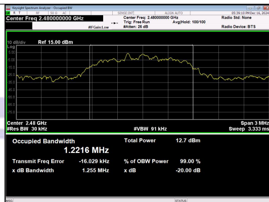
n/4DQPSK_2-DH1_Channel 78
