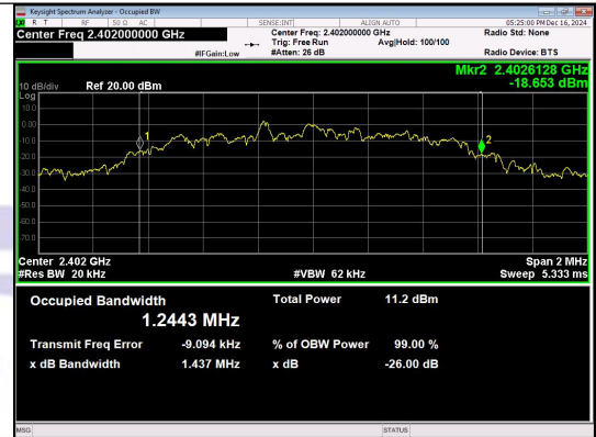
n/4DQPSK_2-DH1_Channel 0
