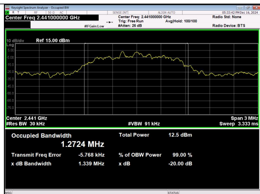
n/4DQPSK_2-DH1_Channel 39
