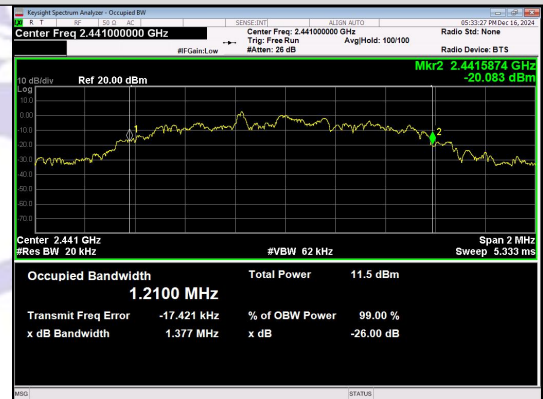
n/4DQPSK_2-DH1_Channel 39
