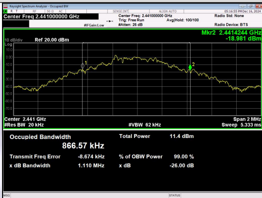
GFSK_DH1_Channel 39
