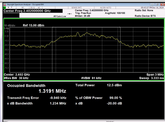
8DPSK_3-DH1_Channel 0
