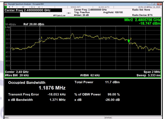
n/4DQPSK_2-DH1_Channel 78
