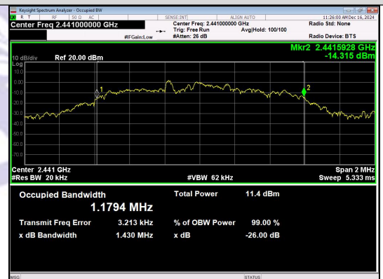
8DPSK_3-DH1_Channel 39
