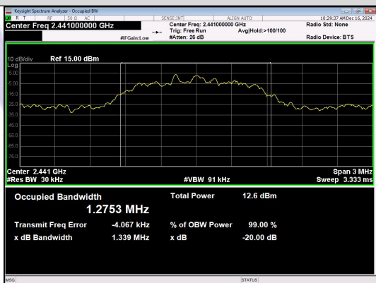
n/4DQPSK_2-DH1_Channel 39
