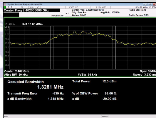
n/4DQPSK_2-DH1_Channel 0
