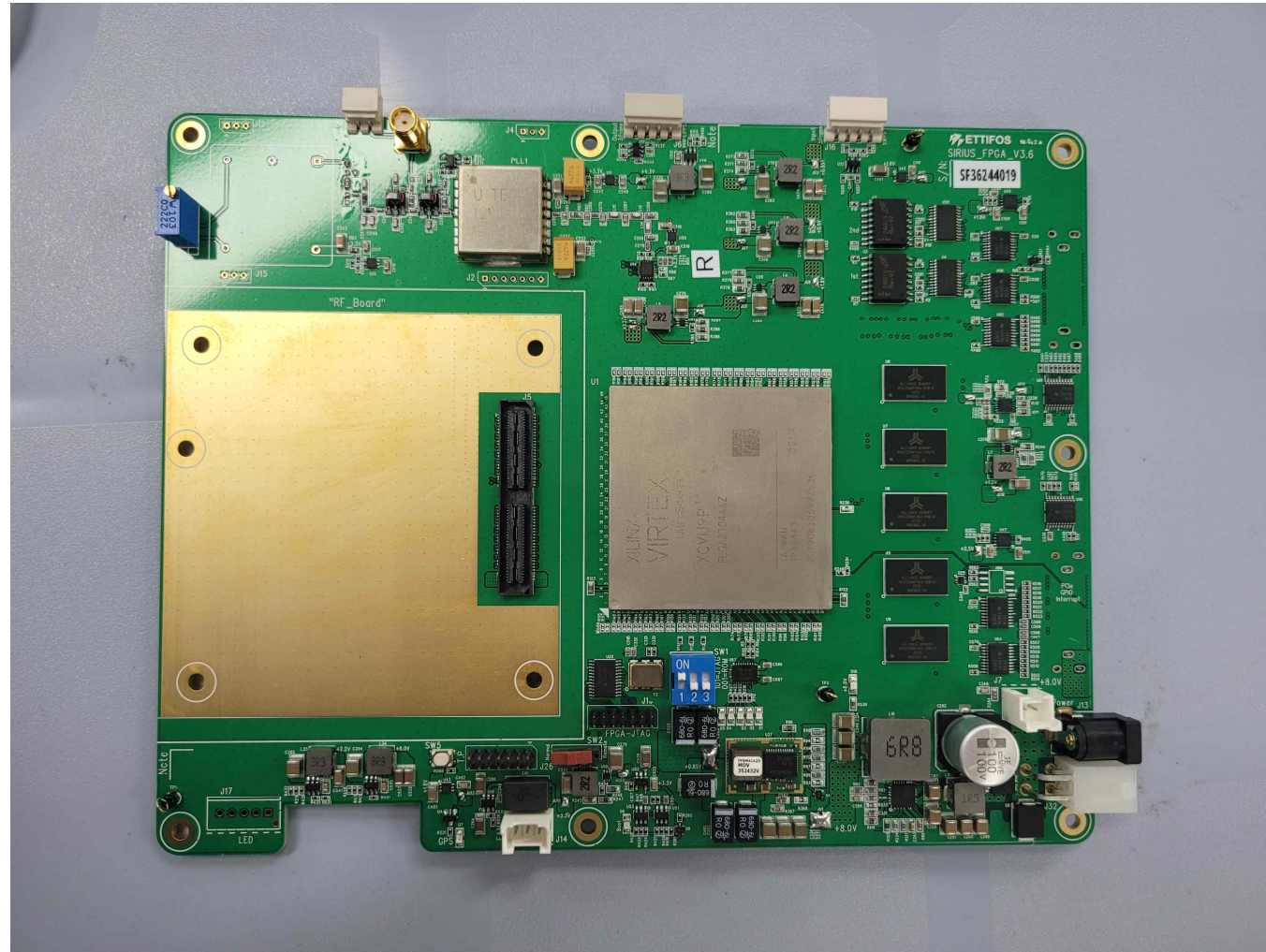
[Main board_Top]
