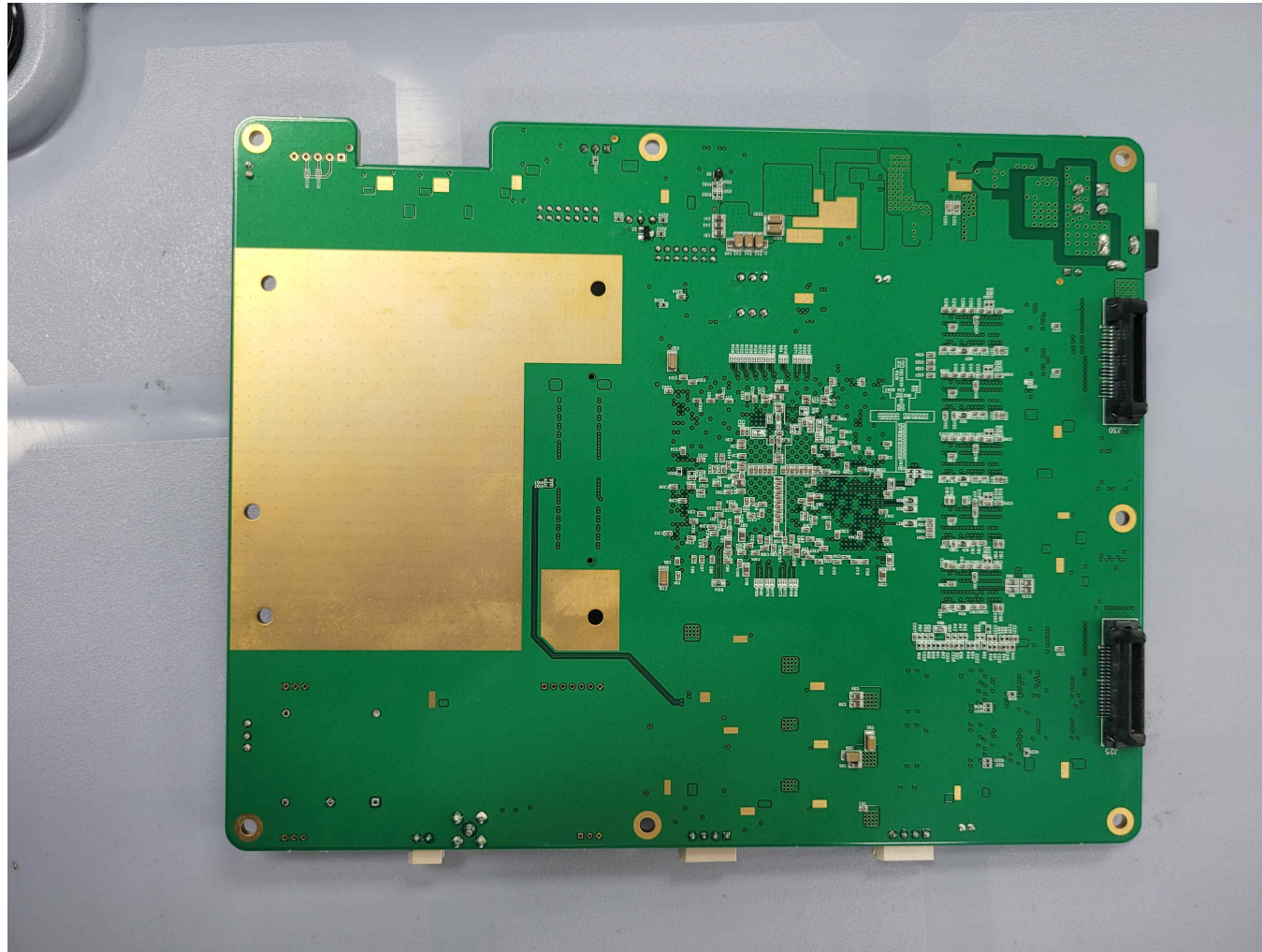
[Main board_Bottom]
