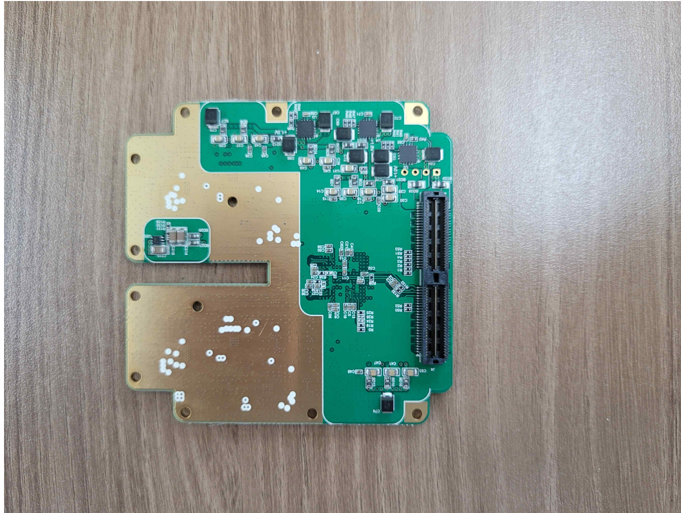
[RF Board_Bottom]
