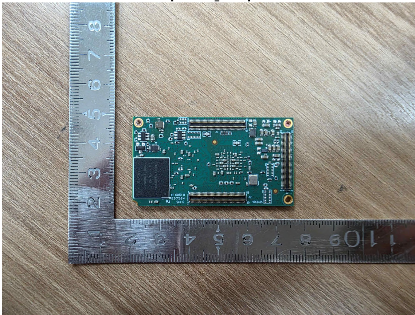
[Sub Board_Bottom]
