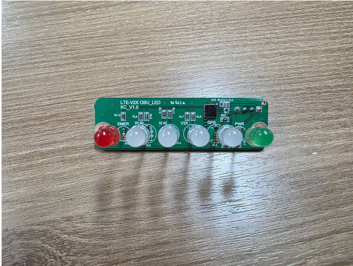
[LED Board_Top]
