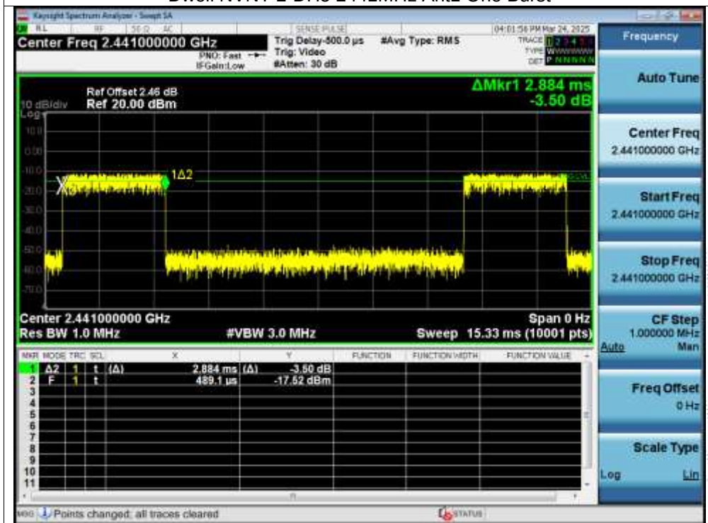
Dwell NVNT 2-DH5 2441MHz Ant1 One Burst
