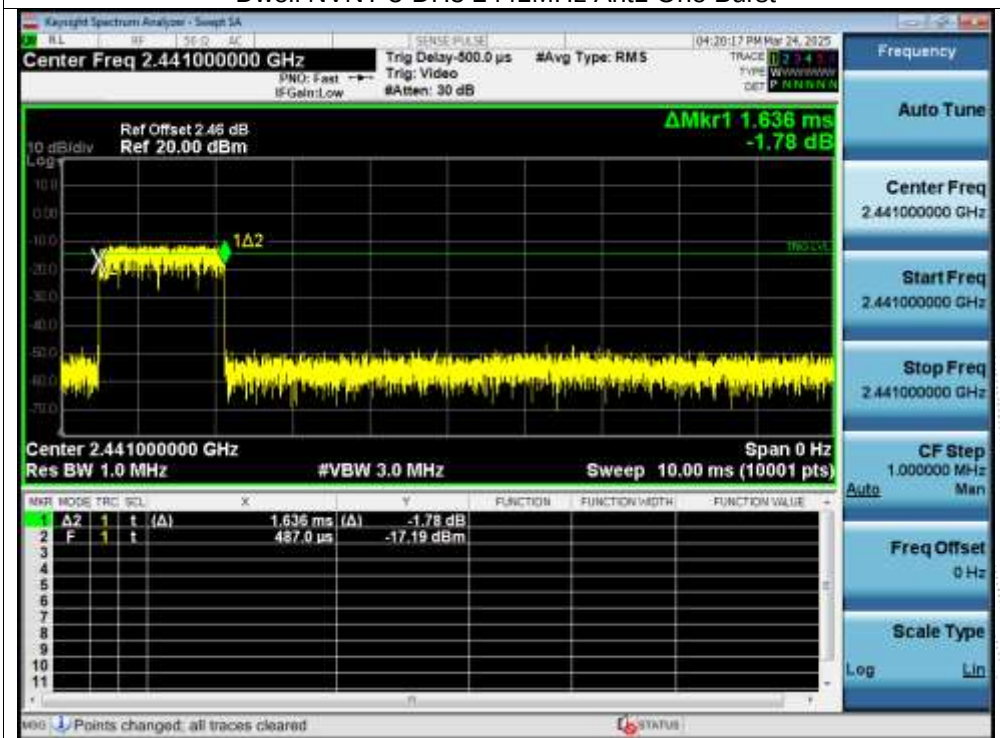
Dwell NVNT 3-DH3 2441MHz Ant1 One Burst
