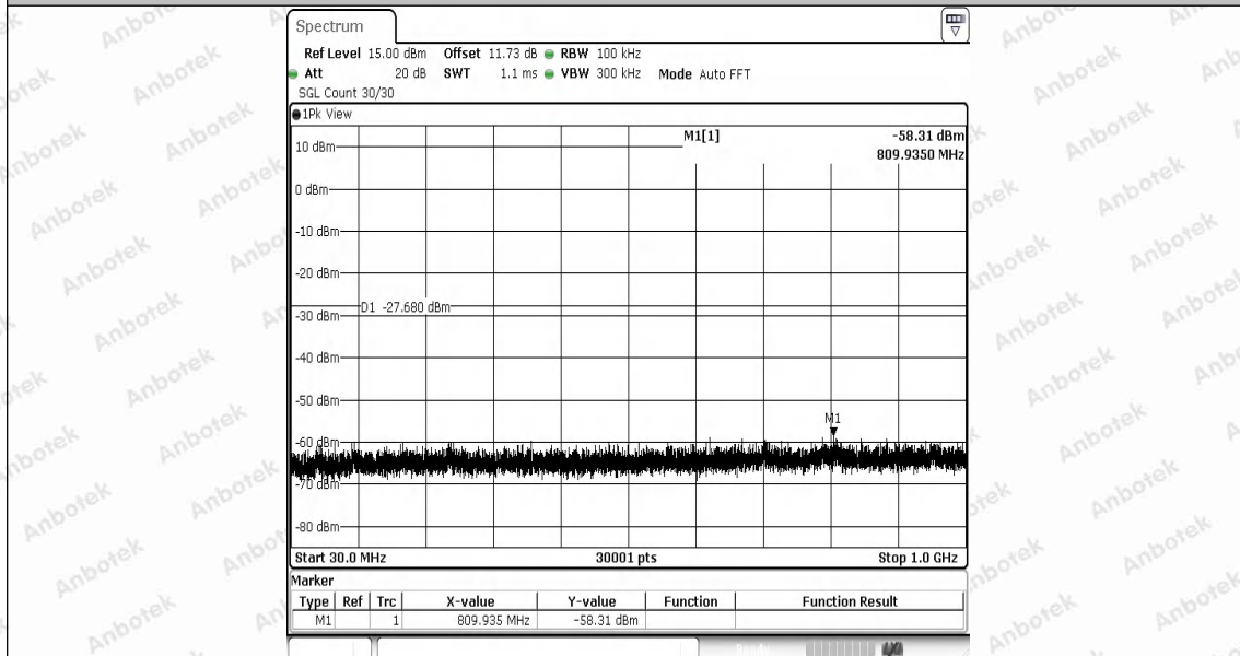
11B-Ant1-2462-0~Reference-PASS
