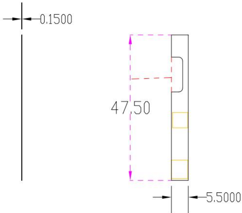
WIFI Antenna
