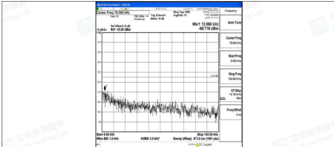
Band41_15MHz_QPSK_41515_1RB#0_0.009~0.15_0.009~0.15
