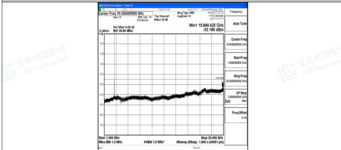
Band41_5MHz_QPSK_40620_1RB#0_1000~20000_1000~20000
