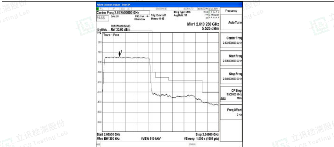
Band38_15MHz_QPSK_38175_75RB#0
