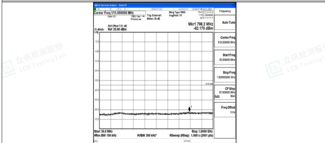
Band38_20MHz_16QAM_37850_1RB#0_30~1000_30~1000
