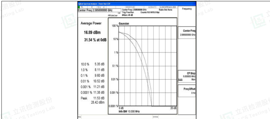
Band38-10MHz-16QAM-38000-50RB#0-PASS
