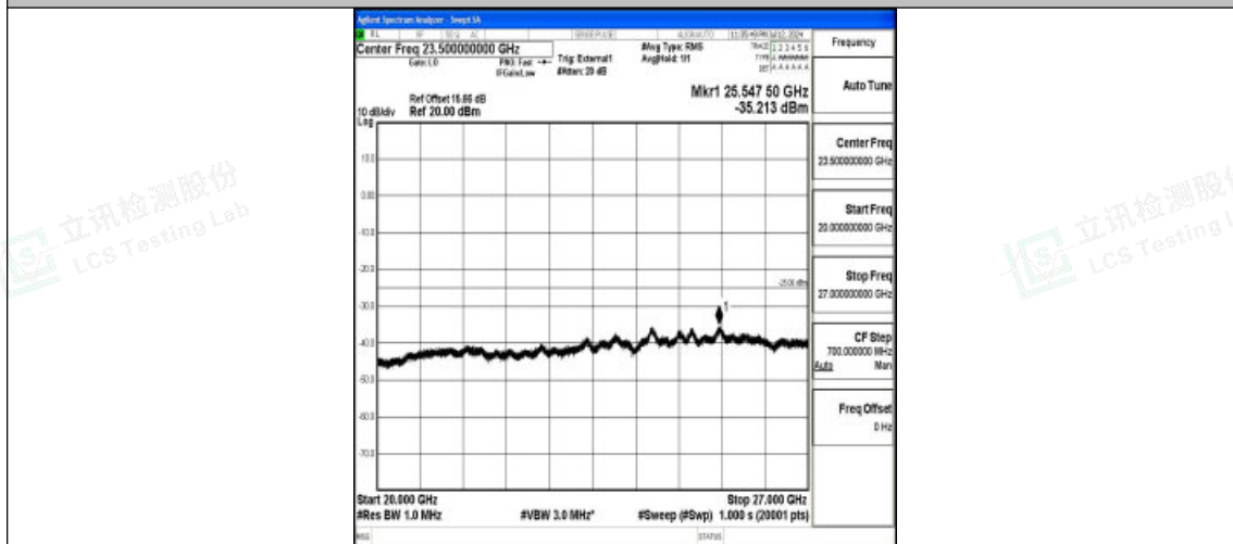
Band38_10MHz_16QAM_38000_1RB#0_20000~27000_20000~27000
