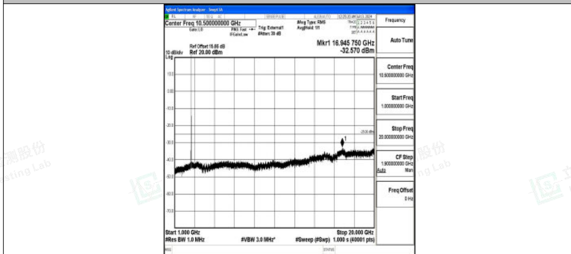
Band38_20MHz_QPSK_37850_1RB#0_1000~20000_1000~20000
