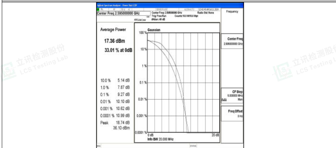
Band38-20MHz-QPSK-38000-100RB#0-PASS
