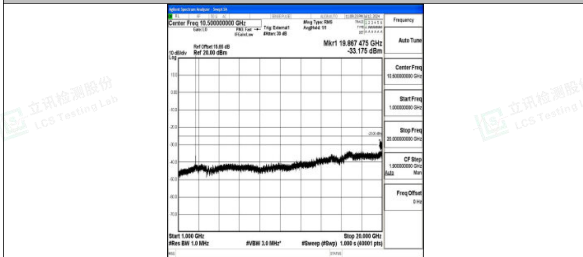
Band38_5MHz_16QAM_38225_1RB#0_1000~20000_1000~20000
