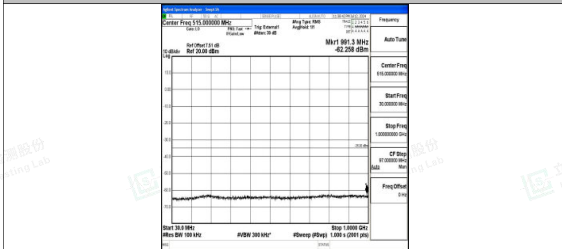
Band38_10MHz_16QAM_38200_1RB#0_30~1000_30~1000
