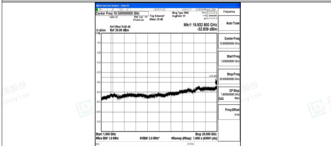
Band38_5MHz_16QAM_38000_1RB#0_1000~20000_1000~20000
