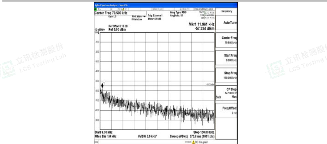
Band38_15MHz_16QAM_38175_1RB#0_0.009~0.15_0.009~0.15
