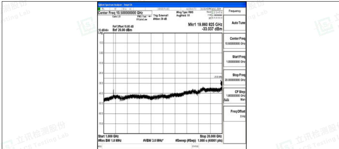
Band38_10MHz_16QAM_37800_1RB#0_1000~20000_1000~20000
