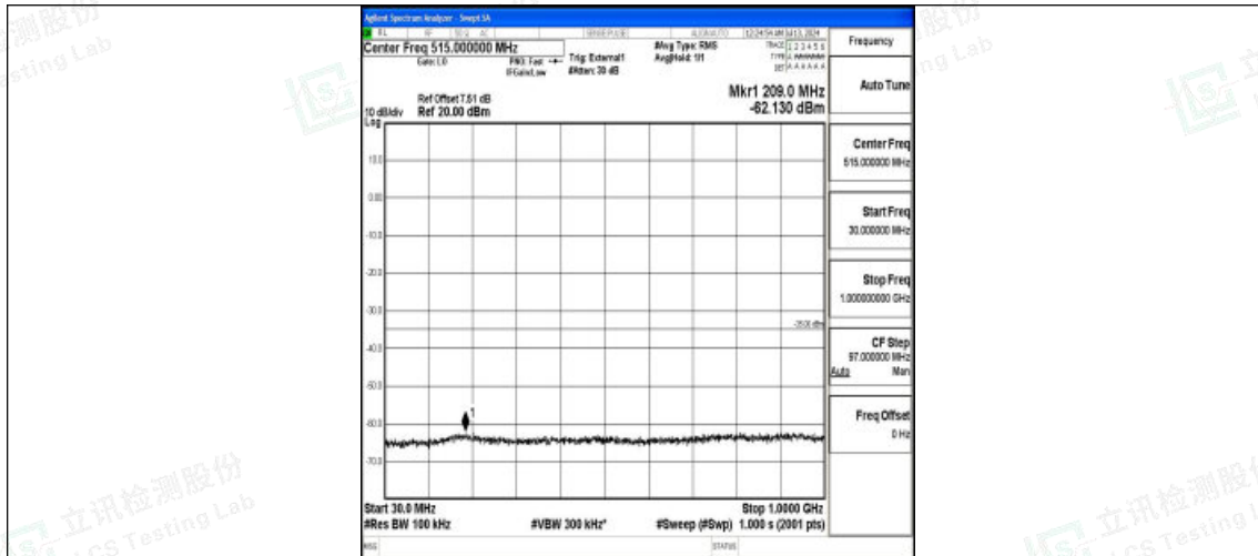
Band38_20MHz_QPSK_37850_1RB#0_30~1000_30~1000
