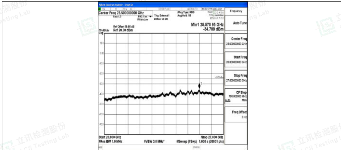
Band38_5MHz_16QAM_38225_1RB#0_20000~27000_20000~27000
