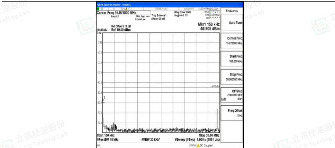
Band38_10MHz_QPSK_38000_1RB#0_0.15~30_0.15~30
