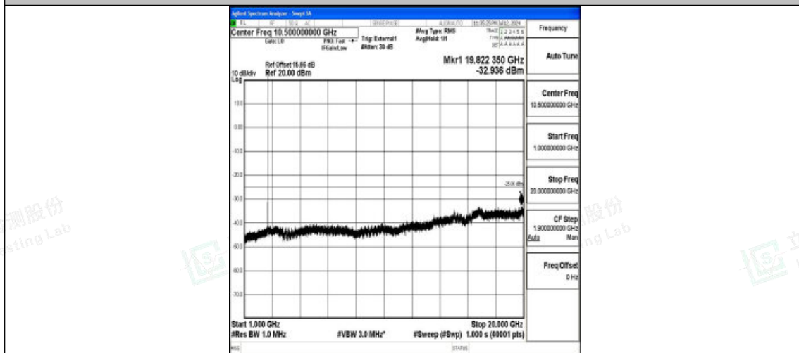
Band38_10MHz_16QAM_38000_1RB#0_1000~20000_1000~20000
