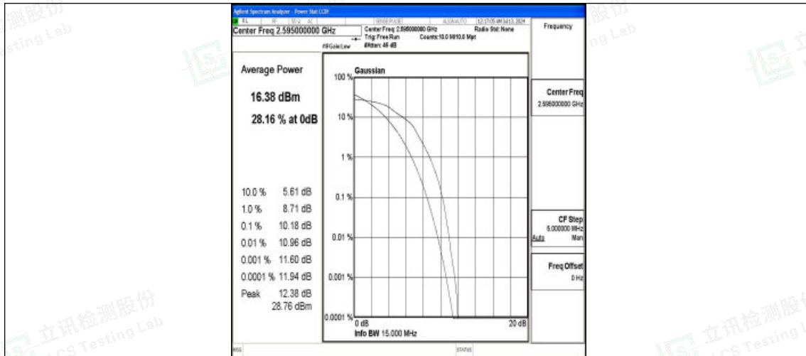
Band38-15MHz-16QAM-38000-75RB#0-PASS
