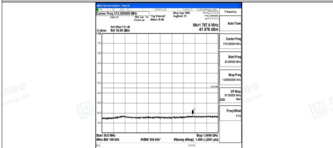
Band38_10MHz_QPSK_38000_1RB#0_30~1000_30~1000
