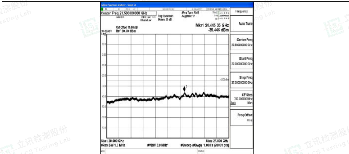
Band38_15MHz_QPSK_38000_1RB#0_20000~27000_20000~27000
