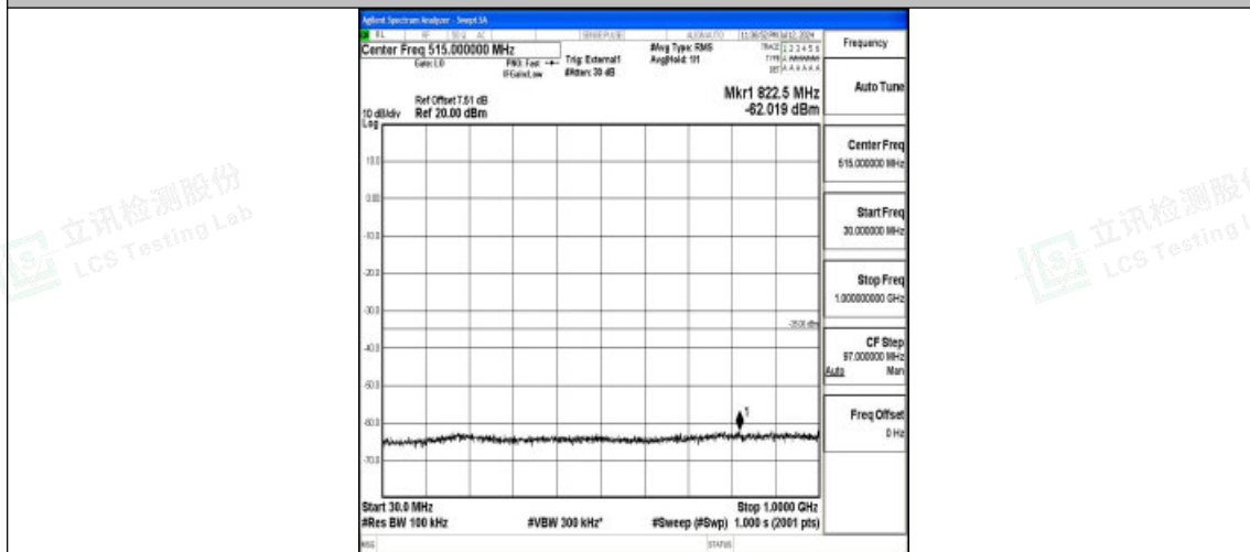
Band38_10MHz_QPSK_38200_1RB#0_30~1000_30~1000
