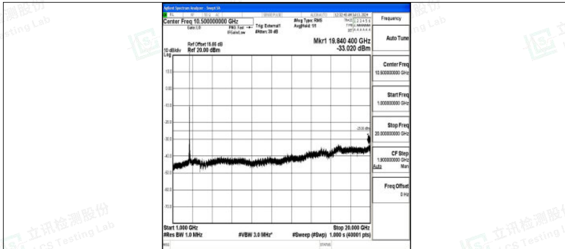
Band38_20MHz_QPSK_38150_1RB#0_1000~20000_1000~20000
