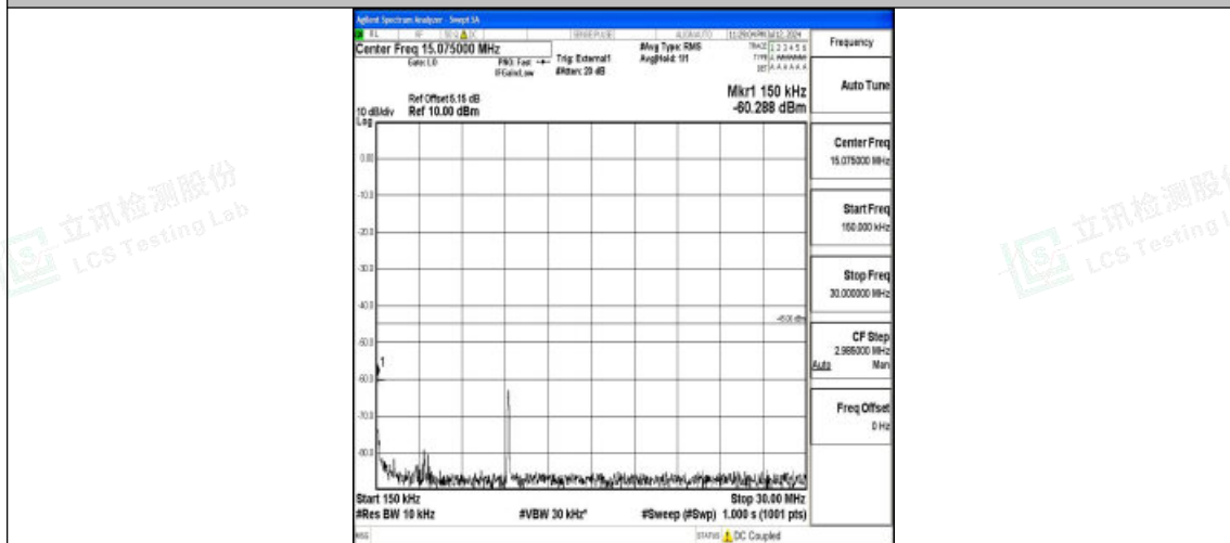
Band38_10MHz_QPSK_37800_1RB#0_0.15~30_0.15~30
