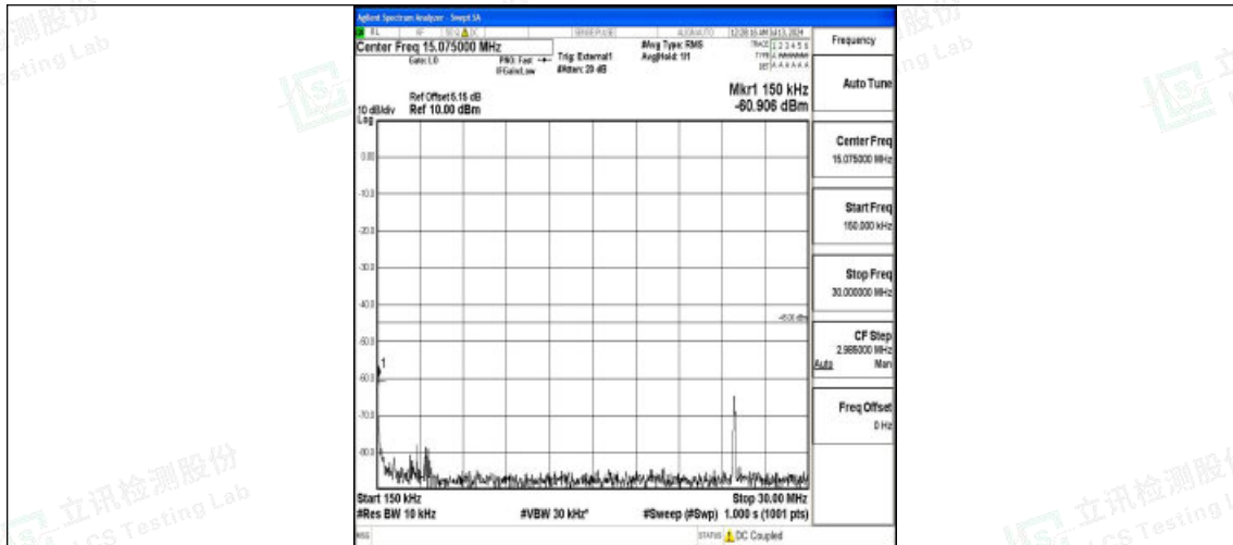
Band38_20MHz_QPSK_38000_1RB#0_0.15~30_0.15~30
