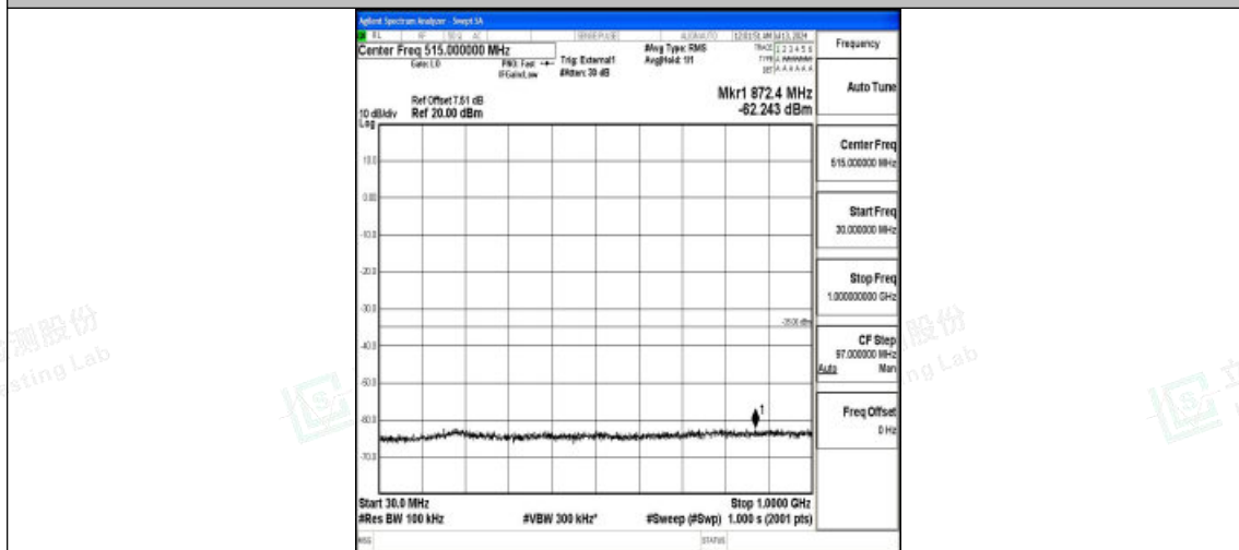
Band38_15MHz_QPSK_38000_1RB#0_30~1000_30~1000
