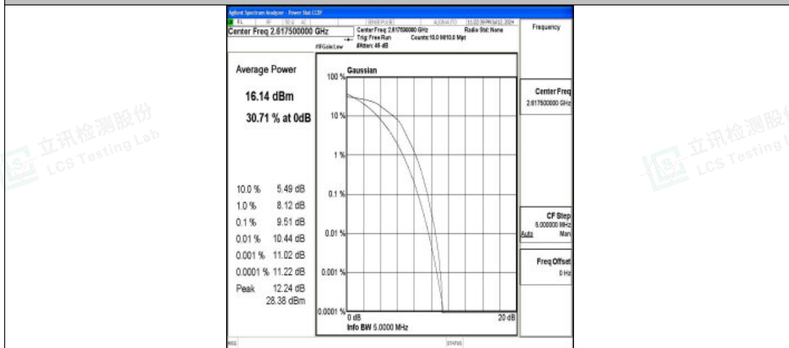
Band38-5MHz-16QAM-38225-25RB#0-PASS
