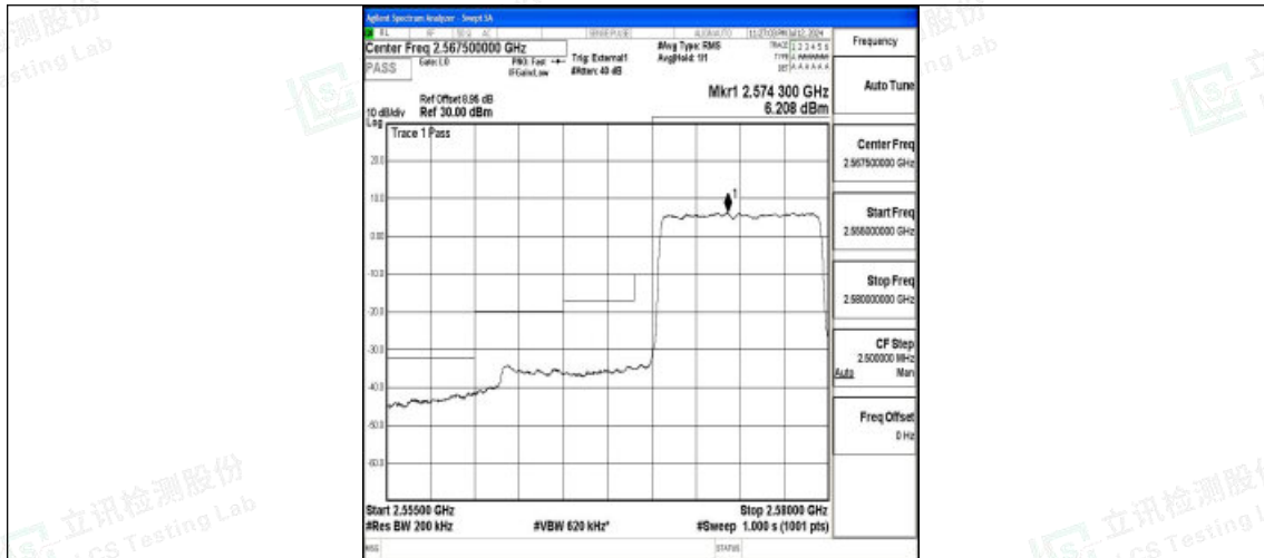
Band38_10MHz_QPSK_37800_50RB#0
