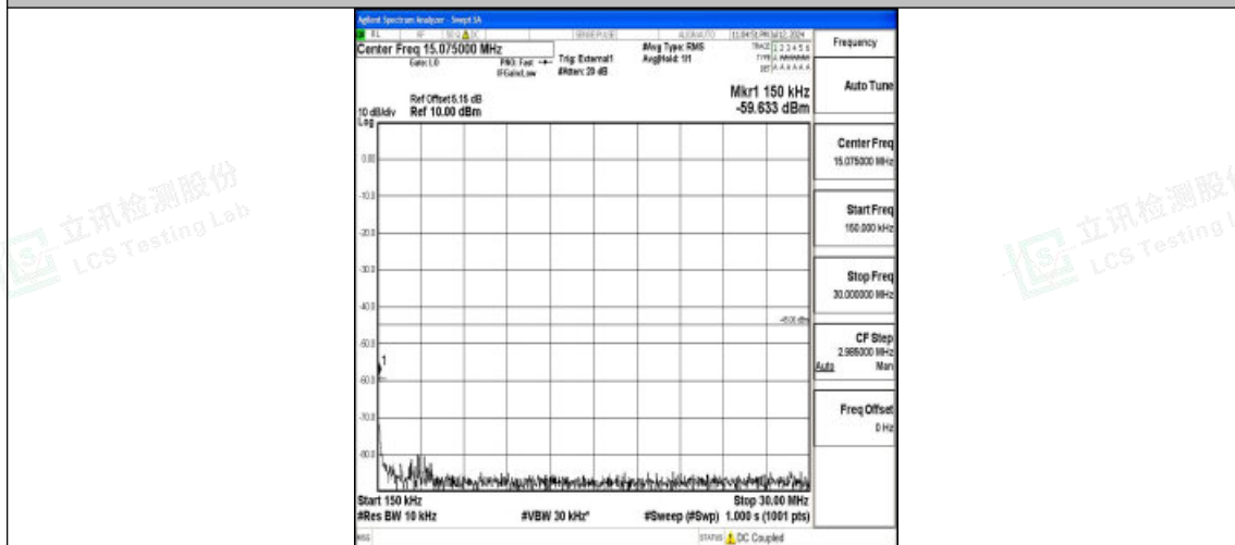
Band38_5MHz_16QAM_38000_1RB#0_0.15~30_0.15~30
