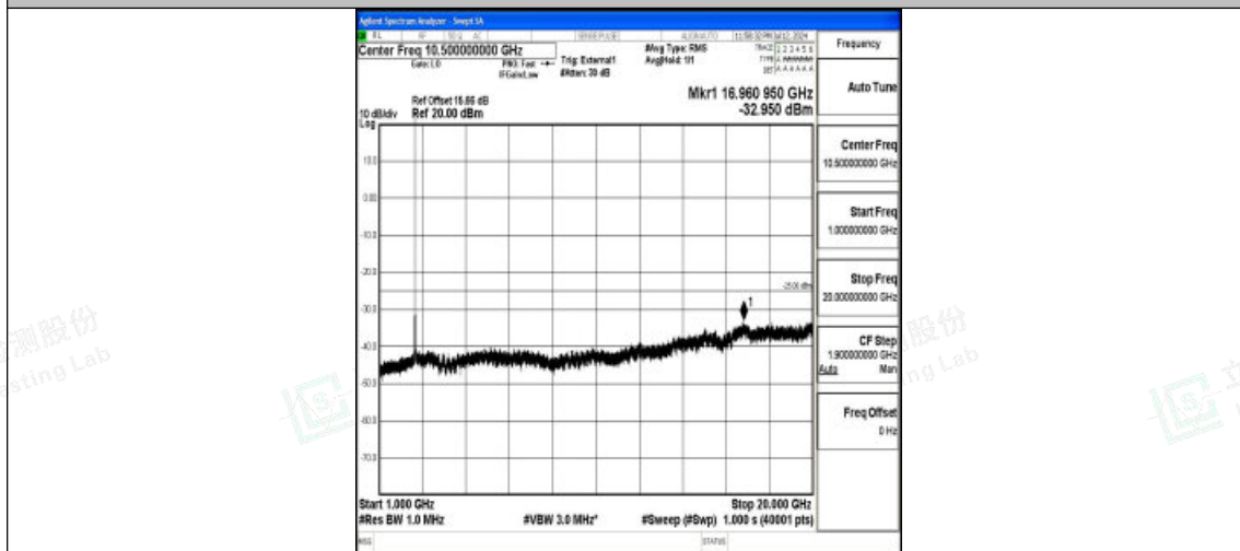
Band38_15MHz_QPSK_37825_1RB#0_1000~20000_1000~20000
