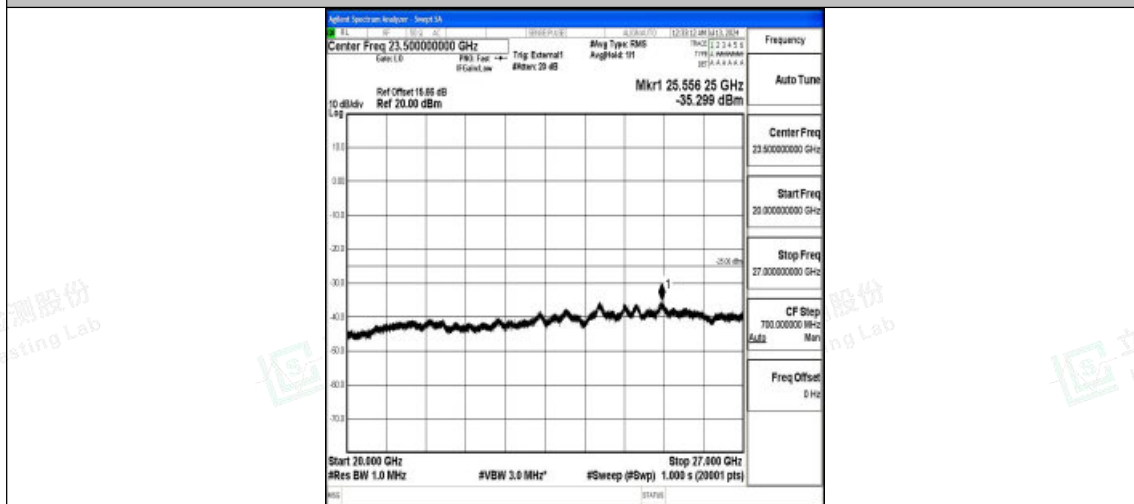
Band38_20MHz_QPSK_38150_1RB#0_20000~27000_20000~27000
