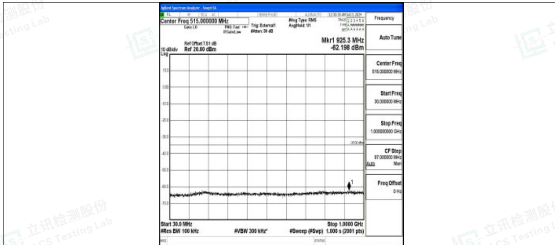
Band38_20MHz_16QAM_38000_1RB#0_30~1000_30~1000
