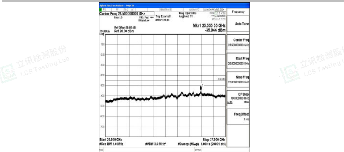
Band38_5MHz_16QAM_38000_1RB#0_20000~27000_20000~27000
