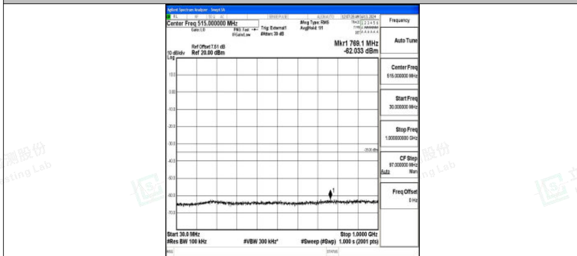
Band38_15MHz_16QAM_38175_1RB#0_30~1000_30~1000
