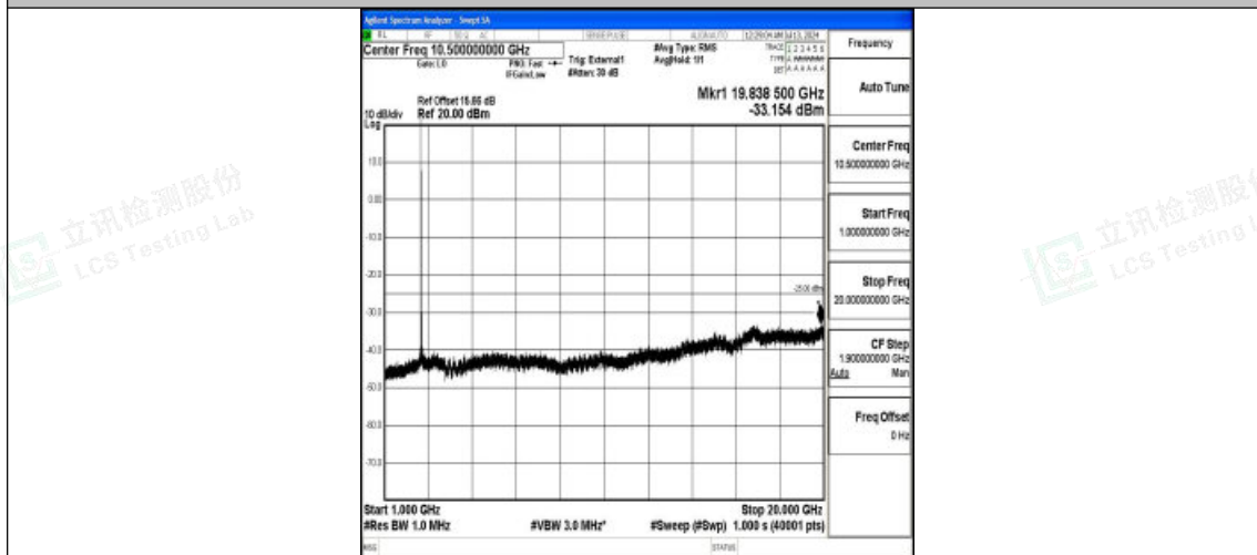
Band38_20MHz_QPSK_38000_1RB#0_1000~20000_1000~20000
