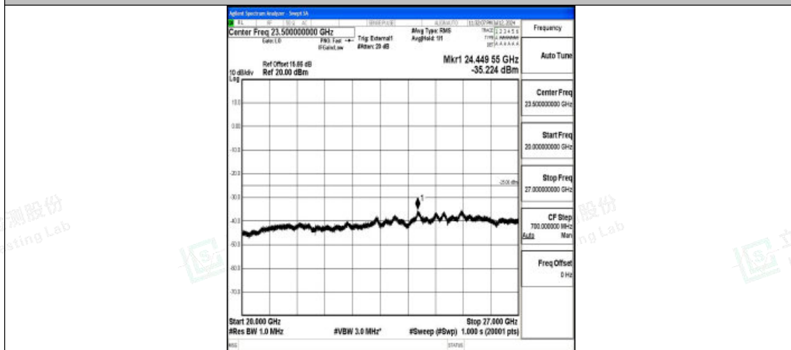
Band38_10MHz_16QAM_37800_1RB#0_20000~27000_20000~27000
