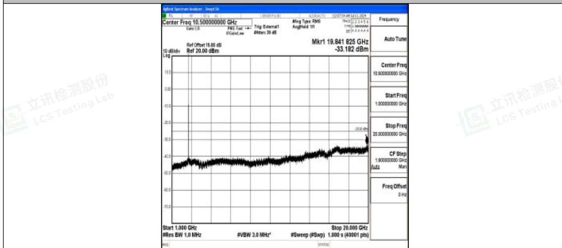
Band38_15MHz_16QAM_38175_1RB#0_1000~20000_1000~20000
