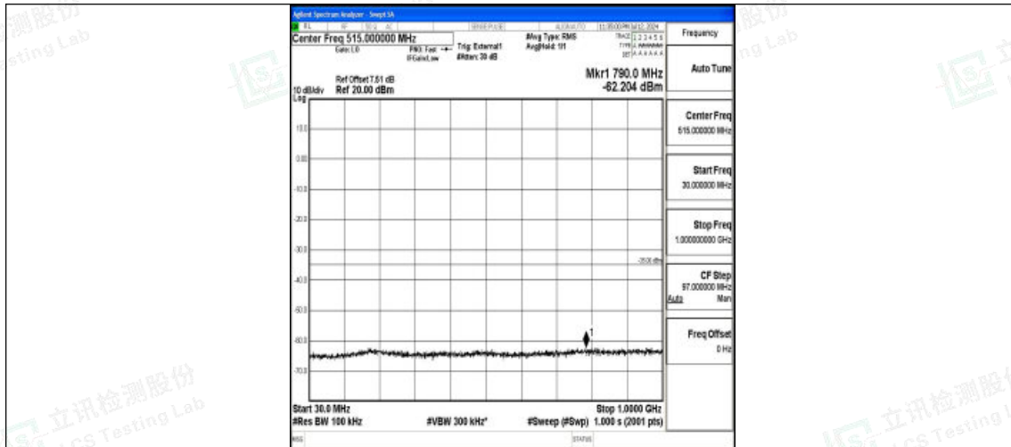
Band38_10MHz_16QAM_38000_1RB#0_30~1000_30~1000
