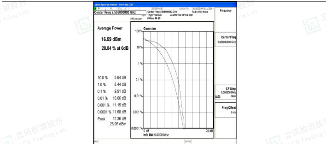
Band38-5MHz-16QAM-38000-25RB#0-PASS
