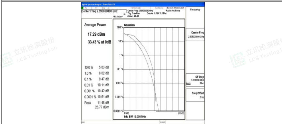
Band38-15MHz-QPSK-38000-75RB#0-PASS
