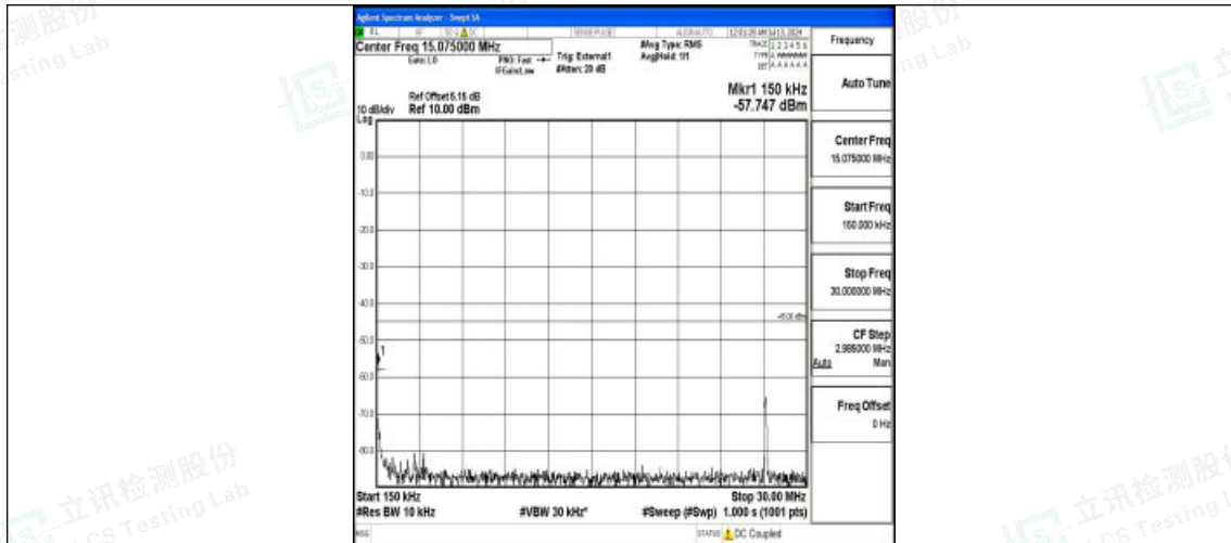
Band38_15MHz_QPSK_38000_1RB#0_0.15~30_0.15~30
