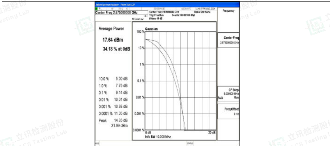
Band38-10MHz-QPSK-37800-50RB#0-PASS
