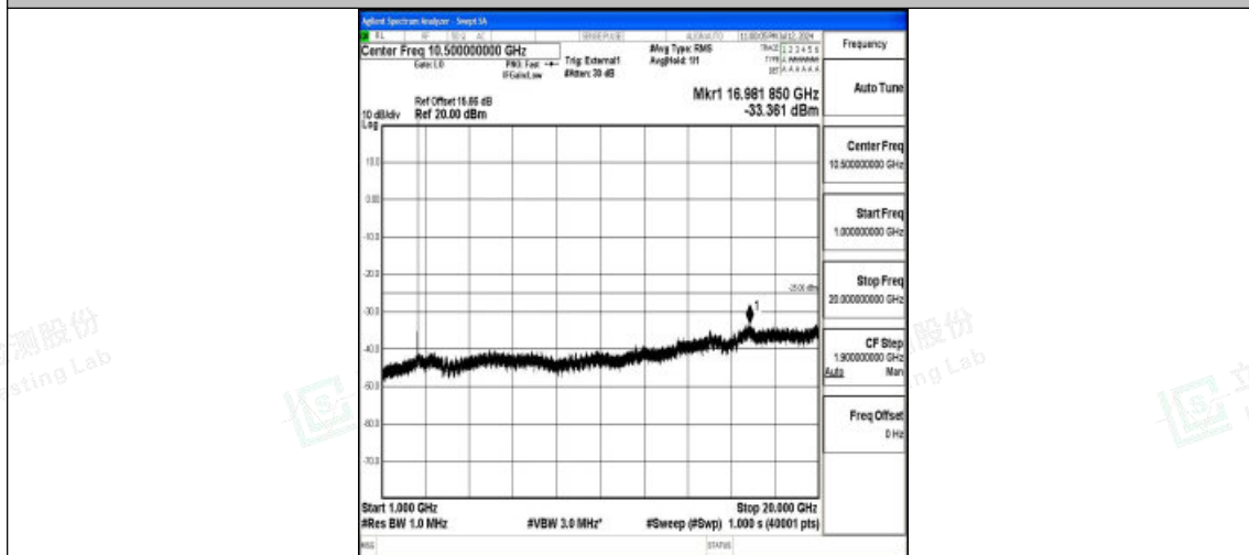
Band38_5MHz_QPSK_37775_1RB#0_1000~20000_1000~20000
