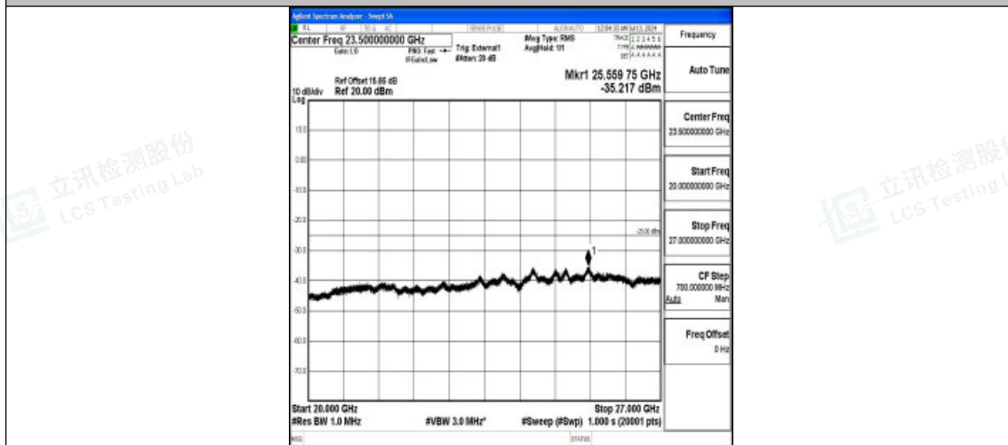
Band38_15MHz_16QAM_38000_1RB#0_20000~27000_20000~27000
