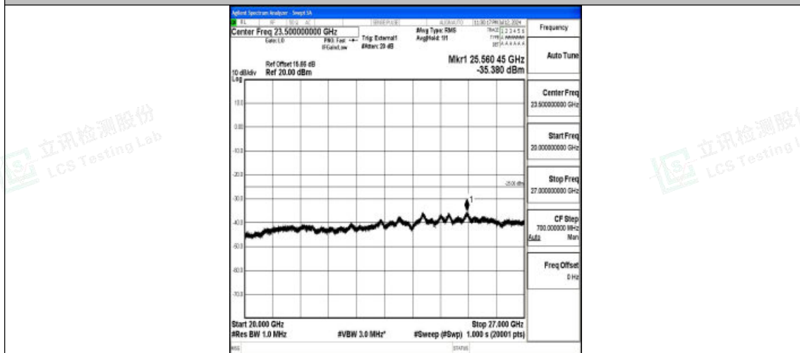
Band38_10MHz_QPSK_37800_1RB#0_20000~27000_20000~27000
