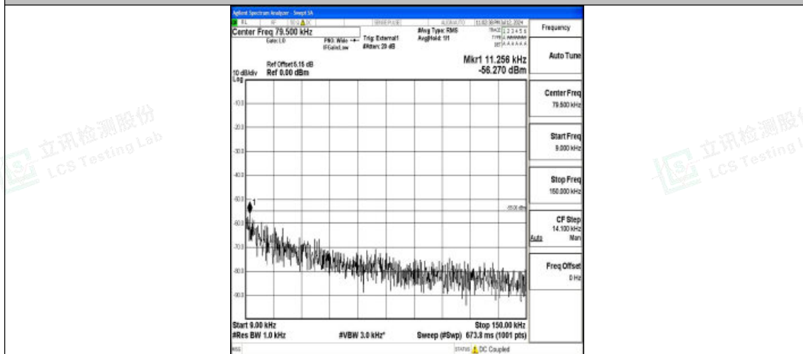
Band38_5MHz_QPSK_38000_1RB#0_0.009~0.15_0.009~0.15
