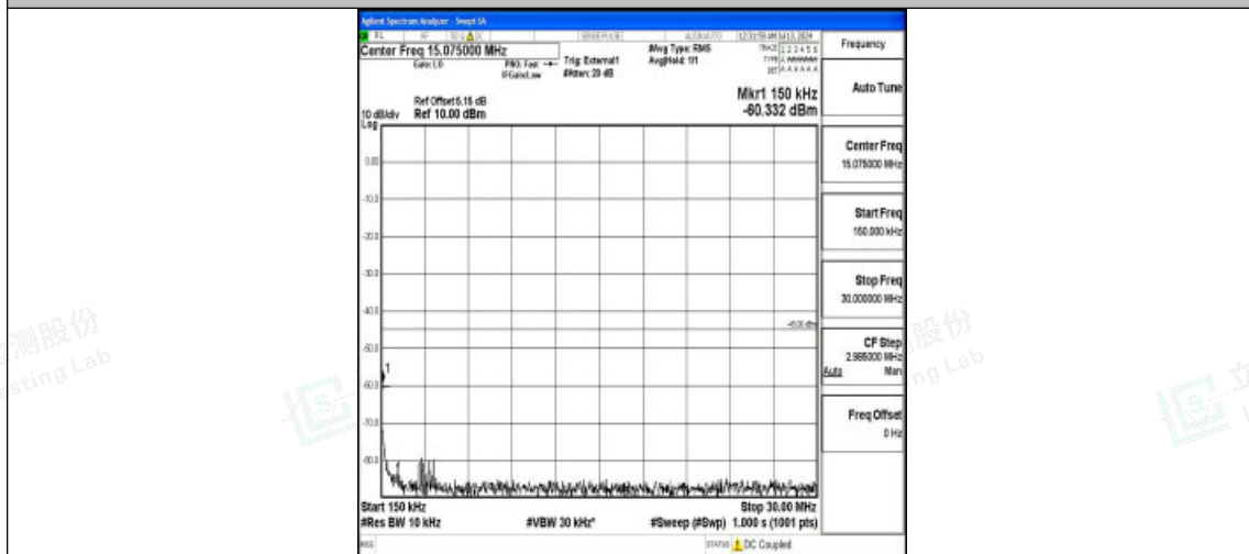
Band38_20MHz_QPSK_38150_1RB#0_0.15~30_0.15~30
