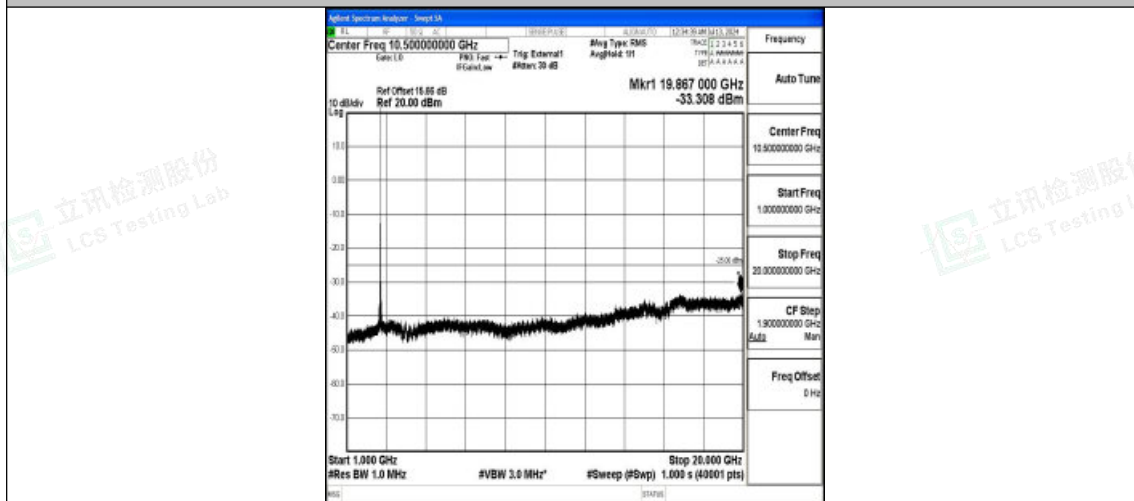
Band38_20MHz_16QAM_38150_1RB#0_1000~20000_1000~20000
