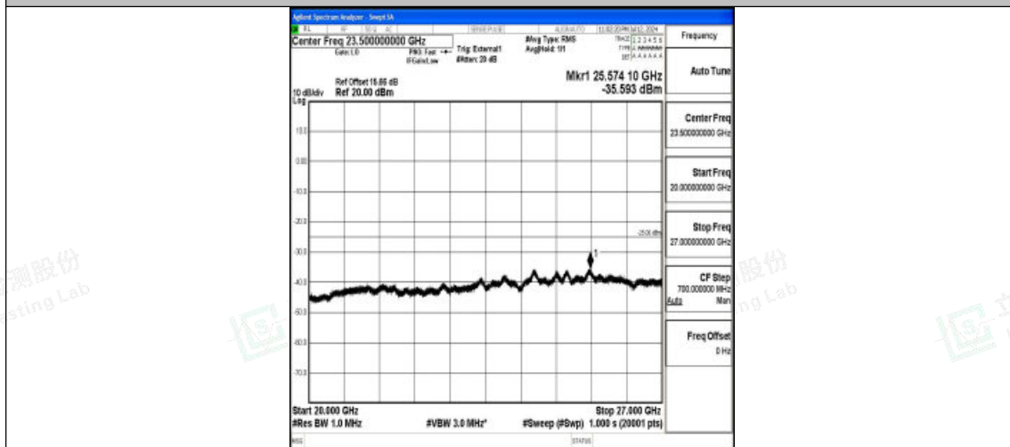
Band38_5MHz_16QAM_37775_1RB#0_20000~27000_20000~27000
