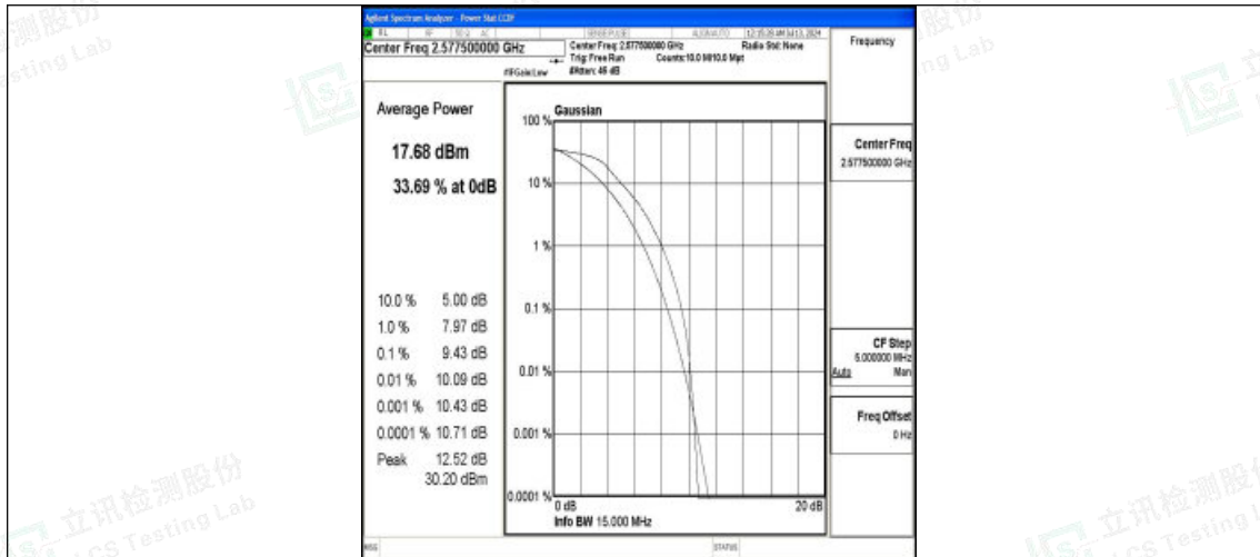
Band38-15MHz-QPSK-37825-75RB#0-PASS
