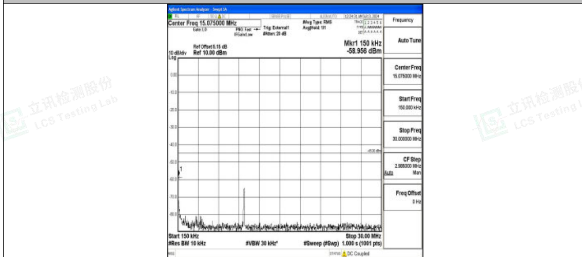
Band38_20MHz_QPSK_37850_1RB#0_0.15~30_0.15~30
