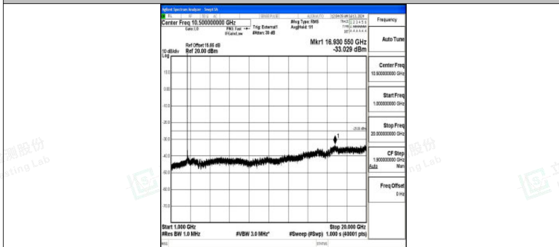
Band38_15MHz_16QAM_38000_1RB#0_1000~20000_1000~20000
