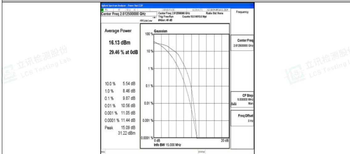
Band38-15MHz-16QAM-38175-75RB#0-PASS
