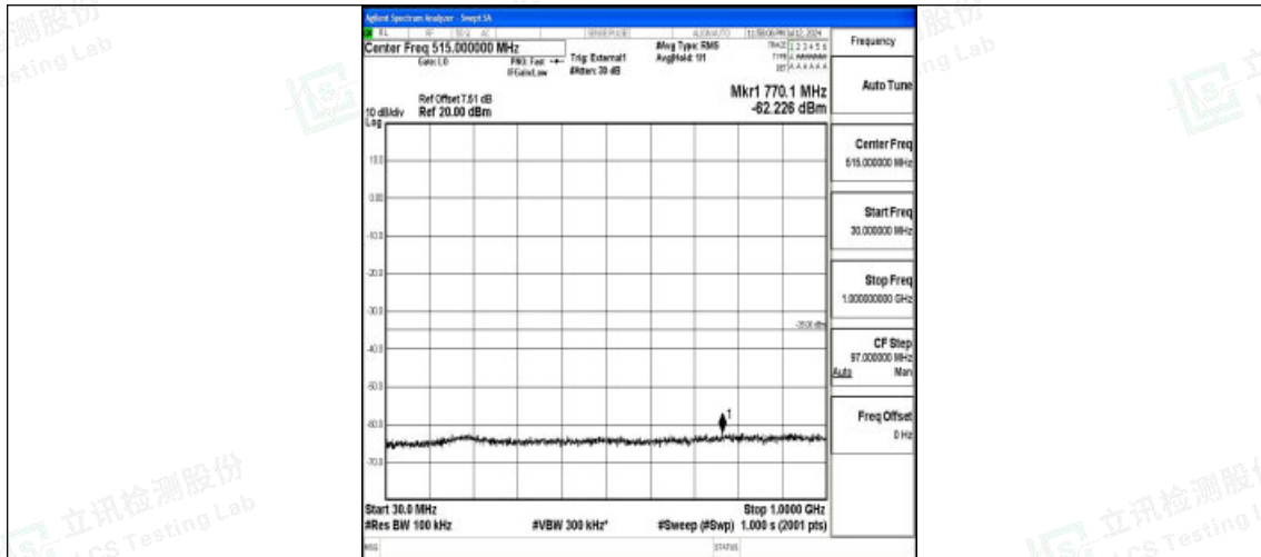
Band38_15MHz_QPSK_37825_1RB#0_30~1000_30~1000
