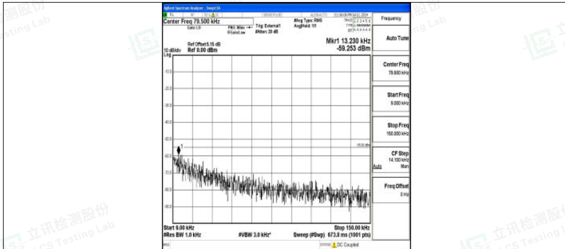
Band38_10MHz_QPSK_38200_1RB#0_0.009~0.15_0.009~0.15
