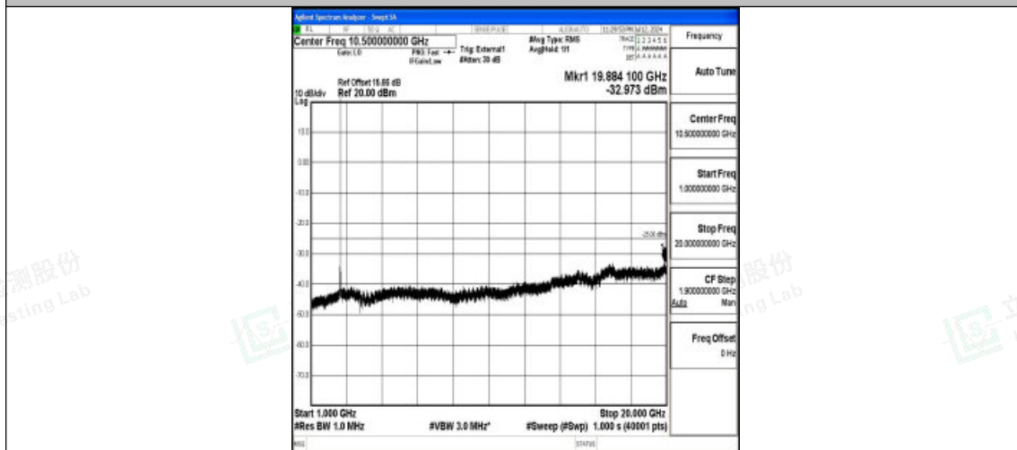
Band38_10MHz_QPSK_37800_1RB#0_1000~20000_1000~20000
