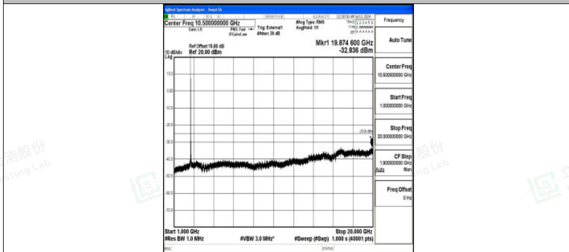
Band38_20MHz_16QAM_38000_1RB#0_1000~20000_1000~20000
