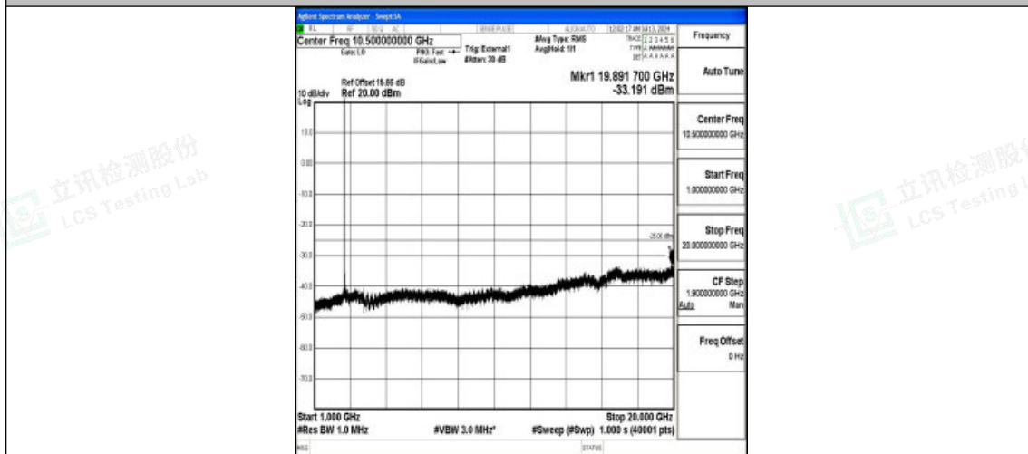
Band38_15MHz_QPSK_38000_1RB#0_1000~20000_1000~20000
