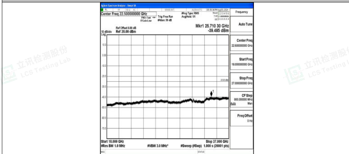
Band7-10MHz-16QAM-21400-1RB#0-18000~27000-PASS
