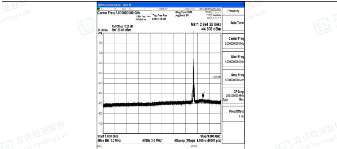
Band7-15MHz-QPSK-21100-1RB#0-1000~3000-PASS
