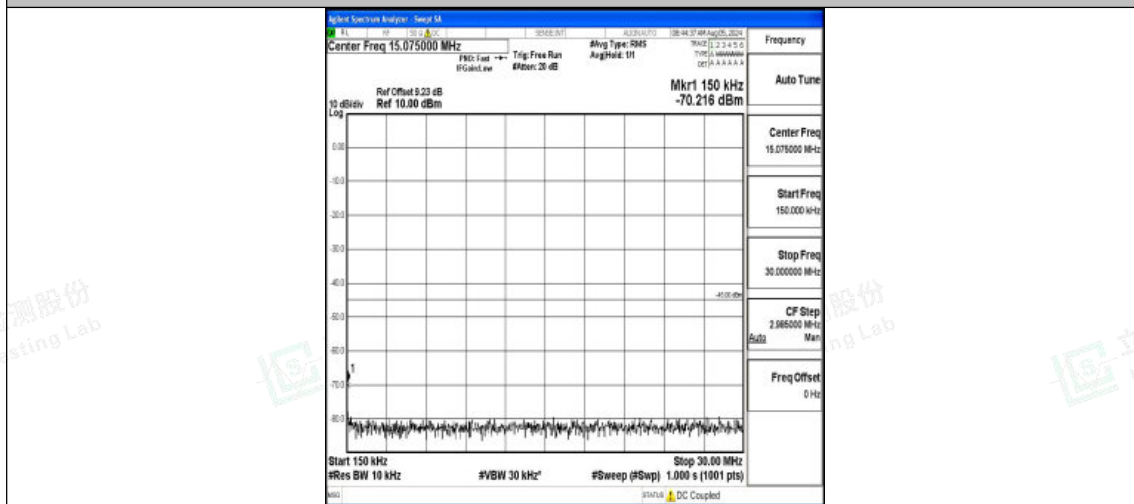
Band7-15MHz-16QAM-21375-1RB#0-0.15~30-PASS
