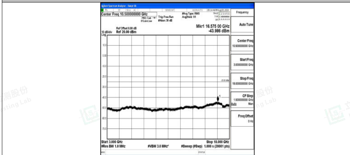
Band7-5MHz-16QAM-21425-1RB#0-3000~18000-PASS
