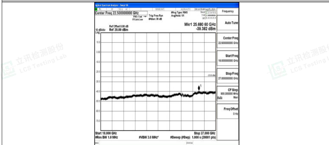
Band7-20MHz-QPSK-20850-1RB#0-18000~27000-PASS
