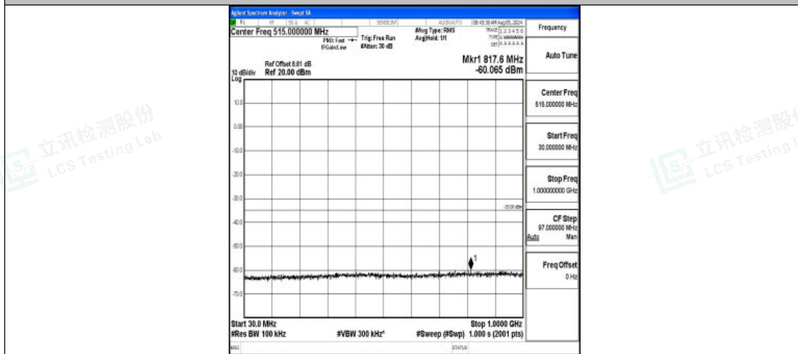
Band7-15MHz-QPSK-21375-1RB#0-30~1000-PASS
