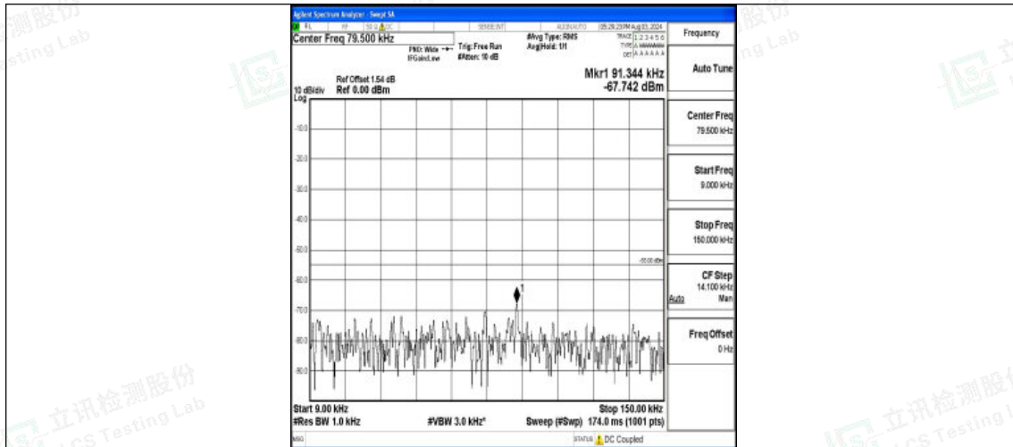
Band7-10MHz-16QAM-20800-1RB#0-0.009~0.15-PASS
