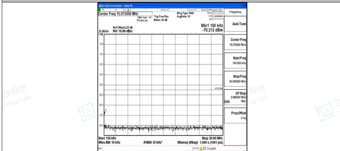
Band7-10MHz-QPSK-21400-1RB#0-0.15~30-PASS
