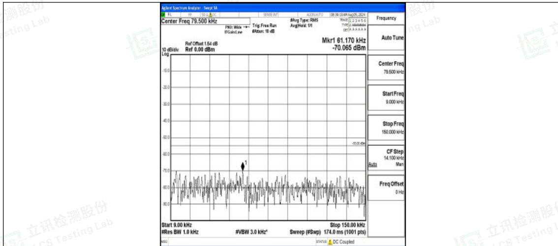
Band7-15MHz-16QAM-20825-1RB#0-0.009~0.15-PASS
