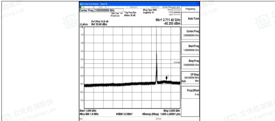
Band7-10MHz-QPSK-20800-1RB#0-1000~3000-PASS
