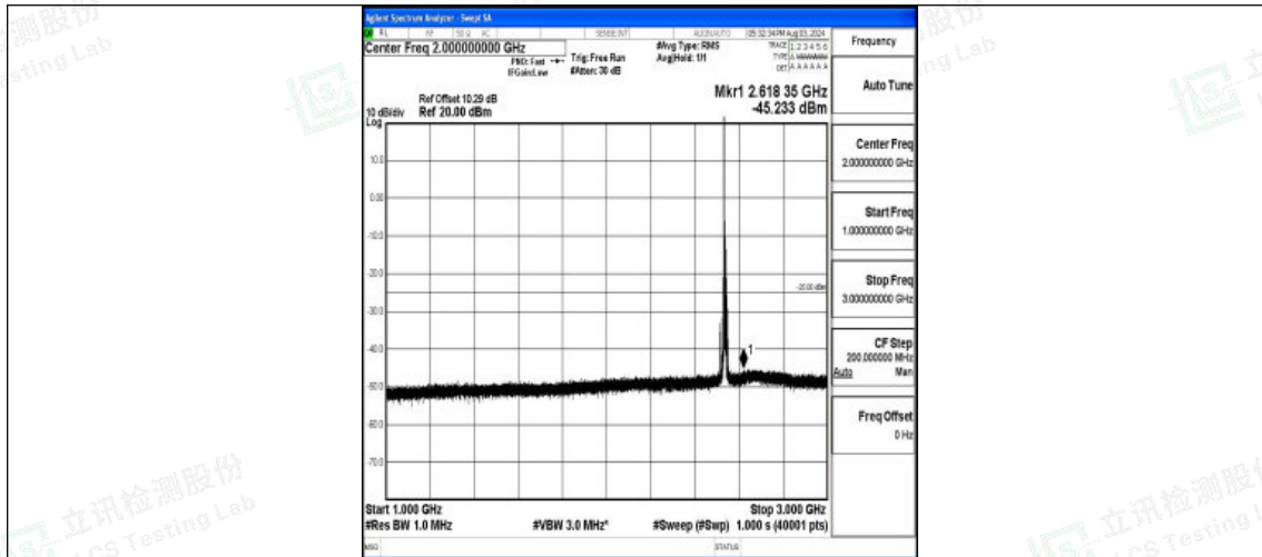
Band7-10MHz-16QAM-21100-1RB#0-1000~3000-PASS
