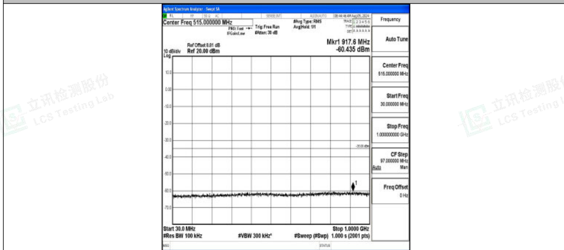
Band7-15MHz-16QAM-21375-1RB#0-30~1000-PASS
