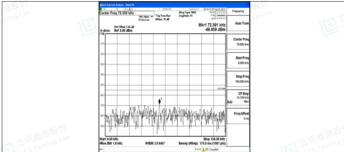
Band7-15MHz-QPSK-21100-1RB#0-0.009~0.15-PASS
