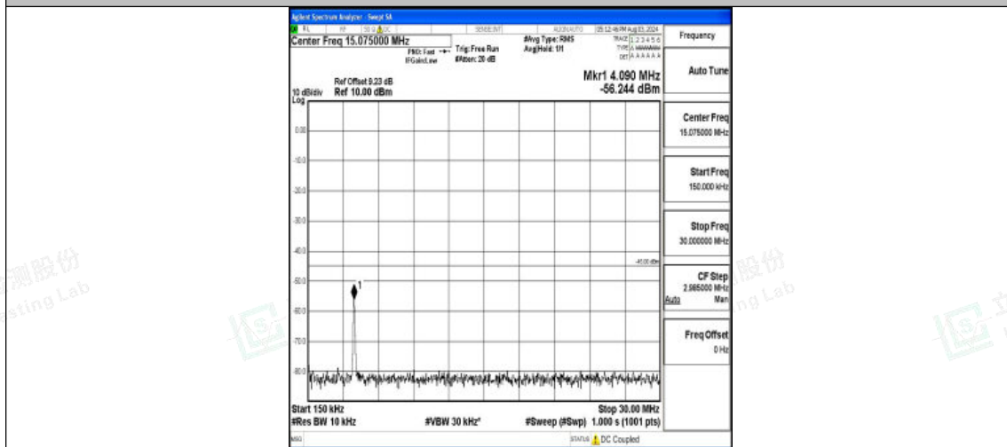
Band7-5MHz-QPSK-21425-1RB#0-0.15~30-PASS
