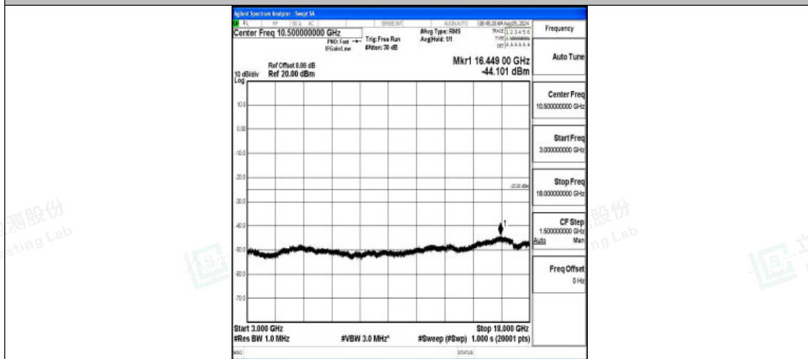
Band7-15MHz-16QAM-21375-1RB#0-3000~18000-PASS
