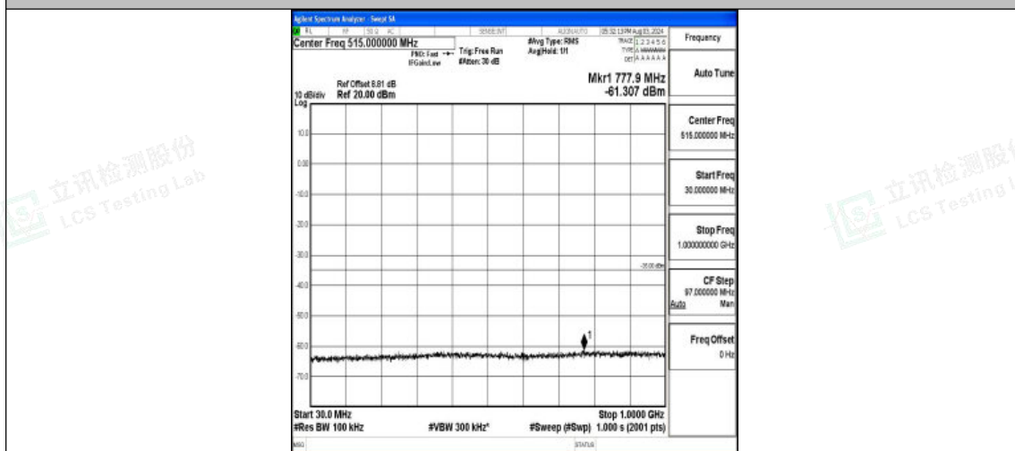
Band7-10MHz-16QAM-21100-1RB#0-30~1000-PASS
