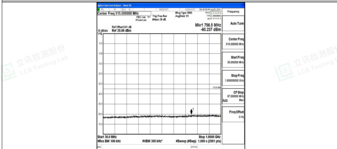
Band7-15MHz-QPSK-21100-1RB#0-30~1000-PASS
