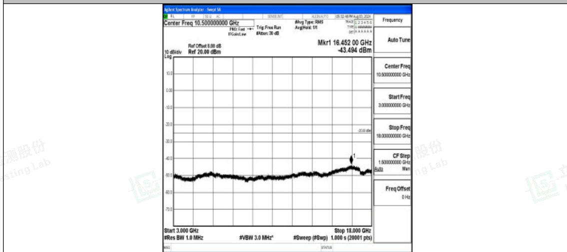
Band7-10MHz-16QAM-21100-1RB#0-3000~18000-PASS
