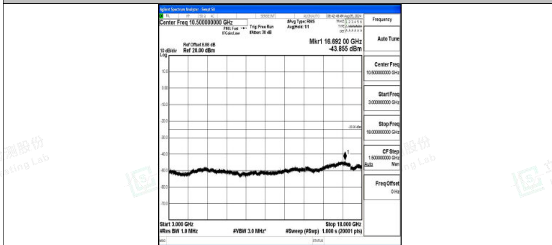
Band7-15MHz-16QAM-21100-1RB#0-3000~18000-PASS
