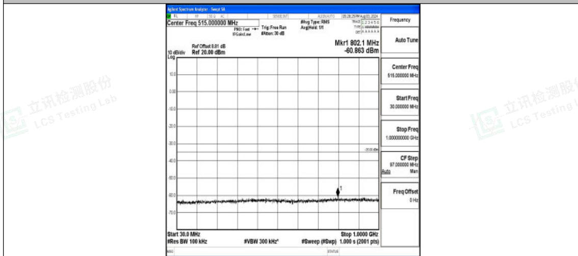
Band7-10MHz-QPSK-20800-1RB#0-30~1000-PASS
