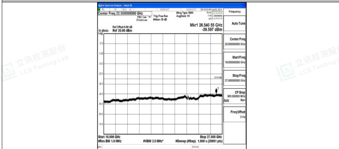
Band7-15MHz-16QAM-21100-1RB#0-18000~27000-PASS
