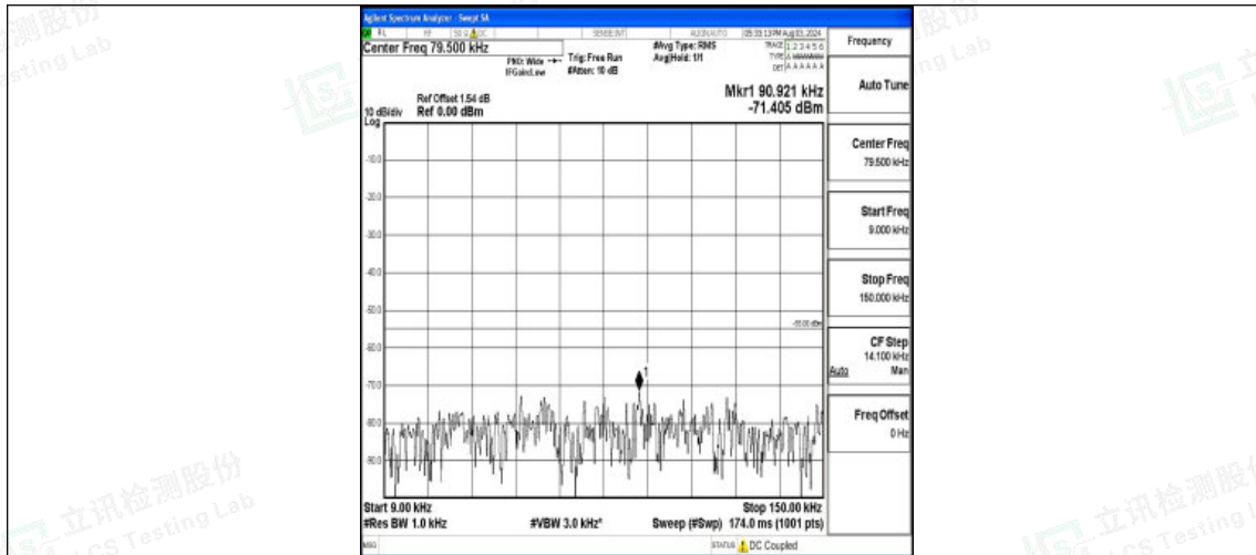
Band7-10MHz-QPSK-21400-1RB#0-0.009~0.15-PASS
