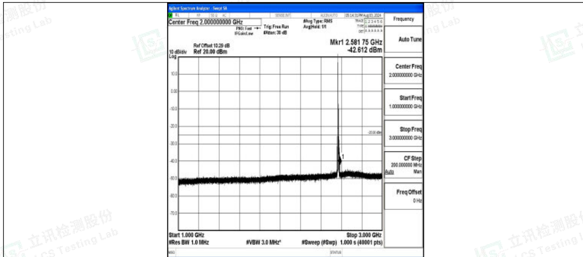
Band7-5MHz-16QAM-21425-1RB#0-1000~3000-PASS
