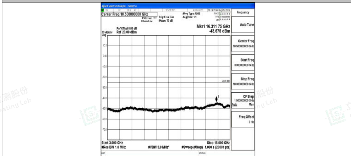
Band7-20MHz-QPSK-21350-1RB#0-3000~18000-PASS
