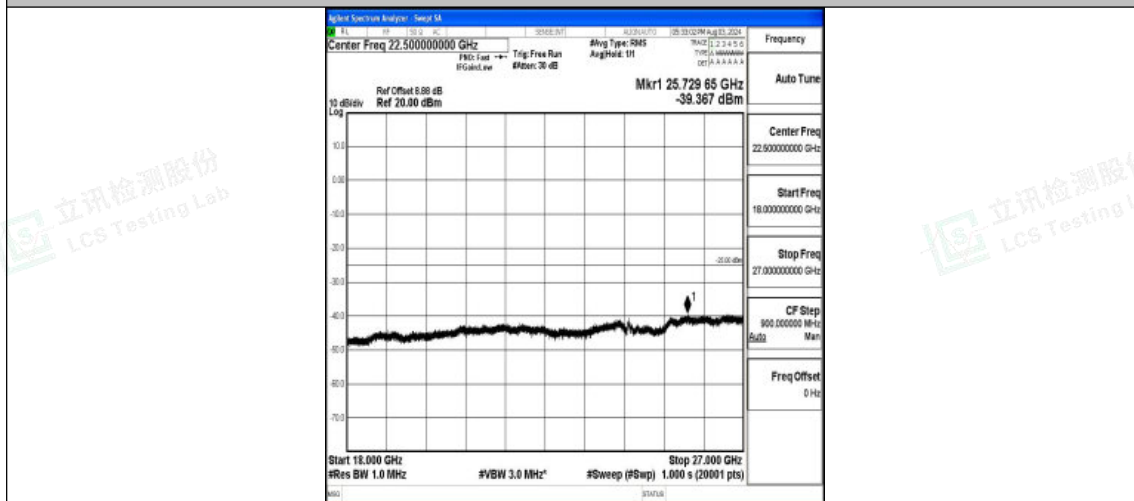
Band7-10MHz-16QAM-21100-1RB#0-18000~27000-PASS
