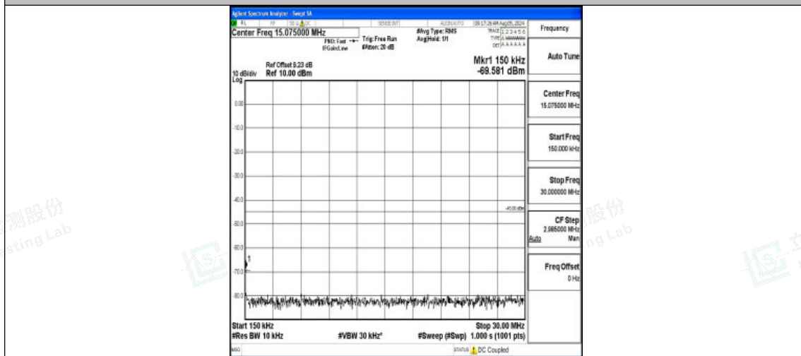
Band7-20MHz-16QAM-21100-1RB#0-0.15~30-PASS
