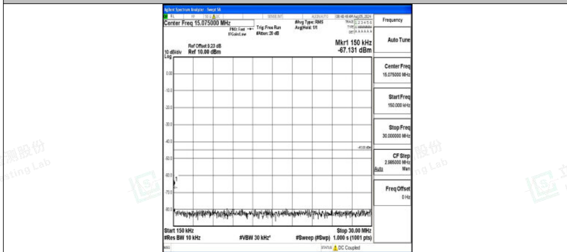
Band7-15MHz-QPSK-21100-1RB#0-0.15~30-PASS
