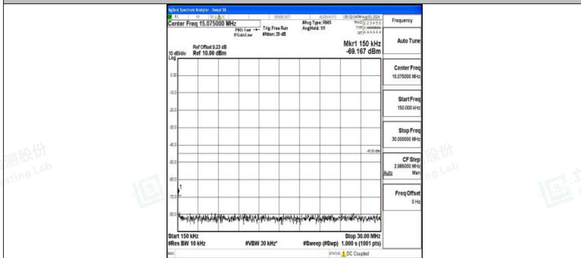
Band7-10MHz-16QAM-21100-1RB#0-0.15~30-PASS
