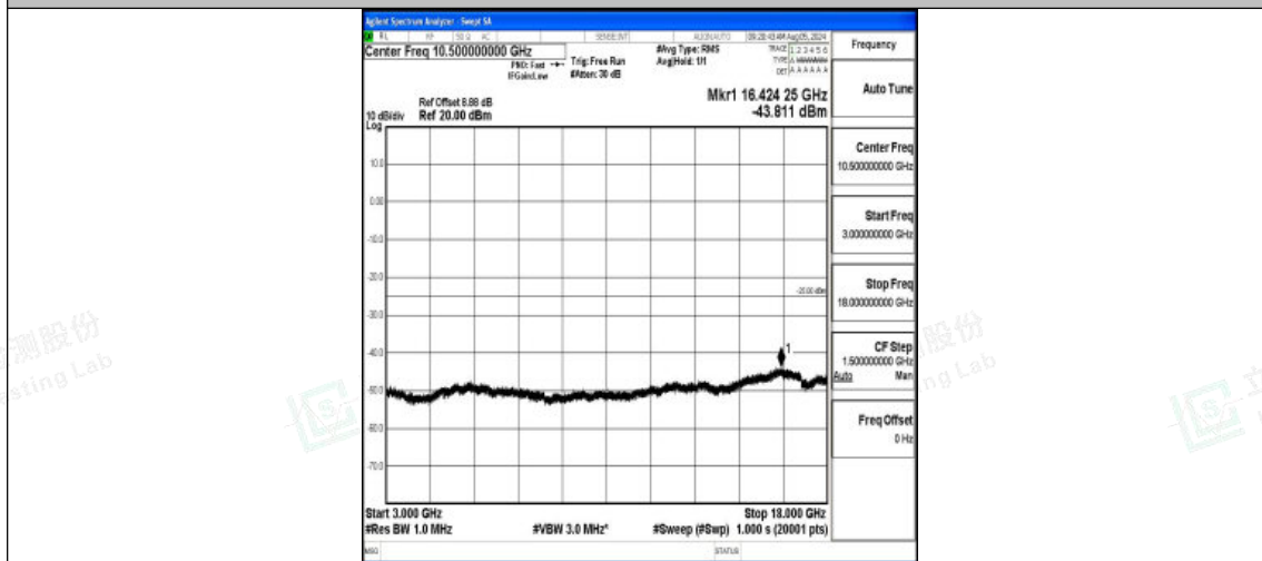
Band7-20MHz-16QAM-21350-1RB#0-3000~18000-PASS
