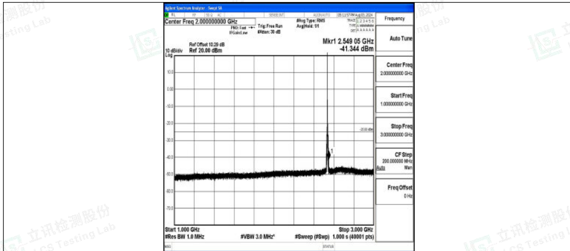
Band7-5MHz-16QAM-21100-1RB#0-1000~3000-PASS
