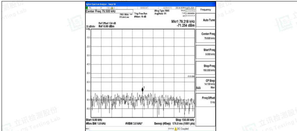
Band7-10MHz-16QAM-21400-1RB#0-0.009~0.15-PASS
