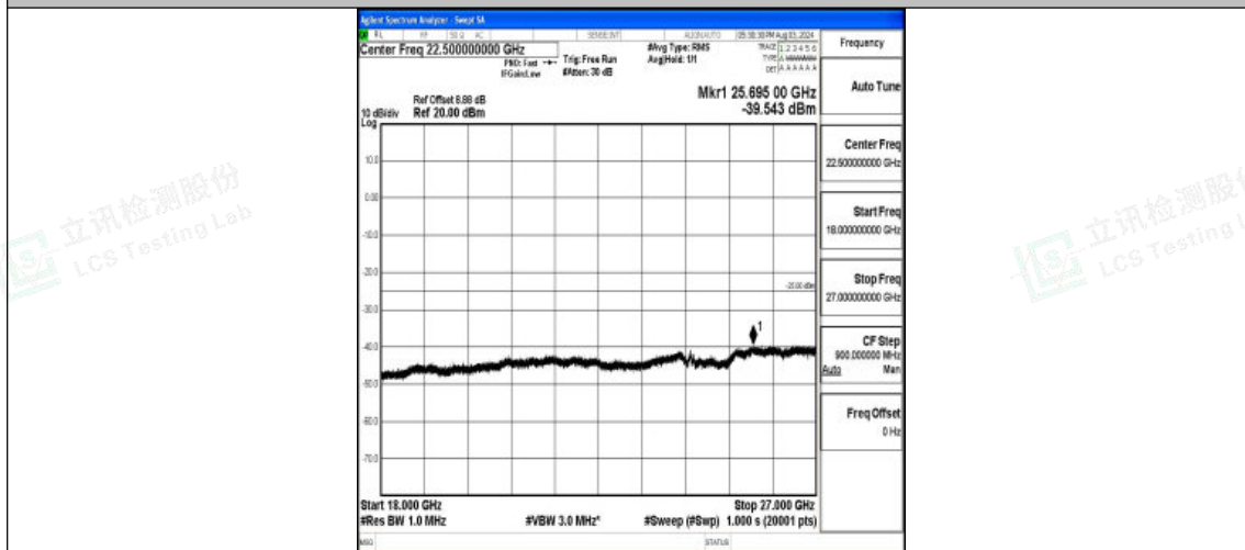
Band7-10MHz-16QAM-20800-1RB#0-18000~27000-PASS
