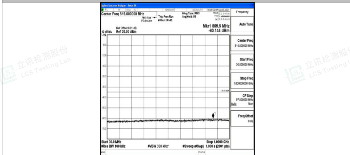
Band7-20MHz-16QAM-20850-1RB#0-30~1000-PASS
