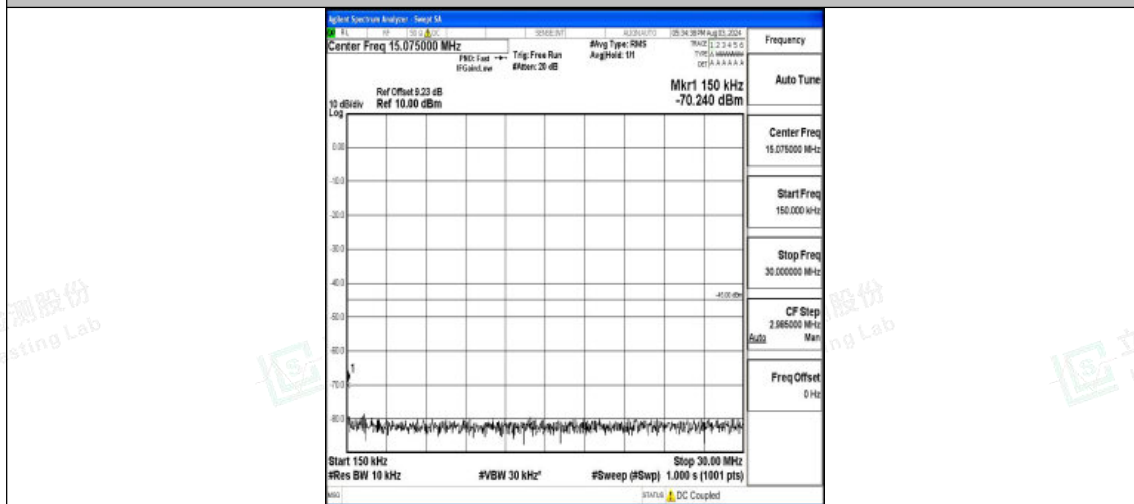
Band7-10MHz-16QAM-21400-1RB#0-0.15~30-PASS
