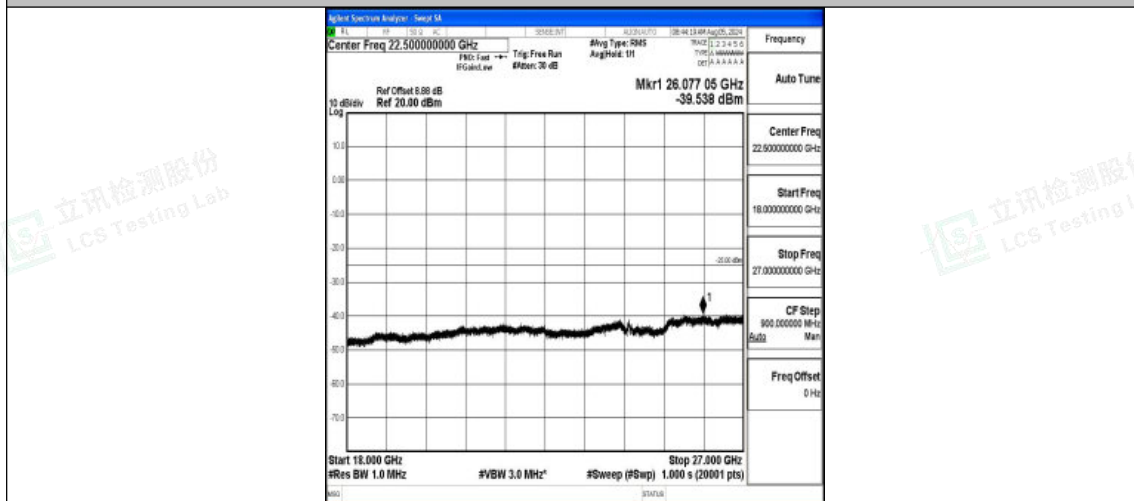
Band7-15MHz-QPSK-21375-1RB#0-18000~27000-PASS
