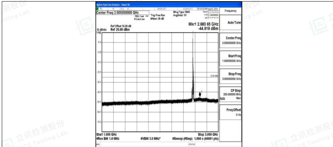
Band7-10MHz-QPSK-21400-1RB#0-1000~3000-PASS
