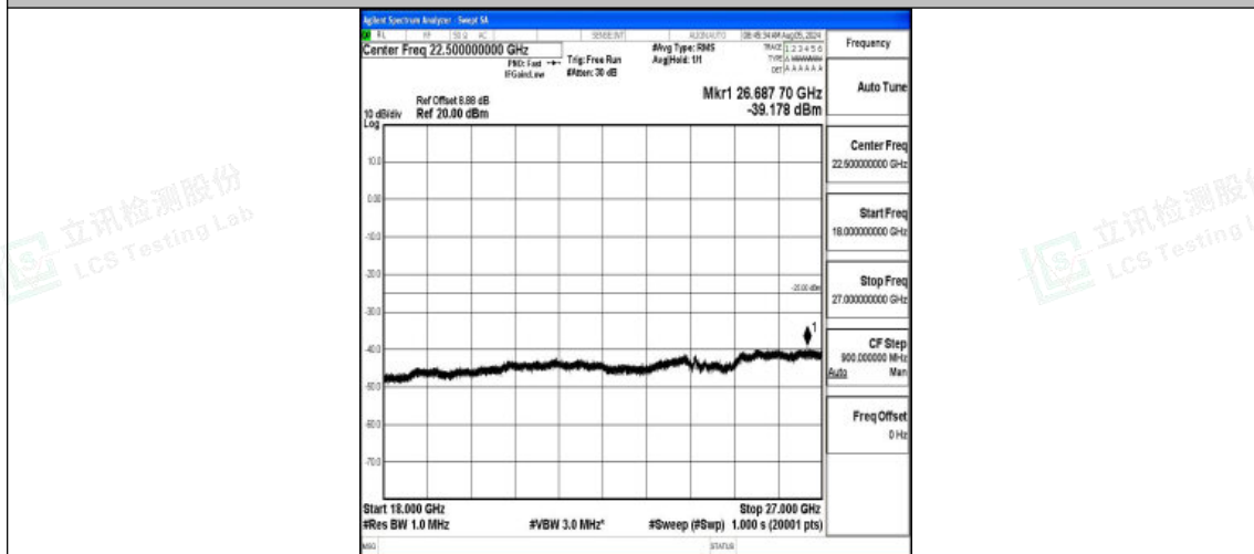
Band7-15MHz-16QAM-21375-1RB#0-18000~27000-PASS
