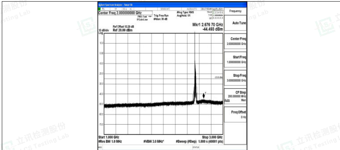
Band7-20MHz-16QAM-21100-1RB#0-1000~3000-PASS
