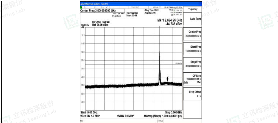
Band7-15MHz-16QAM-21100-1RB#0-1000~3000-PASS
