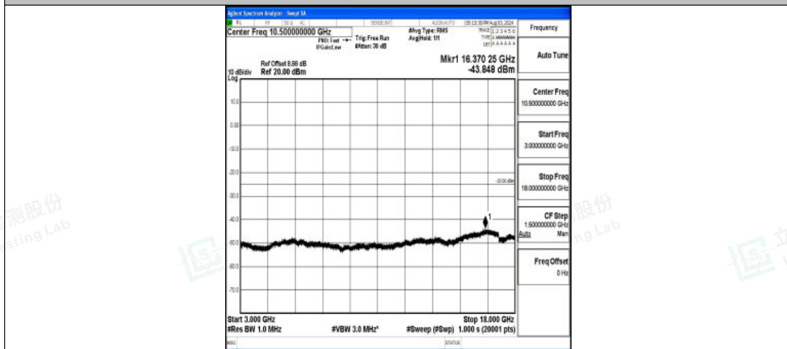
Band7-5MHz-QPSK-21425-1RB#0-3000~18000-PASS
