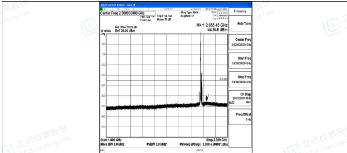
Band7-15MHz-QPSK-21375-1RB#0-1000~3000-PASS
