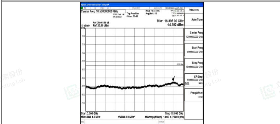
Band7-15MHz-16QAM-20825-1RB#0-3000~18000-PASS
