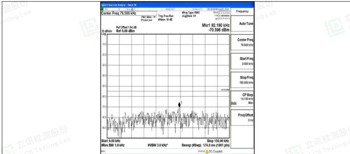
Band7-10MHz-QPSK-20800-1RB#0-0.009~0.15-PASS
