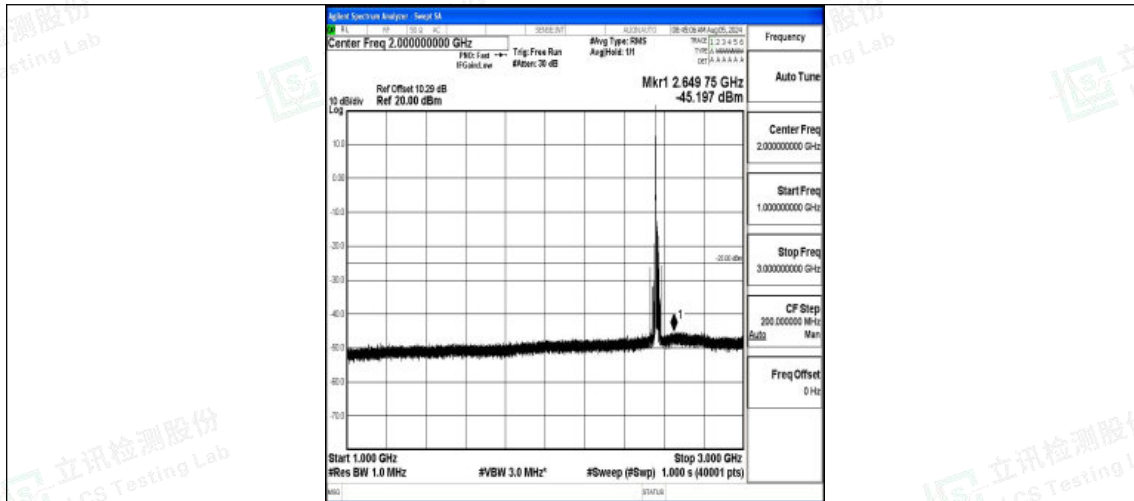
Band7-15MHz-16QAM-21375-1RB#0-1000~3000-PASS
