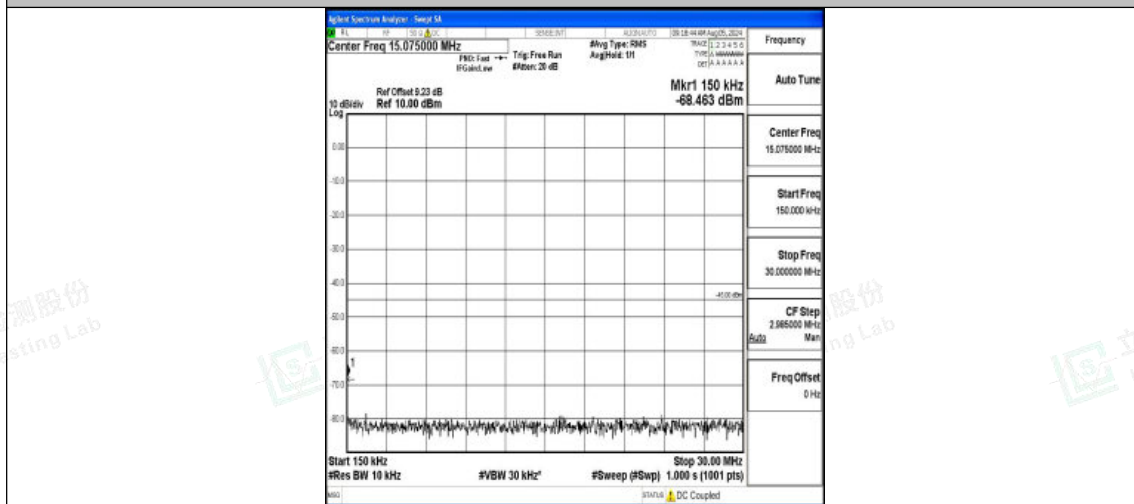
Band7-20MHz-QPSK-21350-1RB#0-0.15~30-PASS
