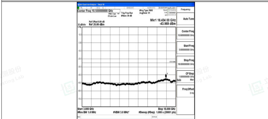
Band7-15MHz-QPSK-20825-1RB#0-3000~18000-PASS
