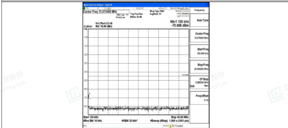
Band7-20MHz-QPSK-20850-1RB#0-0.15~30-PASS
