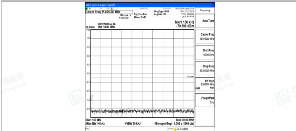
Band7-15MHz-QPSK-21375-1RB#0-0.15~30-PASS
