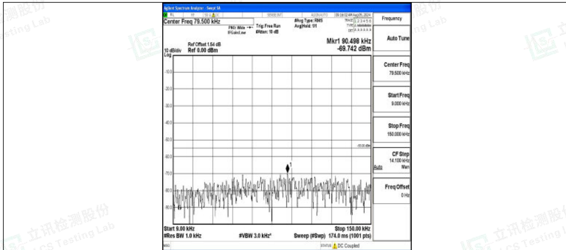
Band7-20MHz-QPSK-21100-1RB#0-0.009~0.15-PASS
