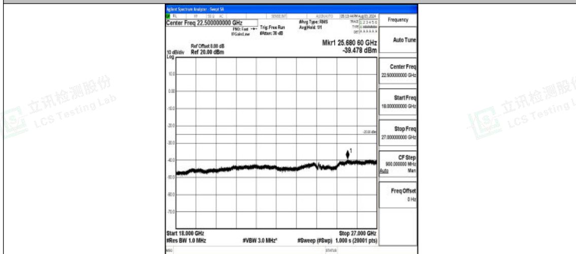
Band7-5MHz-QPSK-21425-1RB#0-18000~27000-PASS
