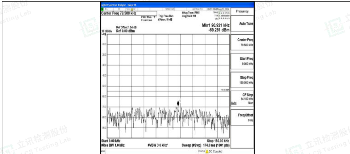
Band7-20MHz-16QAM-21100-1RB#0-0.009~0.15-PASS
