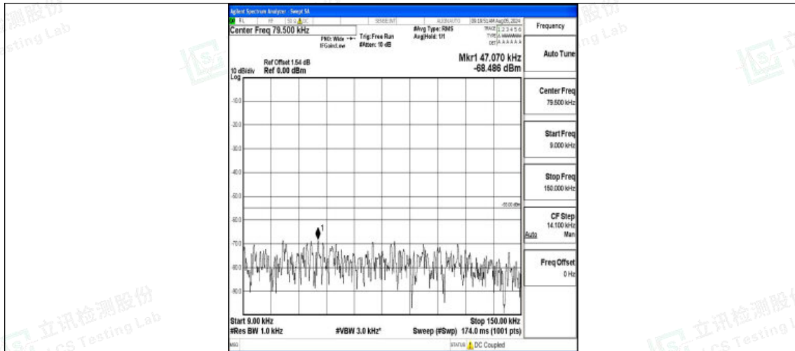
Band7-20MHz-16QAM-21350-1RB#0-0.009~0.15-PASS
