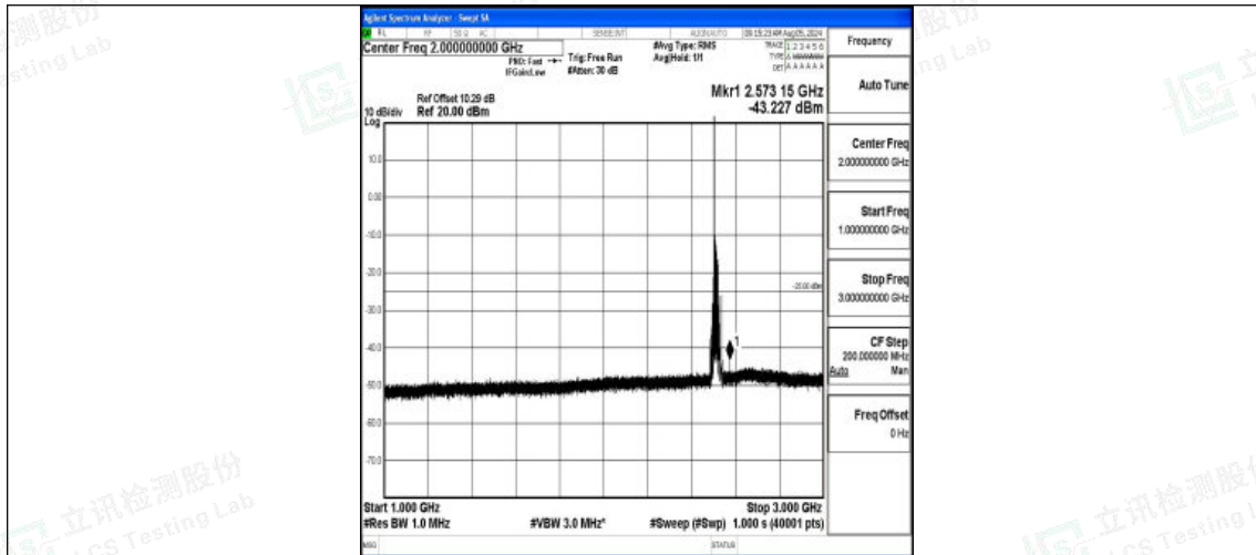
Band7-20MHz-16QAM-20850-1RB#0-1000~3000-PASS
