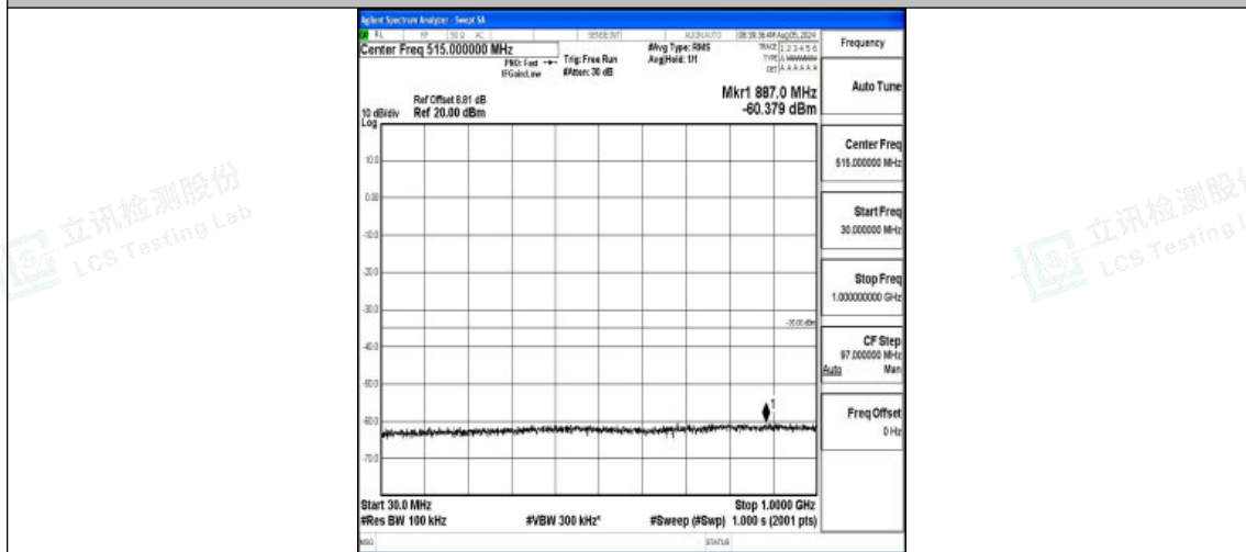
Band7-15MHz-16QAM-20825-1RB#0-30~1000-PASS
