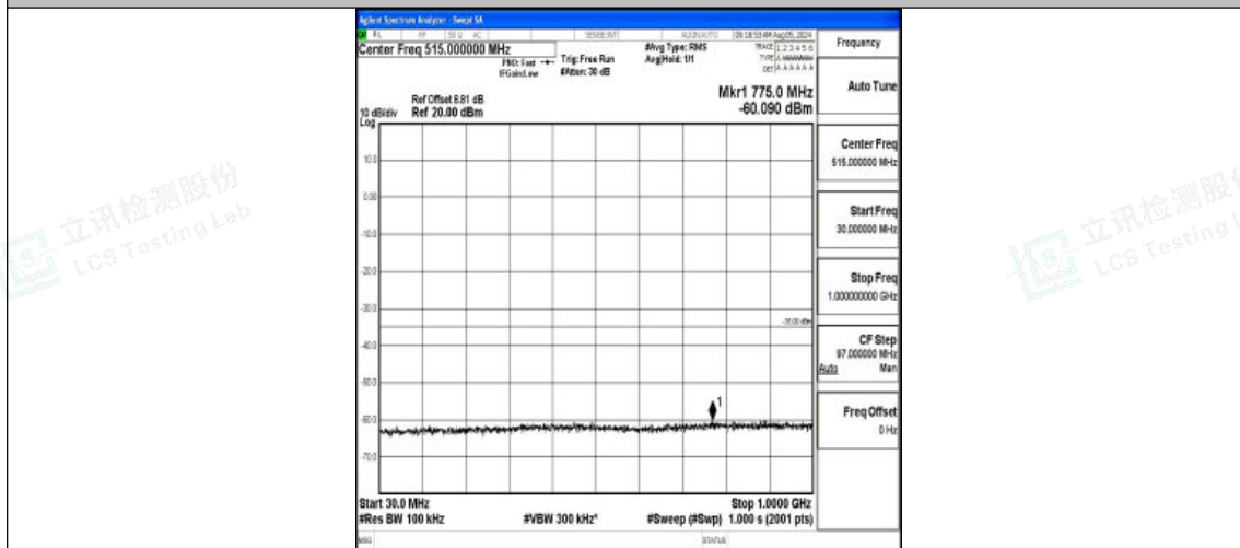
Band7-20MHz-QPSK-21350-1RB#0-30~1000-PASS
