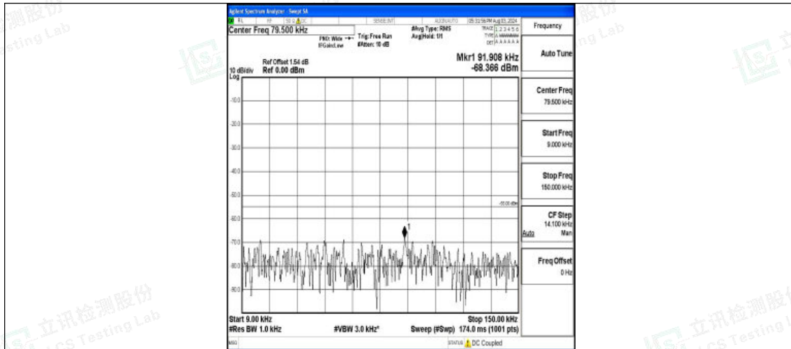
Band7-10MHz-16QAM-21100-1RB#0-0.009~0.15-PASS
