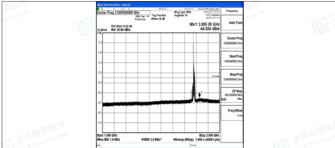
Band7-20MHz-16QAM-21350-1RB#0-1000~3000-PASS
