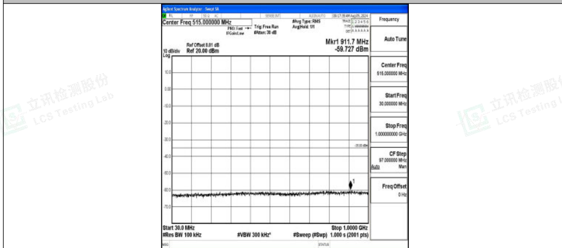
Band7-20MHz-16QAM-21100-1RB#0-30~1000-PASS
