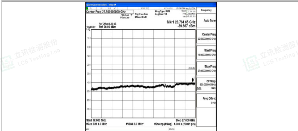
Band7-10MHz-QPSK-20800-1RB#0-18000~27000-PASS
