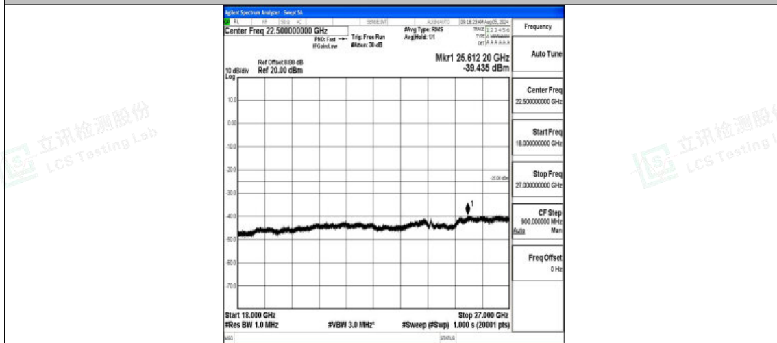
Band7-20MHz-16QAM-21100-1RB#0-18000~27000-PASS
