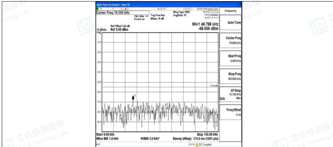
Band7-15MHz-16QAM-21375-1RB#0-0.009~0.15-PASS
