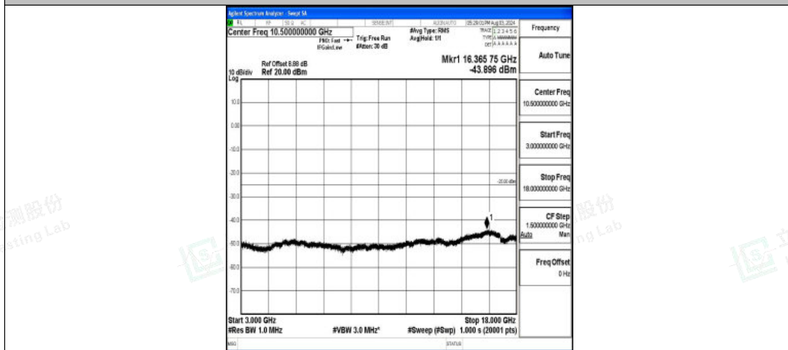
Band7-10MHz-QPSK-20800-1RB#0-3000~18000-PASS
