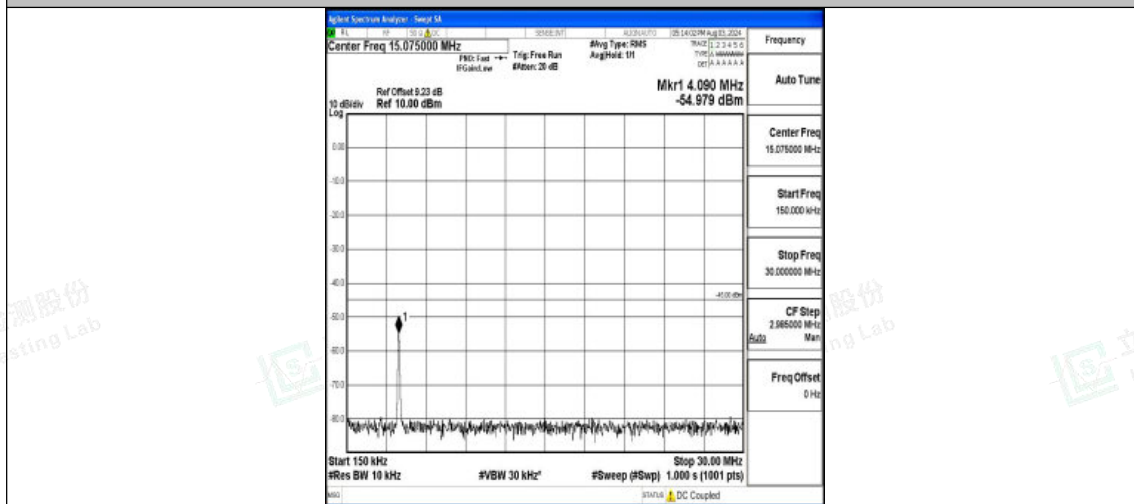
Band7-5MHz-16QAM-21425-1RB#0-0.15~30-PASS
