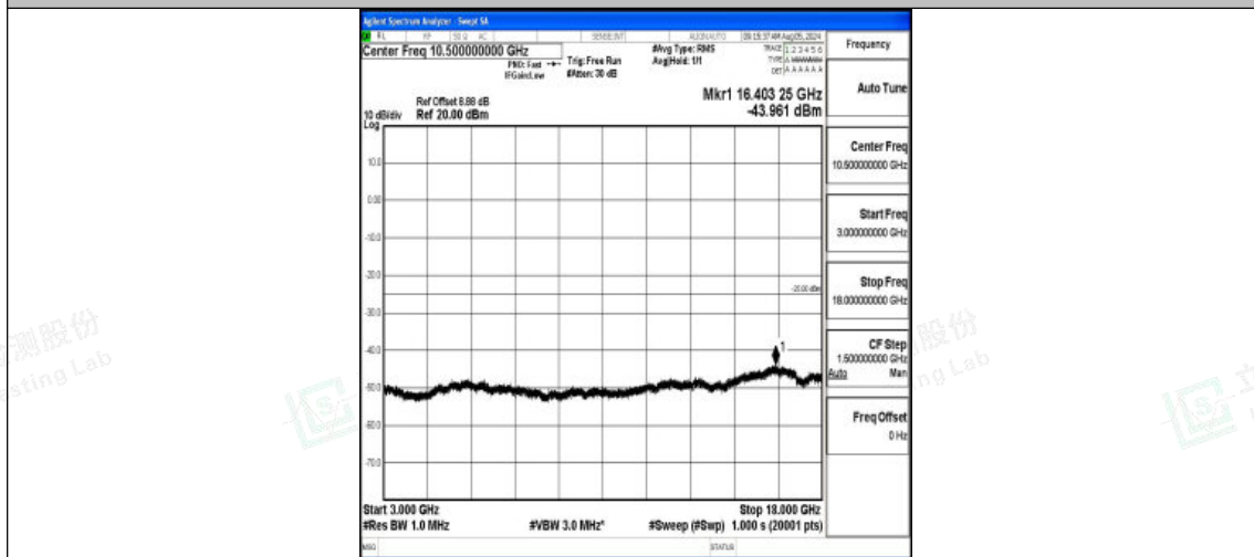
Band7-20MHz-16QAM-20850-1RB#0-3000~18000-PASS
