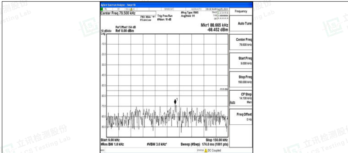
Band7-20MHz-QPSK-21350-1RB#0-0.009~0.15-PASS
