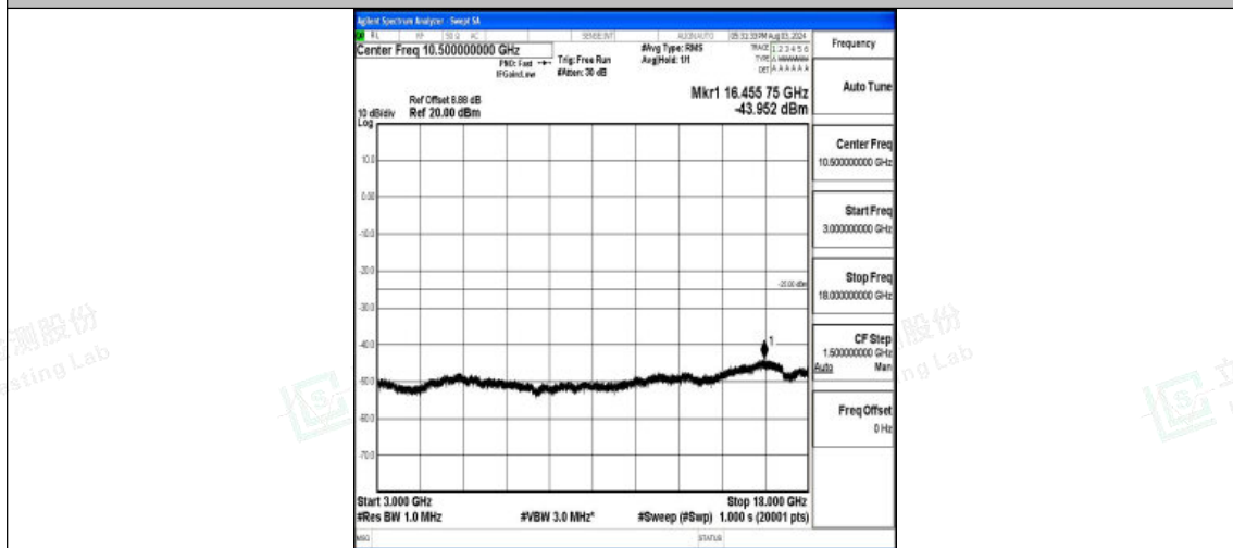
Band7-10MHz-QPSK-21100-1RB#0-3000~18000-PASS
