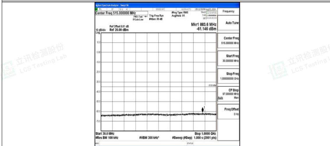
Band7-5MHz-QPSK-21425-1RB#0-30~1000-PASS
