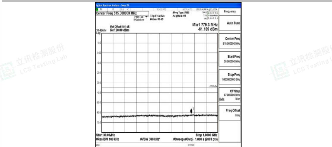
Band7-10MHz-16QAM-20800-1RB#0-30~1000-PASS
