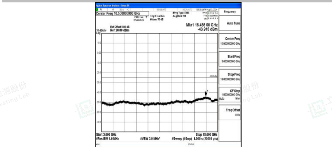
Band7-10MHz-16QAM-20800-1RB#0-3000~18000-PASS
