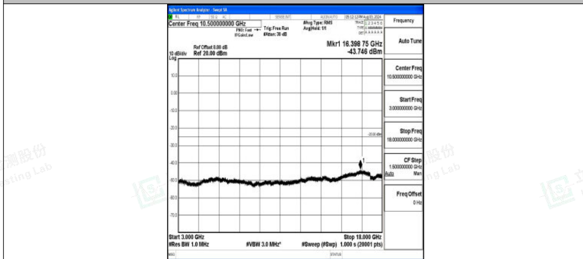
Band7-5MHz-16QAM-21100-1RB#0-3000~18000-PASS
