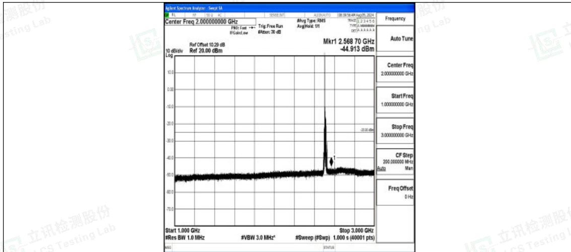
Band7-15MHz-16QAM-20825-1RB#0-1000~3000-PASS
