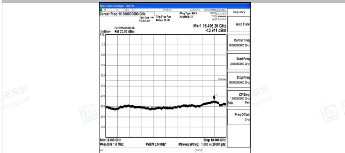
Band7-10MHz-QPSK-21400-1RB#0-3000~18000-PASS
