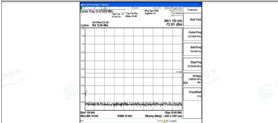
Band7-10MHz-QPSK-20800-1RB#0-0.15~30-PASS
