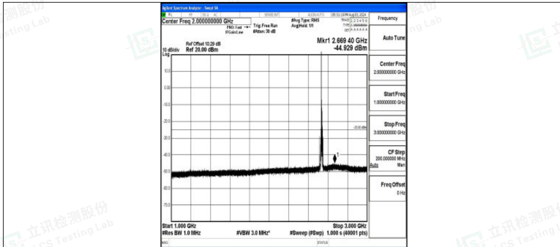
Band7-10MHz-QPSK-21100-1RB#0-1000~3000-PASS
