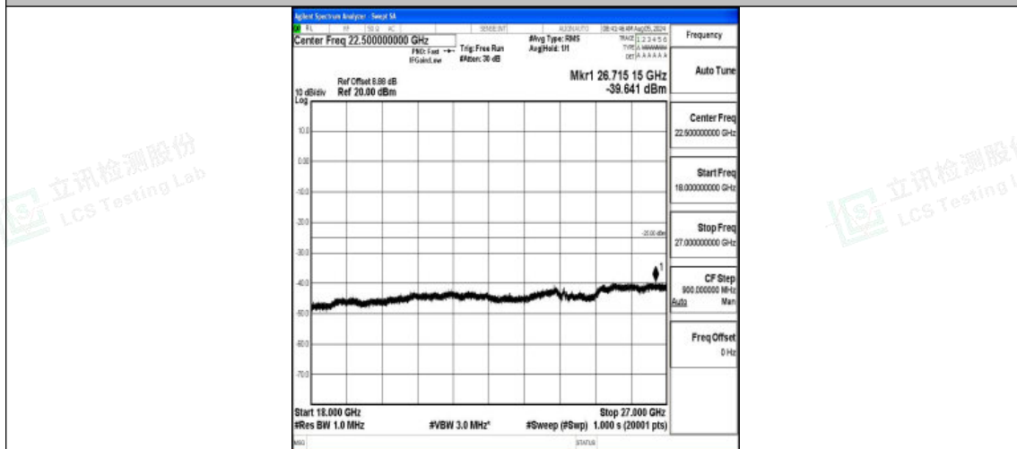
Band7-15MHz-QPSK-21100-1RB#0-18000~27000-PASS
