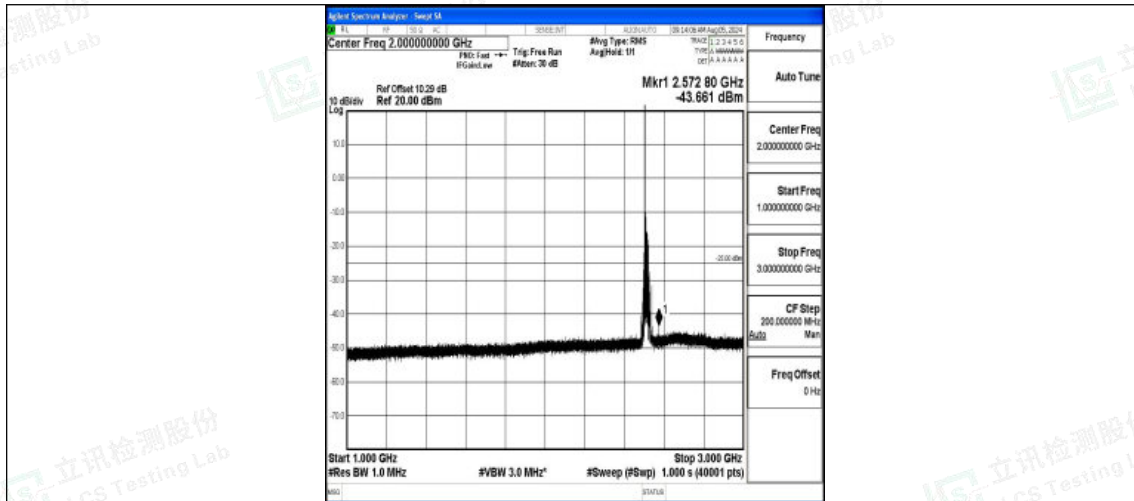
Band7-20MHz-QPSK-20850-1RB#0-1000~3000-PASS
