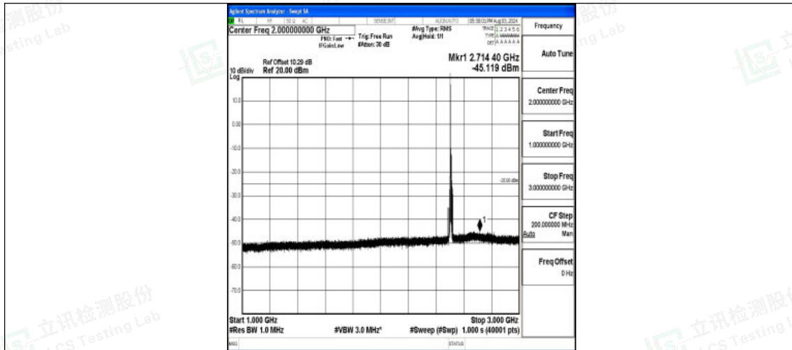
Band7-10MHz-16QAM-20800-1RB#0-1000~3000-PASS
