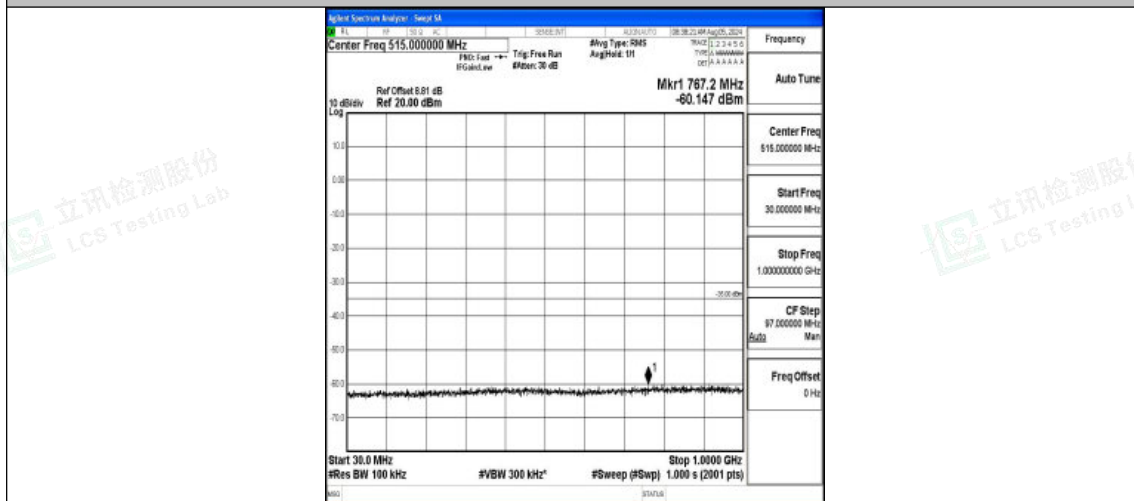
Band7-15MHz-QPSK-20825-1RB#0-30~1000-PASS
