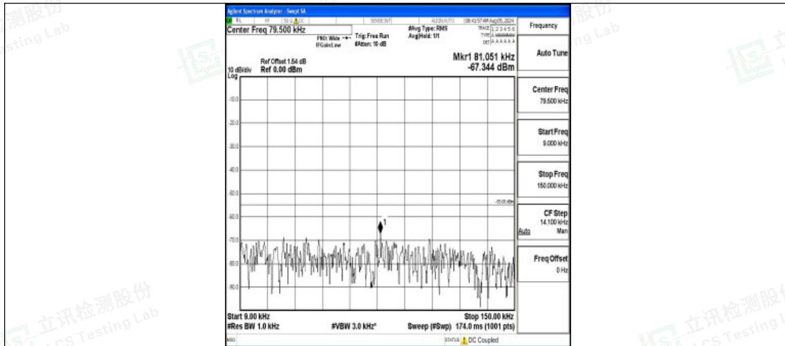
Band7-15MHz-16QAM-21100-1RB#0-0.009~0.15-PASS
