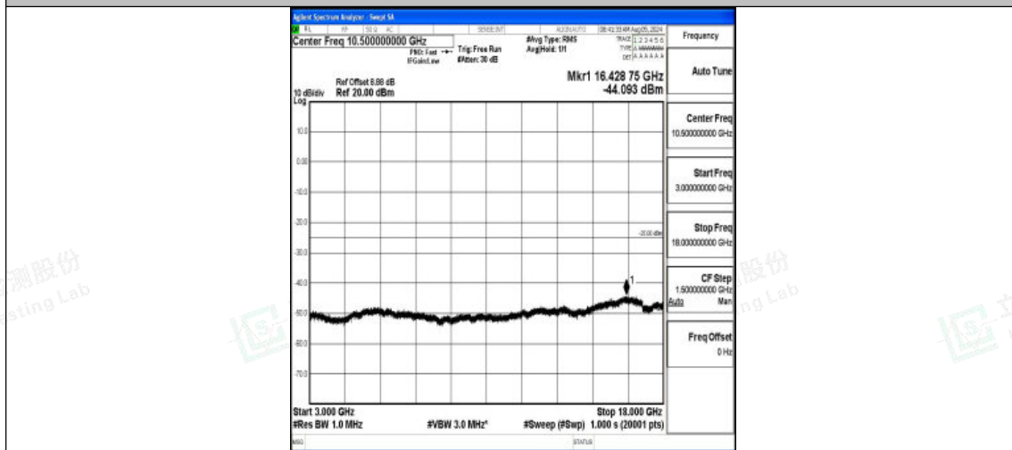
Band7-15MHz-QPSK-21100-1RB#0-3000~18000-PASS
