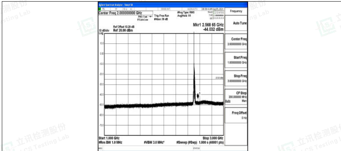
Band7-15MHz-QPSK-20825-1RB#0-1000~3000-PASS
