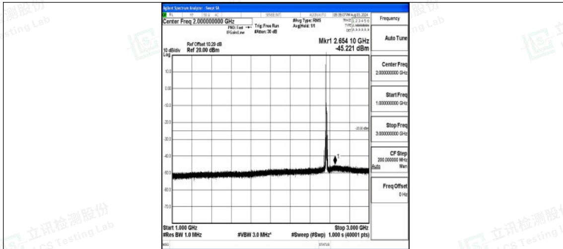
Band7-10MHz-16QAM-21400-1RB#0-1000~3000-PASS
