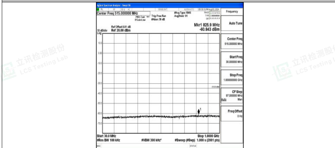
Band7-10MHz-QPSK-21400-1RB#0-30~1000-PASS
