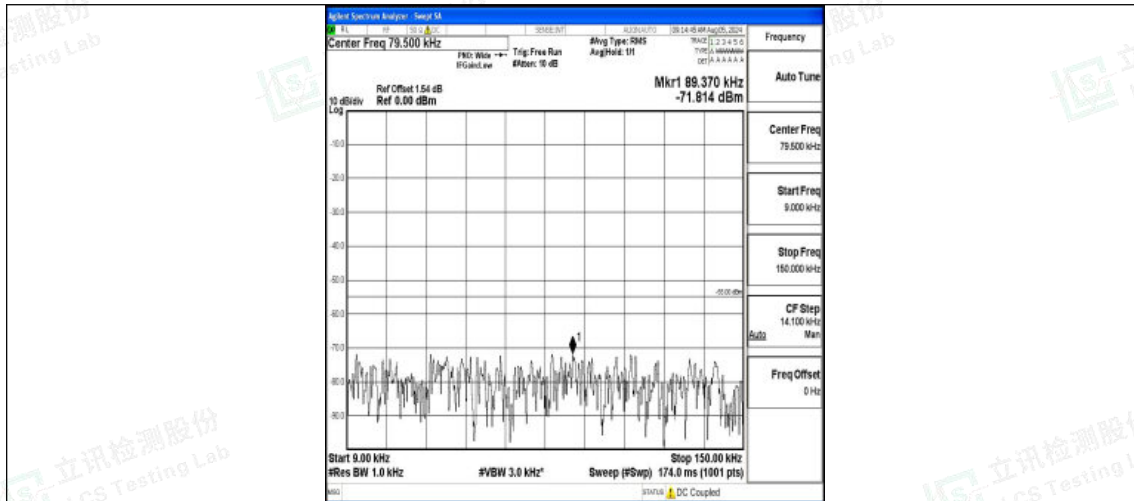
Band7-20MHz-16QAM-20850-1RB#0-0.009~0.15-PASS
