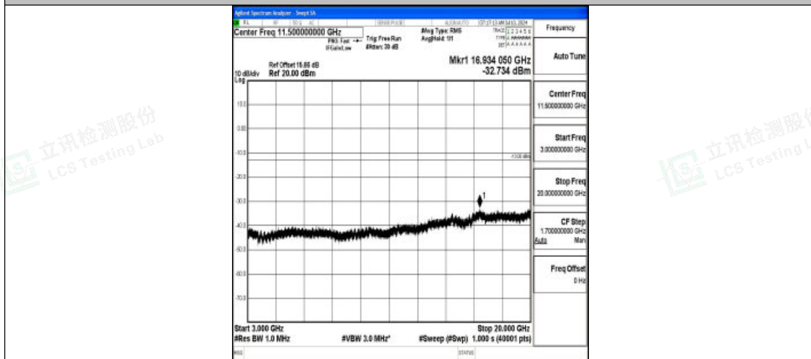
Band2_15MHz_16QAM_18675_1RB#0_3000~20000_3000~20000
