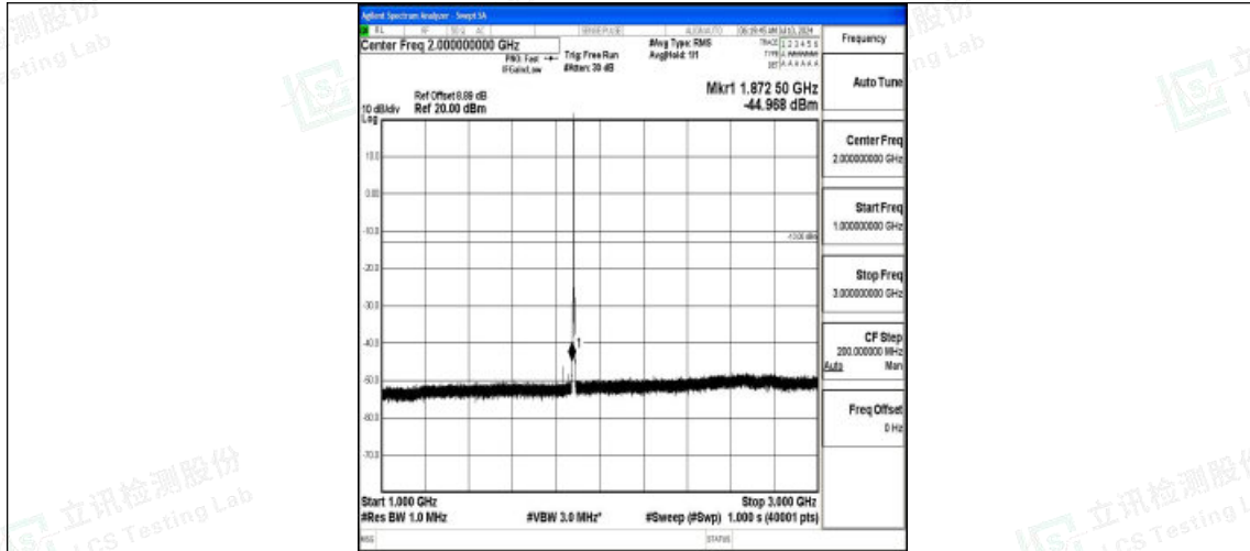
Band2_3MHz_QPSK_18900_1RB#0_1000~3000_1000~3000
