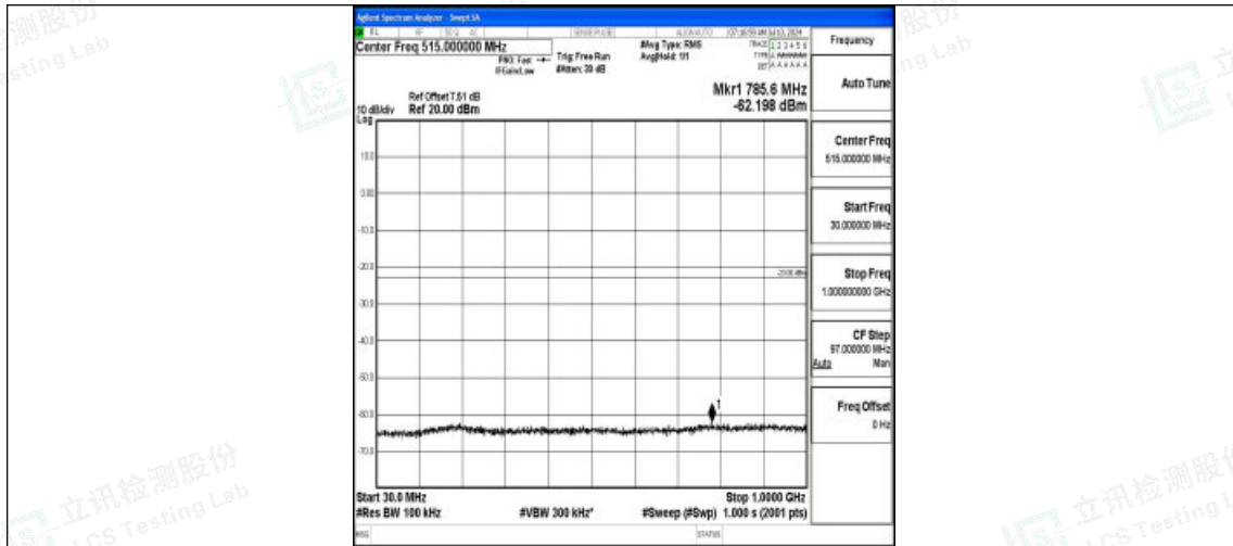
Band2_15MHz_16QAM_18675_1RB#0_30~1000_30~1000
