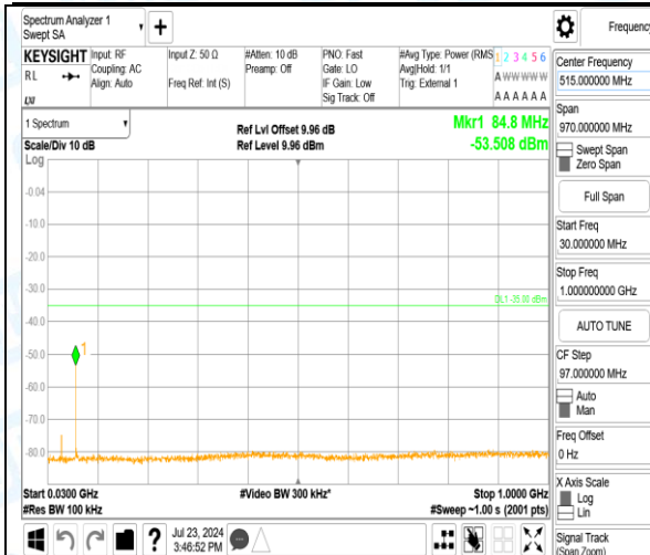
Band41_10MHz_QPSK_41190_1RB#0_20000~27000_20000~27000
