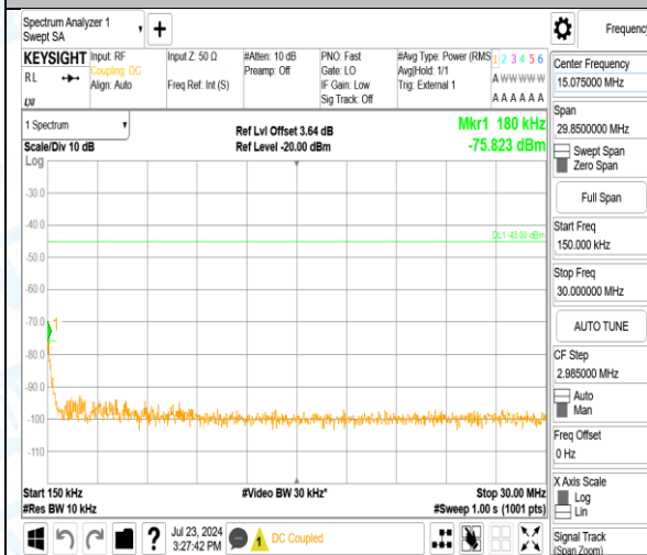
Band41_5MHz_16QAM_41215_1RB#0_1000~20000_1000~20000
