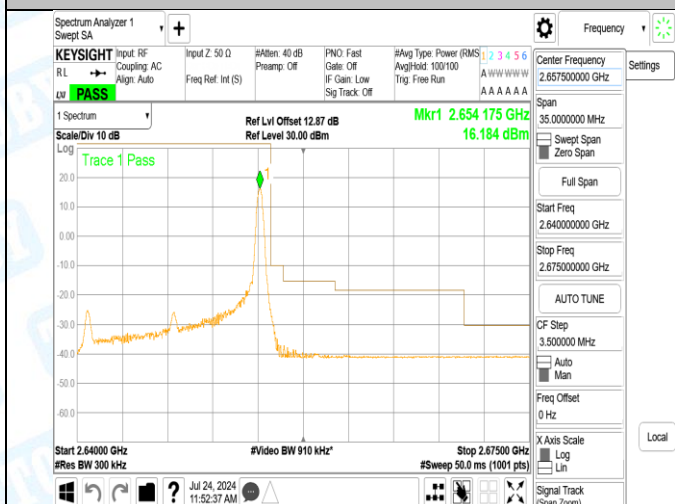
Band41_15MHz_16QAM_40315_1RB#0
