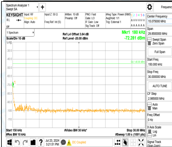
Band41_5MHz_QPSK_40690_1RB#0_1000~20000_1000~20000
