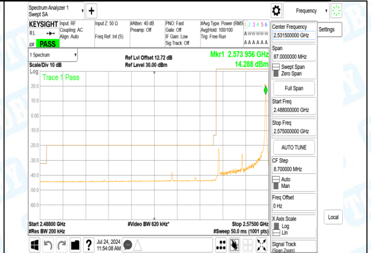
Band41_20MHz_QPSK_41140_1RB#0
