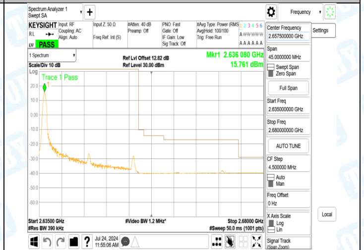
Band41_20MHz_QPSK_41140_100RB#0
