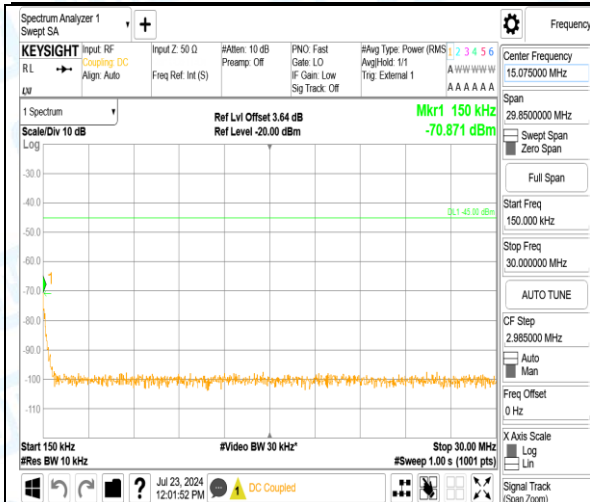
Band38_10MHz_QPSK_38000_1RB#0_1000~20000_1000~20000
