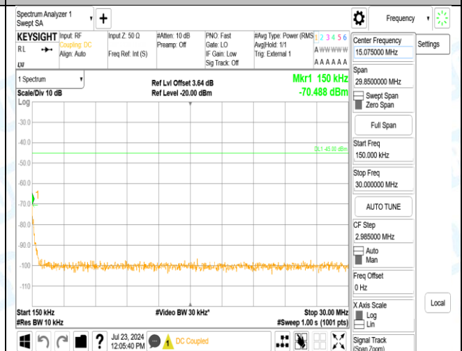
Band38_10MHz_QPSK_38200_1RB#0_1000~20000_1000~20000
