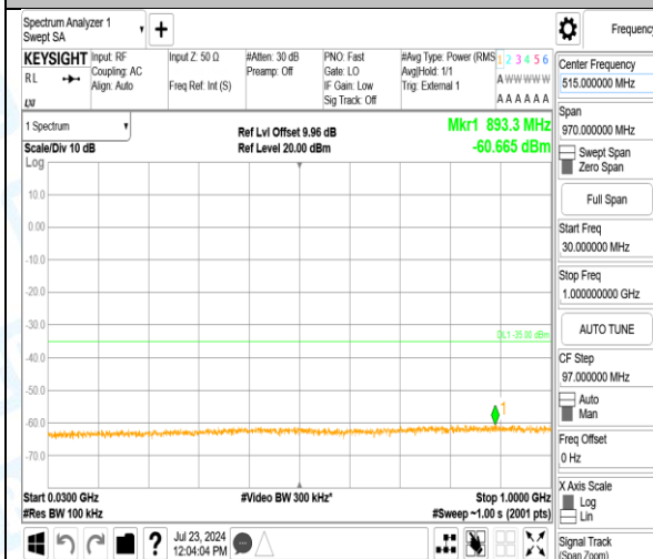
Band38_10MHz_16QAM_38000_1RB#0_20000~27000_20000~27000
