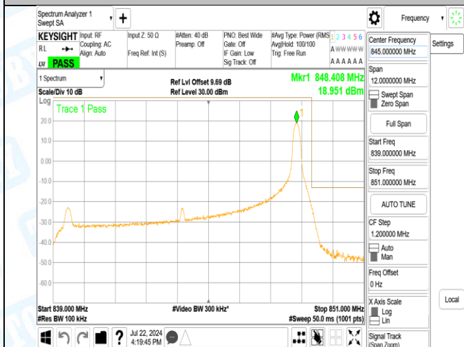
Band5_10MHz_16QAM_20600_1RB#49
