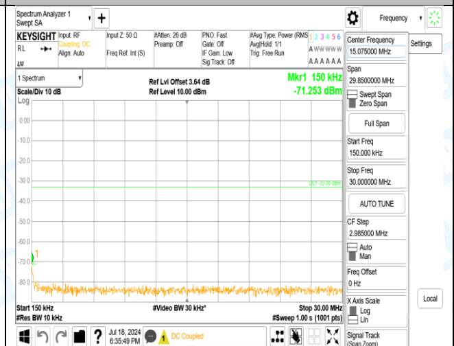
Band2_15MHz_QPSK_19125_1RB#0_1000~3000_1000~3000
