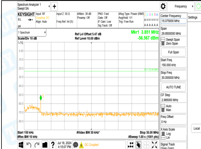
Band5-4233-3-0.15~30MHz-PASS
