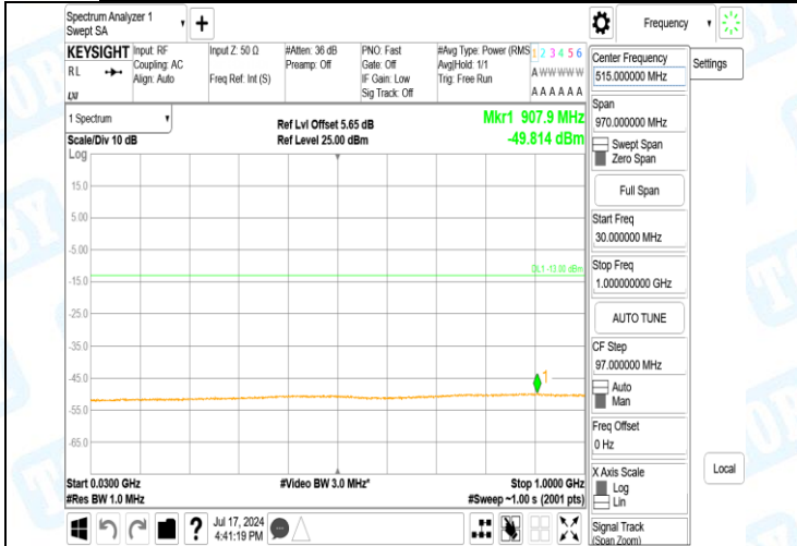
Band2-9262-5-30~1000MHz-PASS
