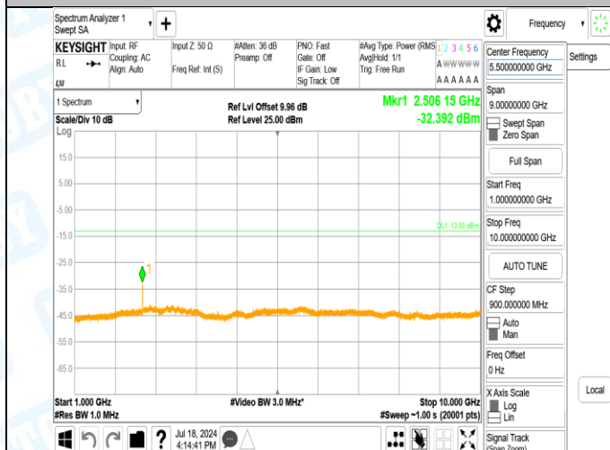
Band5-4182-3-1000~10000MHz-PASS
