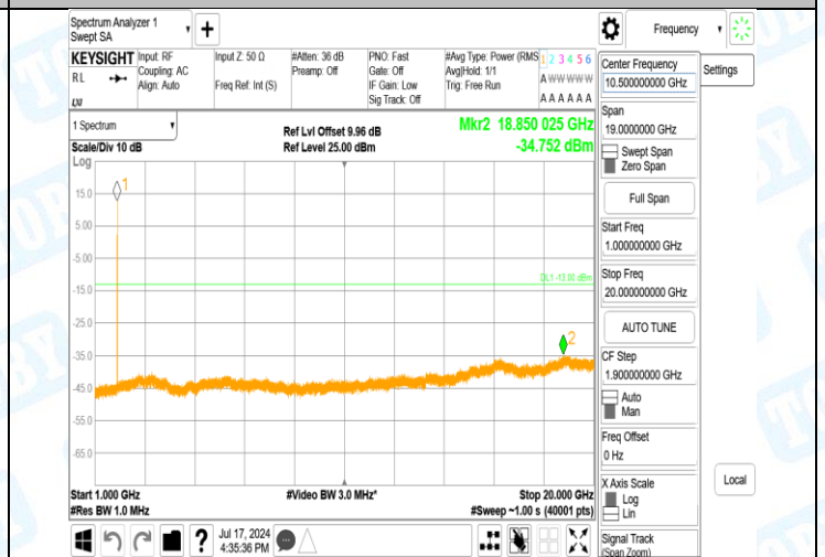
Band2-9262-3-1000~20000MHz-PASS
