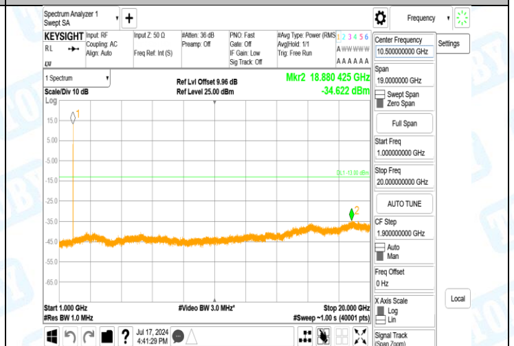
Band2-9262-5-1000~20000MHz-PASS
