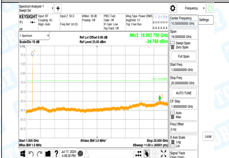
Band2-9262-4-1000~20000MHz-PASS
