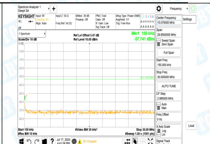
Band2-9262-5-0.15~30MHz-PASS
