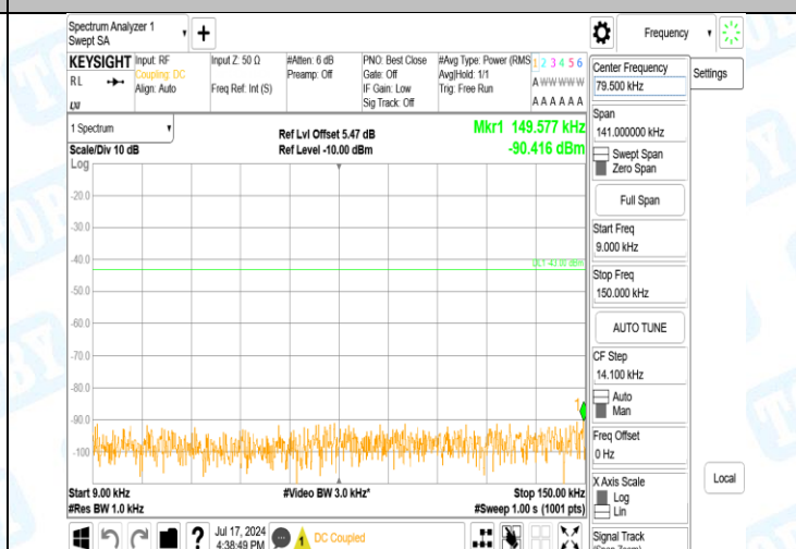
Band2-9400-4-0.009~0.15MHz-PASS
