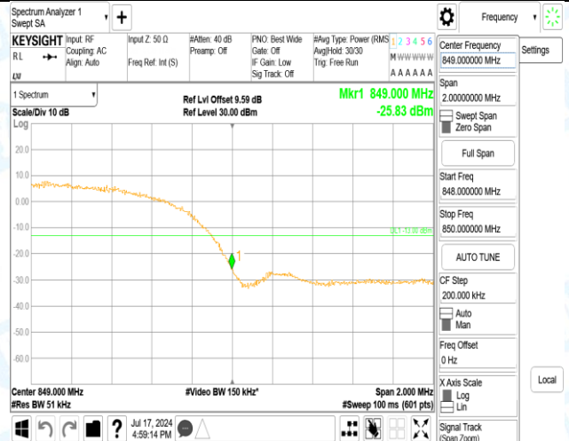
Band5-4233-PASS
