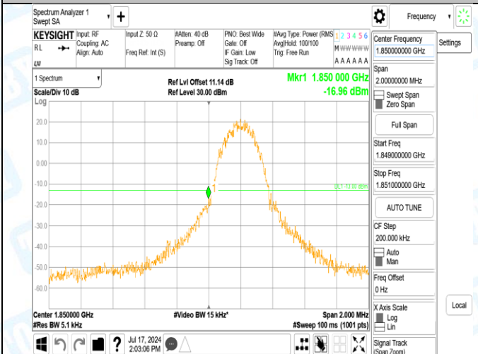
EGPRS1900-512-2-PASS
