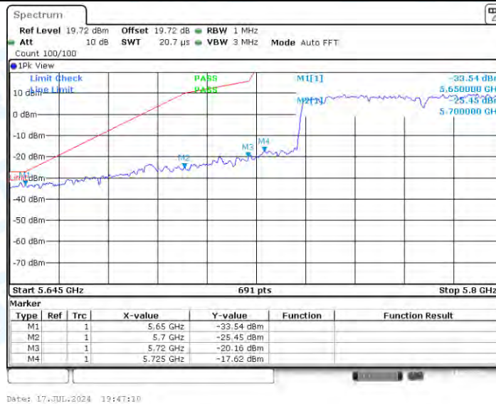
11AC80SISO_Ant1_High_5775_AV
