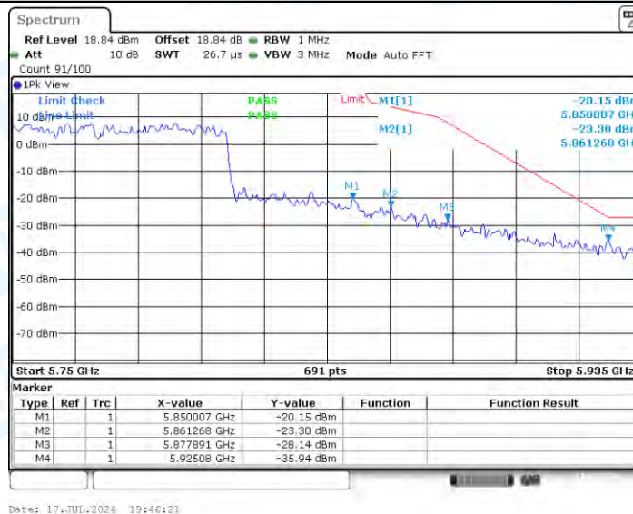
11AC80SISO_Ant1_High_5775
