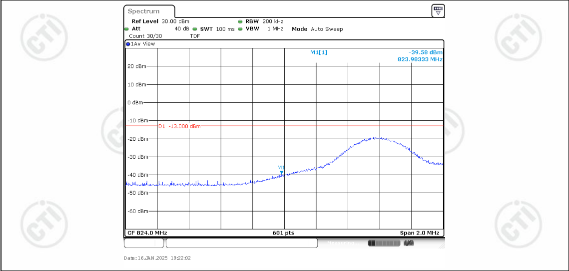
Band5-10MHz-16QAM-20450-1RB#49
