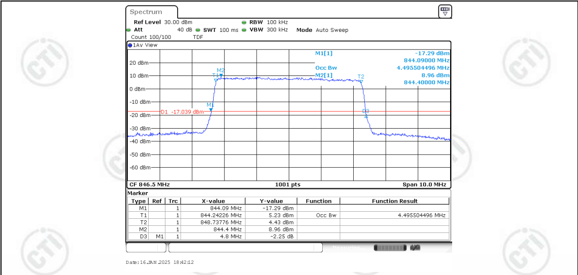
Band5-5MHz-QPSK-20625-25RB#0-4.496
