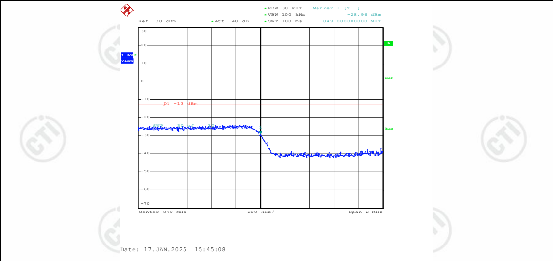
Band5-3MHz-16QAM-20635-1RB#0
