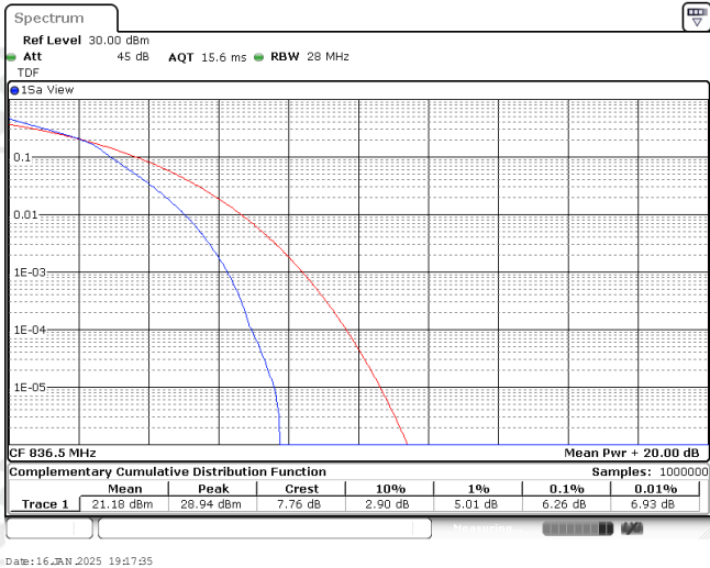
Band5-5MHz-16QAM-20525-25RB#0
