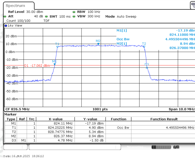
Band5-5MHz-QPSK-20425-25RB#0-4.496
