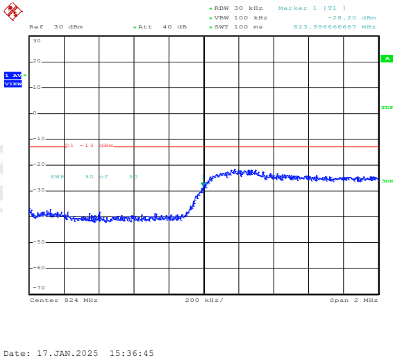
Band5-3MHz-QPSK-20415-1RB#14
