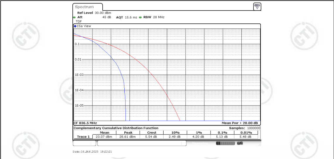
Band5-1.4MHz-QPSK-20525-1RB#0
