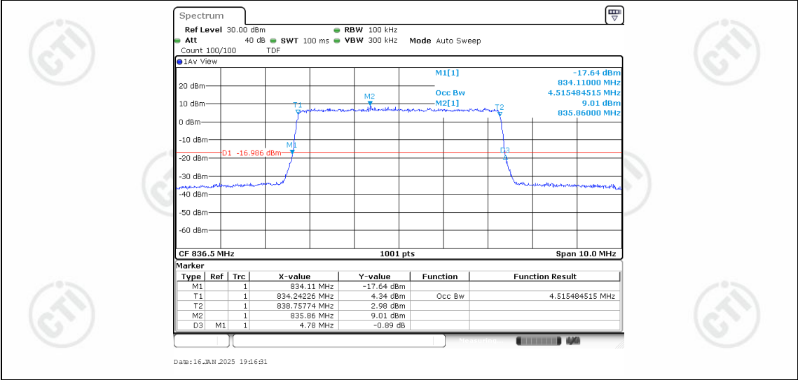
Band5-5MHz-16QAM-20525-25RB#0-4.515
