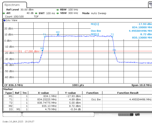
Band5-5MHz-QPSK-20525-25RB#0-4.496
