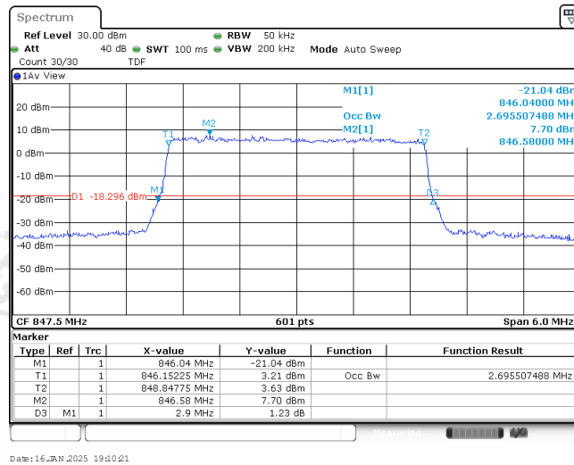
Band5-3MHz-16QAM-20635-15RB#0-2.696
