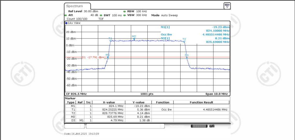
Band5-5MHz-16QAM-20425-25RB#0-4.486
