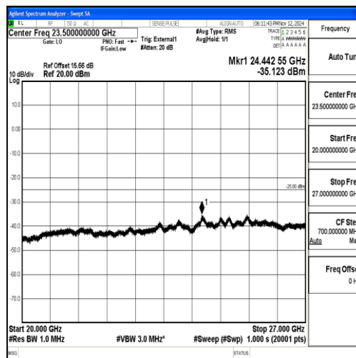
Band38_15MHz_16QAM_38000_1RB#0_20000~27000_20000~27000
