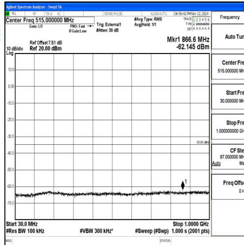
Band38_20MHz_16QAM_38000_1RB#0_30~1000_30~1000
