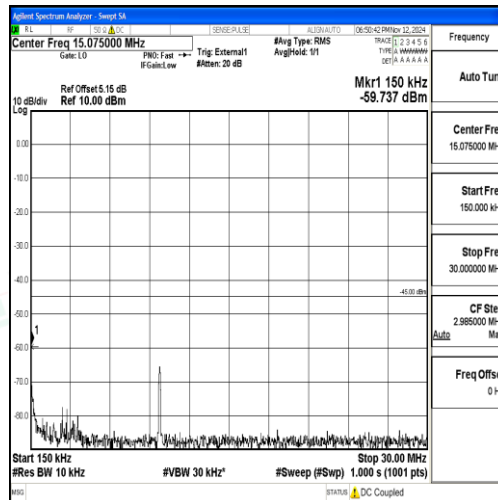
Band38_20MHz_QPSK_37850_1RB#0_0.15~30_0.15~30
