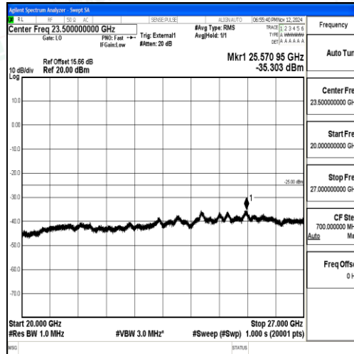
Band38_20MHz_QPSK_38000_1RB#0_20000~27000_20000~27000
