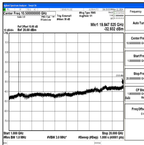
Band38_15MHz_16QAM_38175_1RB#0_1000~20000_1000~20000
