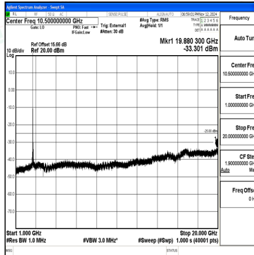
Band38_20MHz_QPSK_38150_1RB#0_1000~20000_1000~20000
