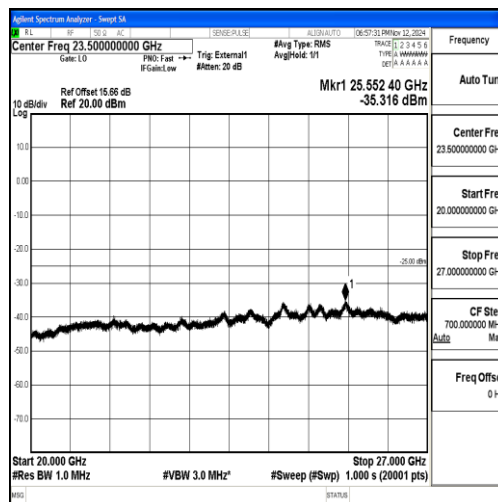
Band38_20MHz_16QAM_38000_1RB#0_20000~27000_20000~27000
