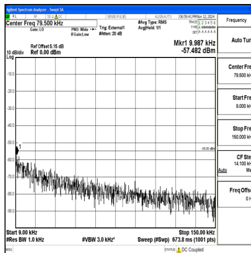
Band38_20MHz_16QAM_38150_1RB#0_0.009~0.15_0.009~0.15
