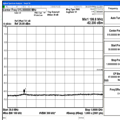
Band38_15MHz_16QAM_38000_1RB#0_30~1000_30~1000
