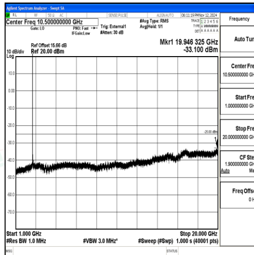
Band38_15MHz_16QAM_38000_1RB#0_1000~20000_1000~20000
