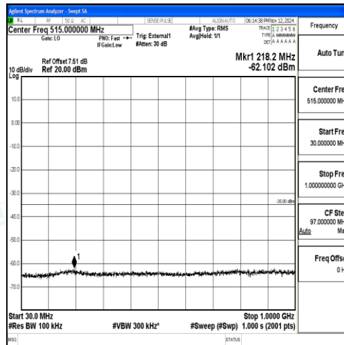
Band38_15MHz_16QAM_38175_1RB#0_30~1000_30~1000
