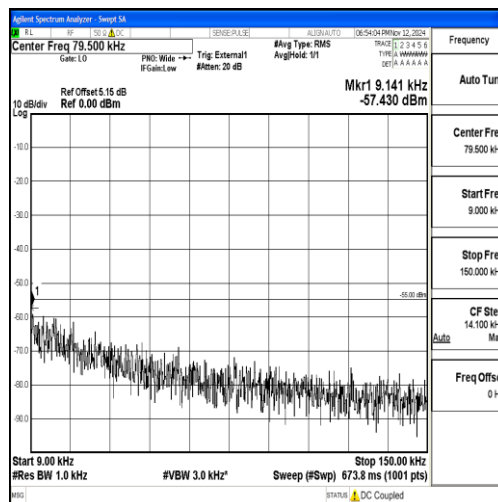
Band38_20MHz_QPSK_38000_1RB#0_0.009~0.15_0.009~0.15
