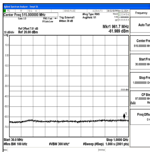
Band38_20MHz_16QAM_37850_1RB#0_30~1000_30~1000
