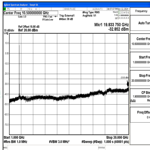
Band38_20MHz_16QAM_38000_1RB#0_1000~20000_1000~20000
