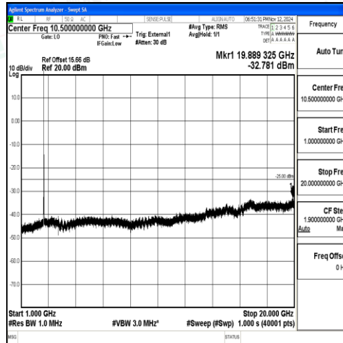
Band38_20MHz_QPSK_37850_1RB#0_1000~20000_1000~20000
