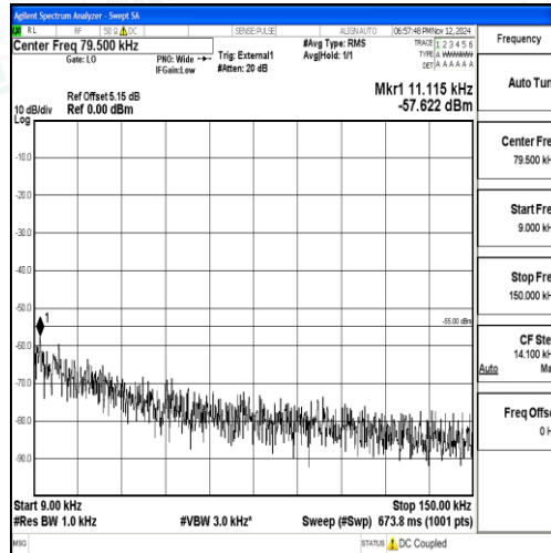
Band38_20MHz_QPSK_38150_1RB#0_0.009~0.15_0.009~0.15
