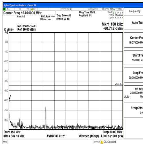
Band38_20MHz_16QAM_37850_1RB#0_0.15~30_0.15~30
