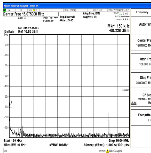
Band38_20MHz_16QAM_38000_1RB#0_0.15~30_0.15~30
