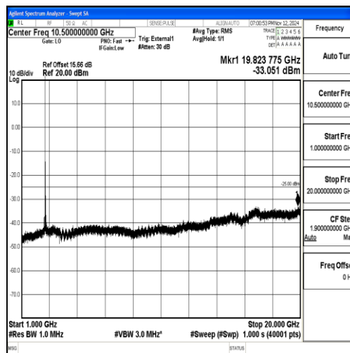
Band38_20MHz_16QAM_38150_1RB#0_1000~20000_1000~20000
