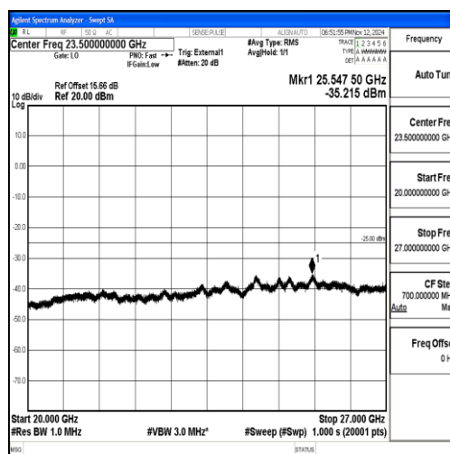
Band38_20MHz_QPSK_37850_1RB#0_20000~27000_20000~27000
