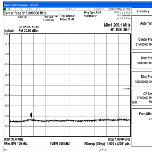
Band38_20MHz_16QAM_38150_1RB#0_30~1000_30~1000
