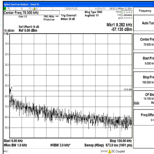
Band38_20MHz_16QAM_37850_1RB#0_0.009~0.15_0.009~0.15
