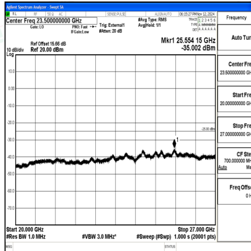
Band38_15MHz_16QAM_38175_1RB#0_20000~27000_20000~27000
