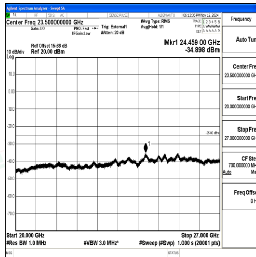
Band38_15MHz_QPSK_38175_1RB#0_20000~27000_20000~27000
