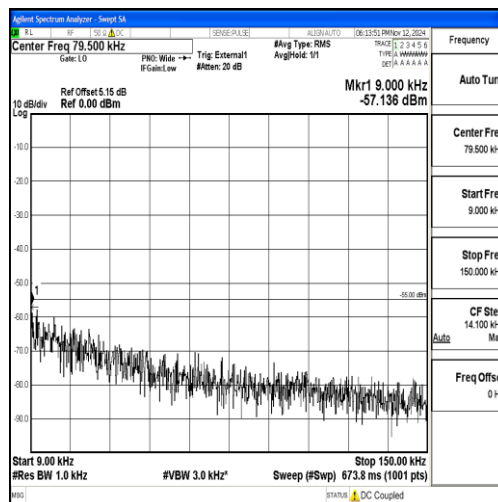
Band38_15MHz_16QAM_38175_1RB#0_0.009~0.15_0.009~0.15
