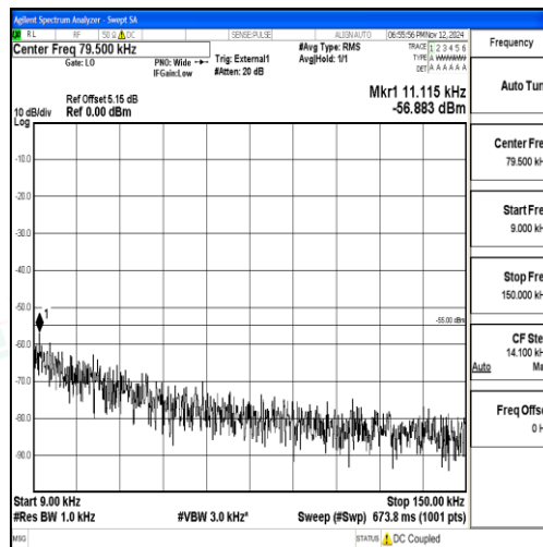
Band38_20MHz_16QAM_38000_1RB#0_0.009~0.15_0.009~0.15
