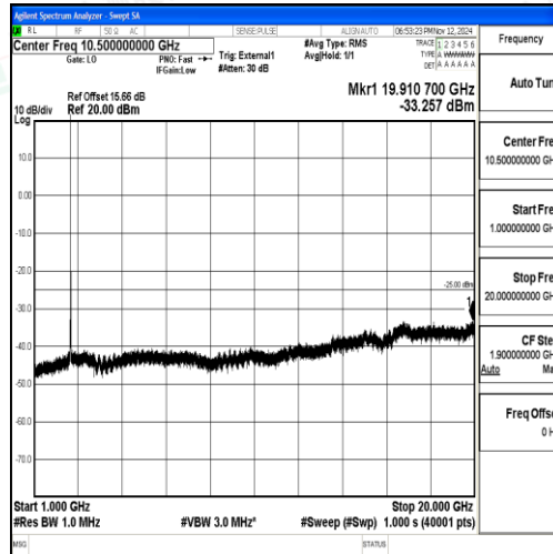
Band38_20MHz_16QAM_37850_1RB#0_1000~20000_1000~20000
