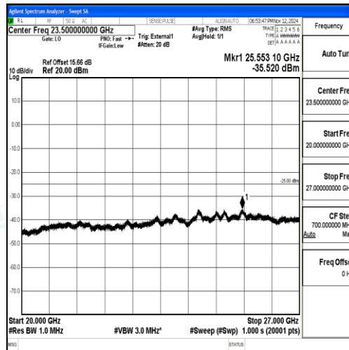
Band38_20MHz_16QAM_37850_1RB#0_20000~27000_20000~27000
