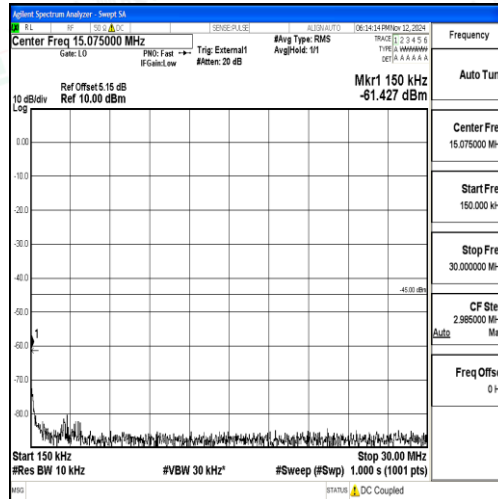
Band38_15MHz_16QAM_38175_1RB#0_0.15~30_0.15~30
