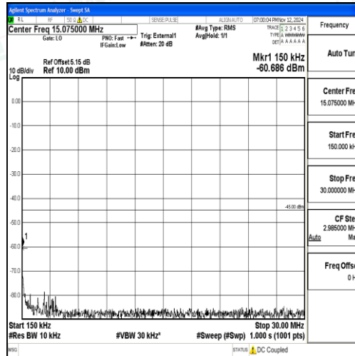
Band38_20MHz_16QAM_38150_1RB#0_0.15~30_0.15~30
