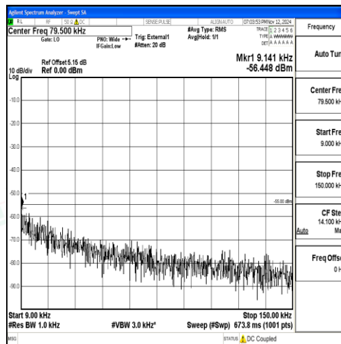
Band38_20MHz_QPSK_37850_1RB#0_0.009~0.15_0.009~0.15
