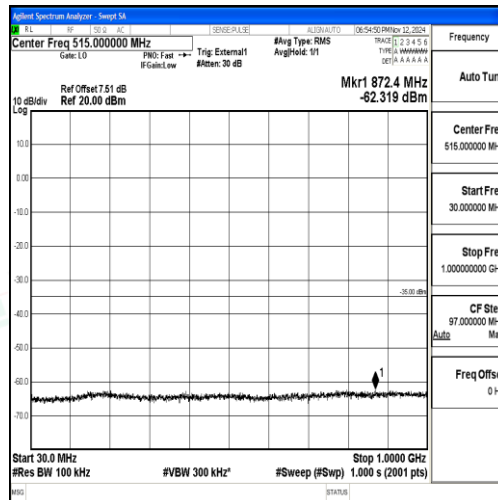
Band38_20MHz_QPSK_38000_1RB#0_30~1000_30~1000
