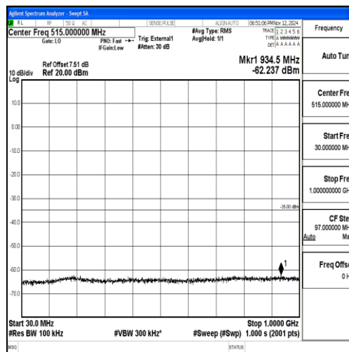
Band38_20MHz_QPSK_37850_1RB#0_30~1000_30~1000
