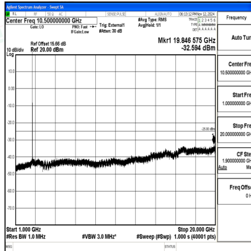
Band38_15MHz_QPSK_38175_1RB#0_1000~20000_1000~20000
