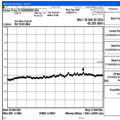
Band38_20MHz_QPSK_38150_1RB#0_20000~27000_20000~27000
