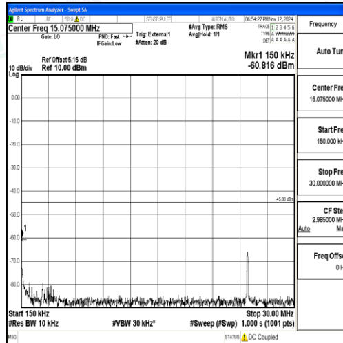
Band38_20MHz_QPSK_38000_1RB#0_0.15~30_0.15~30
