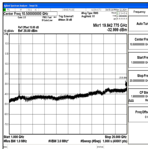
Band38_20MHz_QPSK_38000_1RB#0_1000~20000_1000~20000
