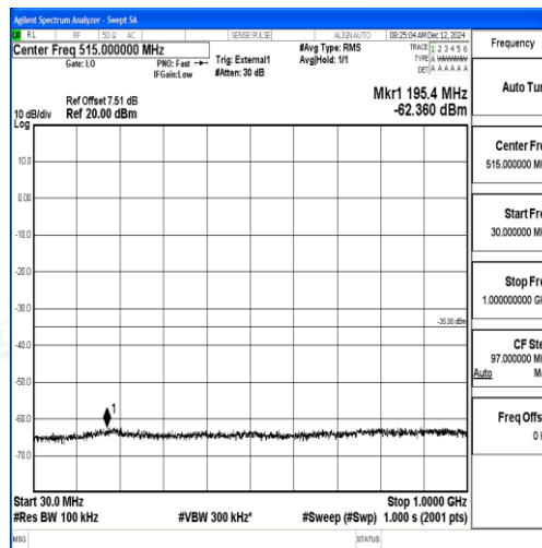
Band38_5MHz_QPSK_38000_1RB#0_30~1000_30~1000
