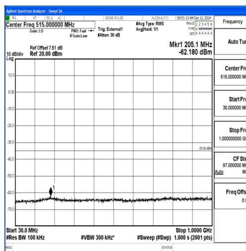
Band38_10MHz_16QAM_37800_1RB#0_30~1000_30~1000
