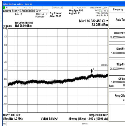
Band38_10MHz_16QAM_37800_1RB#0_1000~20000_1000~20000
