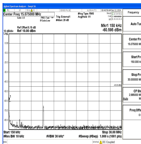
Band38_10MHz_QPSK_37800_1RB#0_0.15~30_0.15~30
