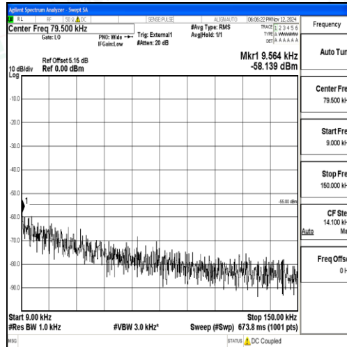
Band38_15MHz_16QAM_37825_1RB#0_0.009~0.15_0.009~0.15
