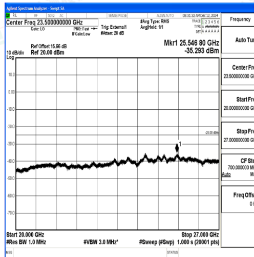
Band38_5MHz_16QAM_38225_1RB#0_20000~27000_20000~27000
