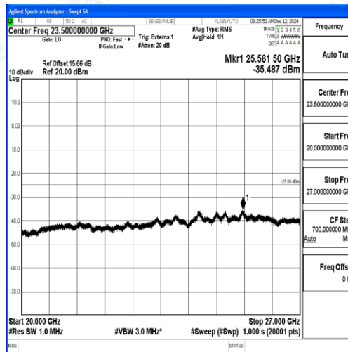
Band38_5MHz_QPSK_38000_1RB#0_20000~27000_20000~27000
