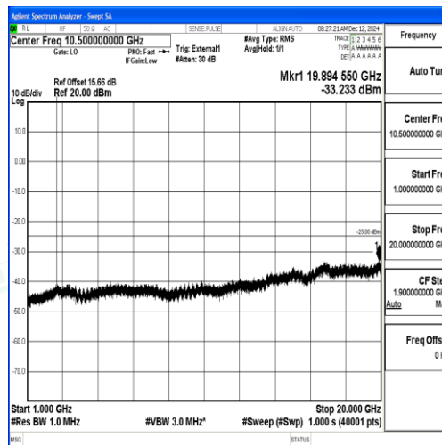
Band38_5MHz_16QAM_38000_1RB#0_1000~20000_1000~20000
