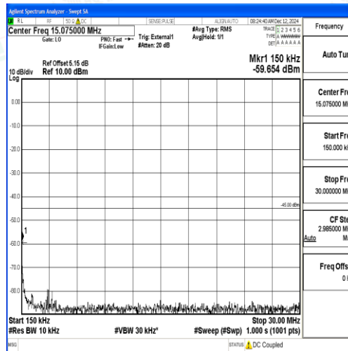
Band38_5MHz_QPSK_38000_1RB#0_0.15~30_0.15~30
