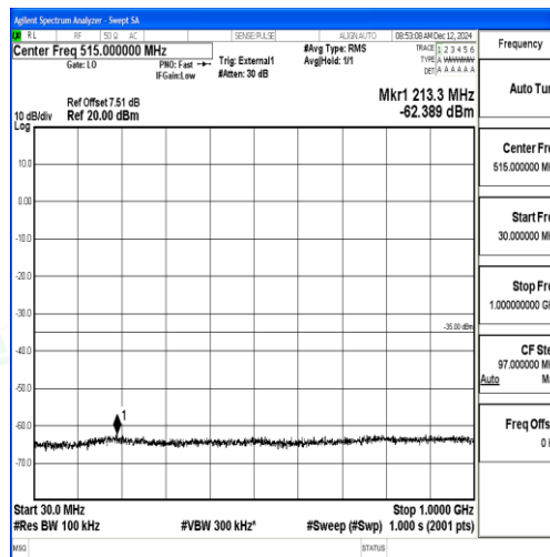
Band38_10MHz_QPSK_38000_1RB#0_30~1000_30~1000
