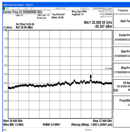
Band38_5MHz_QPSK_38225_1RB#0_20000~27000_20000~27000
