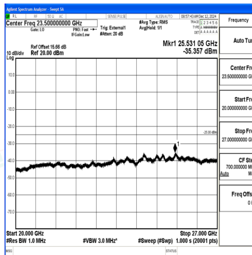
Band38_10MHz_QPSK_38200_1RB#0_20000~27000_20000~27000
