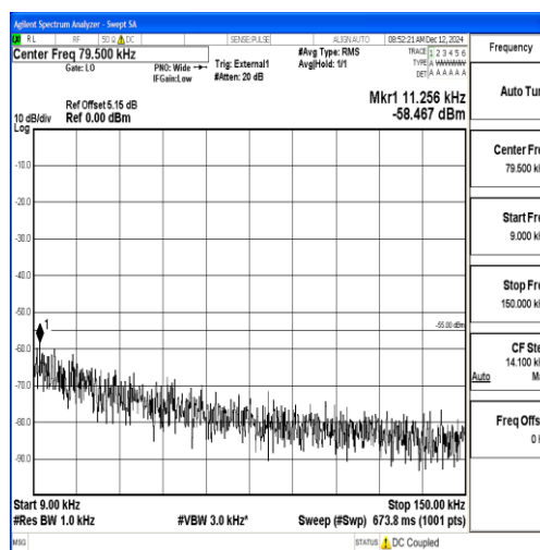
Band38_10MHz_QPSK_38000_1RB#0_0.009~0.15_0.009~0.15
