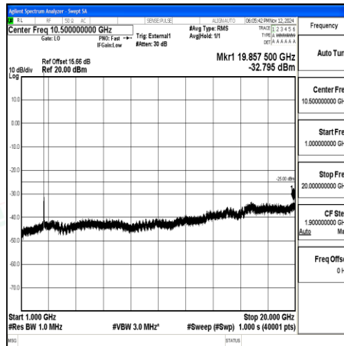
Band38_15MHz_QPSK_37825_1RB#0_1000~20000_1000~20000
