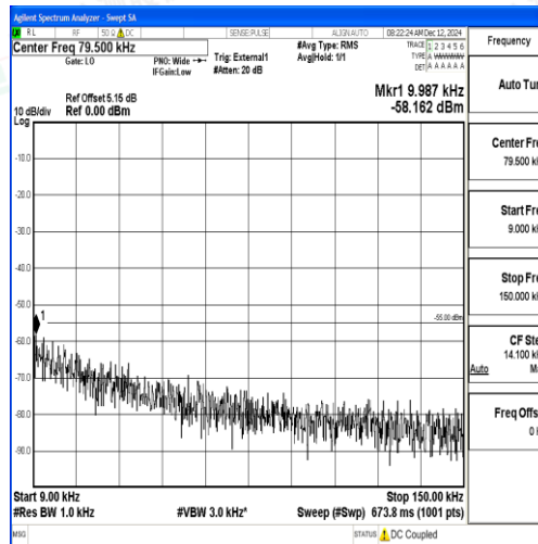
Band38_5MHz_16QAM_37775_1RB#0_0.009~0.15_0.009~0.15
