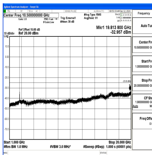
Band38_10MHz_QPSK_38000_1RB#0_1000~20000_1000~20000
