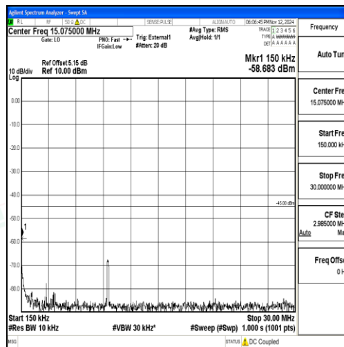
Band38_15MHz_16QAM_37825_1RB#0_0.15~30_0.15~30
