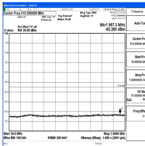
Band38_10MHz_16QAM_38200_1RB#0_30~1000_30~1000
