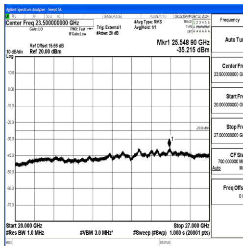
Band38_5MHz_QPSK_37775_1RB#0_20000~27000_20000~27000
