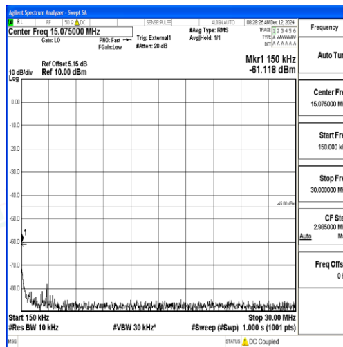
Band38_5MHz_QPSK_38225_1RB#0_0.15~30_0.15~30
