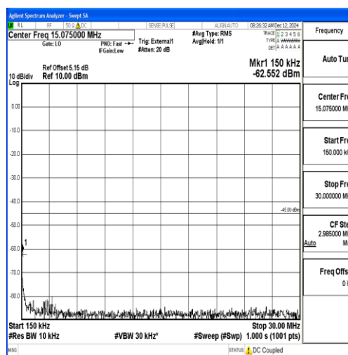
Band38_5MHz_16QAM_38000_1RB#0_0.15~30_0.15~30
