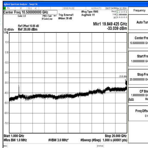
Band38_15MHz_16QAM_37825_1RB#0_1000~20000_1000~20000
