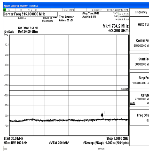
Band38_5MHz_QPSK_38225_1RB#0_30~1000_30~1000
