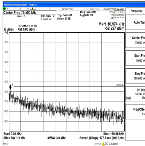
Band38_15MHz_16QAM_38000_1RB#0_0.009~0.15_0.009~0.15
