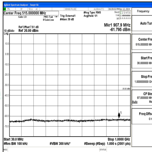
Band38_15MHz_QPSK_38000_1RB#0_30~1000_30~1000
