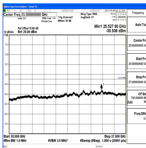
Band38_5MHz_16QAM_38000_1RB#0_20000~27000_20000~27000
