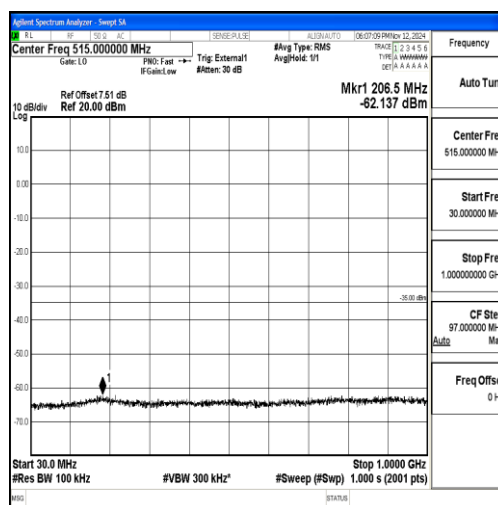
Band38_15MHz_16QAM_37825_1RB#0_30~1000_30~1000
