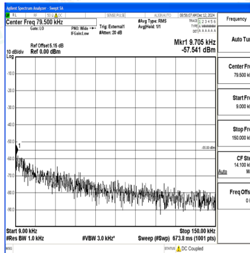
Band38_10MHz_QPSK_38200_1RB#0_0.009~0.15_0.009~0.15
