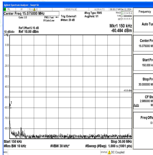
Band38_5MHz_16QAM_38225_1RB#0_0.15~30_0.15~30
