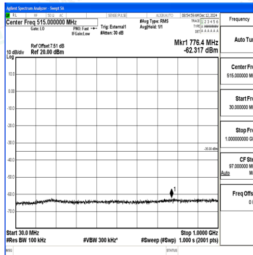
Band38_10MHz_16QAM_38000_1RB#0_30~1000_30~1000
