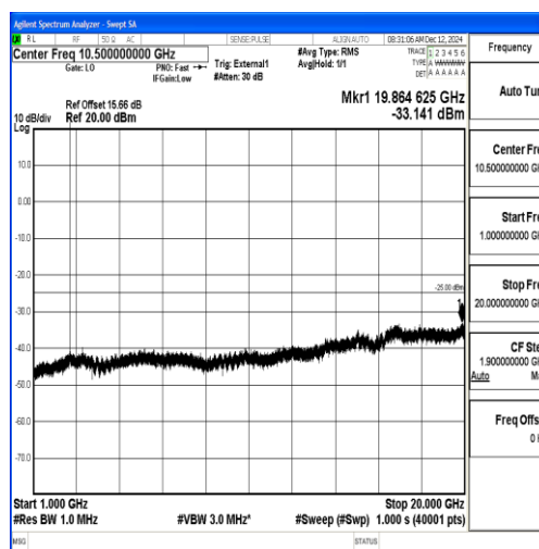
Band38_5MHz_16QAM_38225_1RB#0_1000~20000_1000~20000
