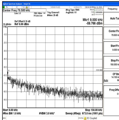
Band38_15MHz_QPSK_37825_1RB#0_0.009~0.15_0.009~0.15
