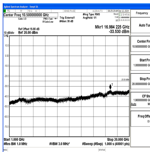
Band38_5MHz_QPSK_38000_1RB#0_1000~20000_1000~20000
