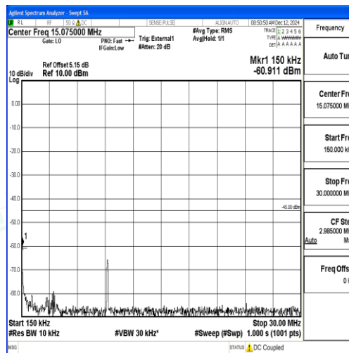
Band38_10MHz_16QAM_37800_1RB#0_0.15~30_0.15~30
