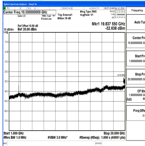
Band38_10MHz_QPSK_38200_1RB#0_1000~20000_1000~20000
