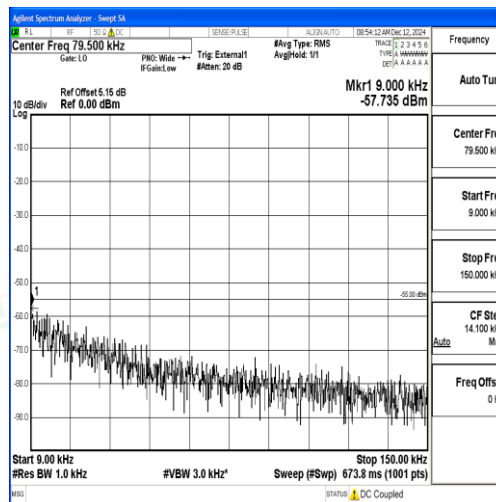
Band38_10MHz_16QAM_38000_1RB#0_0.009~0.15_0.009~0.15
