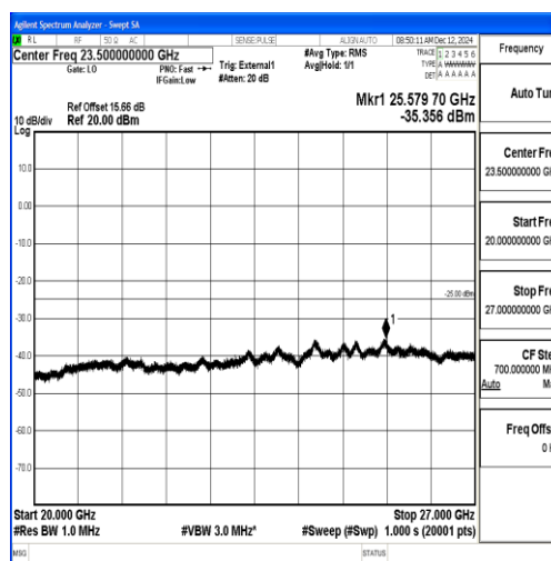
Band38_10MHz_QPSK_37800_1RB#0_20000~27000_20000~27000
