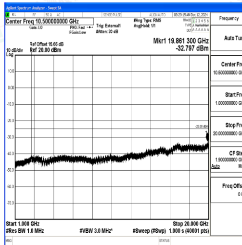
Band38_5MHz_QPSK_38225_1RB#0_1000~20000_1000~20000
