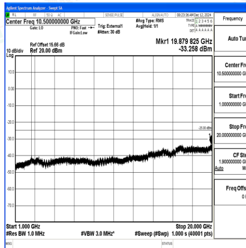
Band38_5MHz_16QAM_37775_1RB#0_1000~20000_1000~20000
