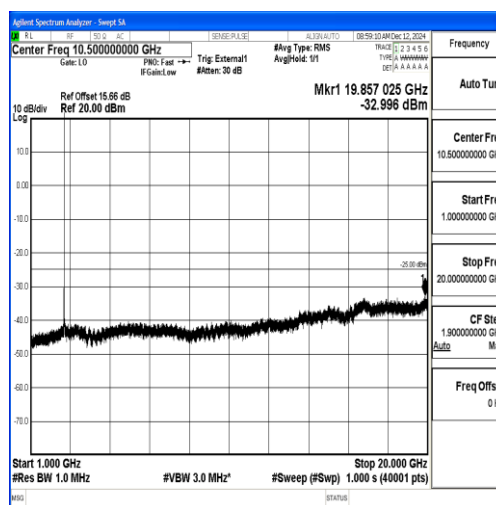
Band38_10MHz_16QAM_38200_1RB#0_1000~20000_1000~20000
