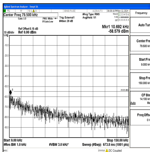
Band38_15MHz_QPSK_38000_1RB#0_0.009~0.15_0.009~0.15
