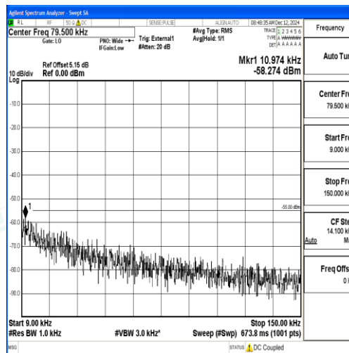
Band38_10MHz_QPSK_37800_1RB#0_0.009~0.15_0.009~0.15
