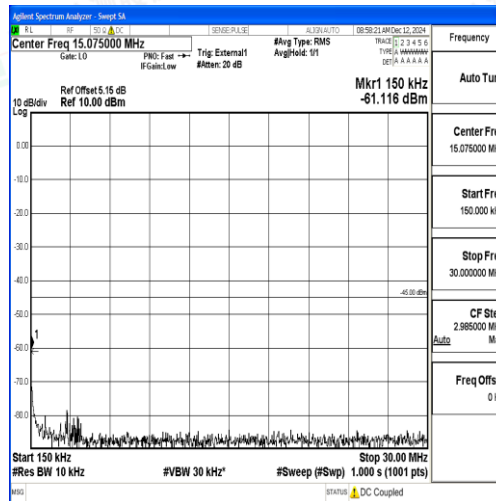
Band38_10MHz_16QAM_38200_1RB#0_0.15~30_0.15~30
