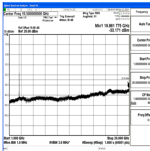
Band38_10MHz_QPSK_37800_1RB#0_1000~20000_1000~20000
