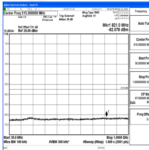
Band38_5MHz_16QAM_38000_1RB#0_30~1000_30~1000
