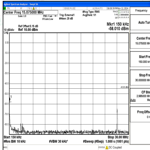
Band38_15MHz_QPSK_38000_1RB#0_0.15~30_0.15~30
