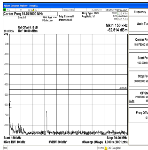
Band38_15MHz_QPSK_37825_1RB#0_0.15~30_0.15~30
