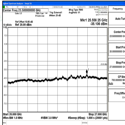
Band38_15MHz_QPSK_38000_1RB#0_20000~27000_20000~27000
