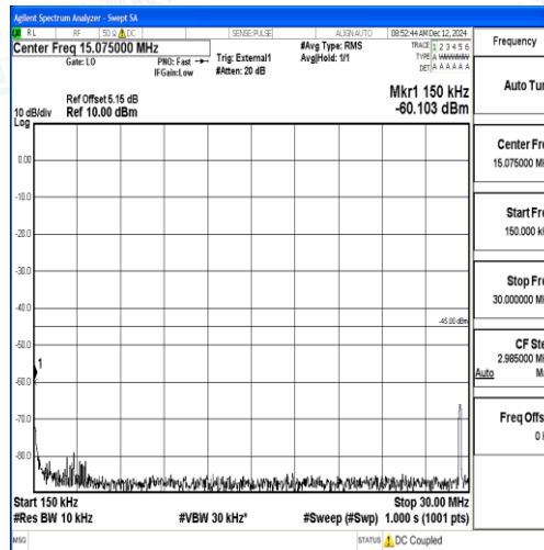
Band38_10MHz_QPSK_38000_1RB#0_0.15~30_0.15~30
