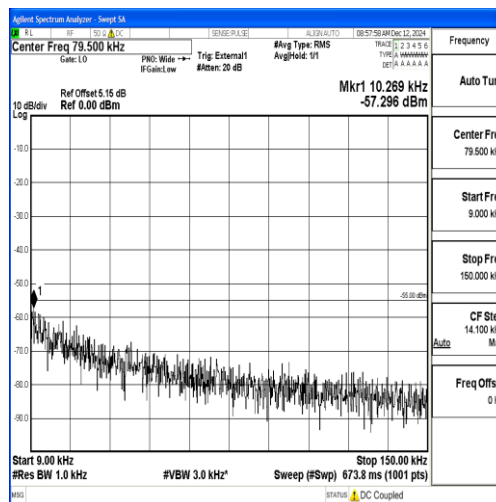
Band38_10MHz_16QAM_38200_1RB#0_0.009~0.15_0.009~0.15
