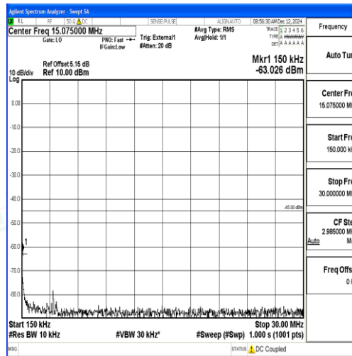
Band38_10MHz_QPSK_38200_1RB#0_0.15~30_0.15~30
