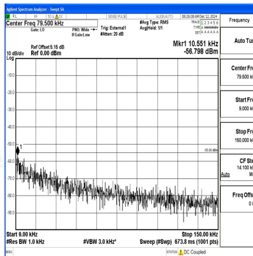
Band38_5MHz_16QAM_38000_1RB#0_0.009~0.15_0.009~0.15
