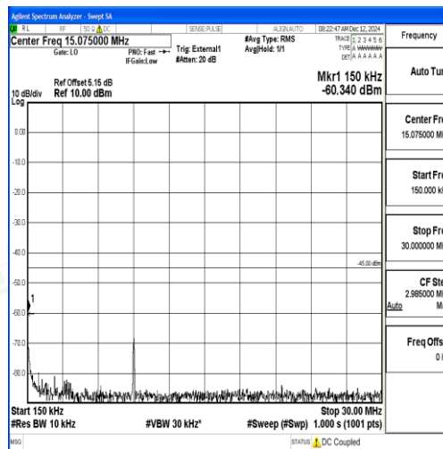
Band38_5MHz_16QAM_37775_1RB#0_0.15~30_0.15~30
