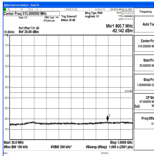
Band38_10MHz_QPSK_37800_1RB#0_30~1000_30~1000
