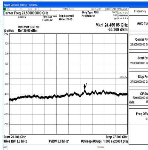
Band38_10MHz_QPSK_38000_1RB#0_20000~27000_20000~27000
