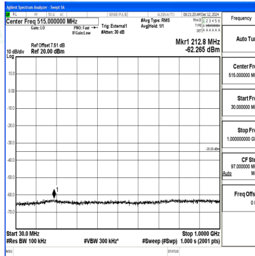
Band38_5MHz_QPSK_37775_1RB#0_30~1000_30~1000
