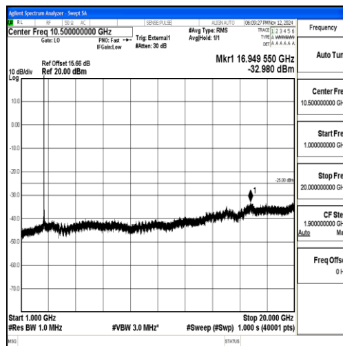
Band38_15MHz_QPSK_38000_1RB#0_1000~20000_1000~20000
