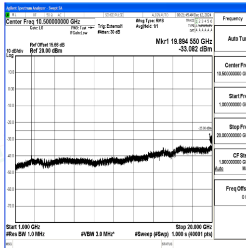
Band38_5MHz_QPSK_37775_1RB#0_1000~20000_1000~20000
