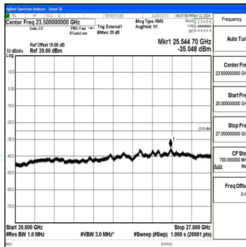
Band38_15MHz_16QAM_37825_1RB#0_20000~27000_20000~27000
