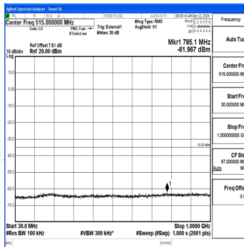
Band38_5MHz_16QAM_38225_1RB#0_30~1000_30~1000
