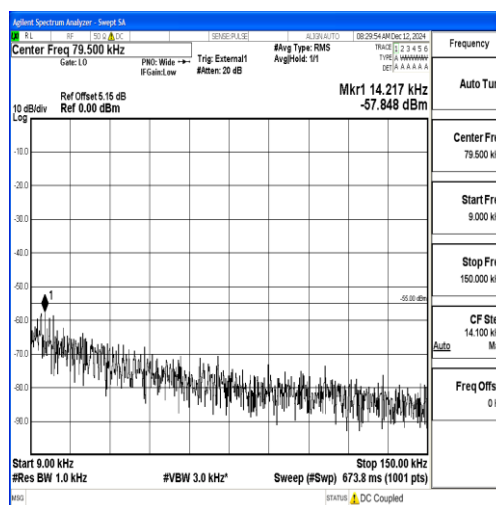
Band38_5MHz_16QAM_38225_1RB#0_0.009~0.15_0.009~0.15
