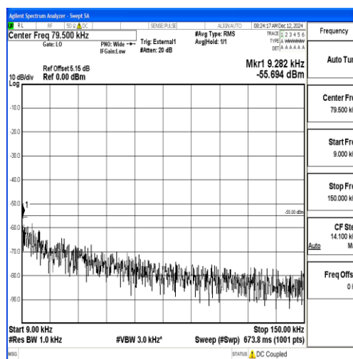
Band38_5MHz_QPSK_38000_1RB#0_0.009~0.15_0.009~0.15
