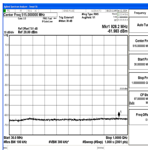
Band38_5MHz_16QAM_37775_1RB#0_30~1000_30~1000
