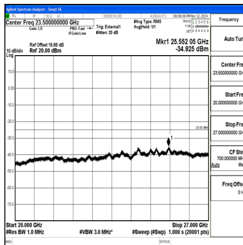
Band38_15MHz_QPSK_37825_1RB#0_20000~27000_20000~27000
