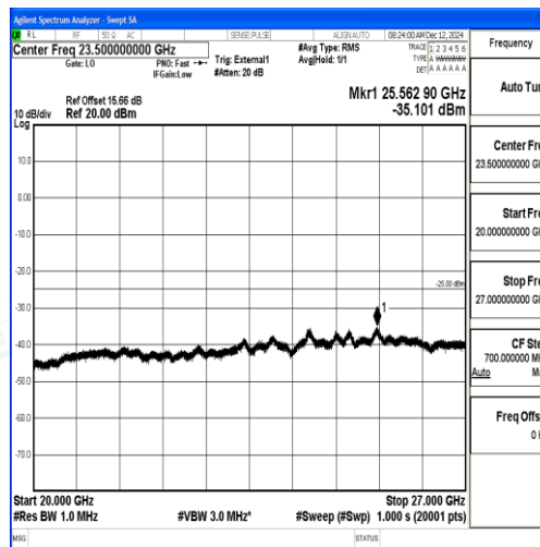
Band38_5MHz_16QAM_37775_1RB#0_20000~27000_20000~27000
