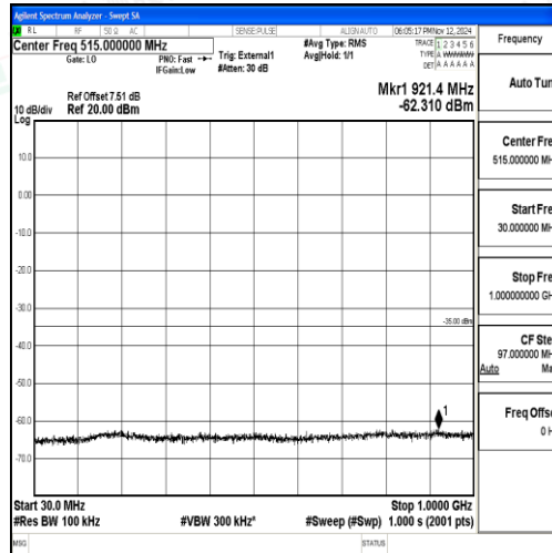
Band38_15MHz_QPSK_37825_1RB#0_30~1000_30~1000
