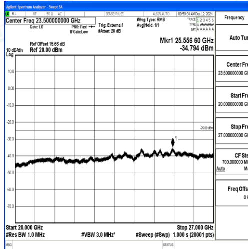
Band38_10MHz_16QAM_38200_1RB#0_20000~27000_20000~27000
