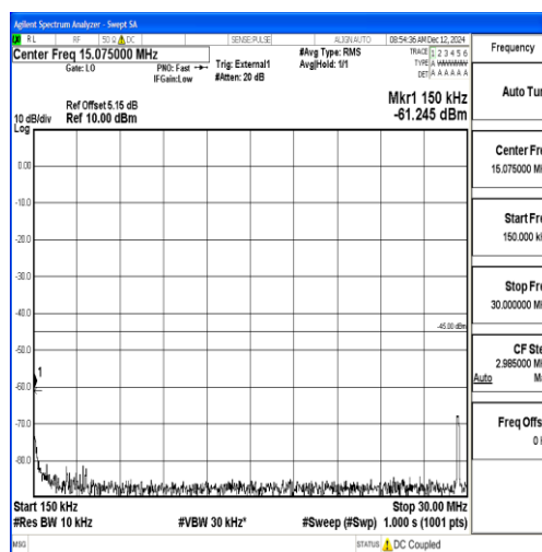
Band38_10MHz_16QAM_38000_1RB#0_0.15~30_0.15~30
