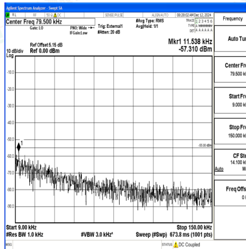
Band38_5MHz_QPSK_38225_1RB#0_0.009~0.15_0.009~0.15
