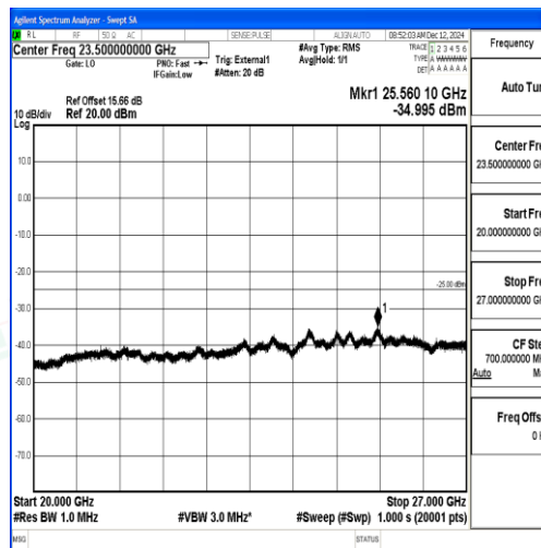
Band38_10MHz_16QAM_37800_1RB#0_20000~27000_20000~27000
