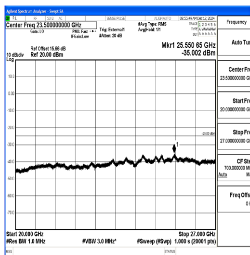
Band38_10MHz_16QAM_38000_1RB#0_20000~27000_20000~27000
