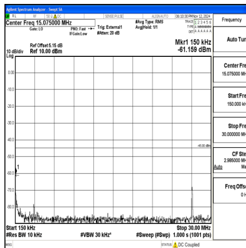
Band38_15MHz_16QAM_38000_1RB#0_0.15~30_0.15~30
