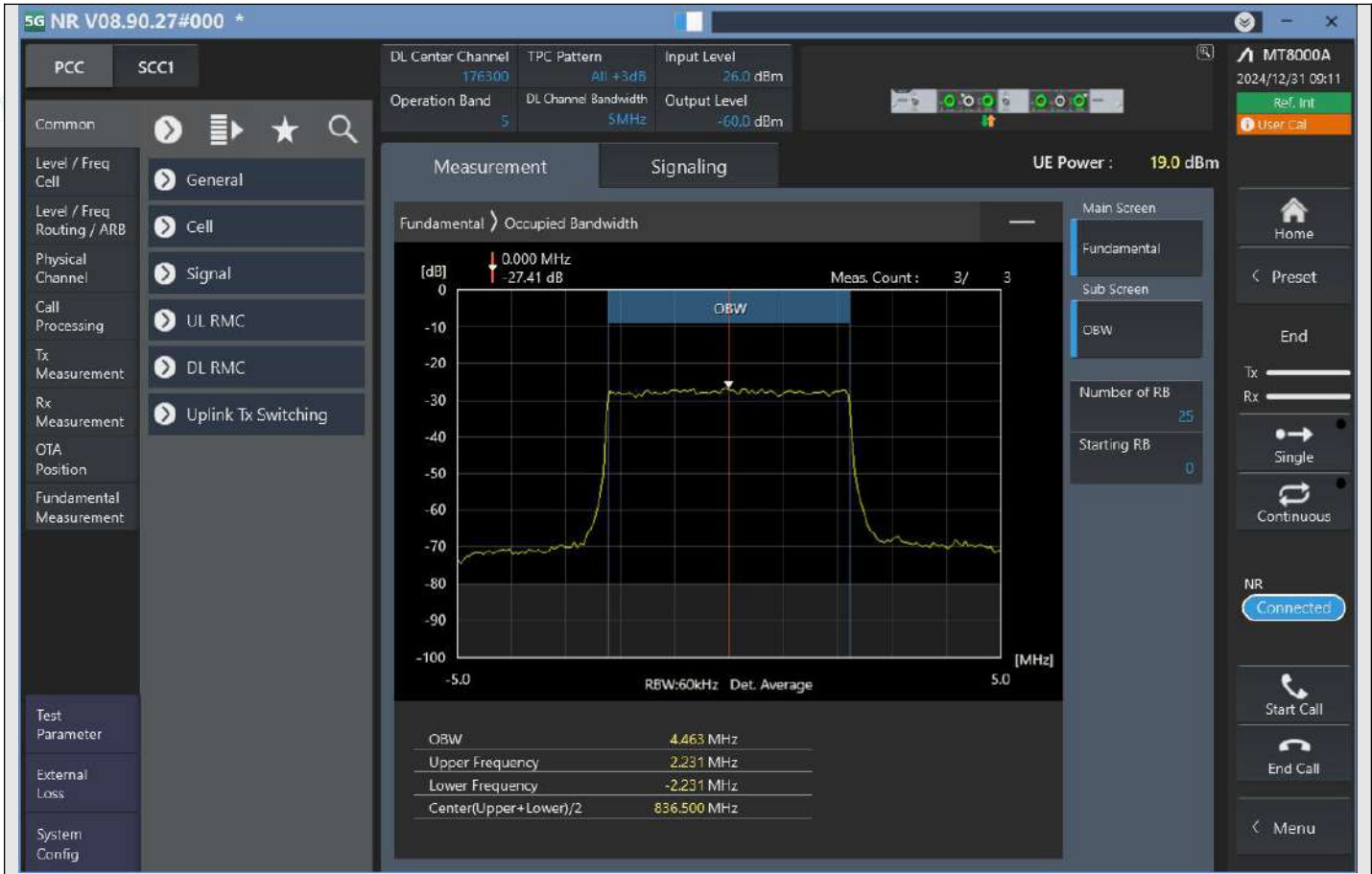
n5_5MHz_15kHz_176300_DFT-s-OFDM 64QAM^Outer_Full
