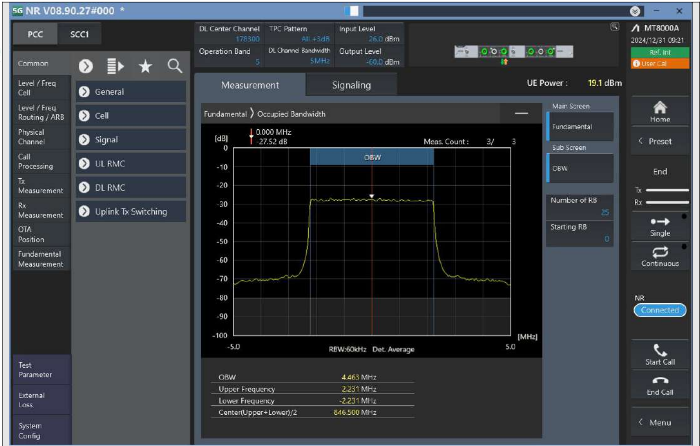
n5_5MHz_15kHz_178300_DFT-s-OFDM 64QAM^Outer_Full
