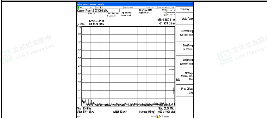
Band41_5MHz_16QAM_40620_1RB#0_0.15~30_0.15~30
