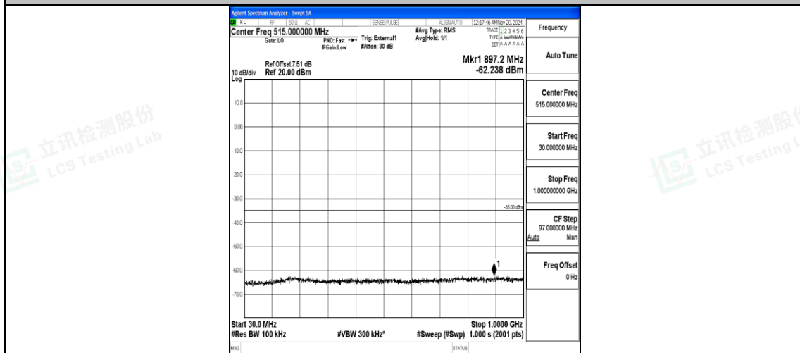
Band38_15MHz_16QAM_37825_1RB#0_30~1000_30~1000
