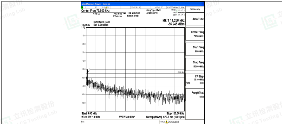
Band38_15MHz_16QAM_37825_1RB#0_0.009~0.15_0.009~0.15
