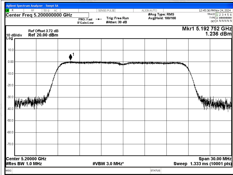
PSD NVNT ac20 5200MHz Ant7
