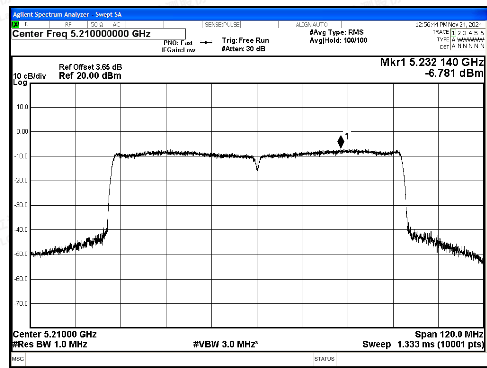
PSD NVNT ac80 5210MHz Ant7
